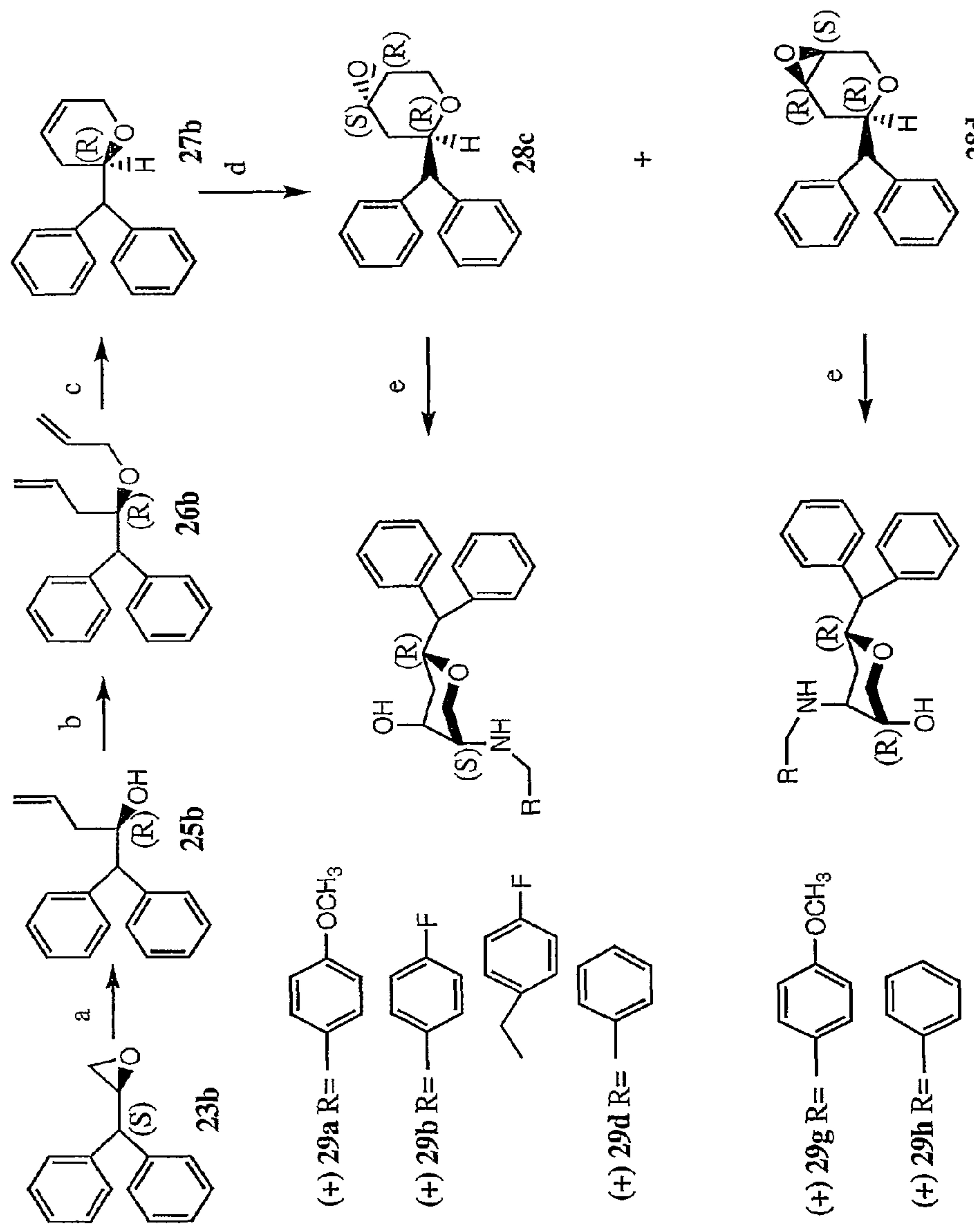
Scheme 3
