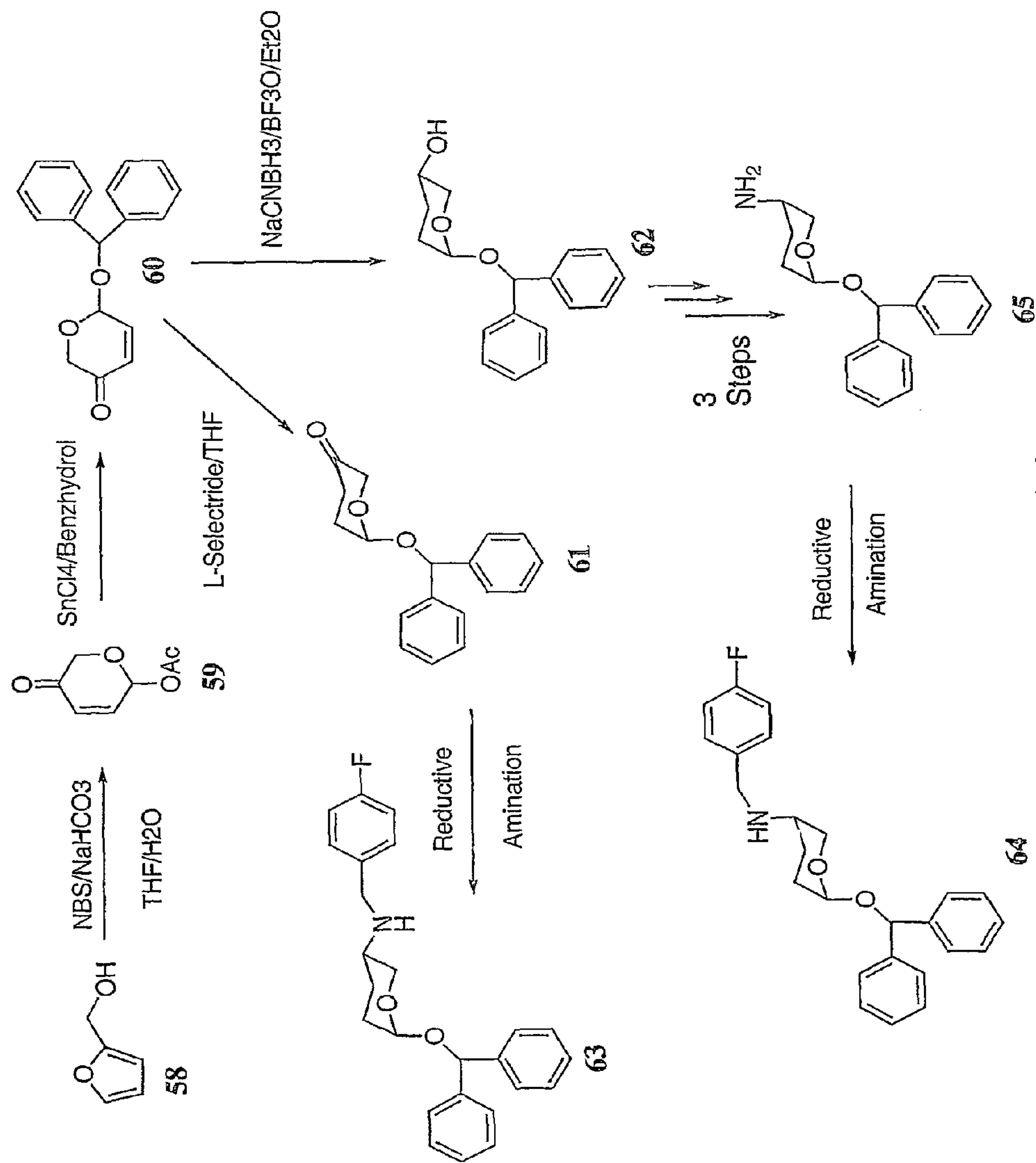
Scheme 9
