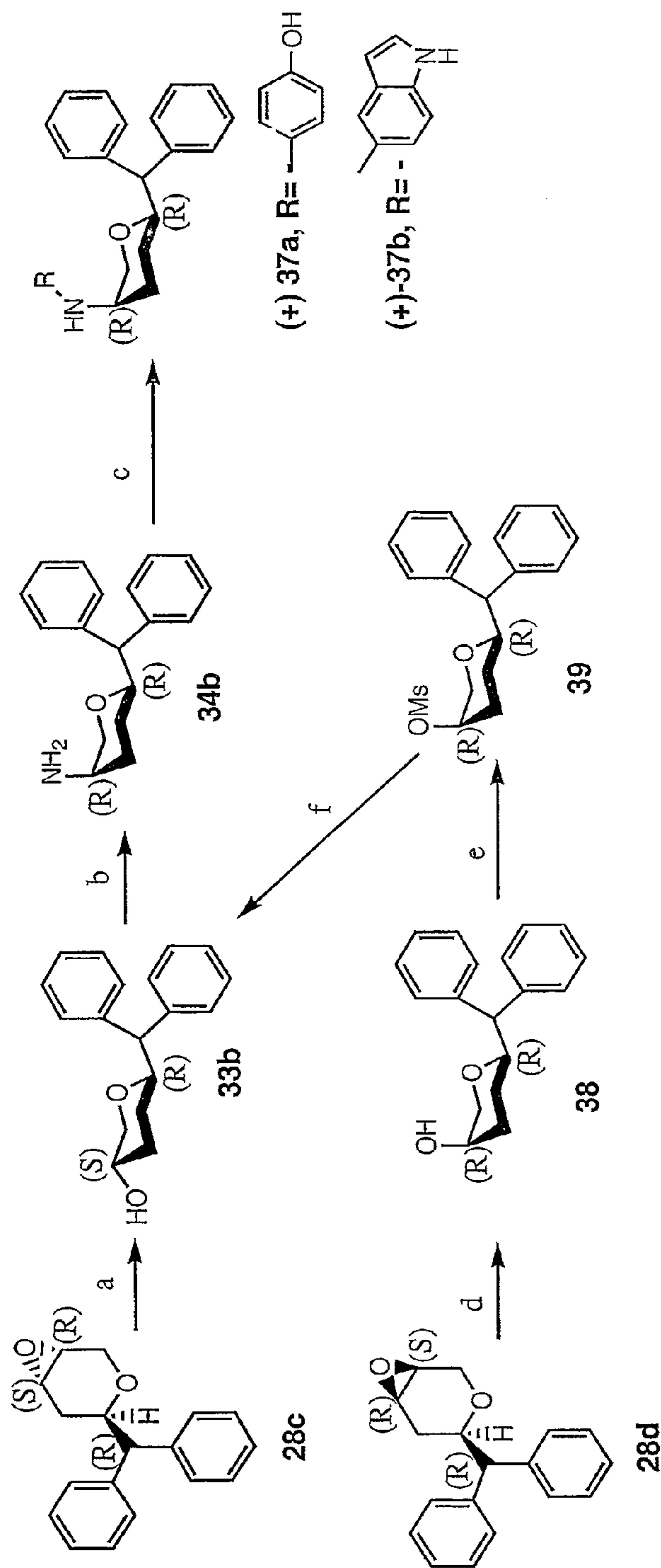
Scheme 6
