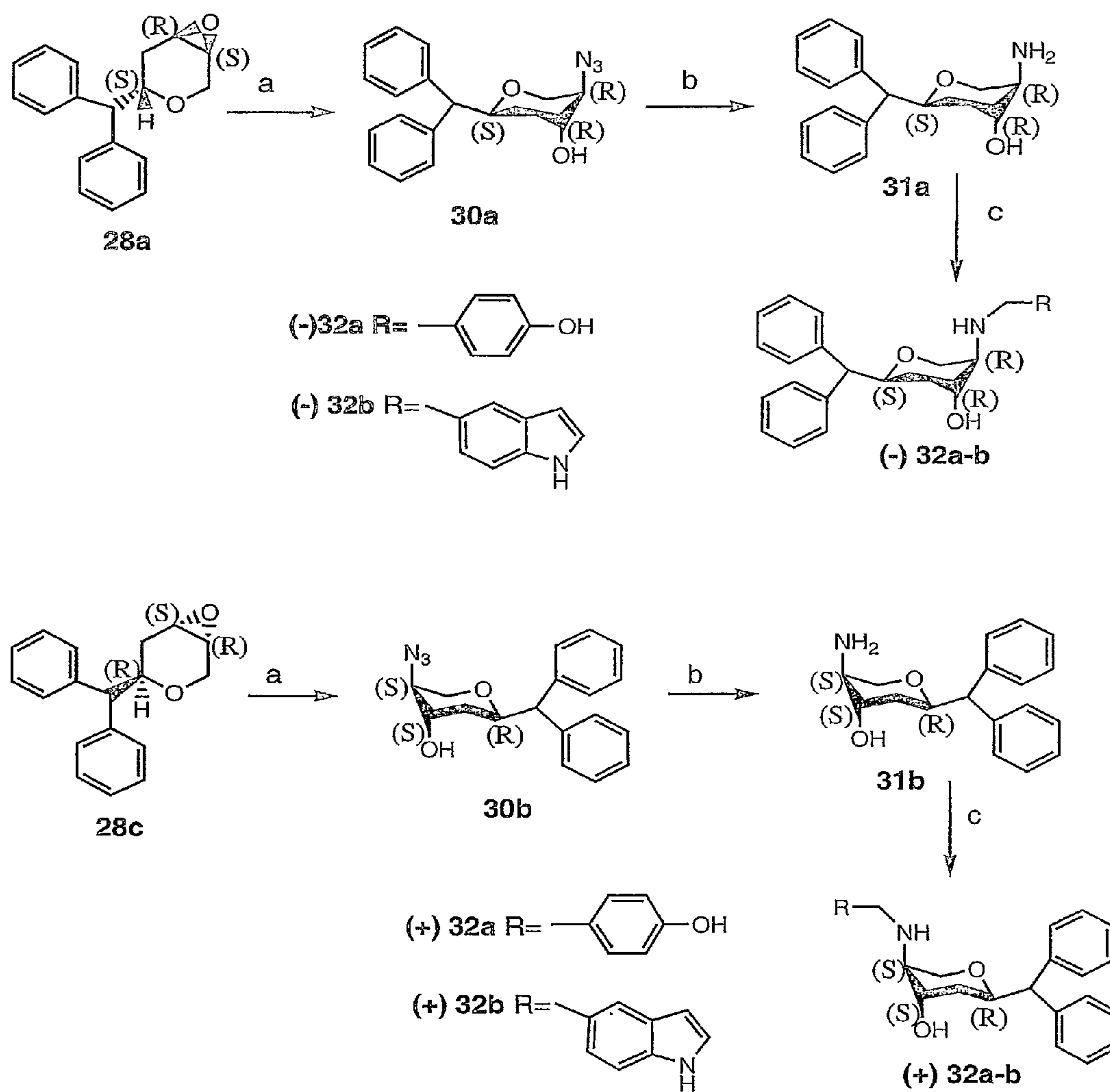
Scheme 4
