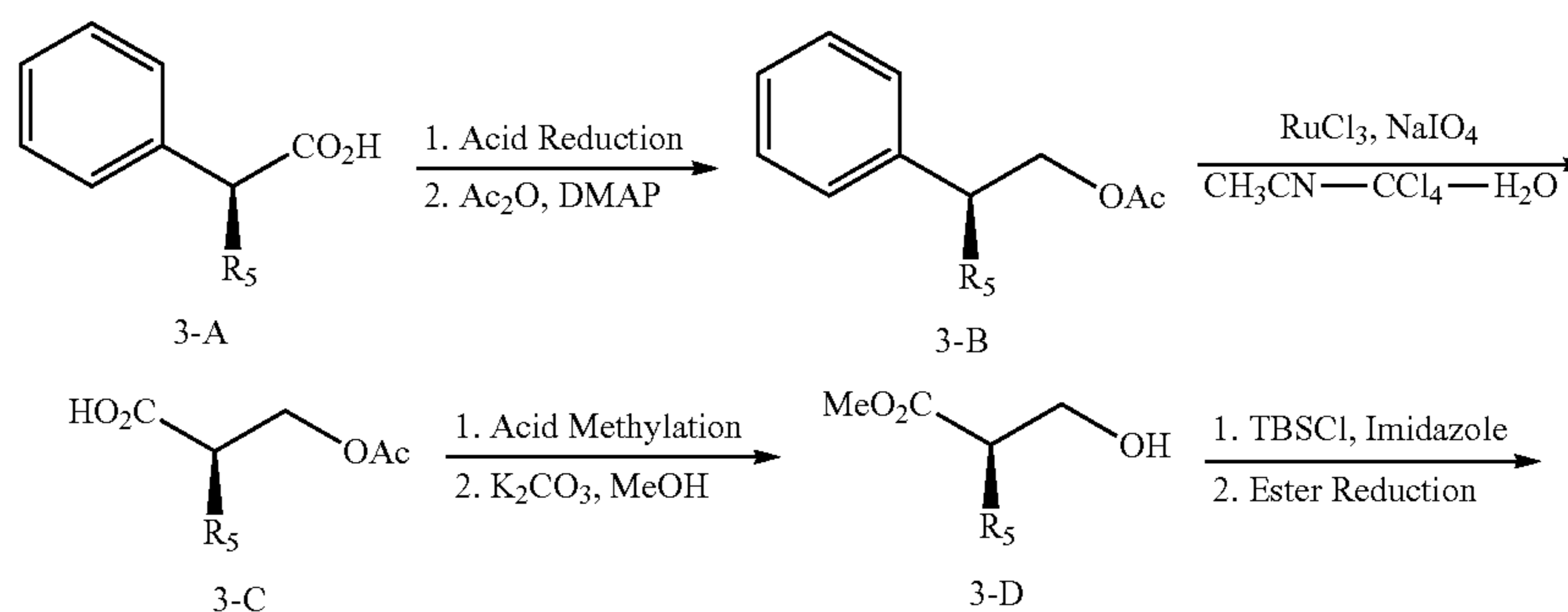
Scheme 3. Synthesis of Compound Ia1
