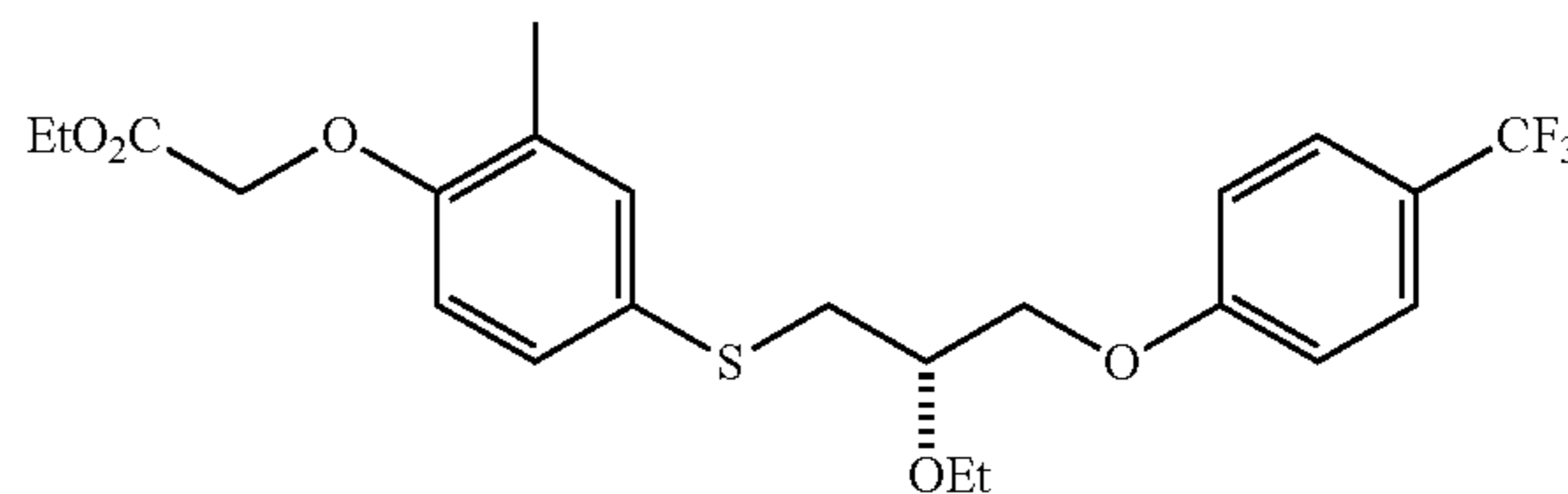
(S)-{4-[2-Ethoxy-3-(4-trifluoromethyl-phenoxy)-propylsulfanyl]-2-methyl-phenoxy}-acetic acid ethyl ester
