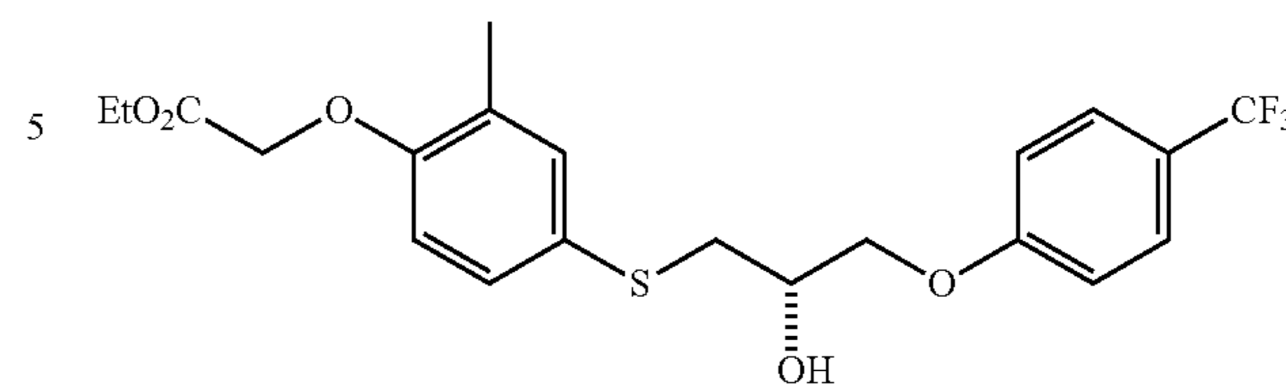
(S)-{4-[2-Hydroxy-3-(4-trifluoromethyl-phenoxy)-propylsulfanyl]-2-methyl-phenoxy}-acetic acid ethyl ester
