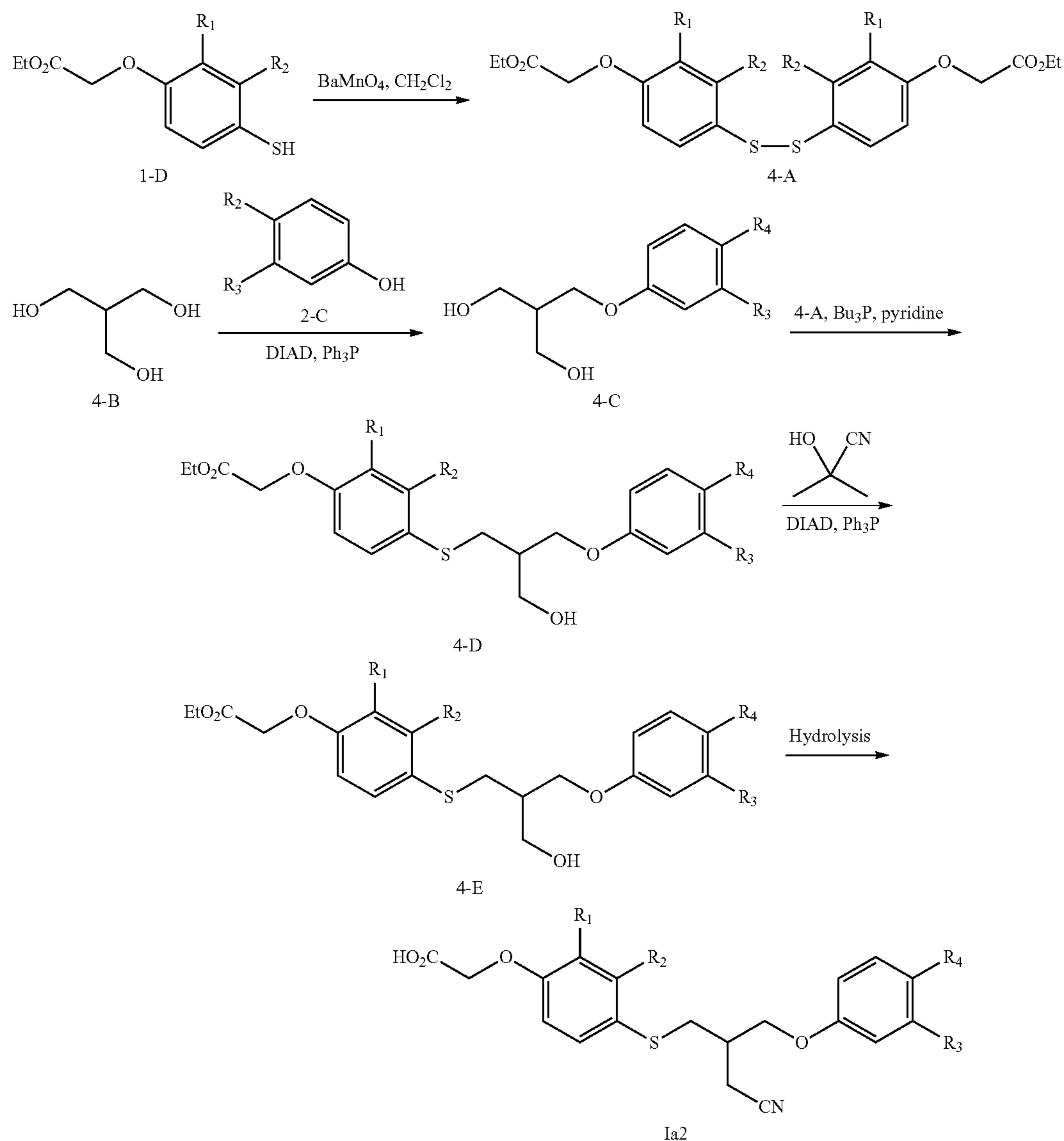
Scheme 4. Synthesis of Compound Ia2
