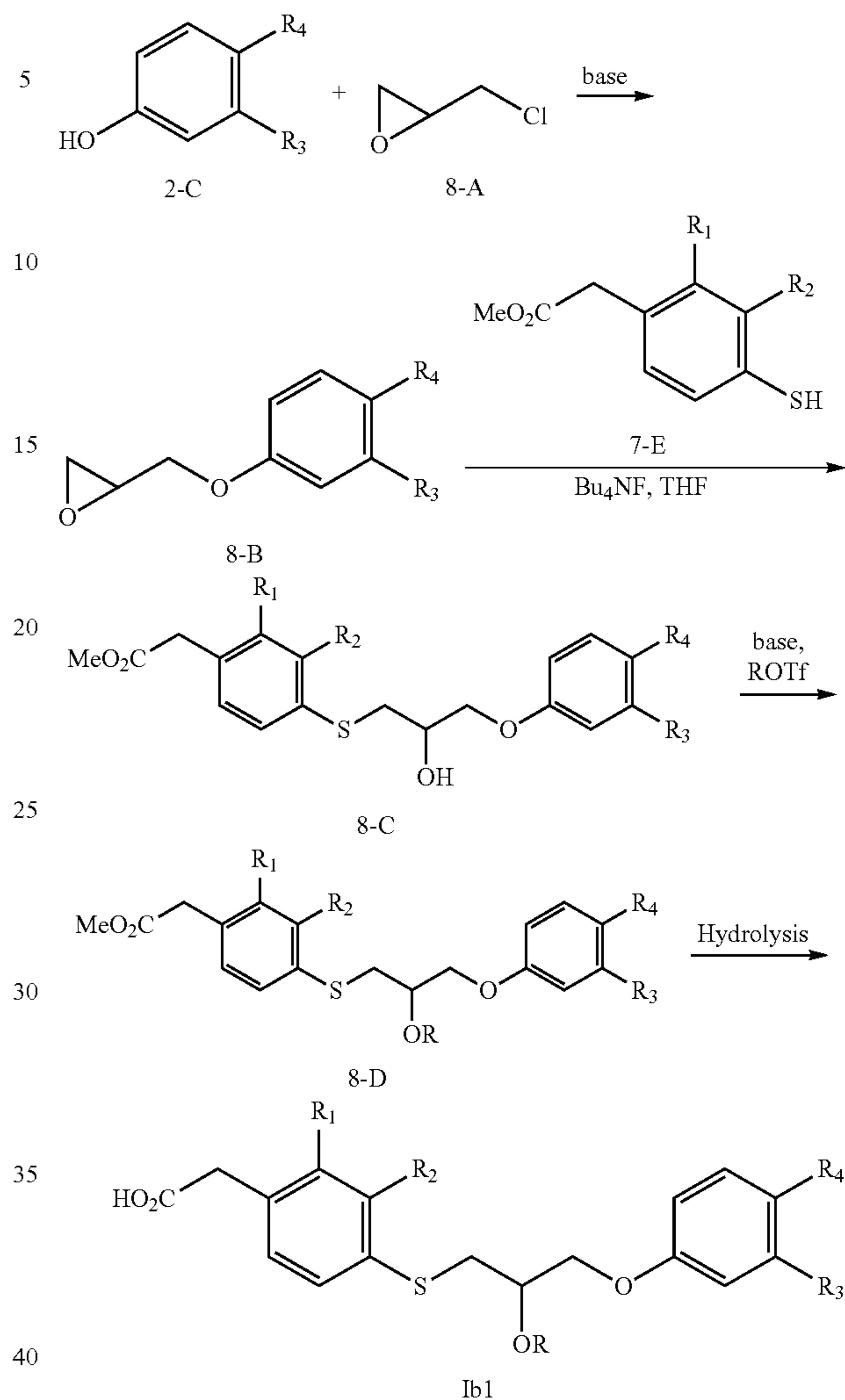
Scheme 8. Synthesis of Compound Ib1
