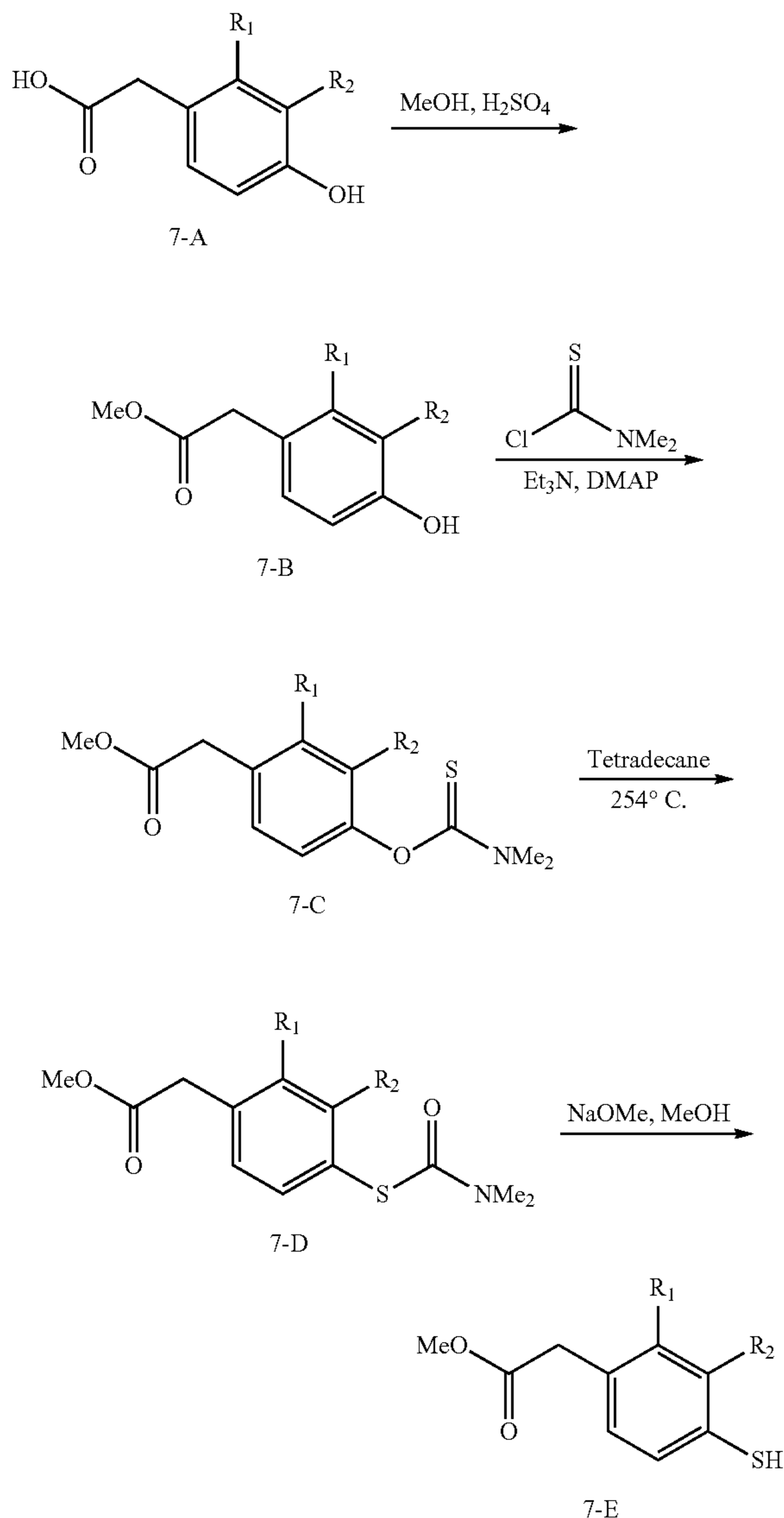
Scheme 7. Synthesis of Intermediate 7-E
