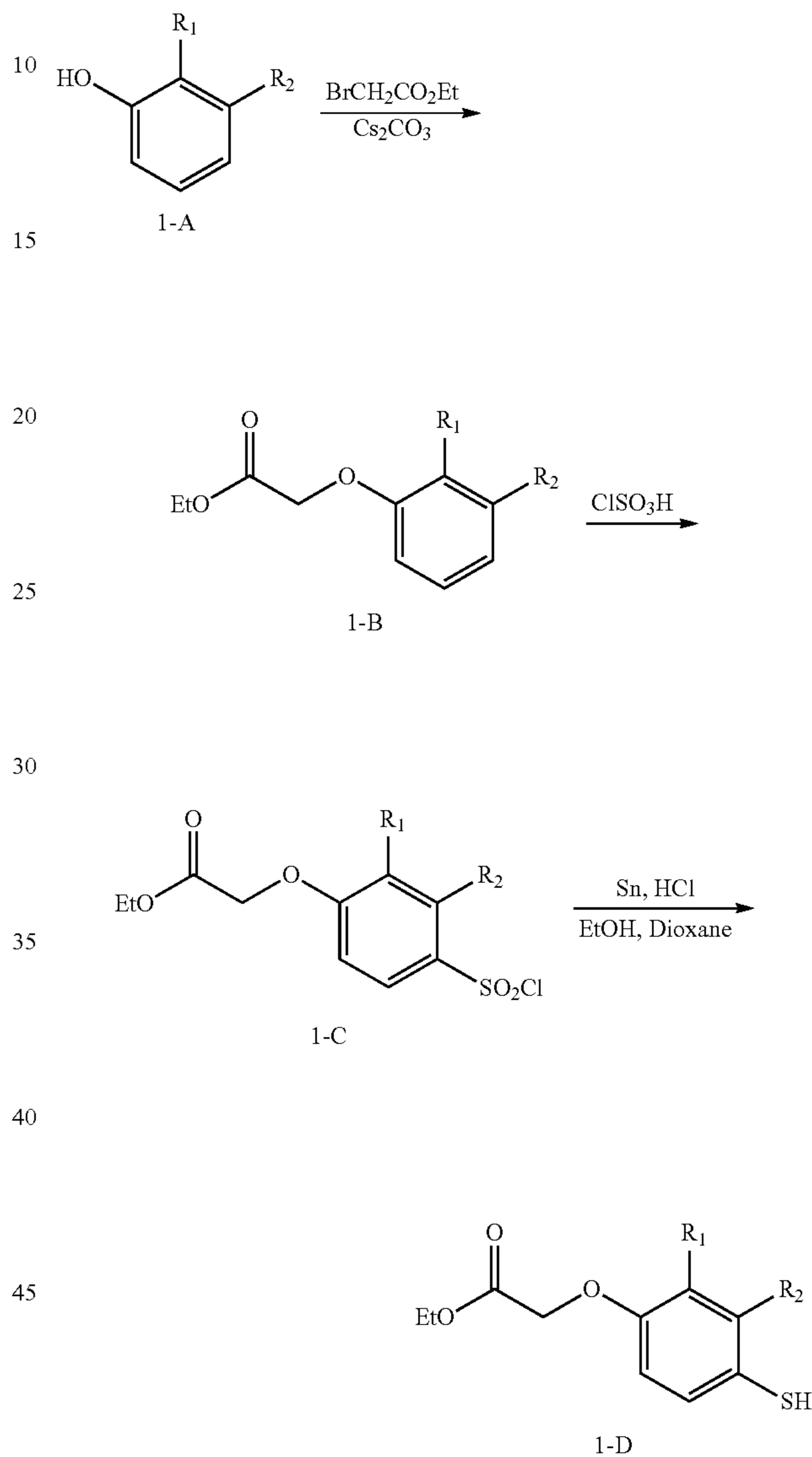
Scheme 1. Synthesis of Intermediate 1-D
