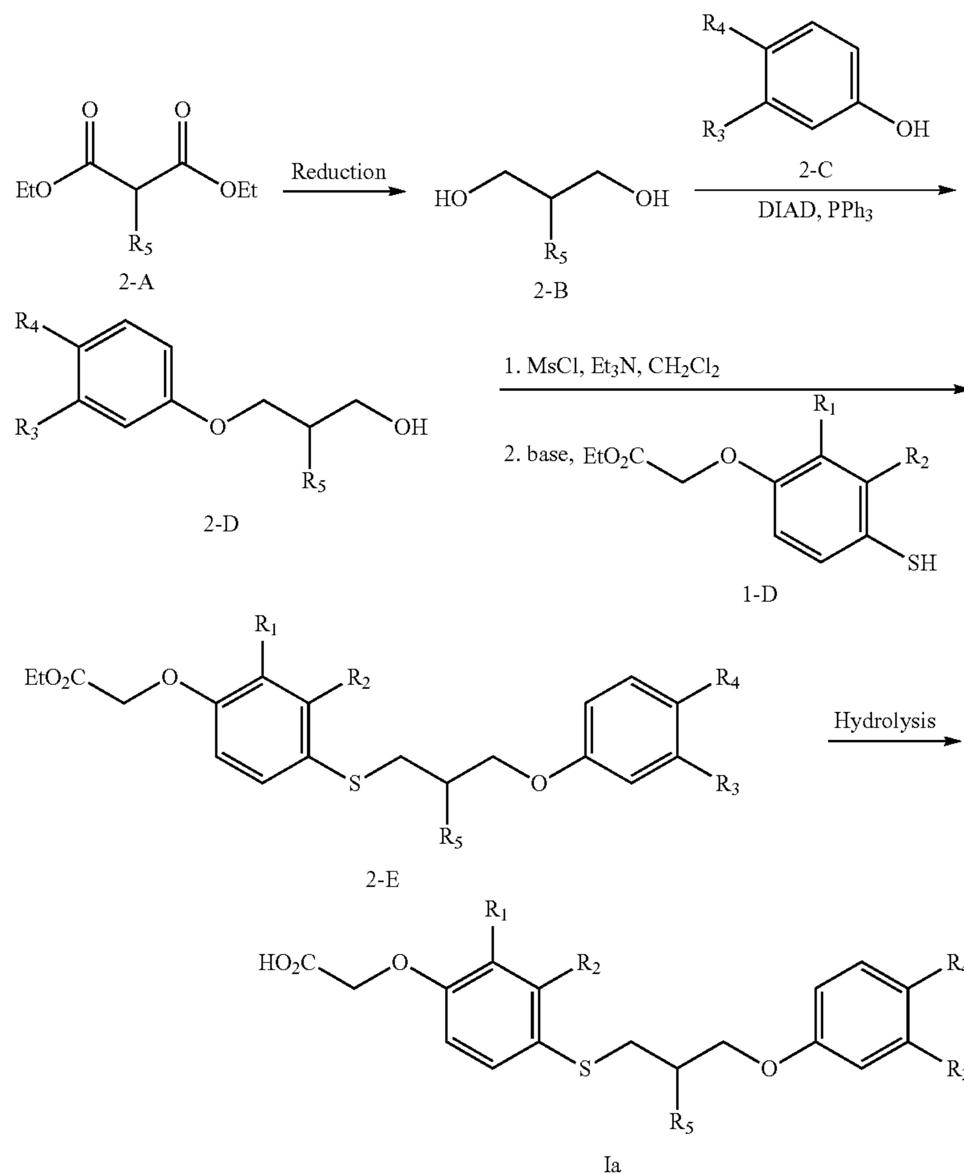
Scheme 2. Synthesis of Compound Ia
