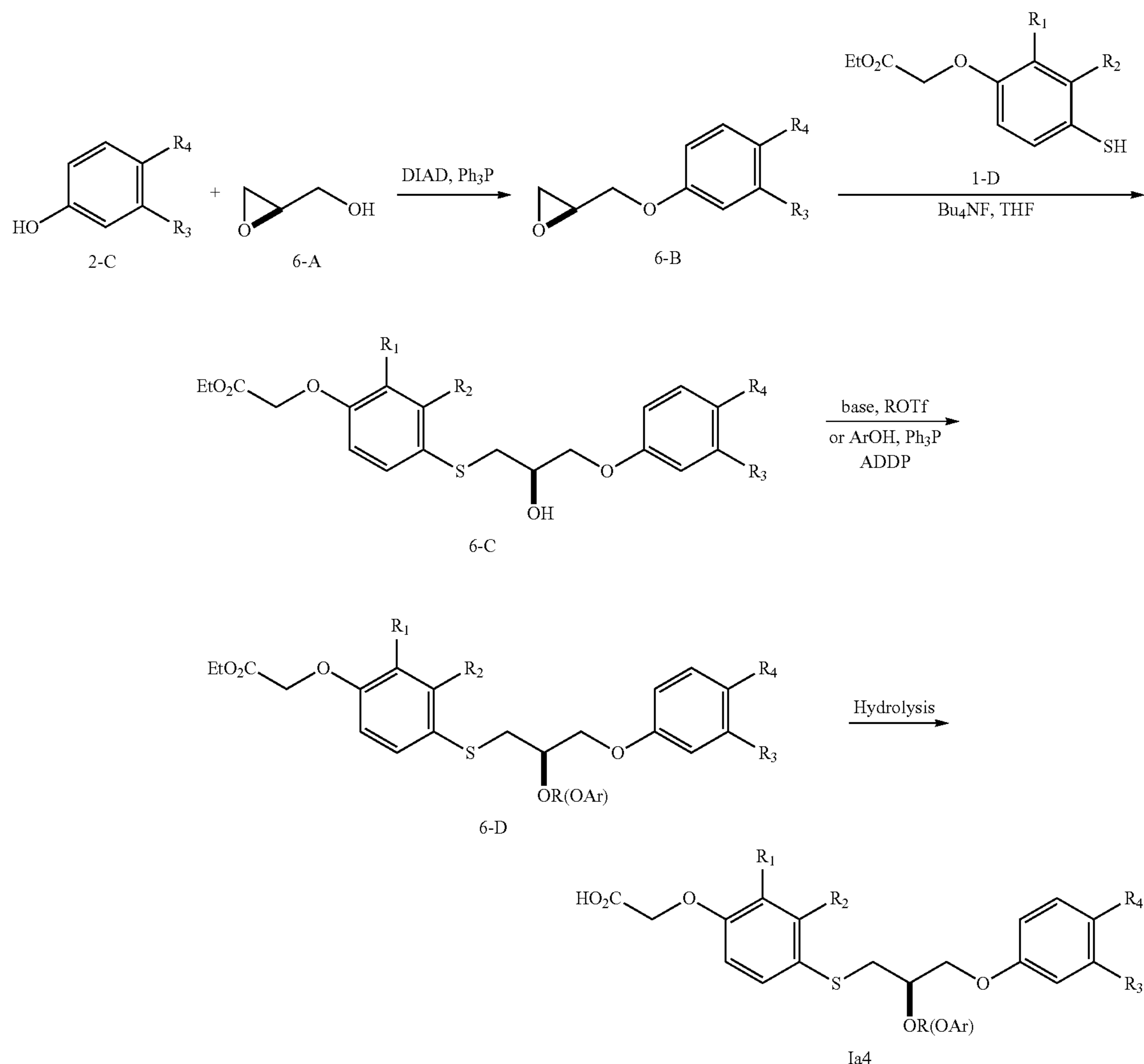
Scheme 6. Synthesis of Compound Ia4
