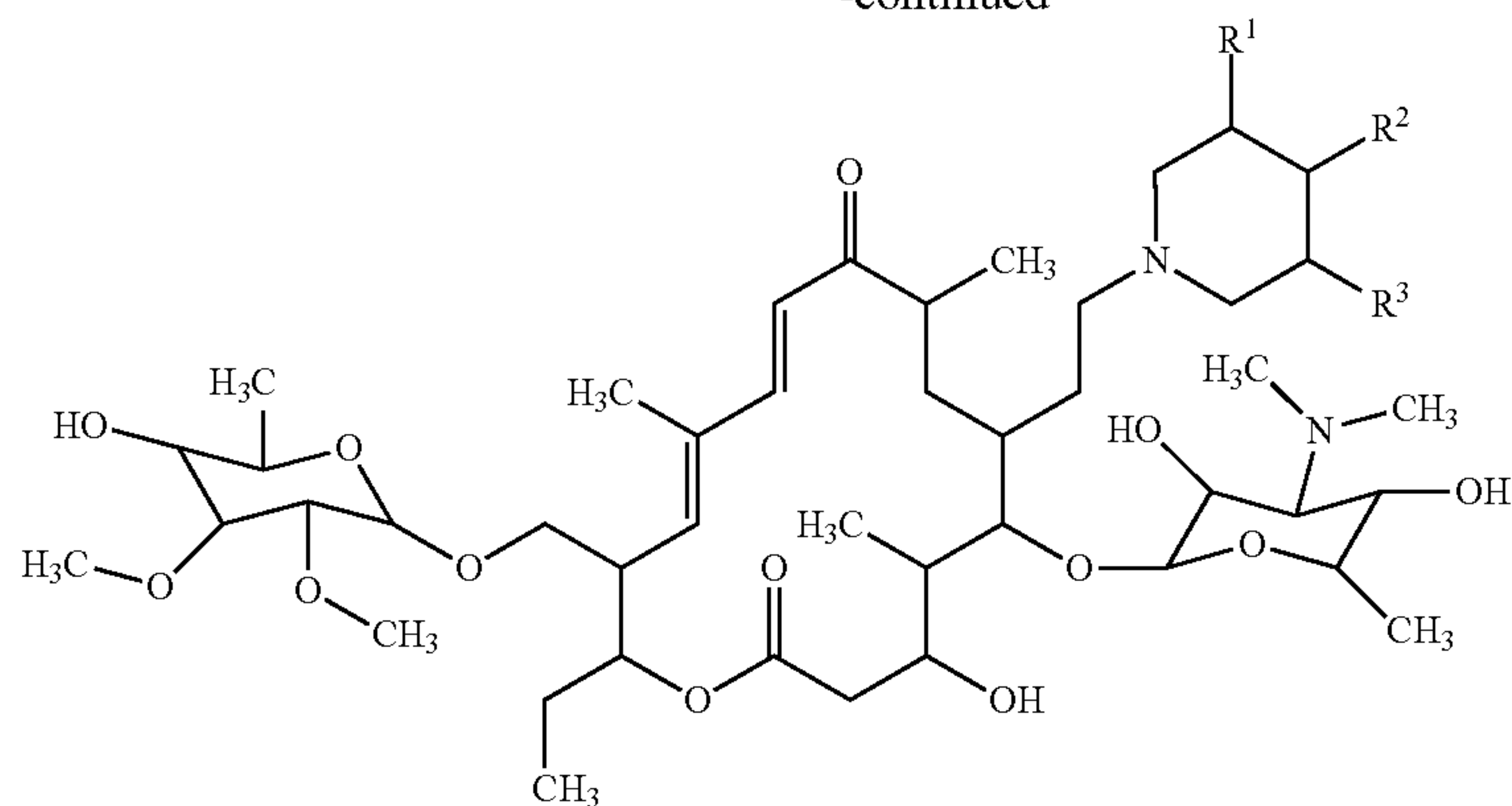
23-O-mycinosyl-20-piperidinyloxy-5-O-mycaminosyl-tylosin compound
