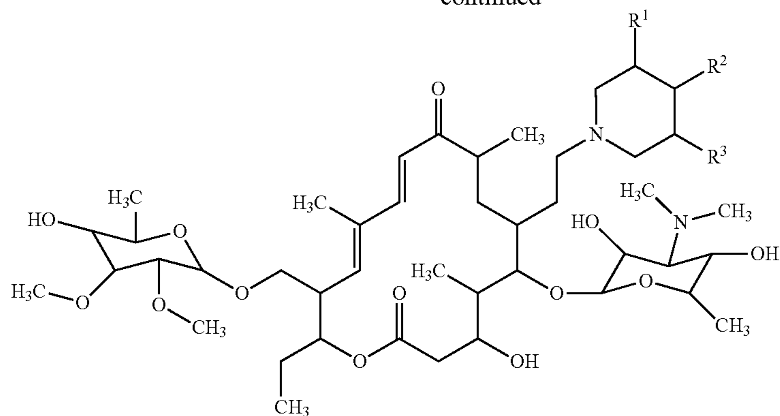
23-O-mycinosyl-20-piperidinyl-5-O-mycaminosyl-tylonolide compound
