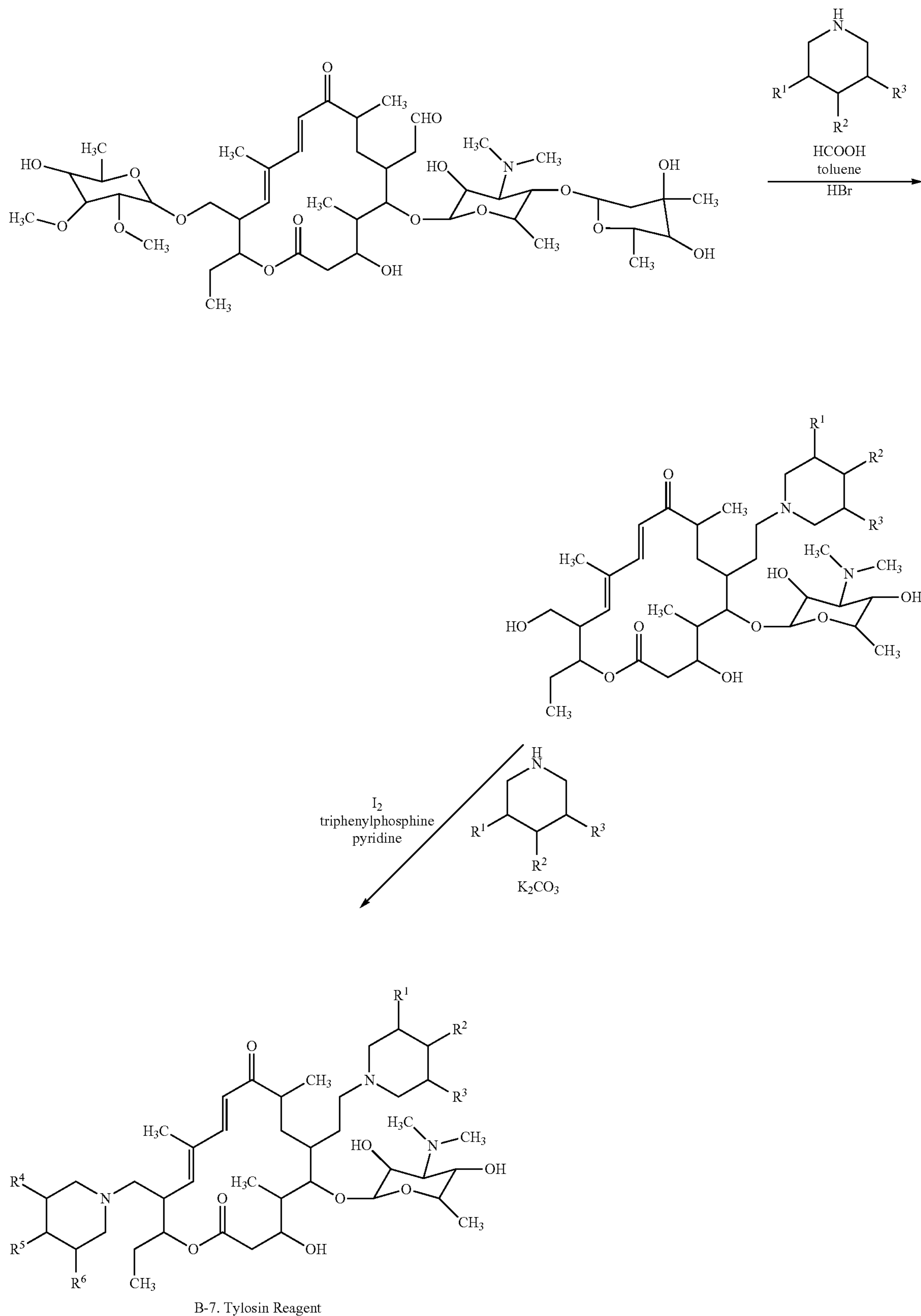
Scheme V
