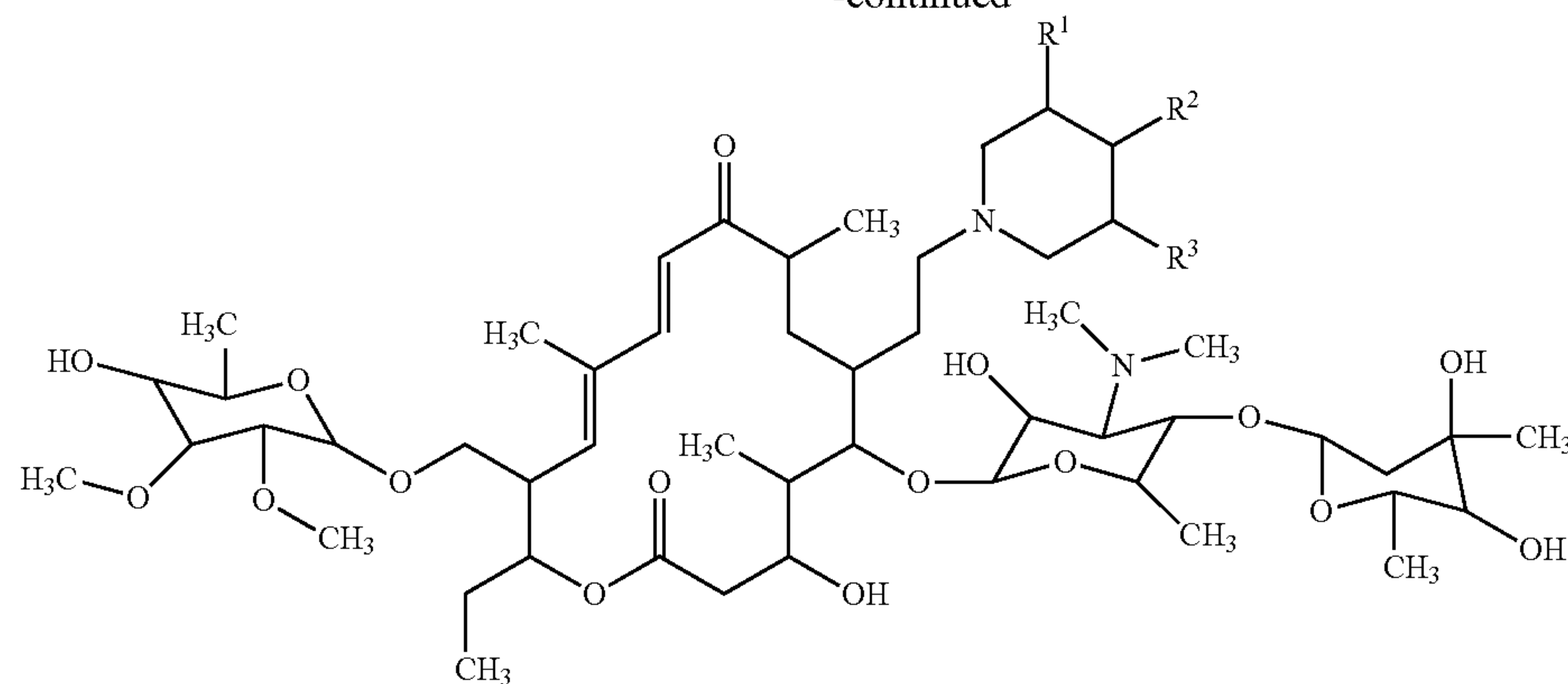
20-piperidinyl-tylosin compound
