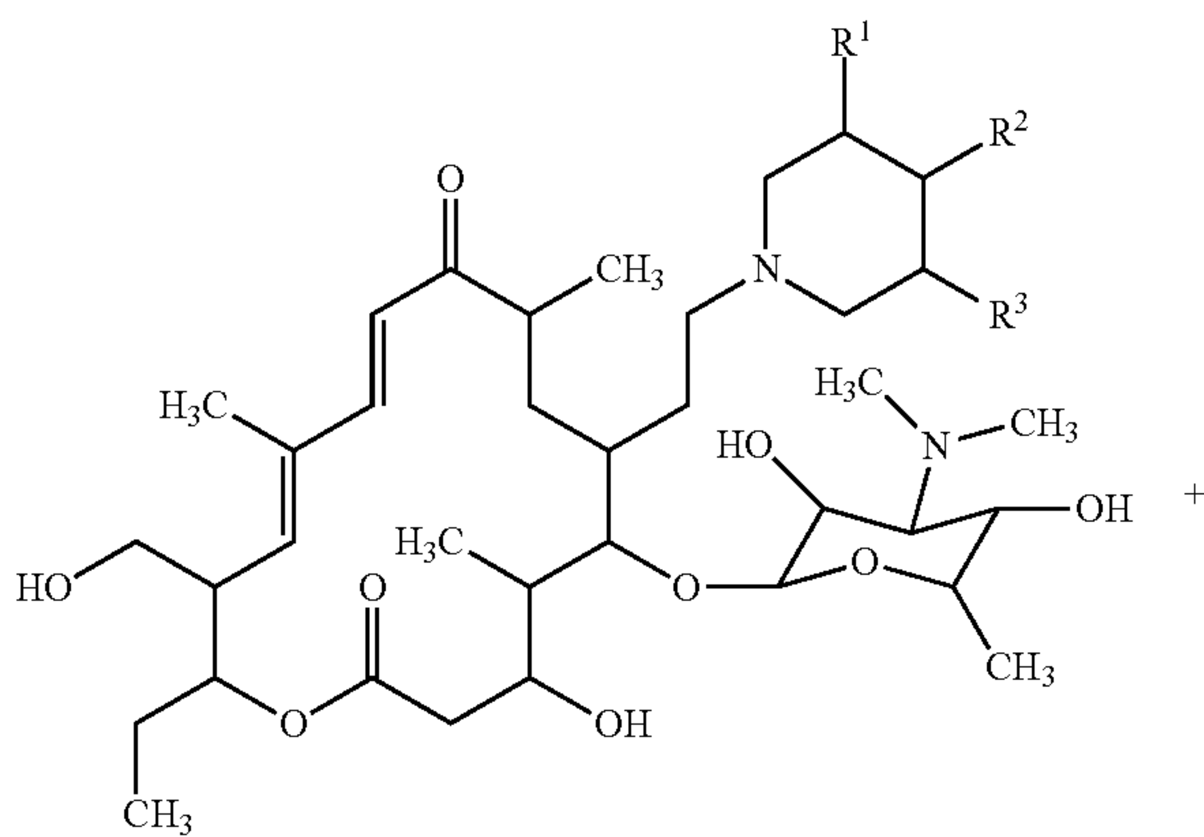
23-hydroxyl-20-piperidinyl-5-O-mycaminosyl-tylonolide compound
