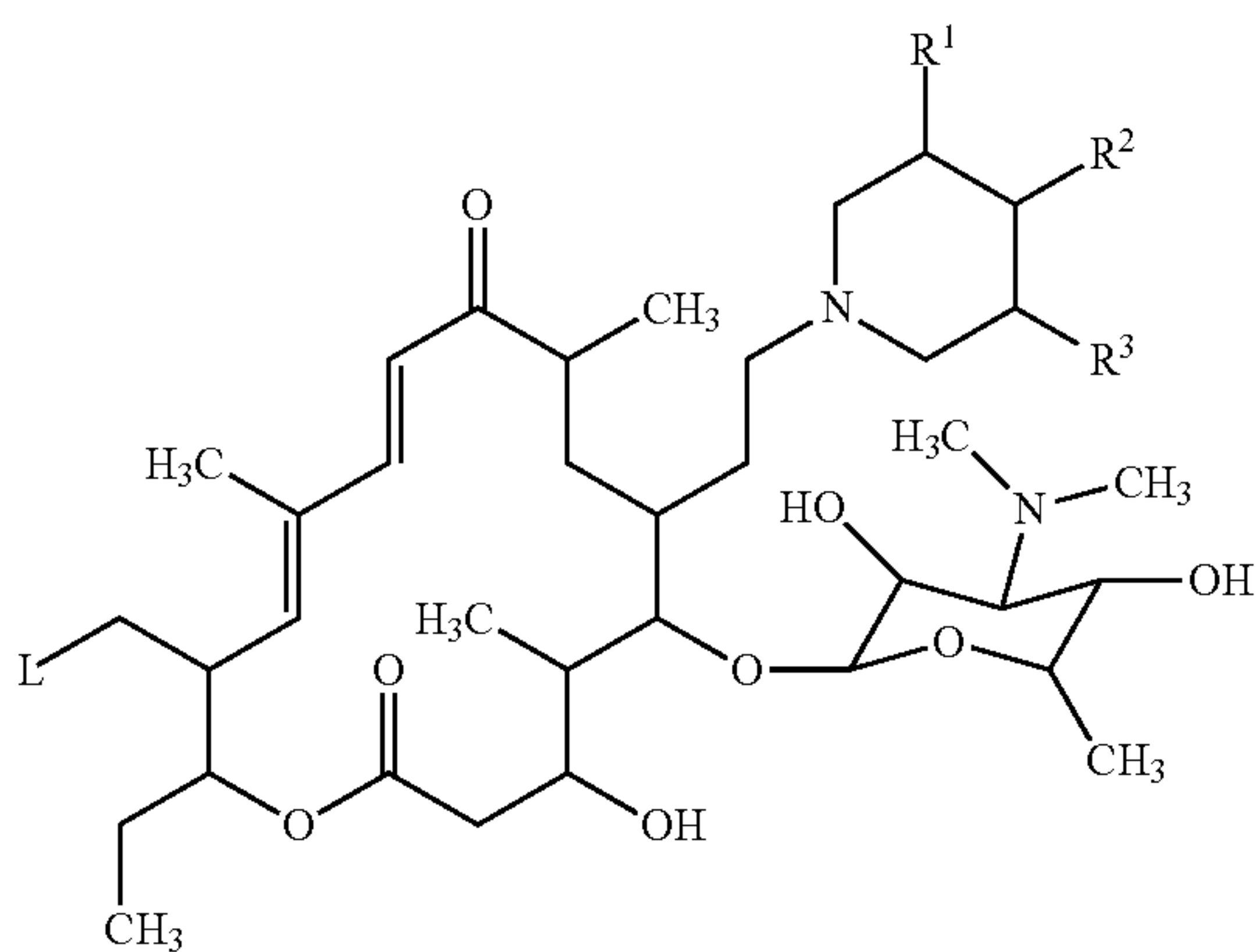
activated compound
