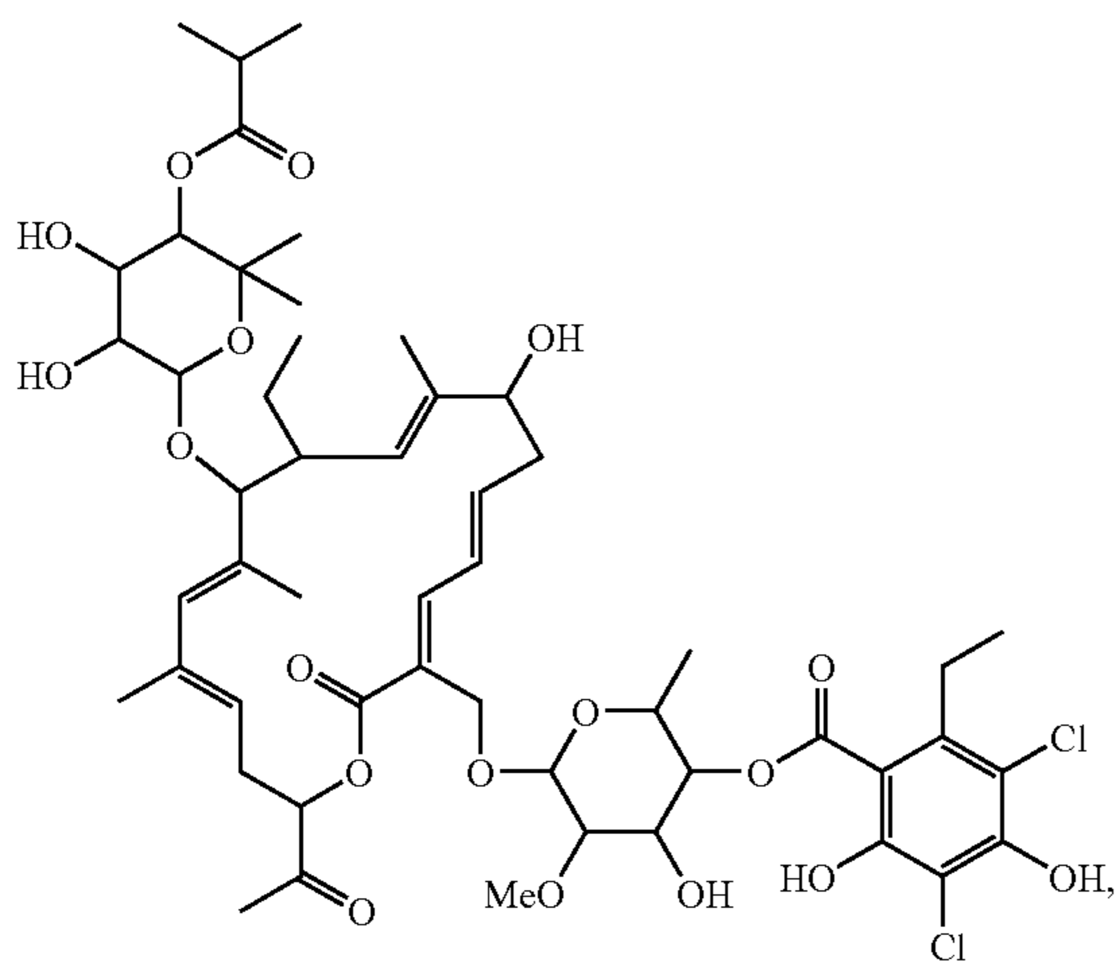
Compound 106
