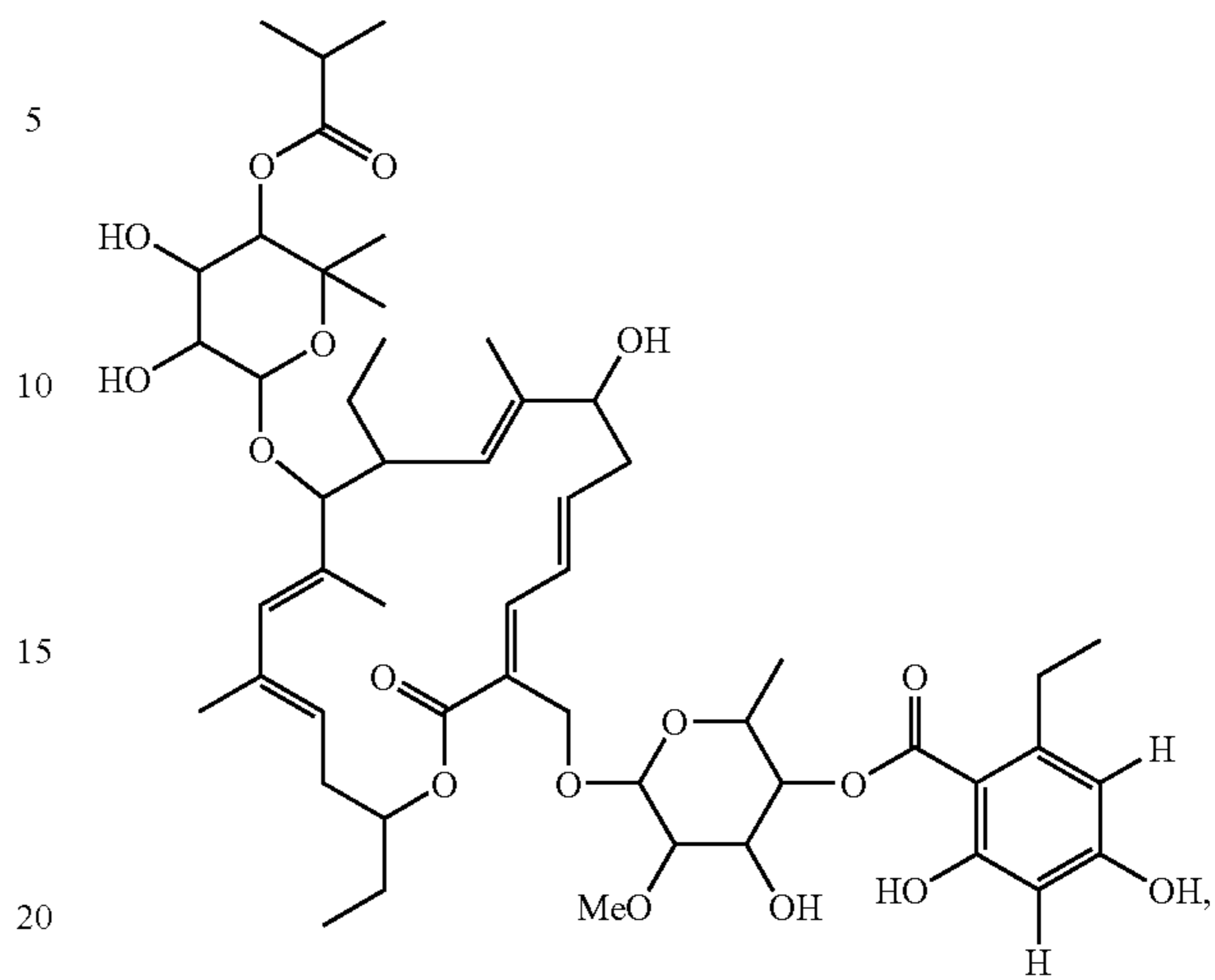
Compound 108
