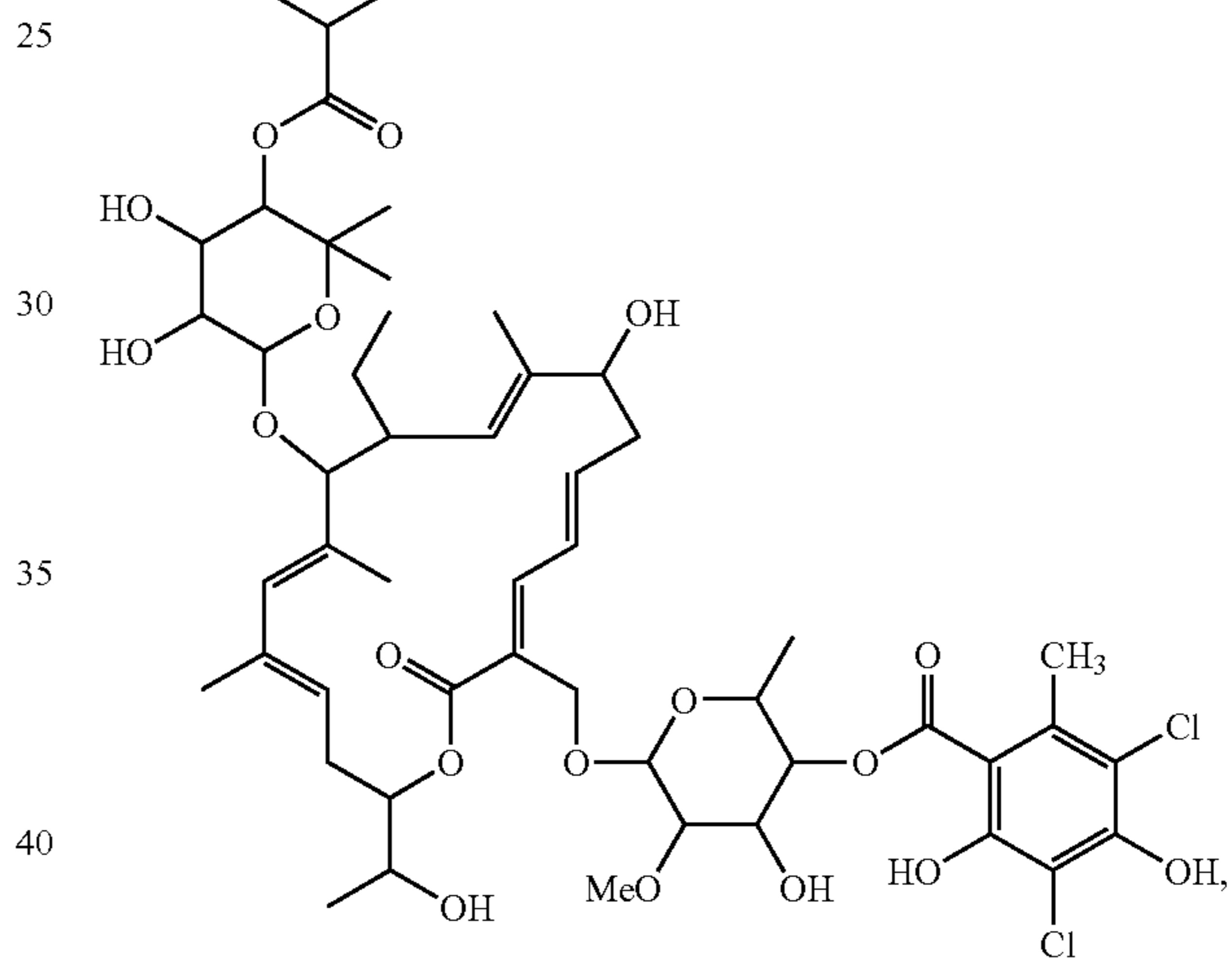
Compound 109
