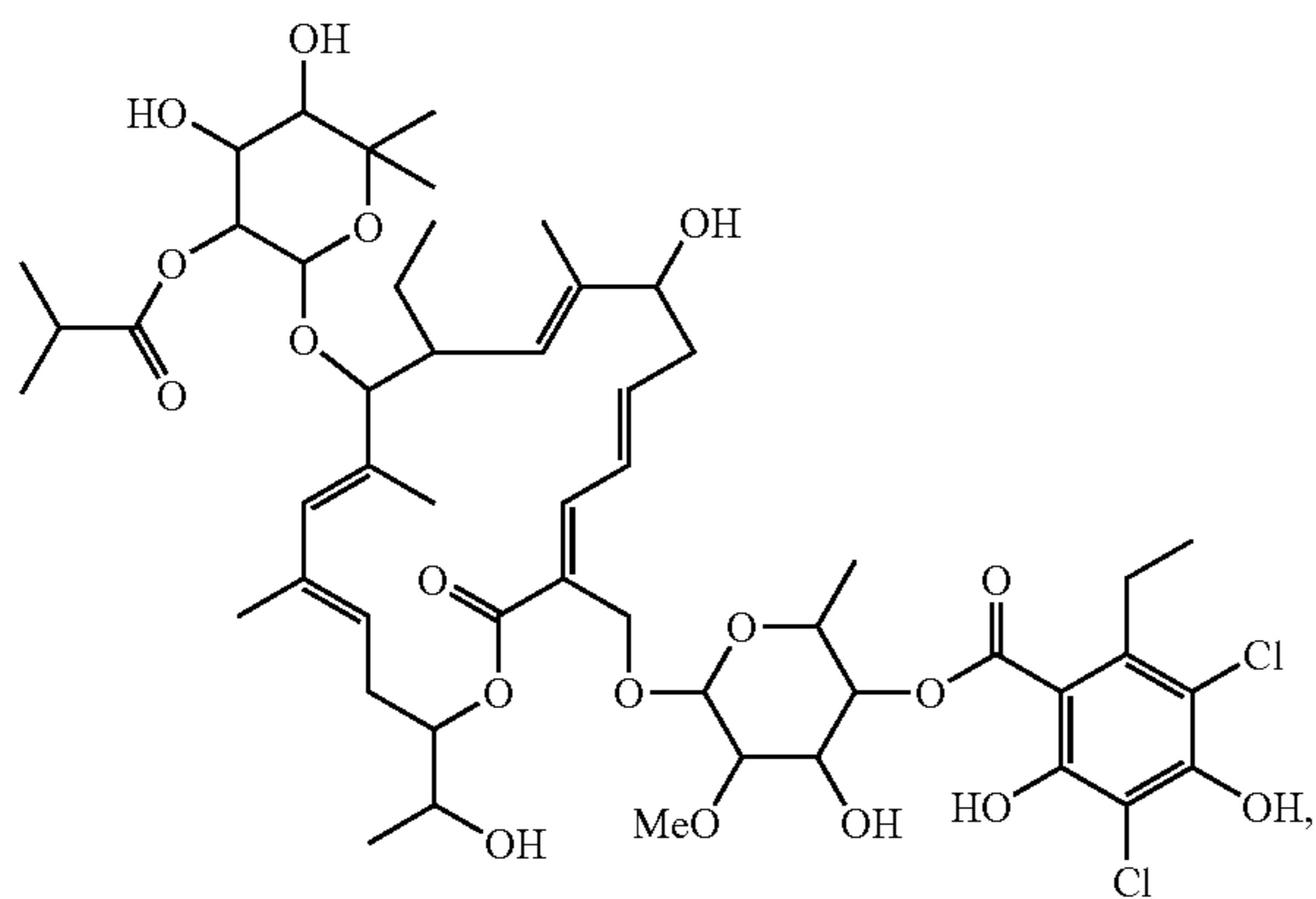
Compound 112
