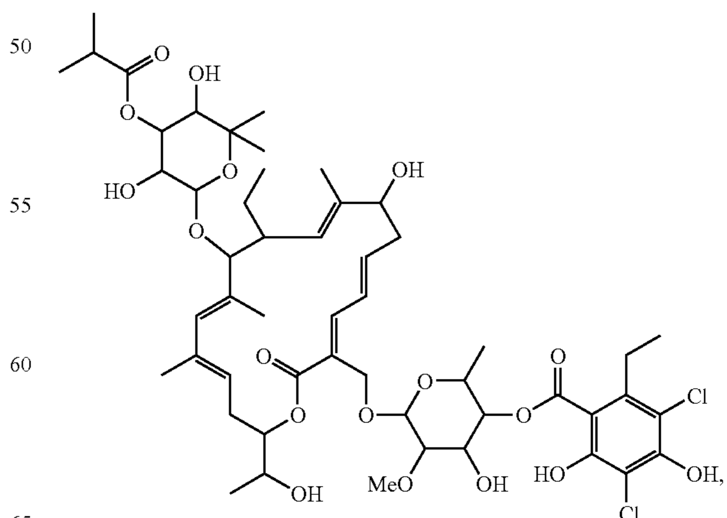
Compound 110
