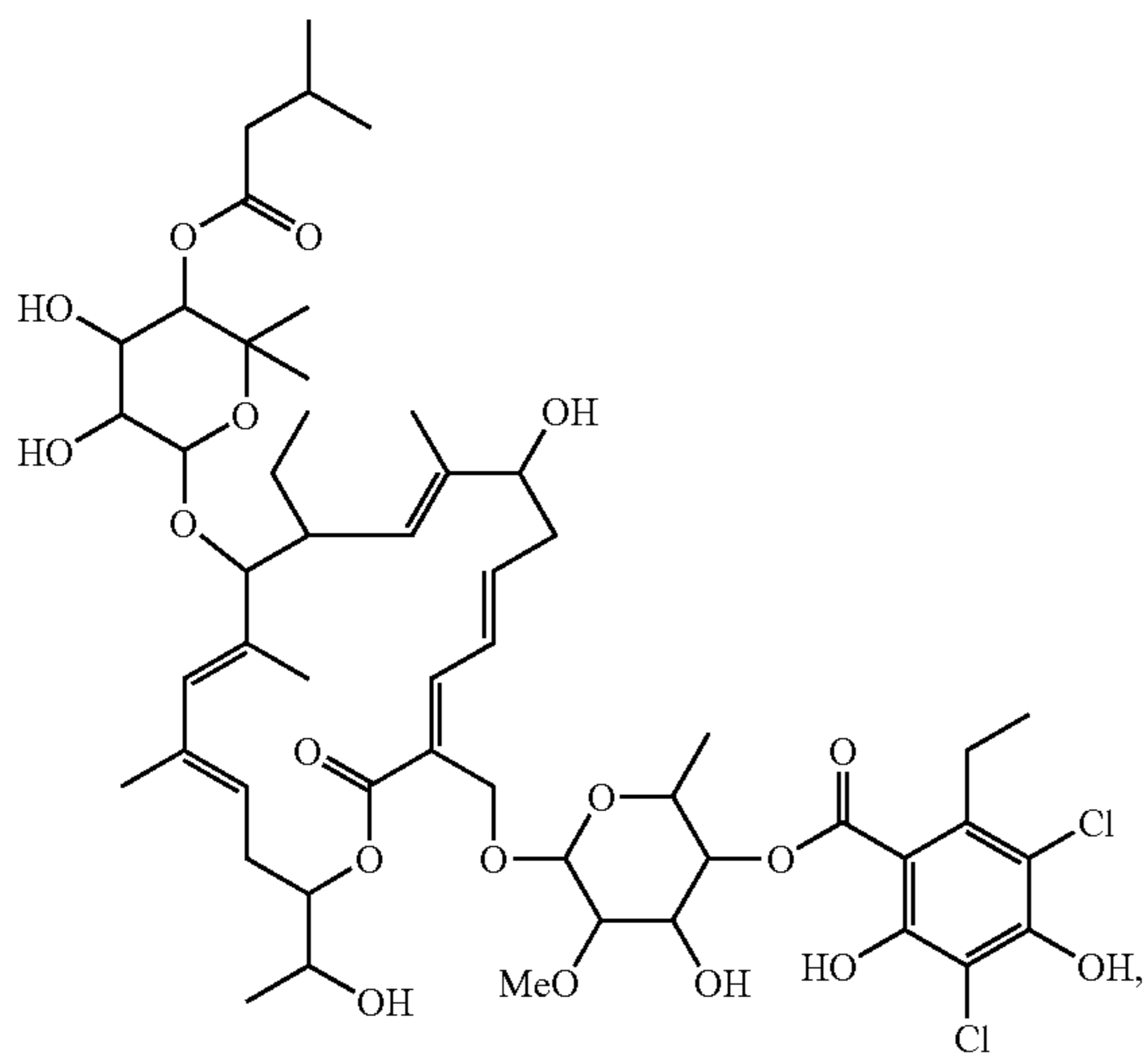
Compound 105
