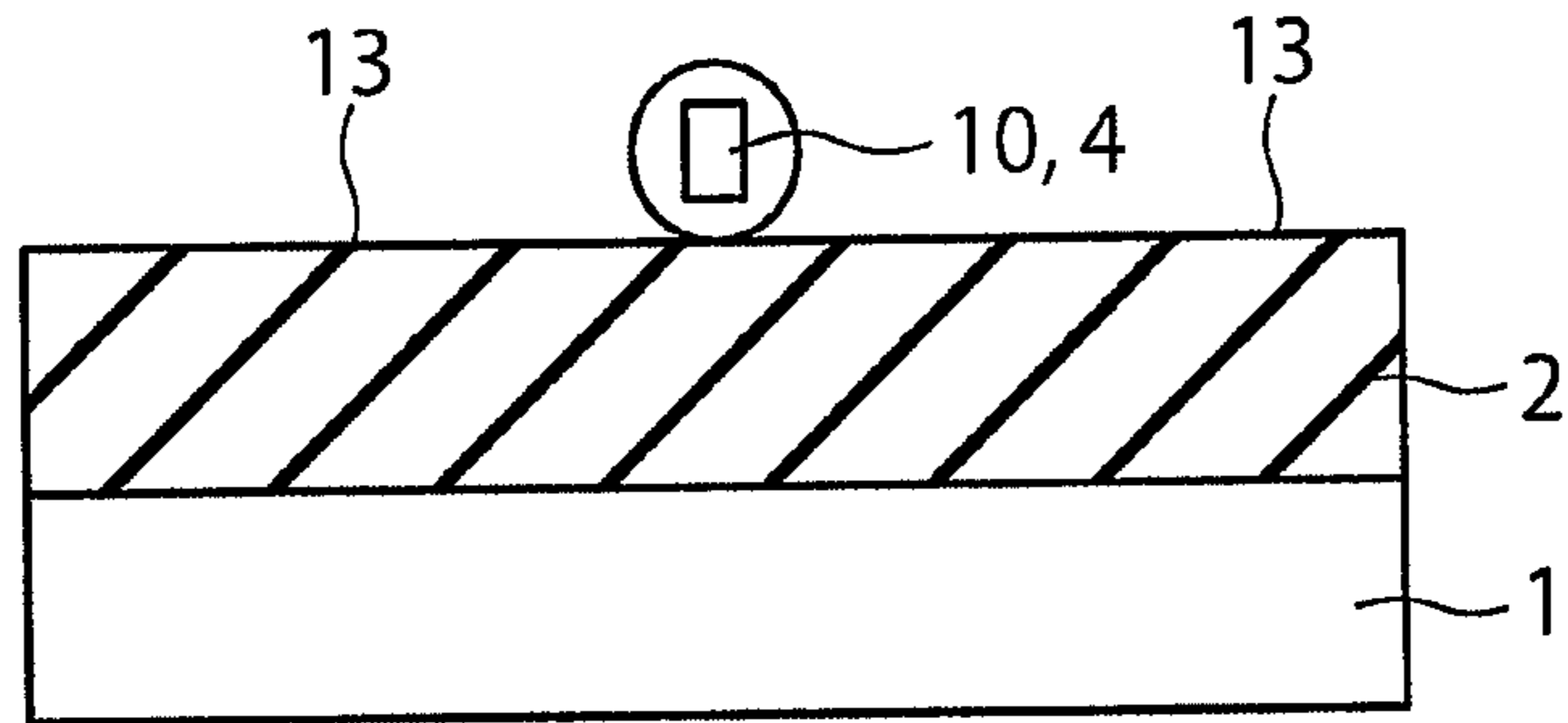
D-D CROSS-SECTION
