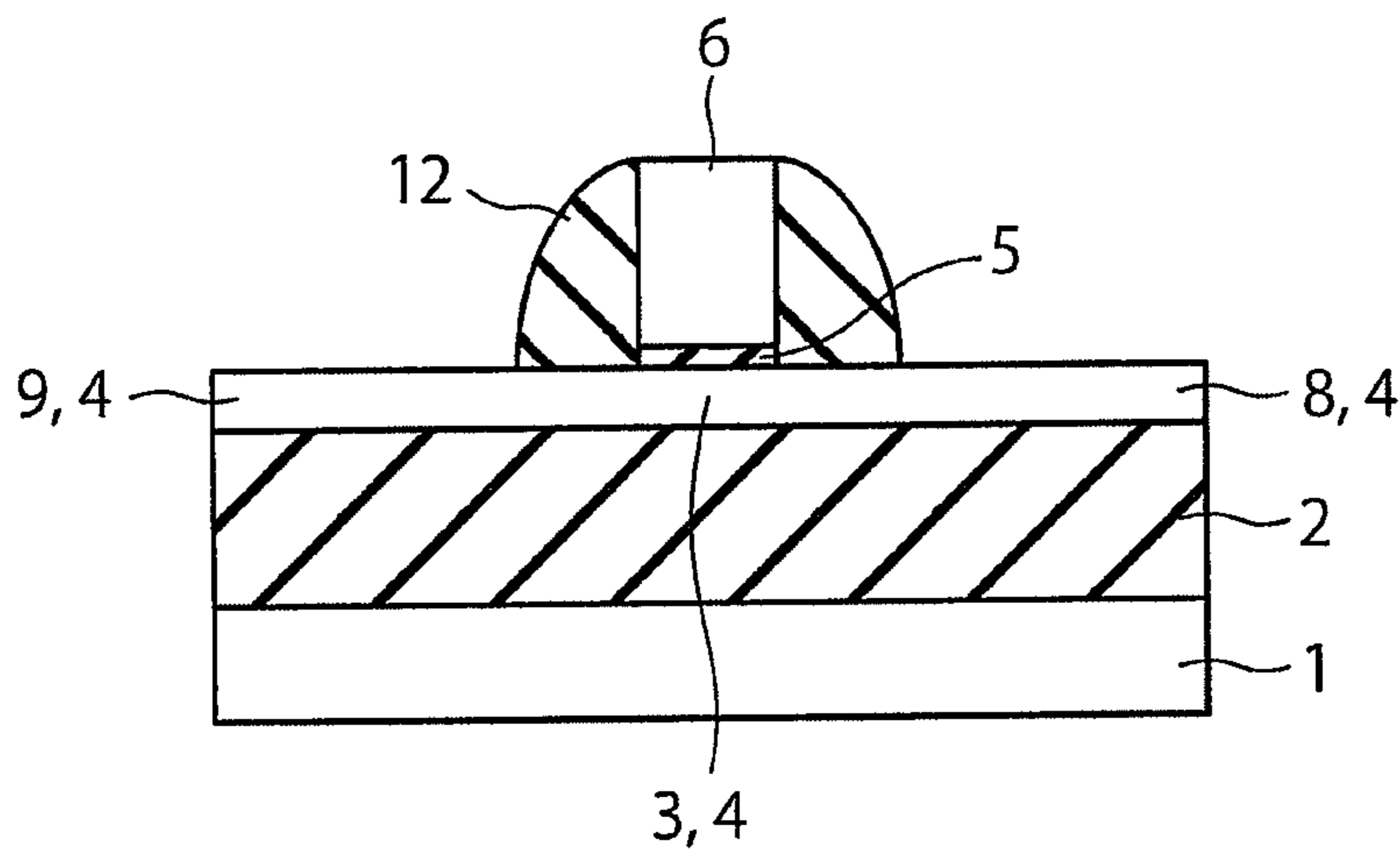
F-F CROSS-SECTION
