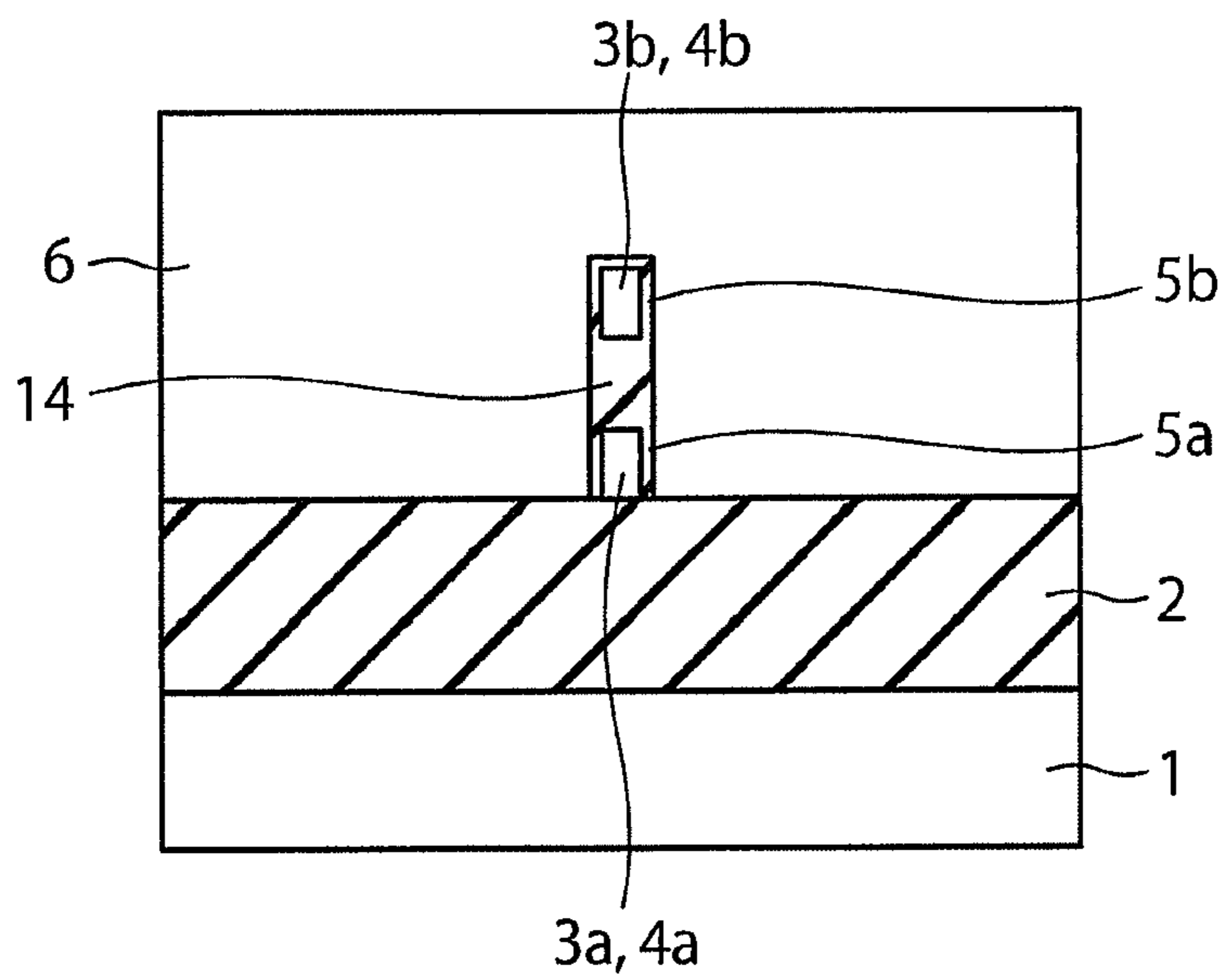
P-P CROSS-SECTION
