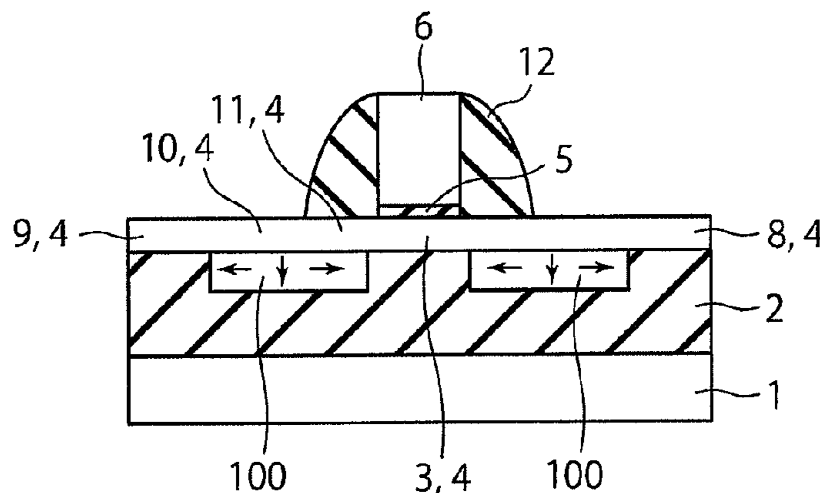
J-J CROSS-SECTION
