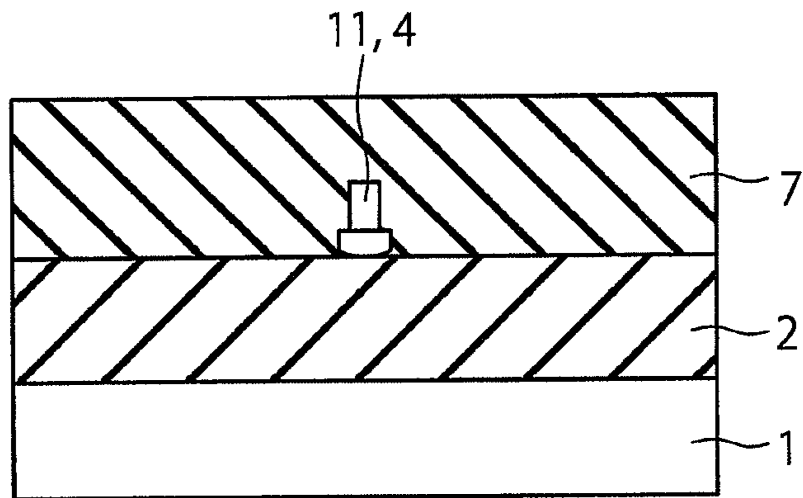
C-C CROSS-SECTION
