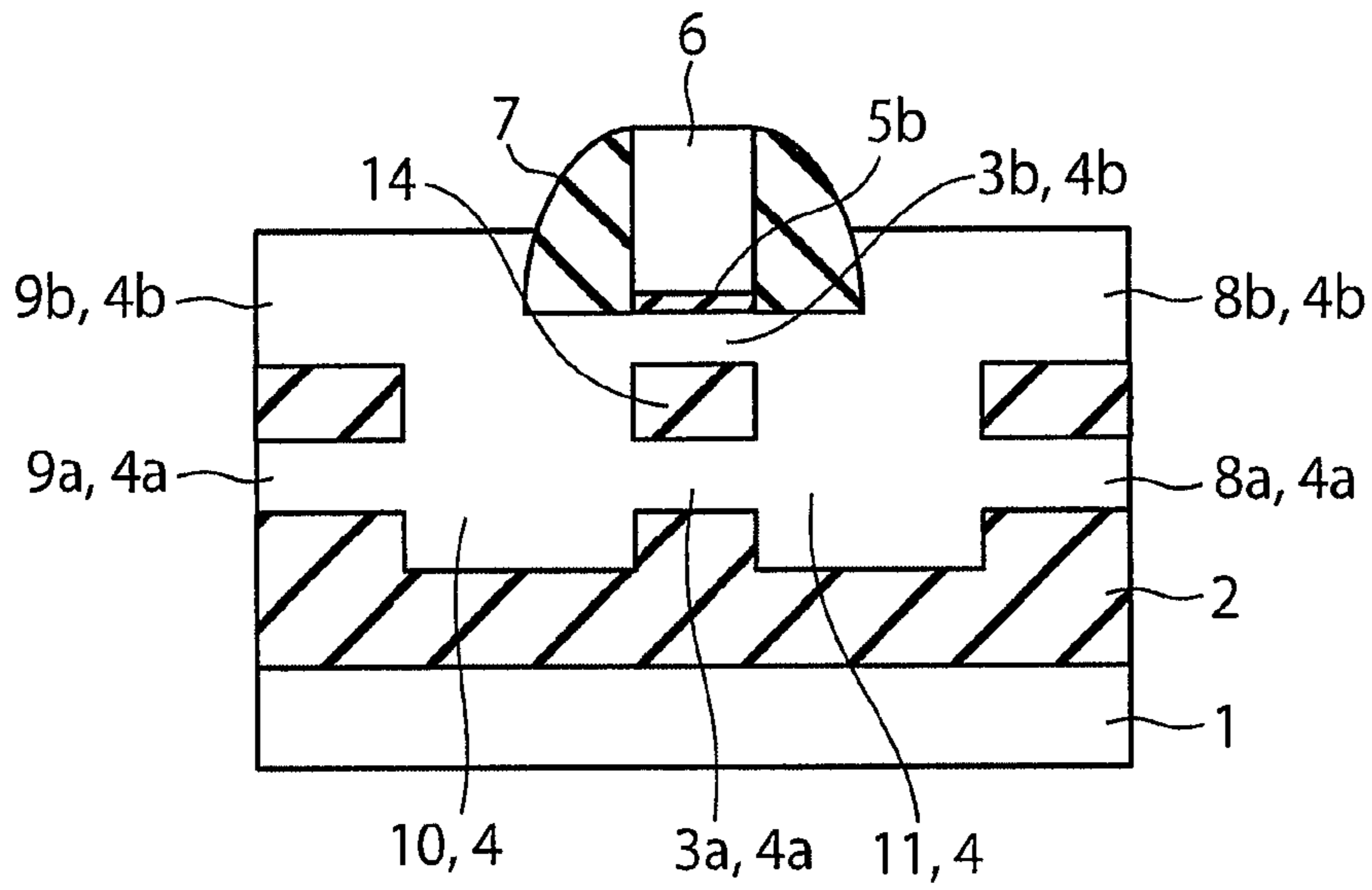
O-O CROSS-SECTION
