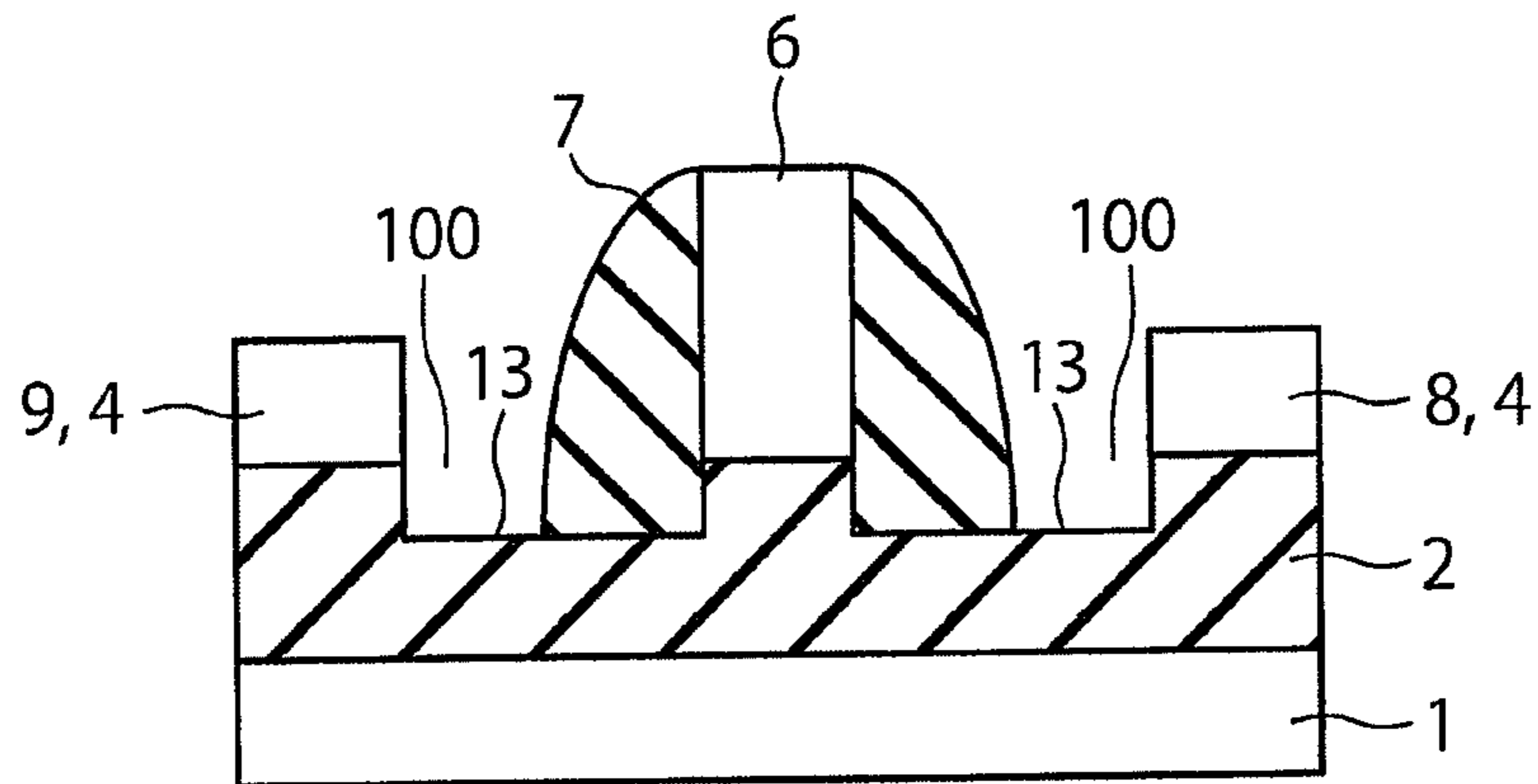
E-E CROSS-SECTION
