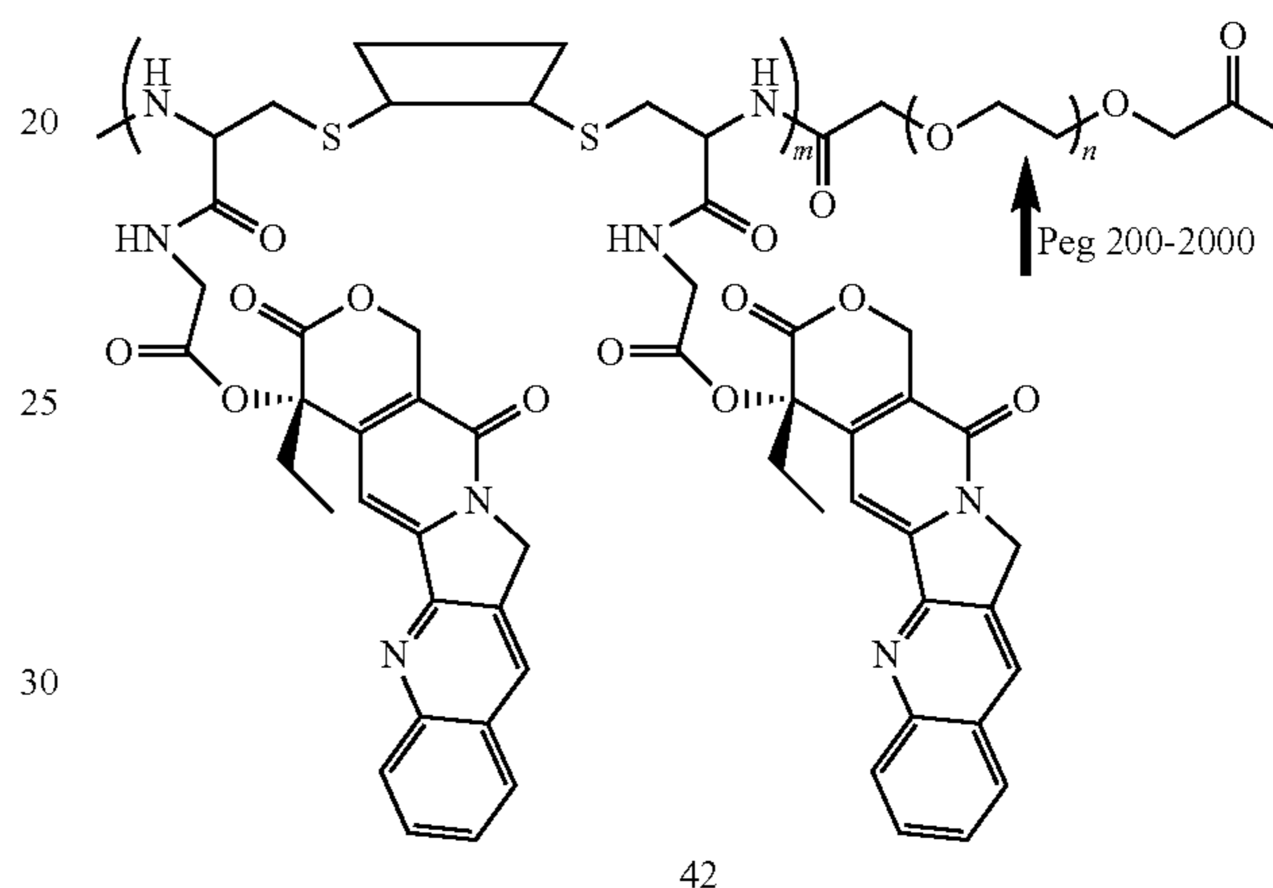
Scheme XXXXII
