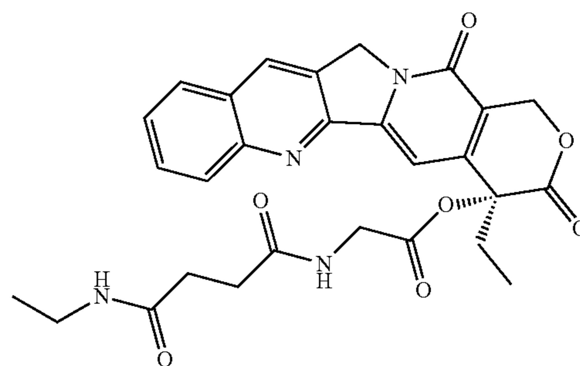
Example 44
