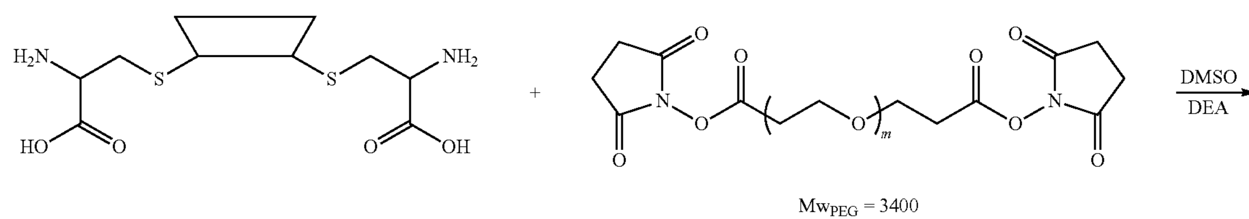
Scheme XIII
