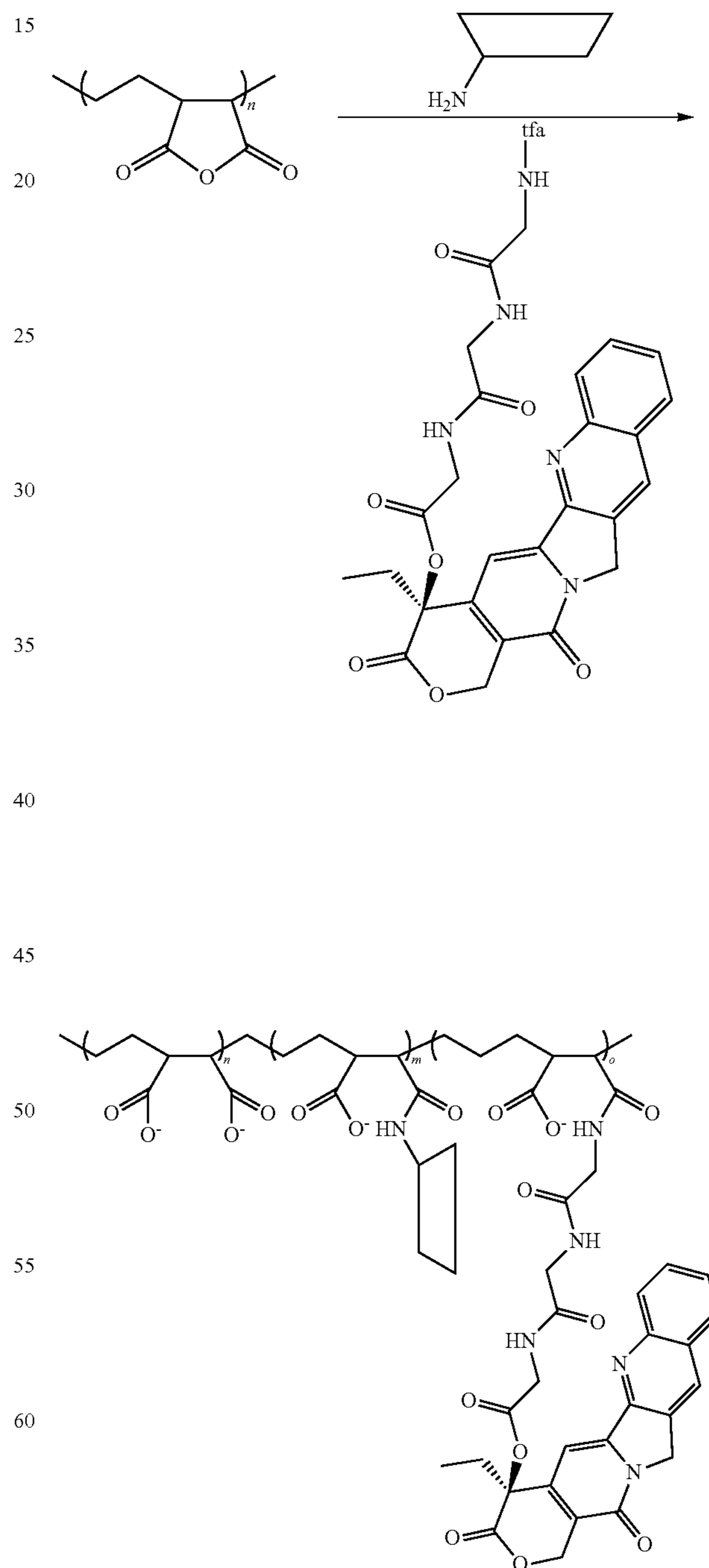
Scheme XXXVI
