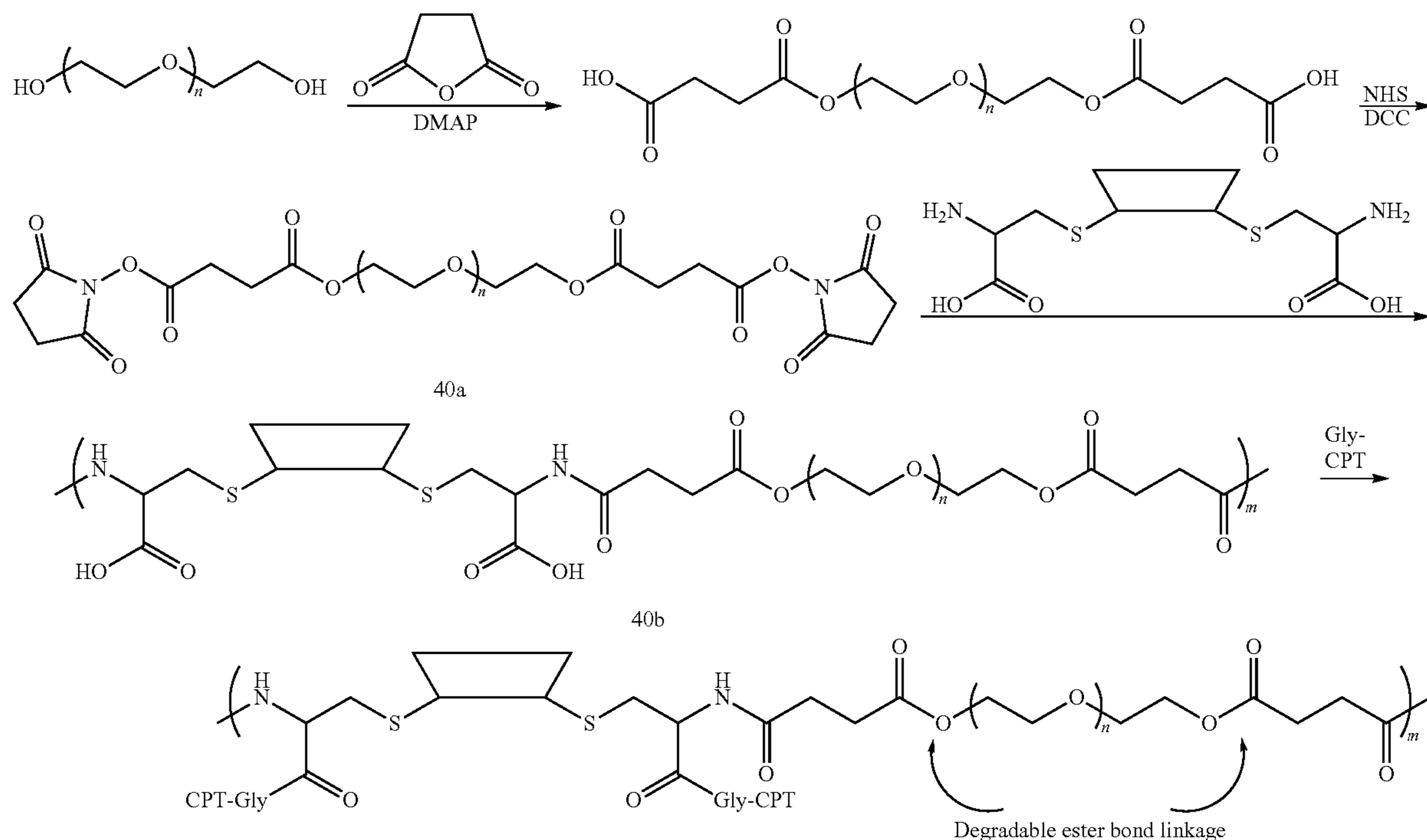
Scheme XXXXI
