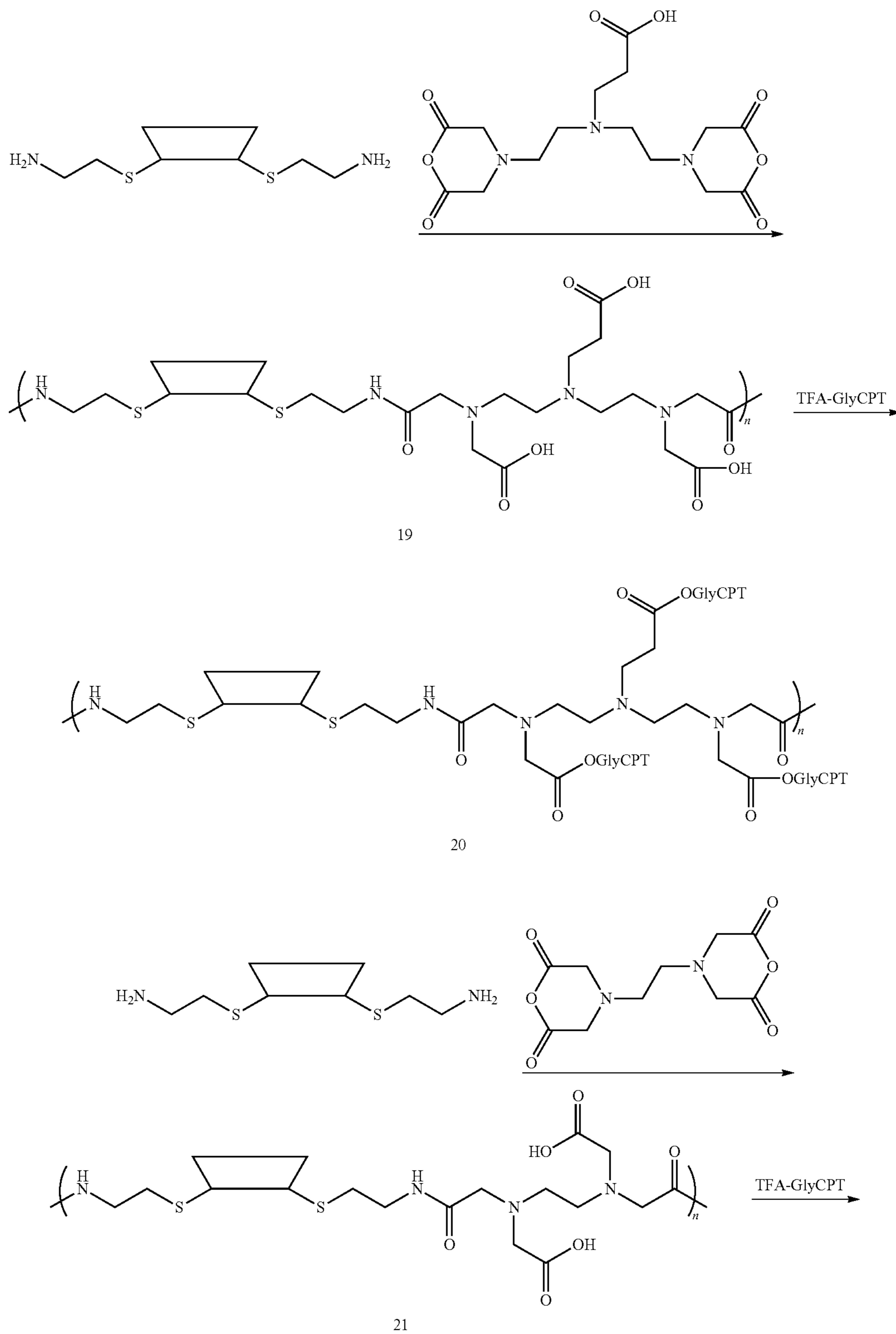
Scheme XXIX
