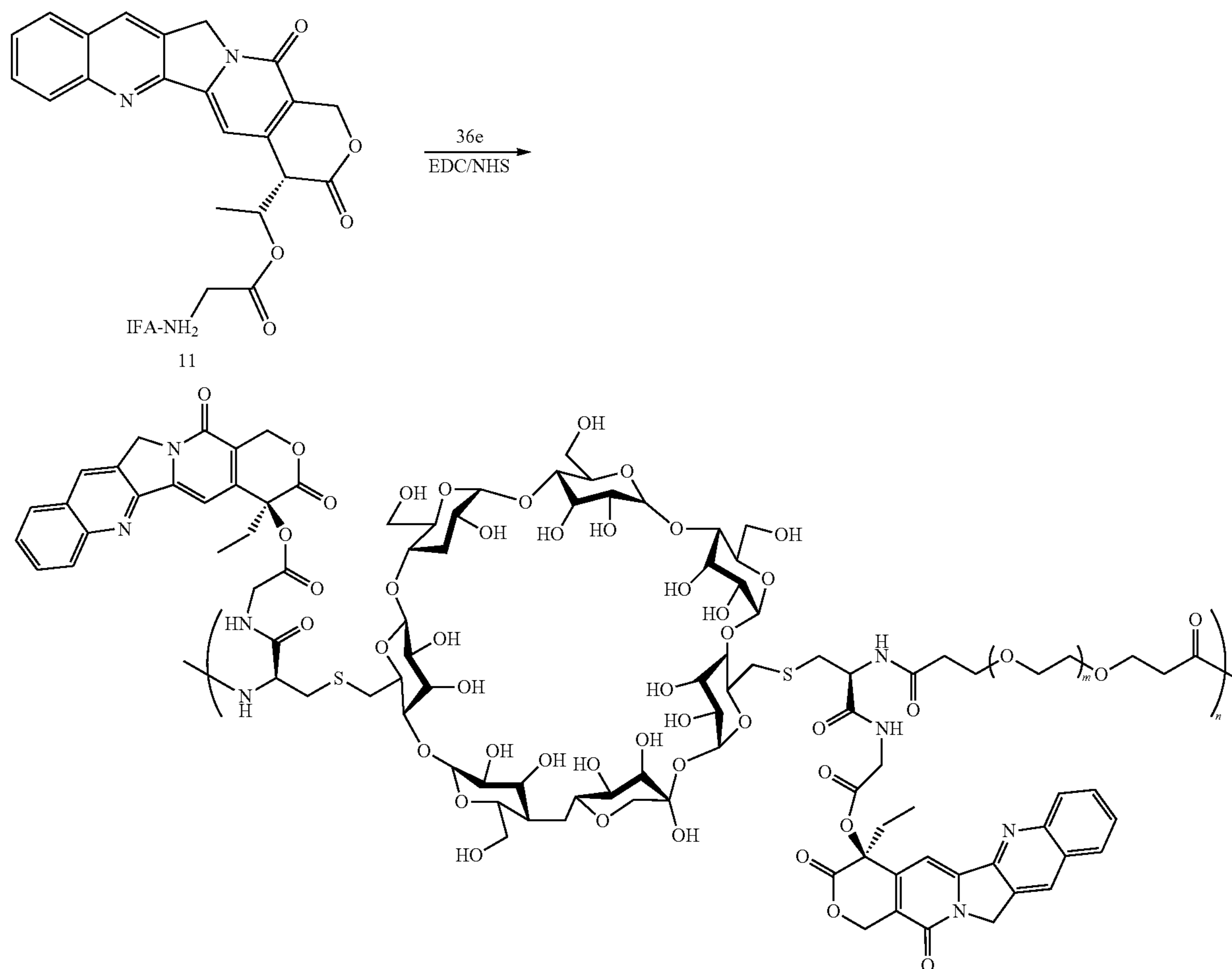
Scheme XXXIX
