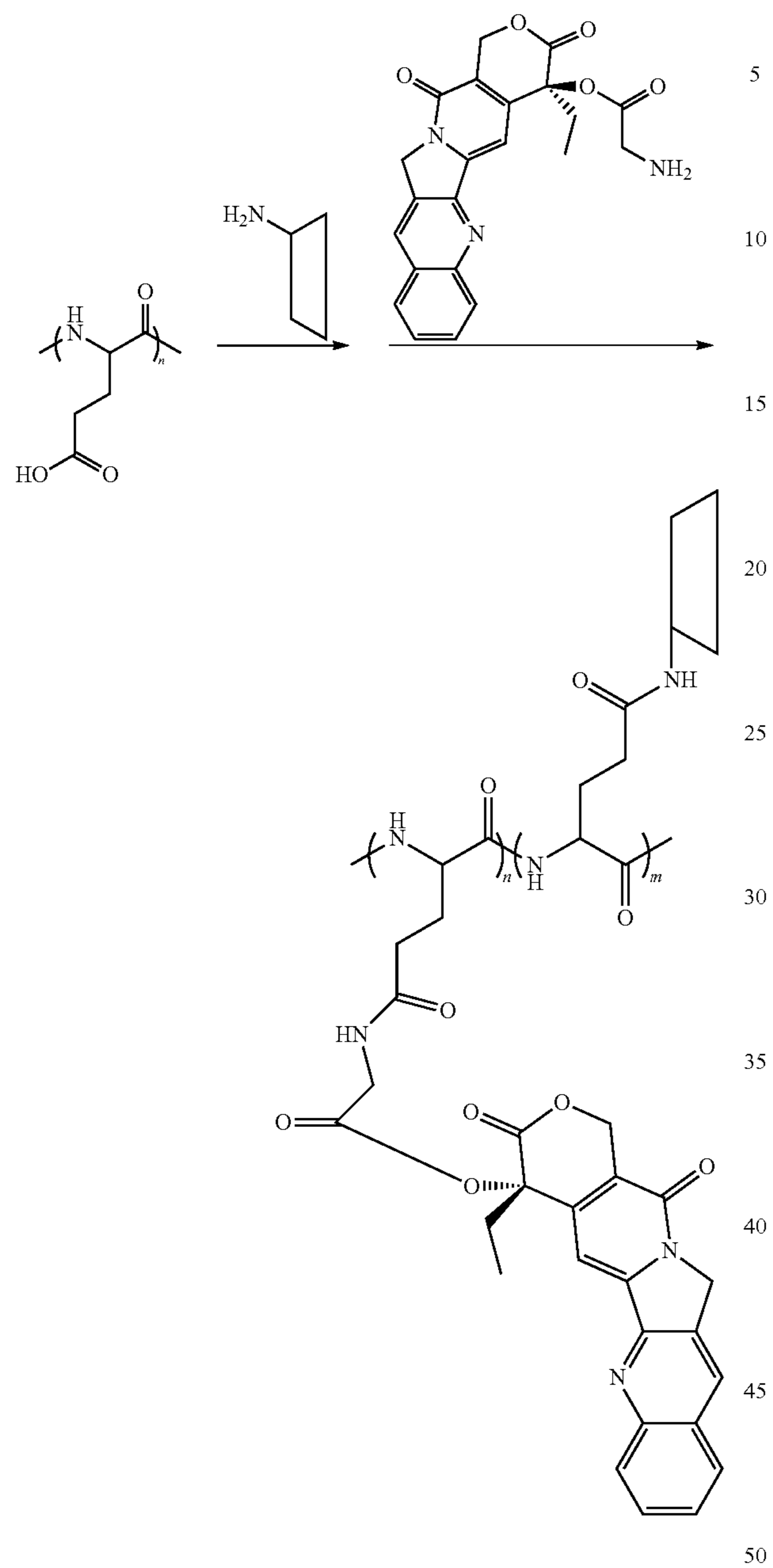
Scheme XII
