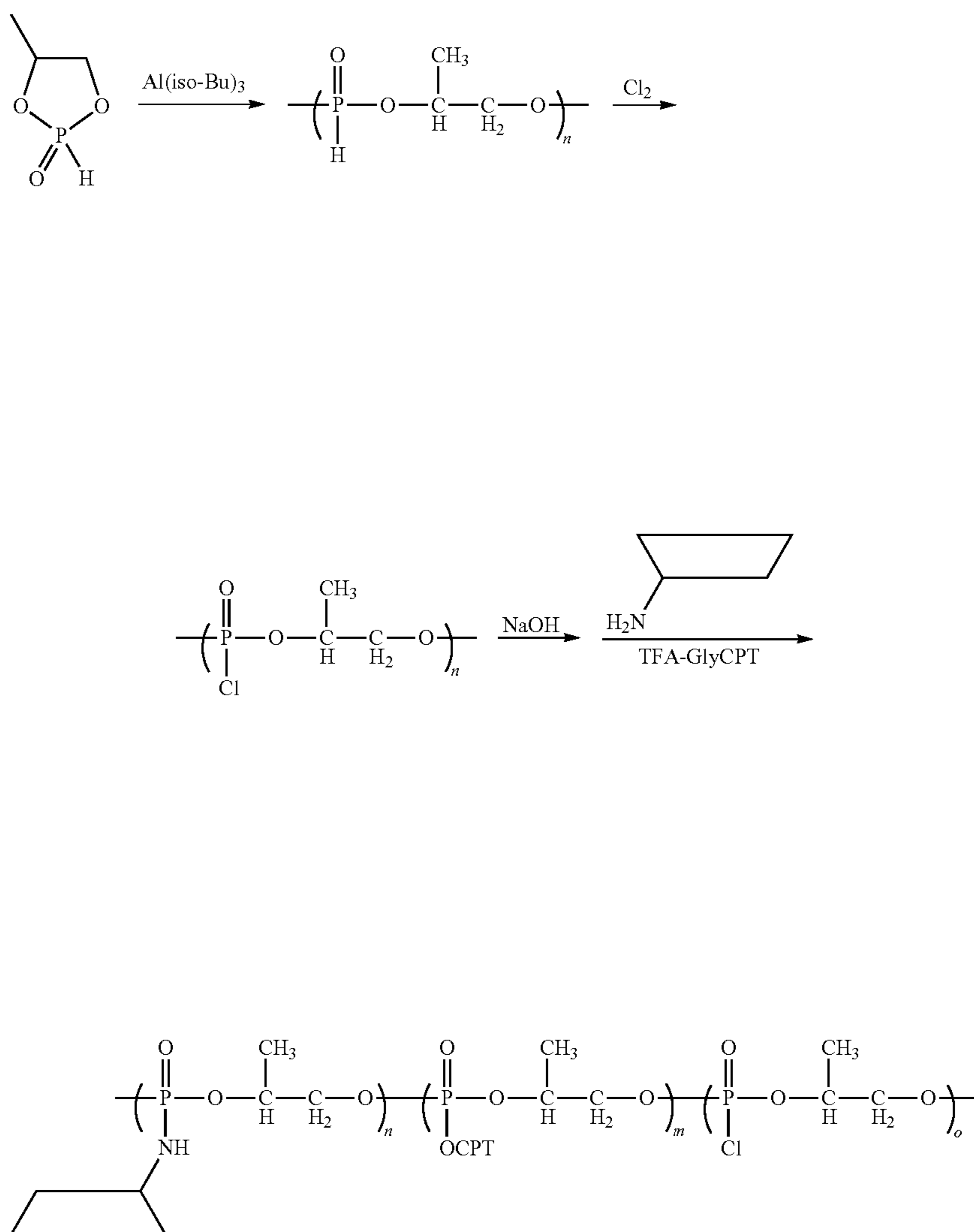
Scheme XXXIV
