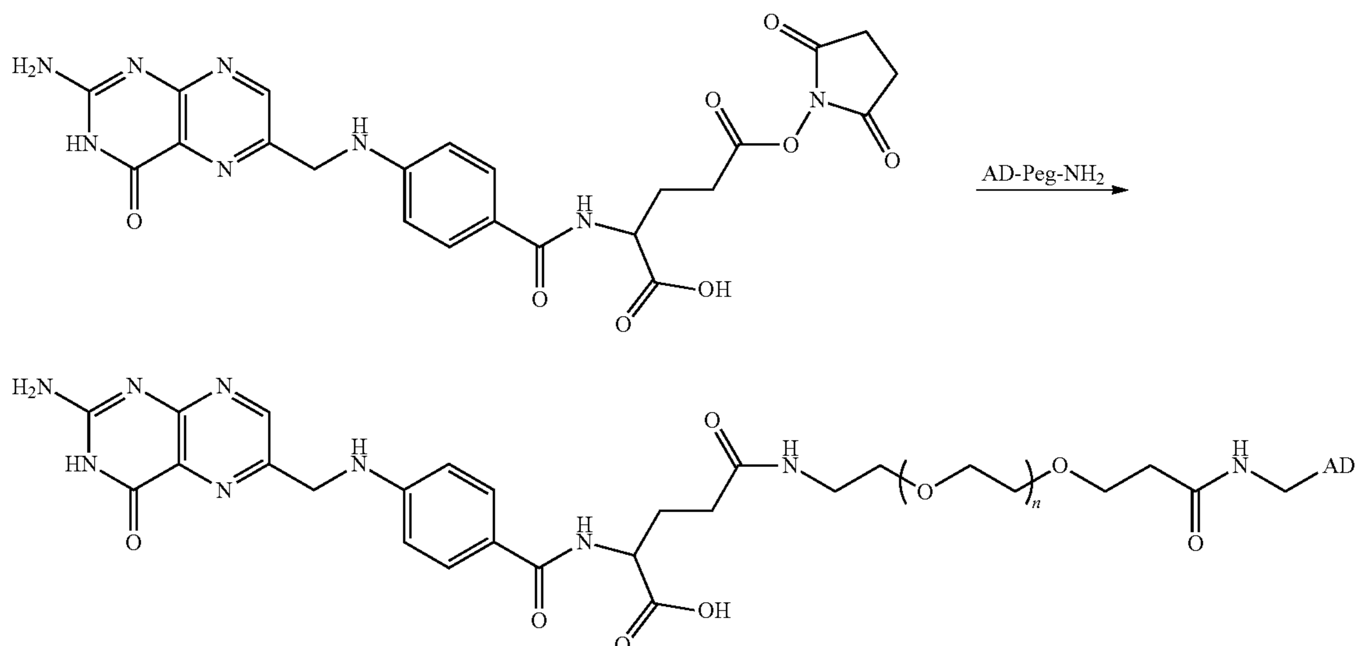
Scheme L
