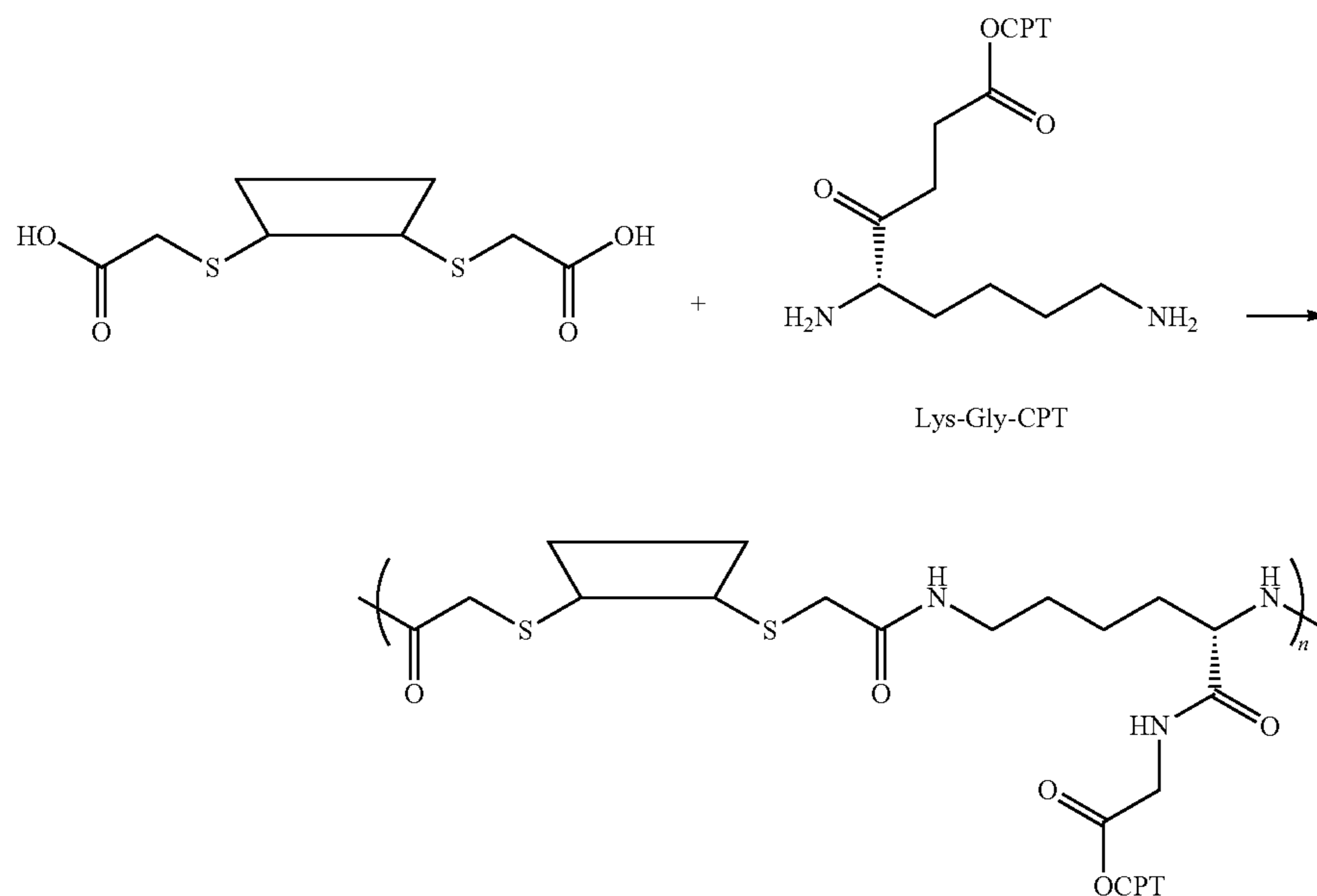
Scheme VIII
