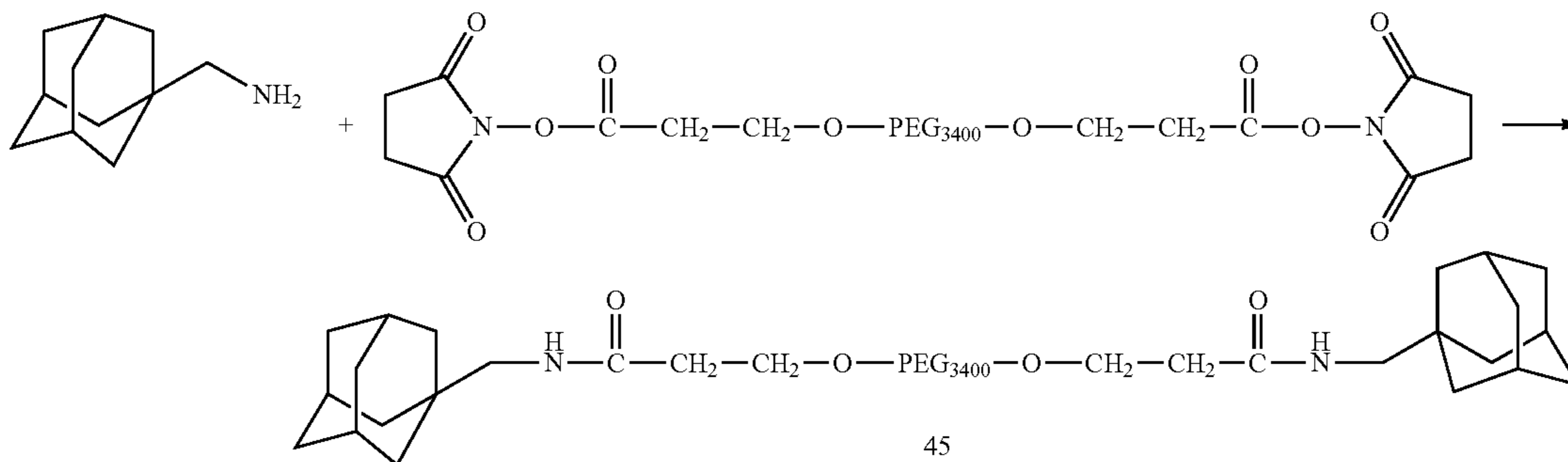
Scheme XXXXVI
