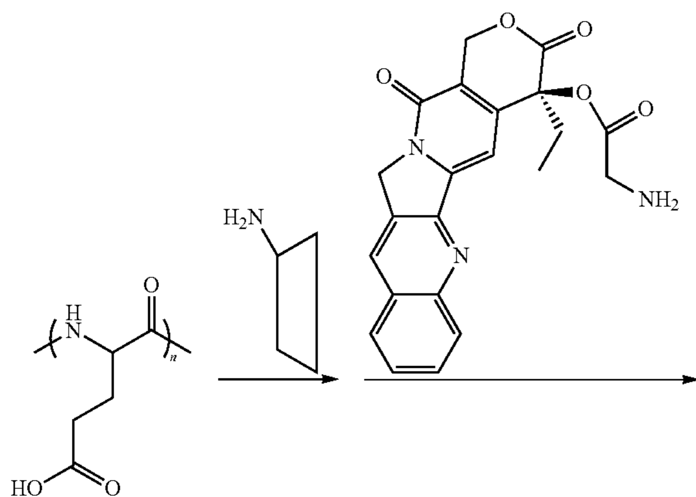
Scheme XXXVII
