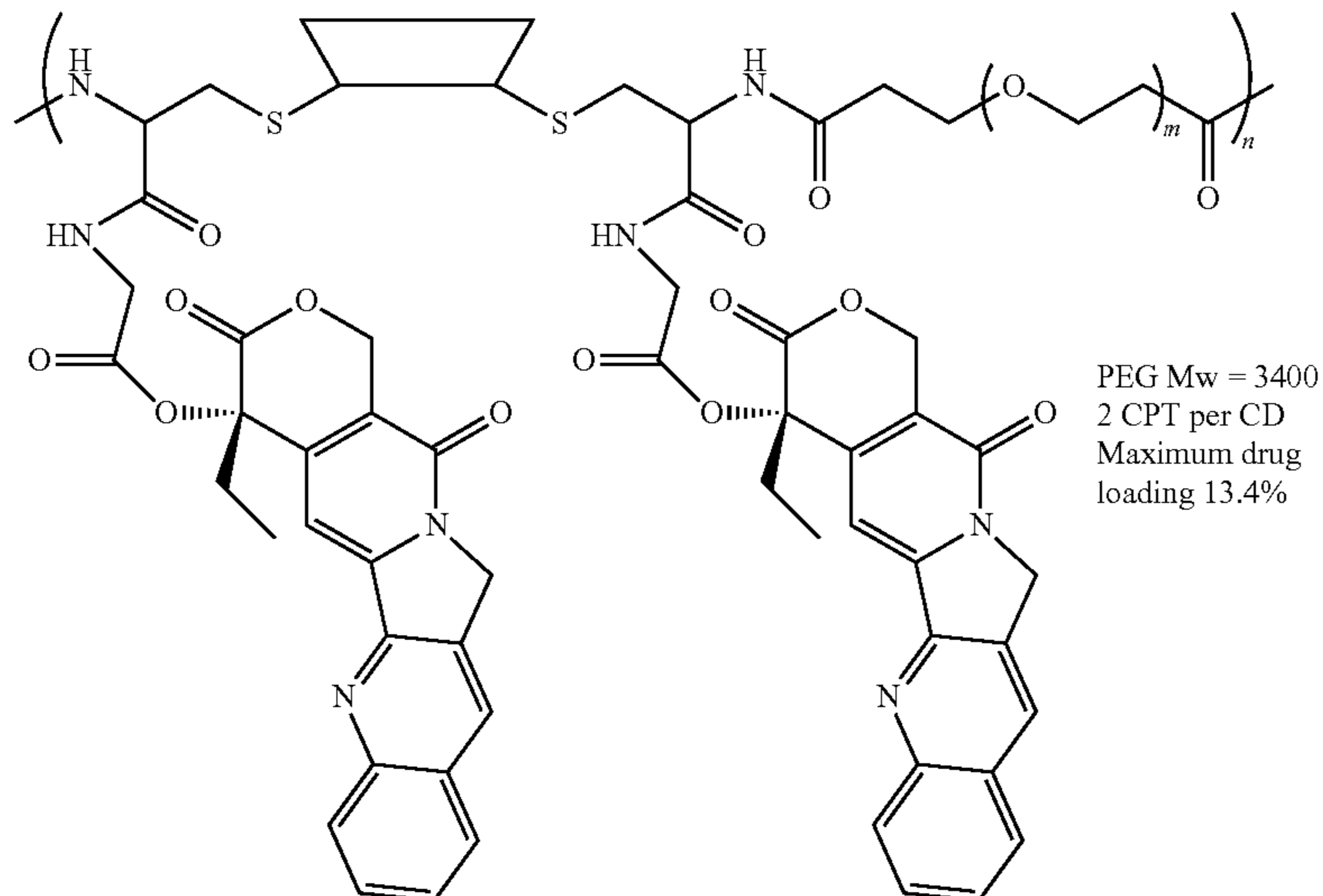
Scheme XXXXIII
