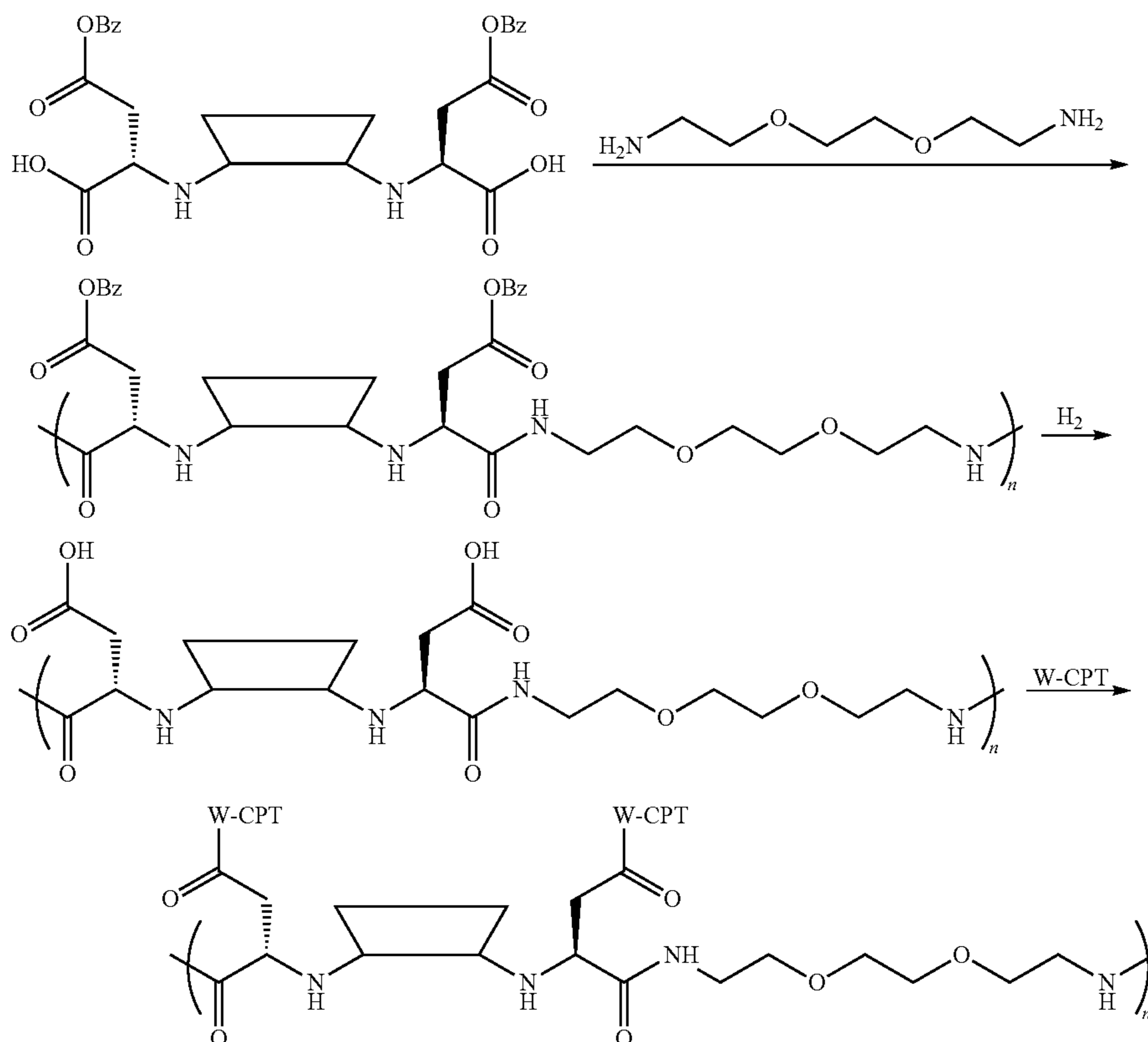
Scheme IV
