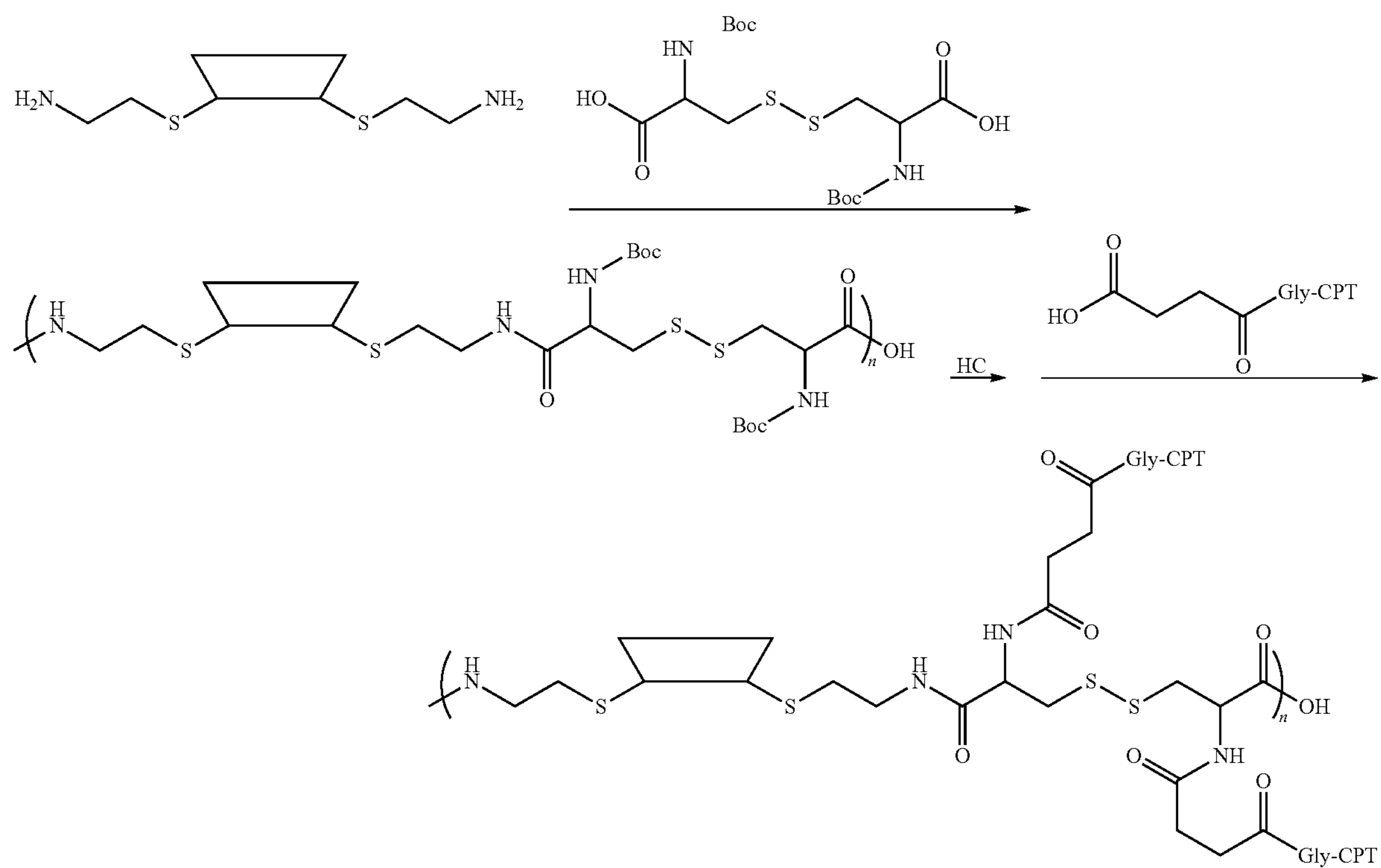
Scheme VII
