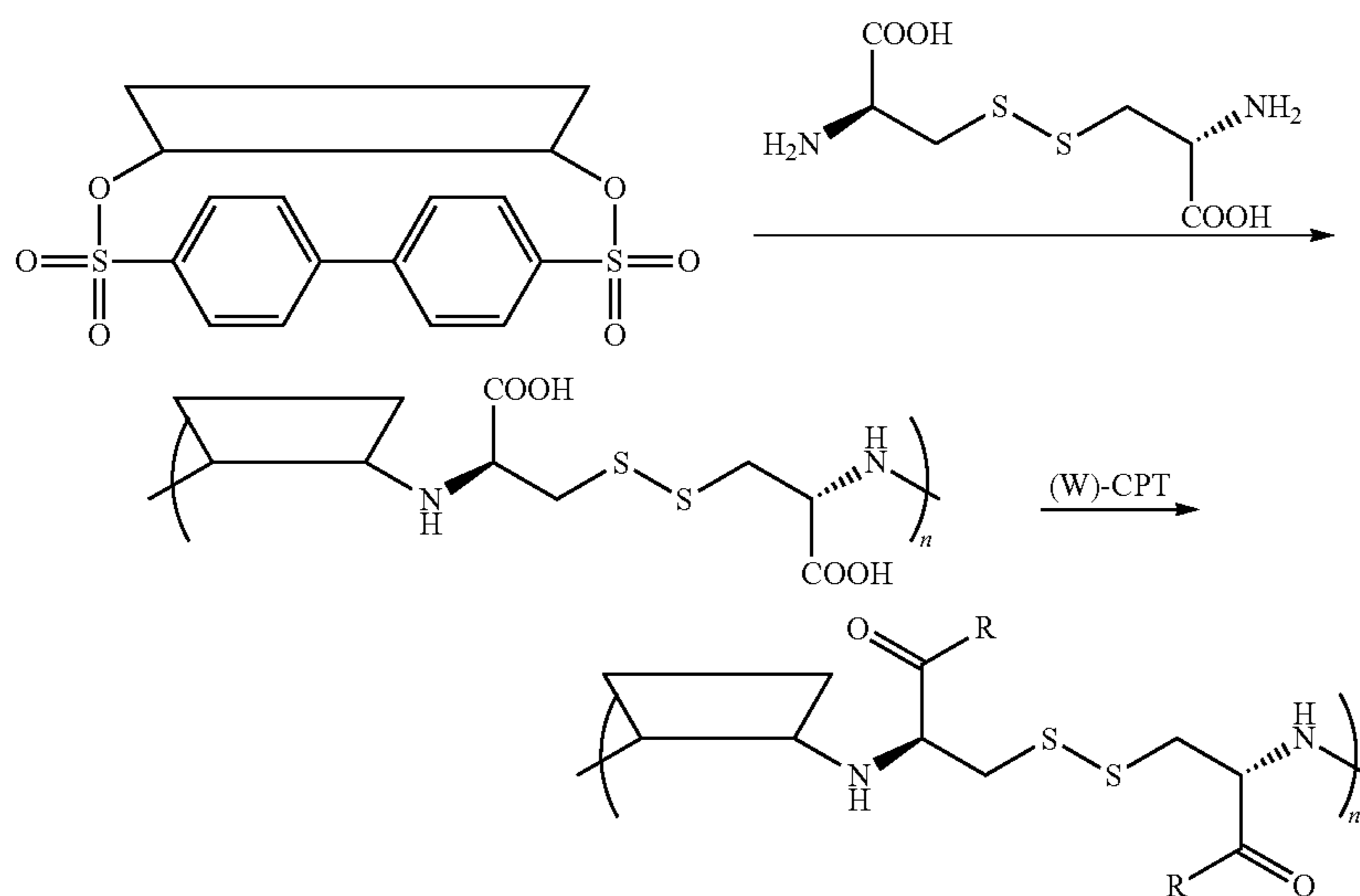
Scheme III
