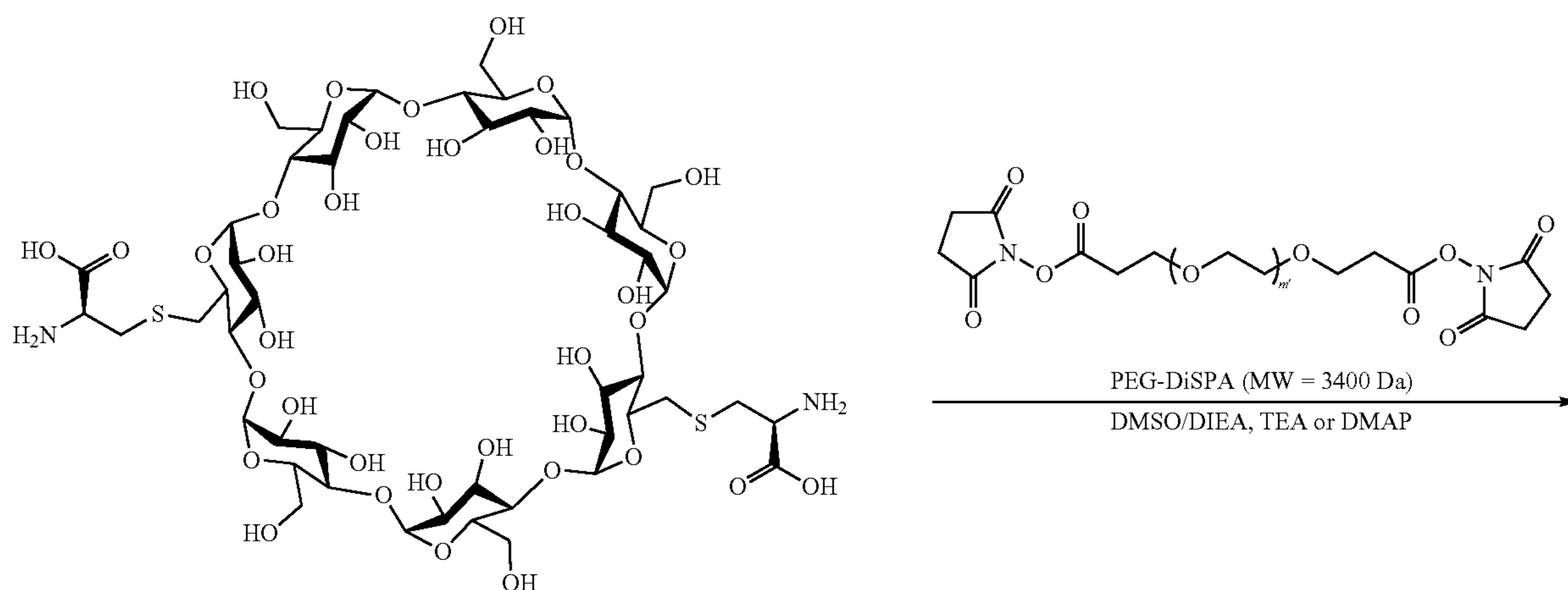
Scheme XXXVIIIa
