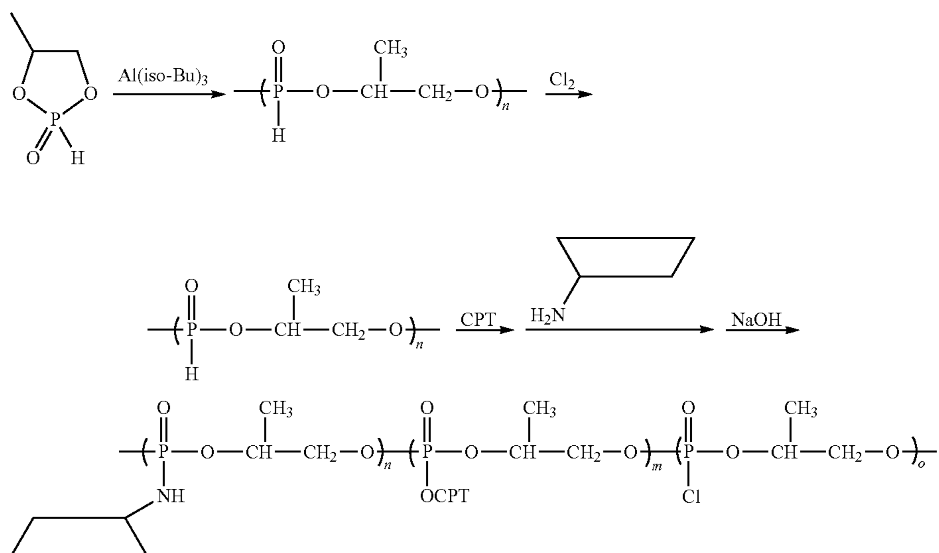
Scheme IX
