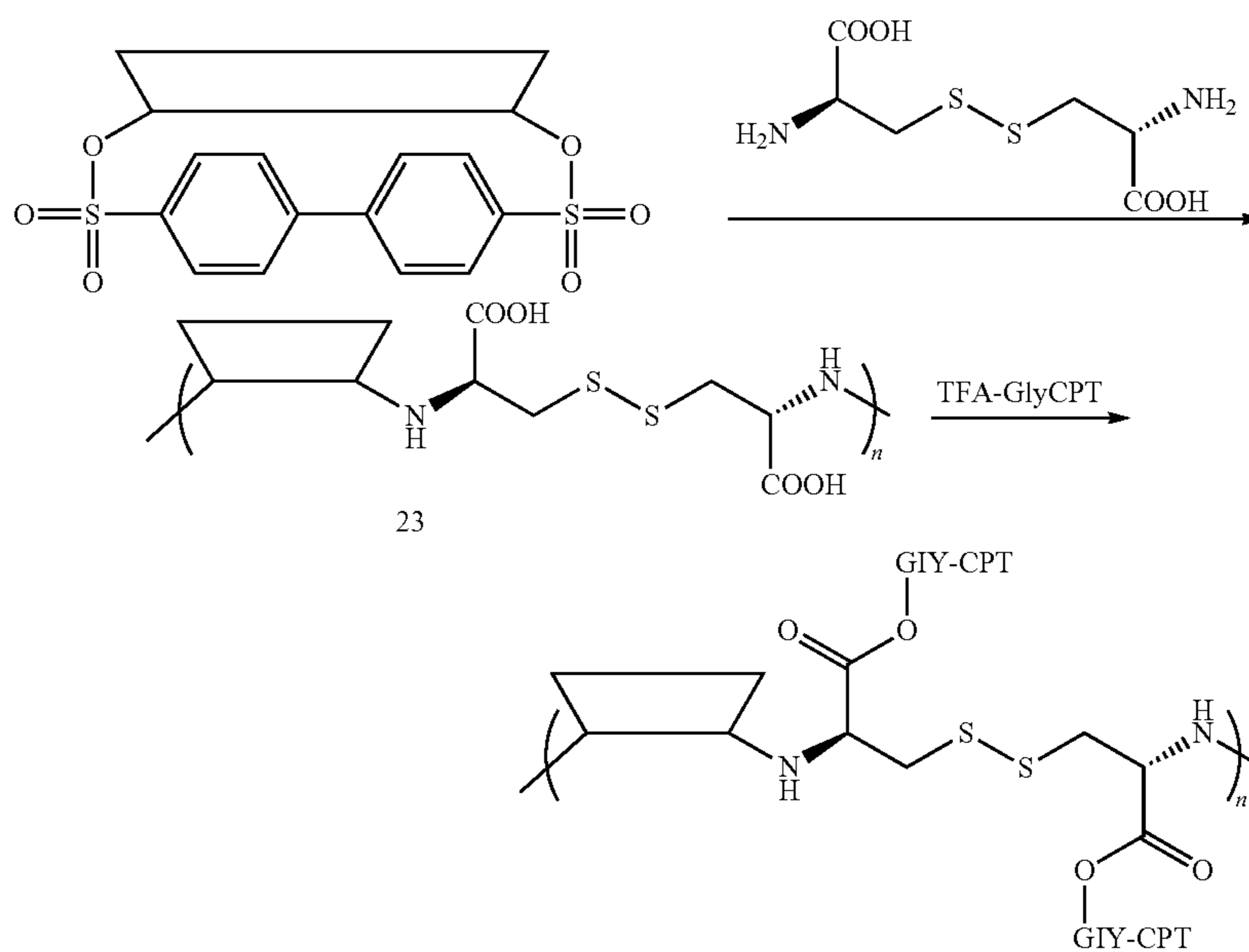
Scheme XXX
