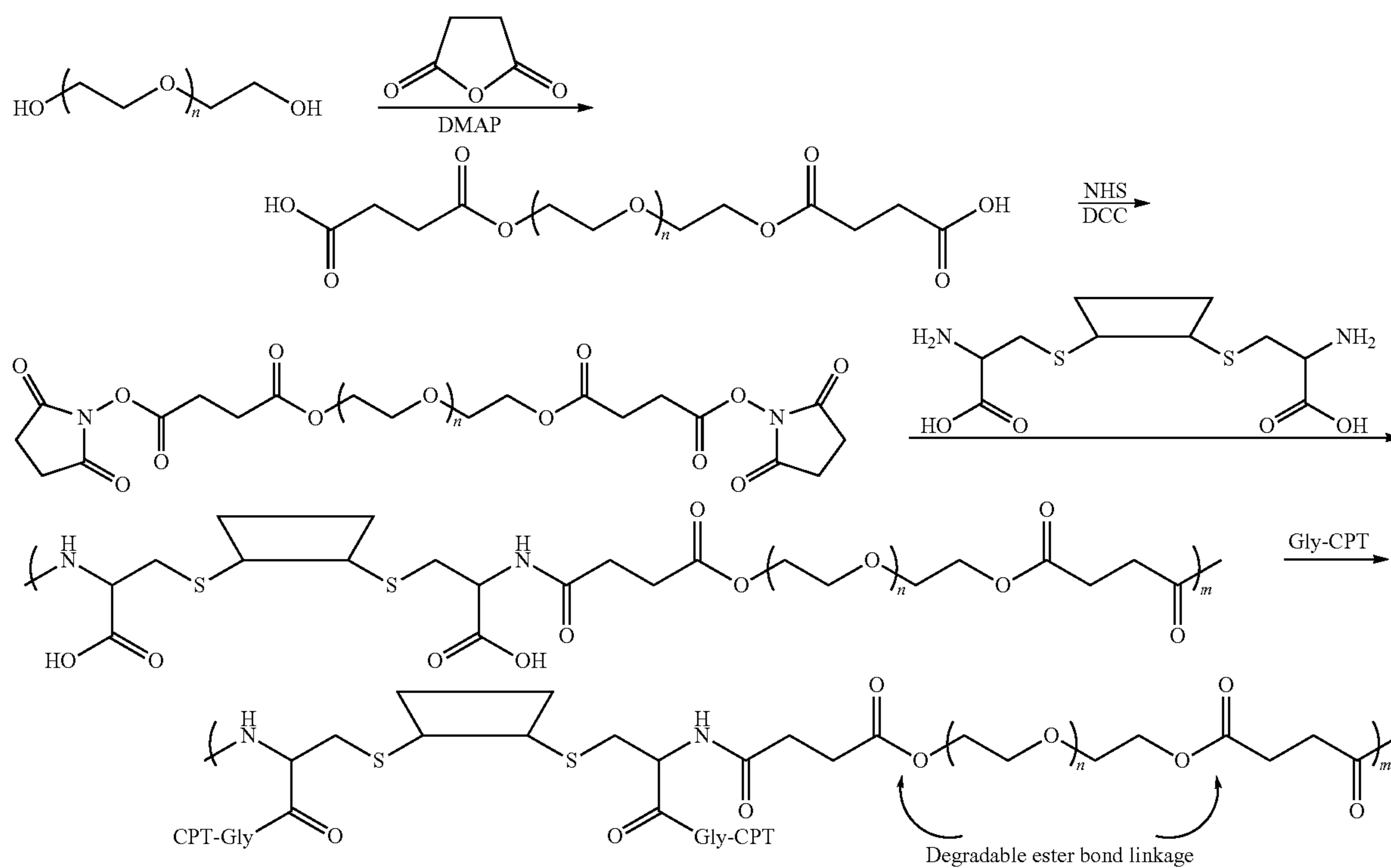
Scheme XIV
