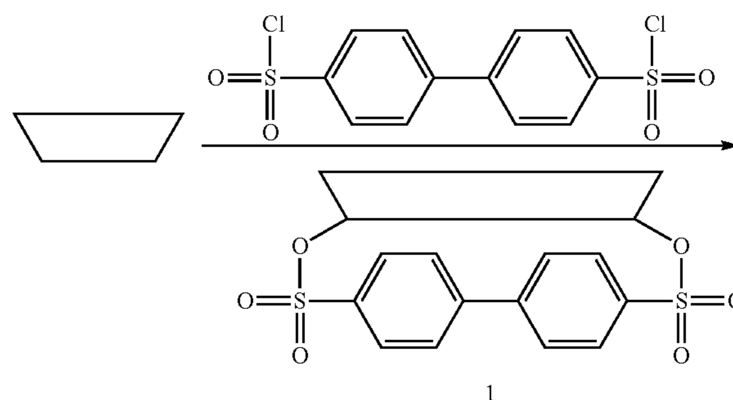
Scheme XV
