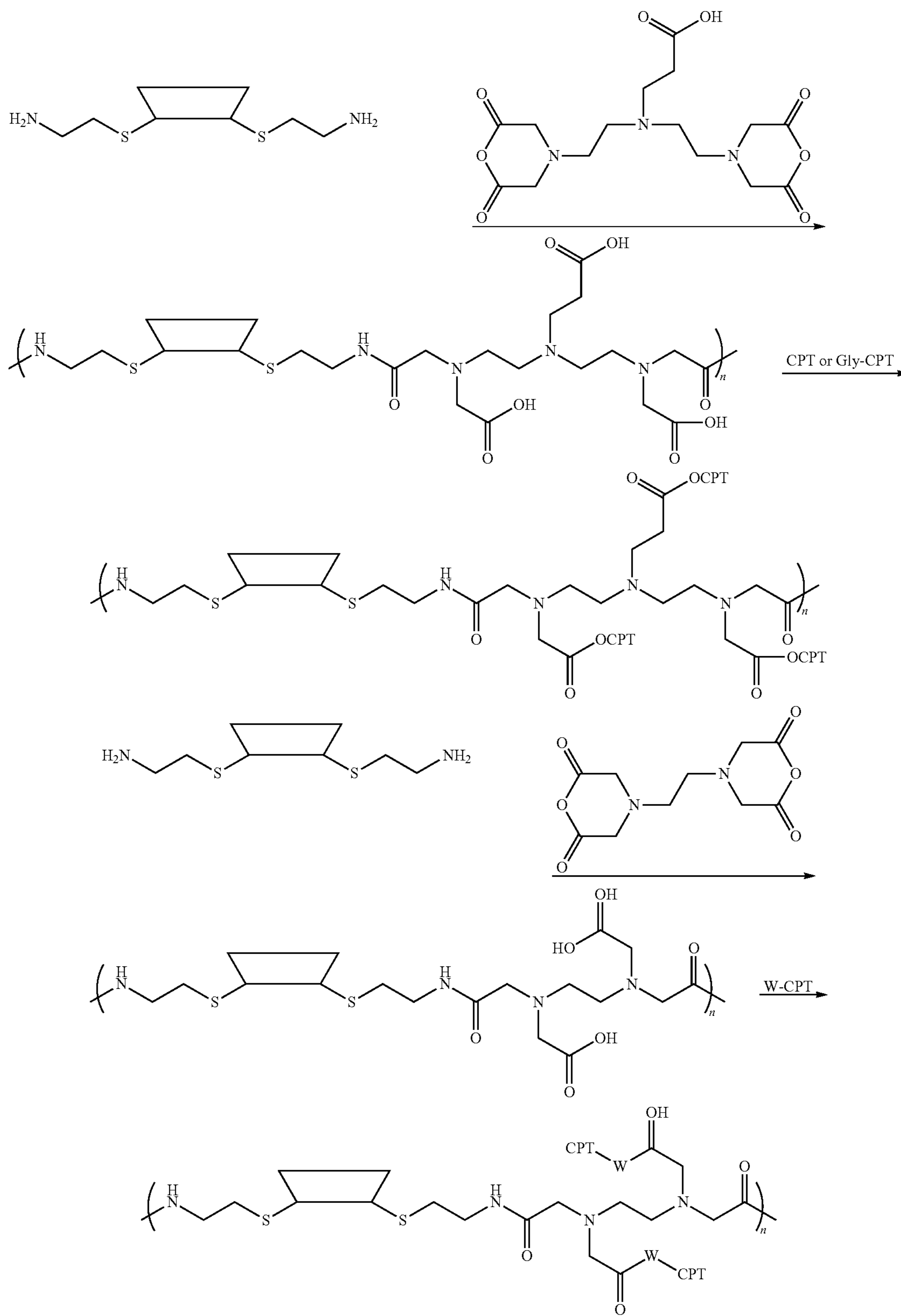
Scheme V
