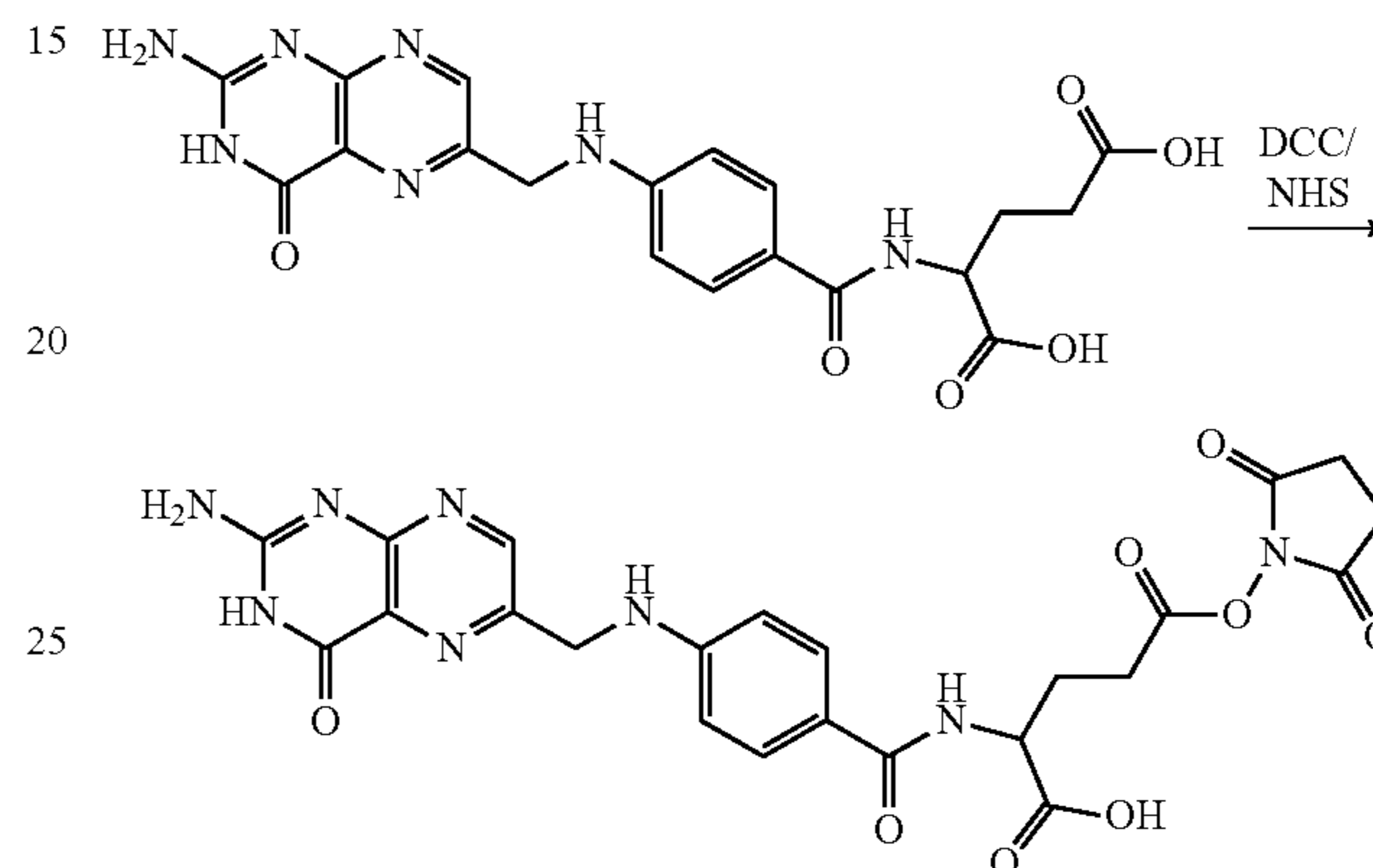
Scheme XXXXIX
