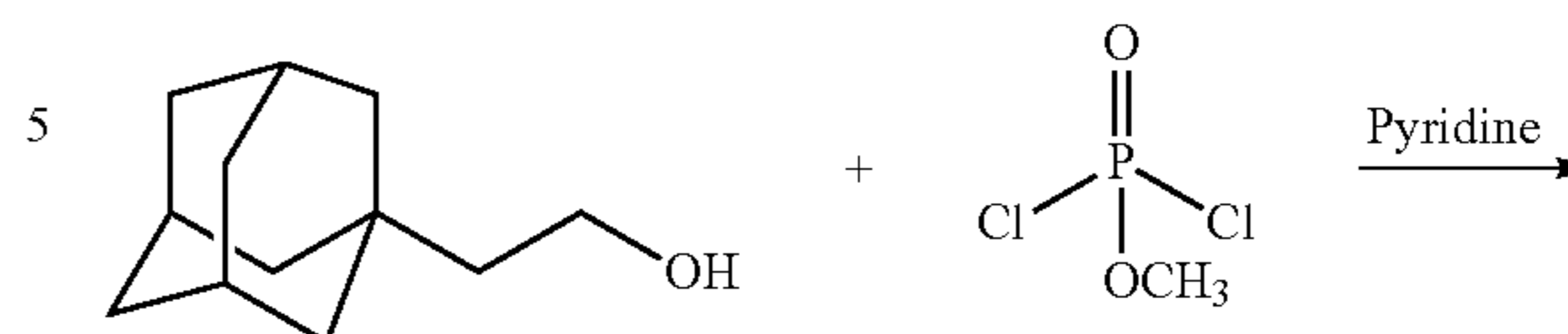
Scheme XXXXVII
