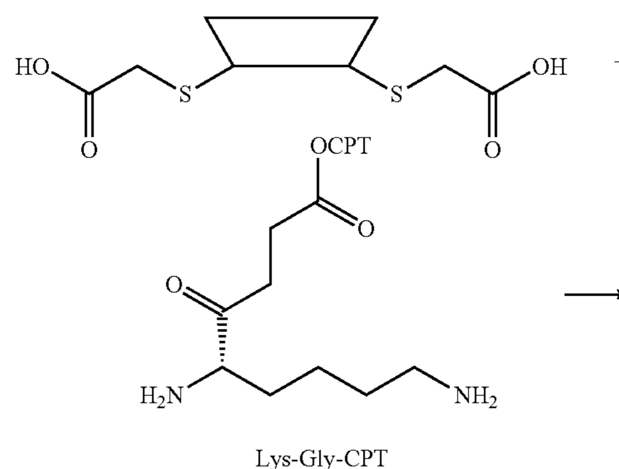
Scheme XXXII
