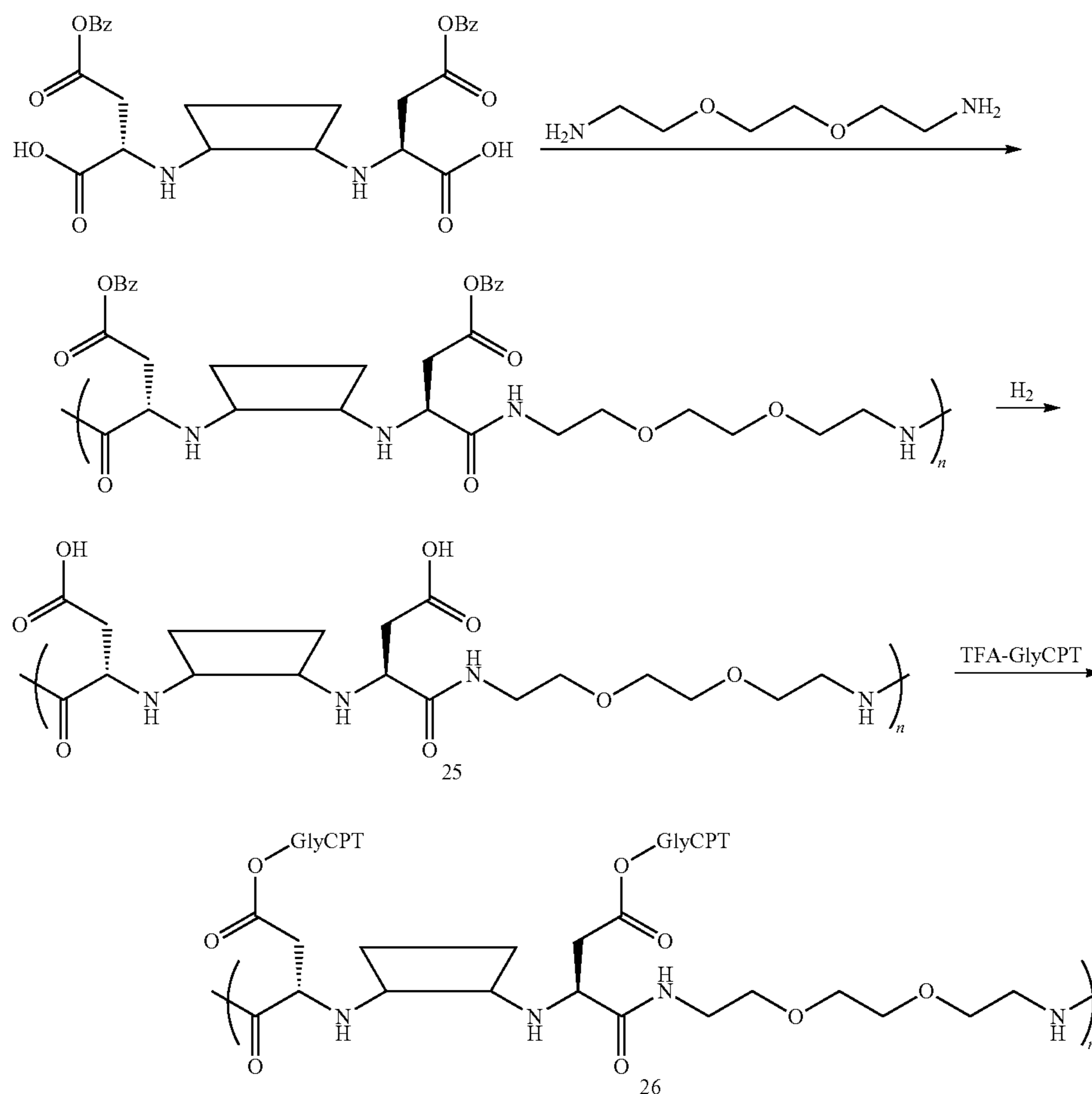
Scheme XXXI
