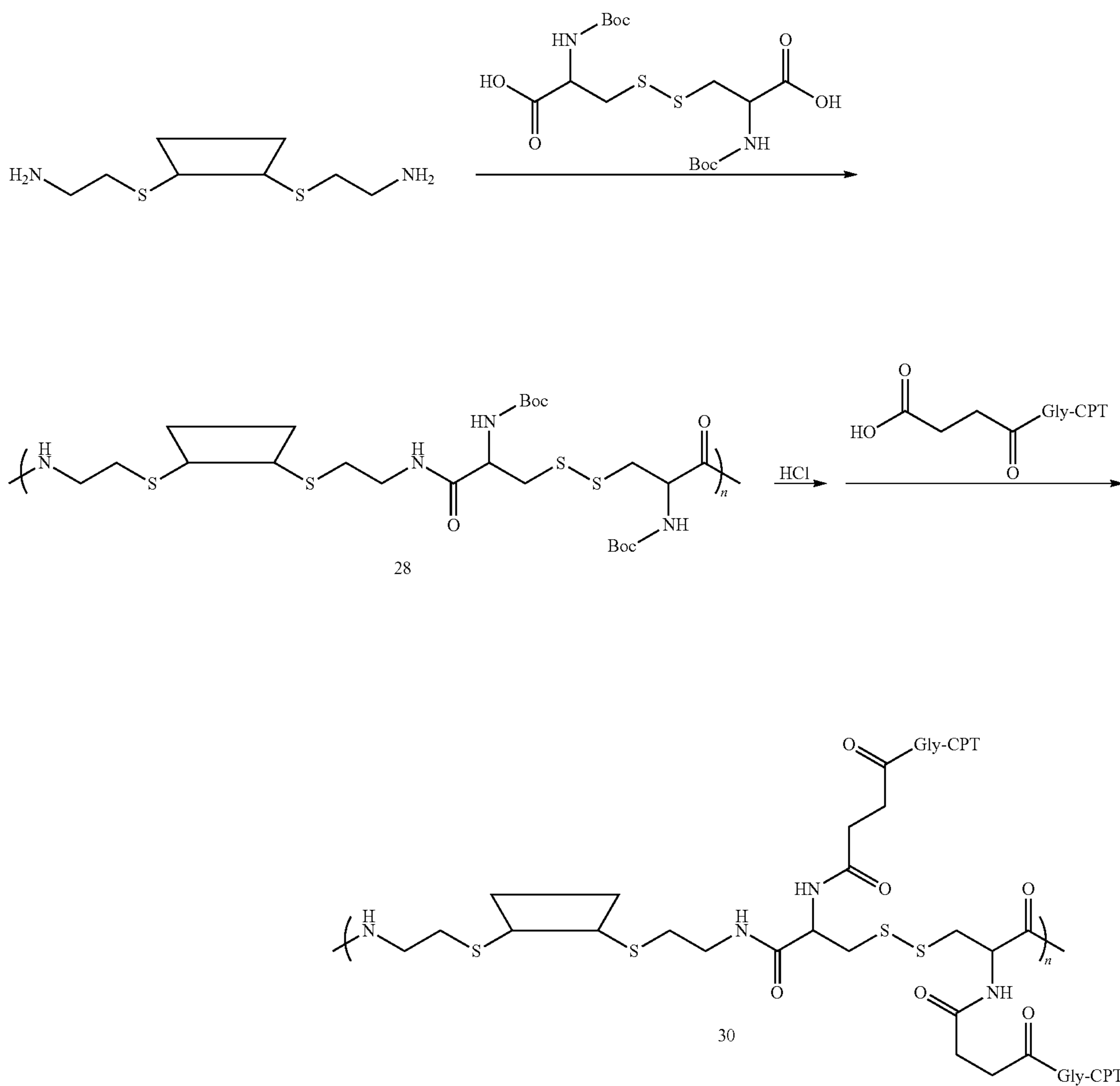
Scheme XXXIII
