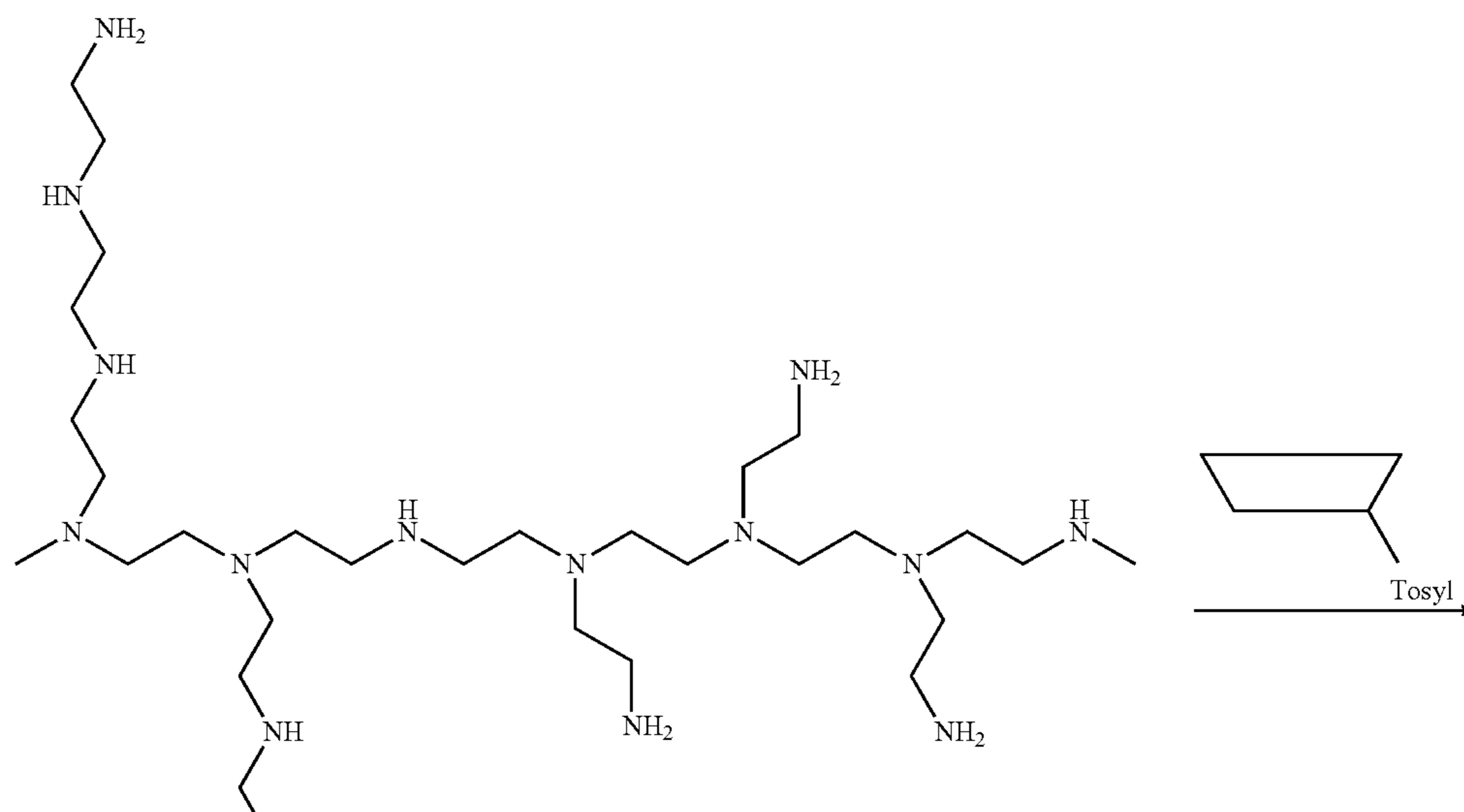
Scheme XXXIV
