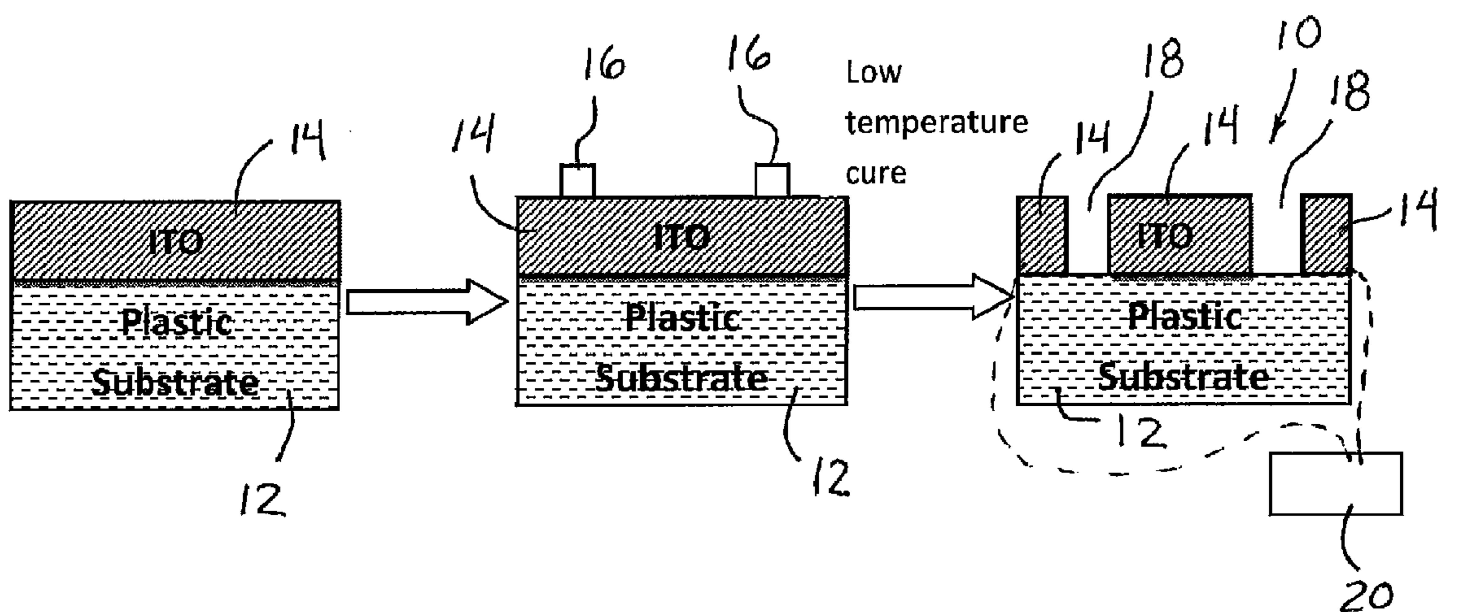
Coat ITO on plastic substrate
