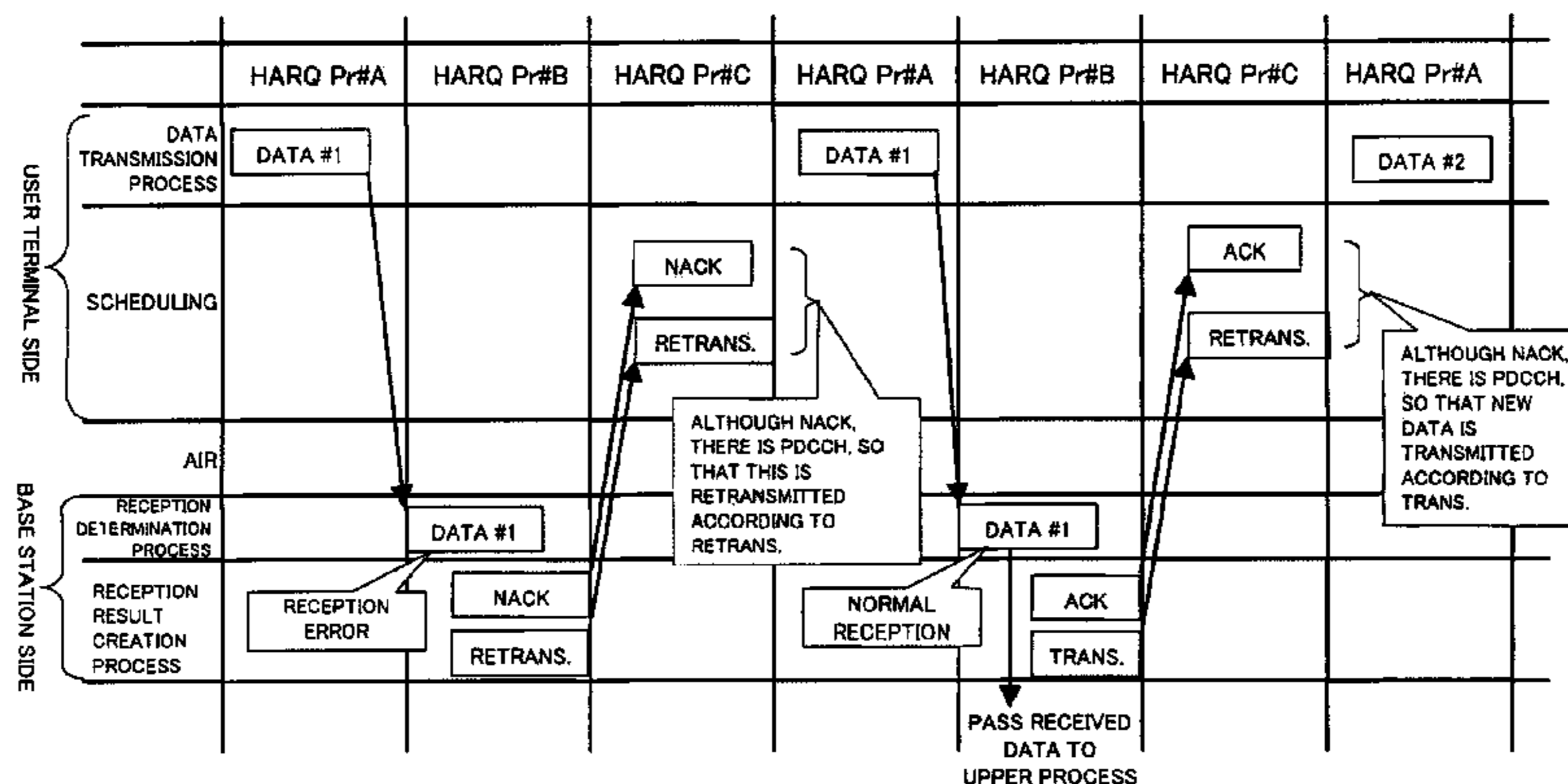
VIEW ILLUSTRATING COMMUNICATION BETWEEN CONVENTIONAL USER TERMINAL AND BASE STATION AND EACH OPERATION
