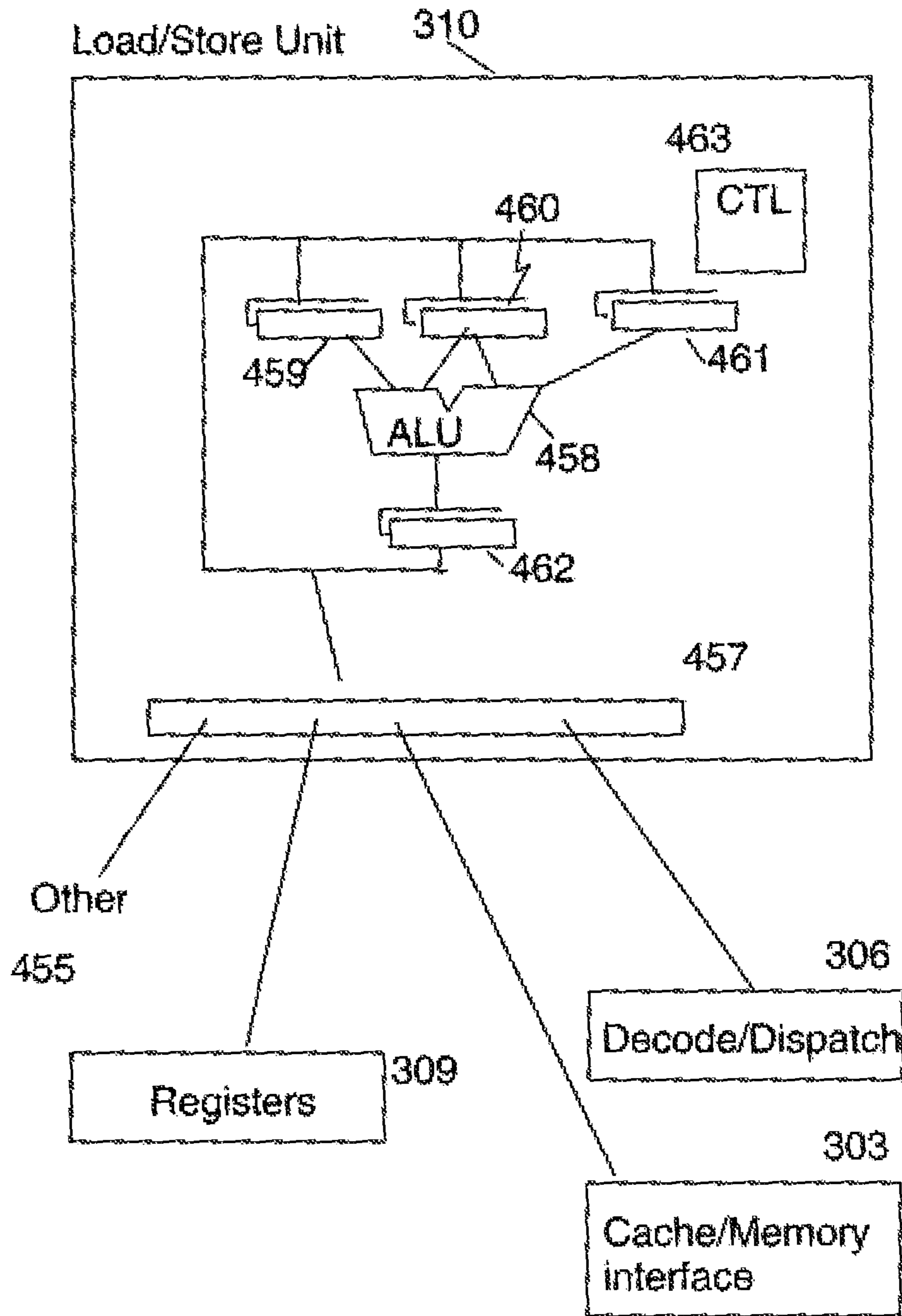
FIG. 4C Prior Art
