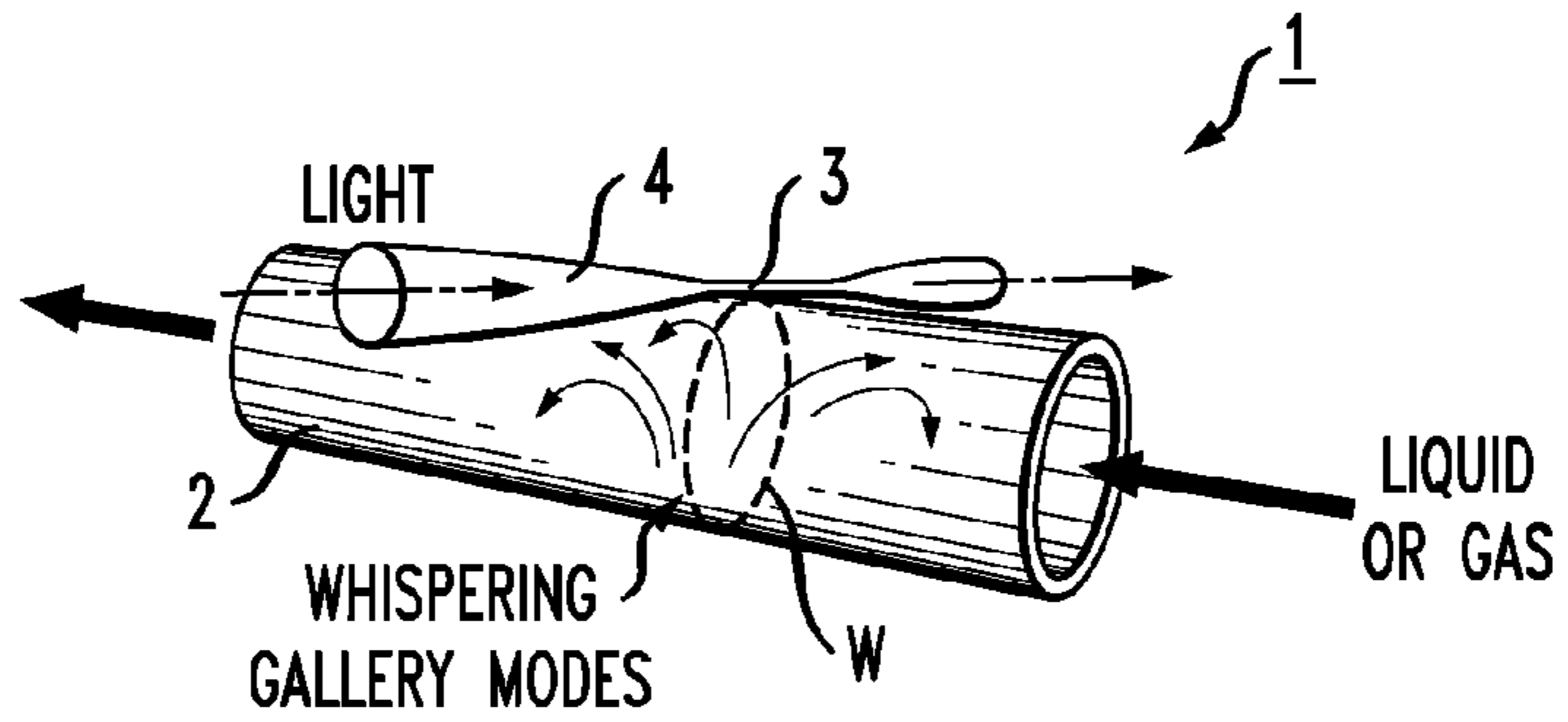
FIG. 1 PRIOR ART
