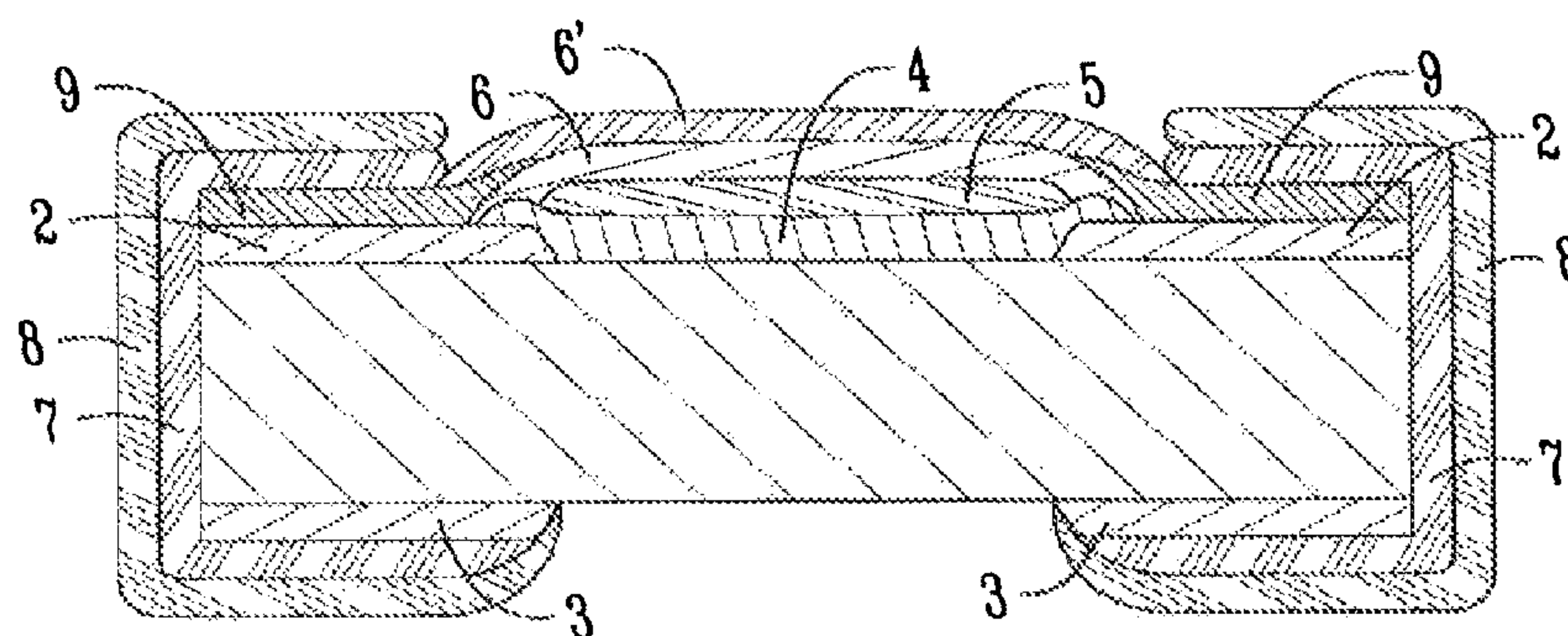
Fig. 3 PRIOR ART
