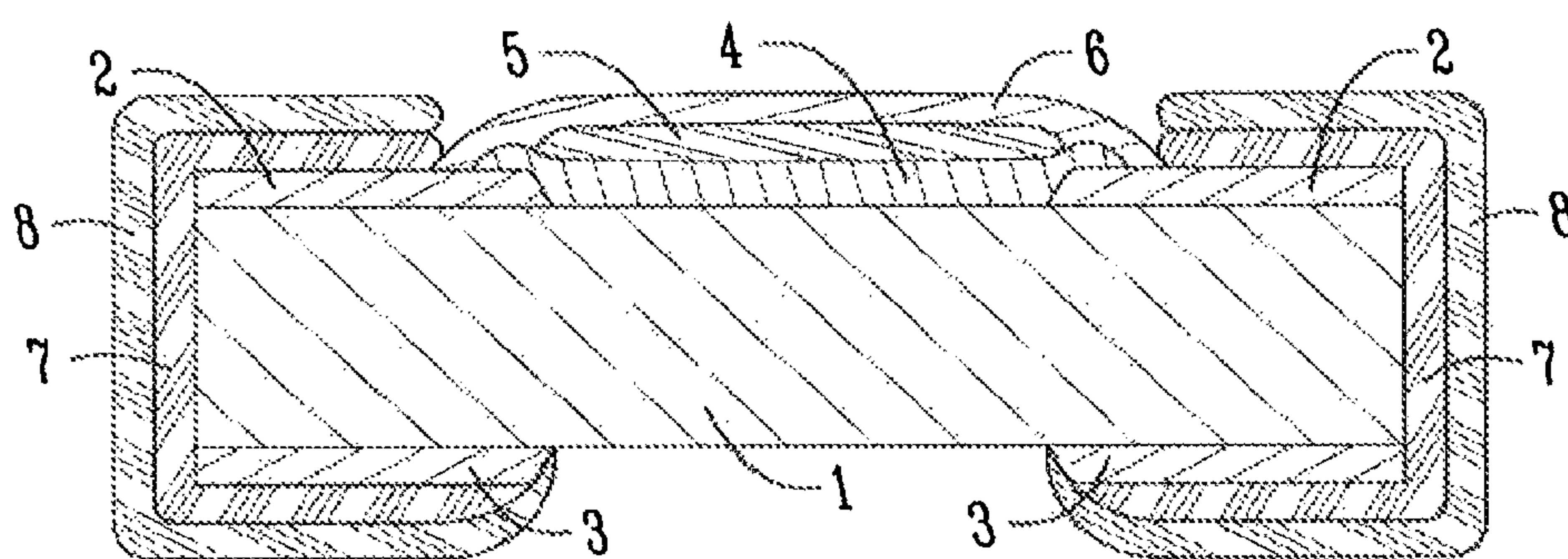
Fig. 2 PRIOR ART
