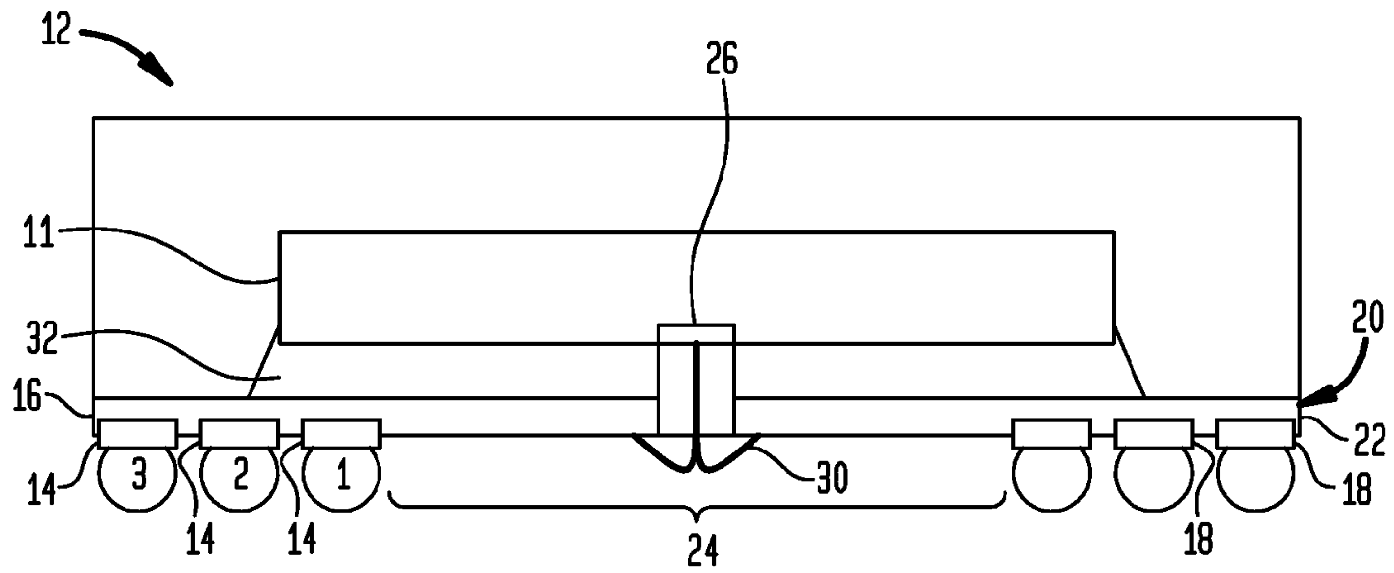
FIG. 1 (PRIOR ART)
