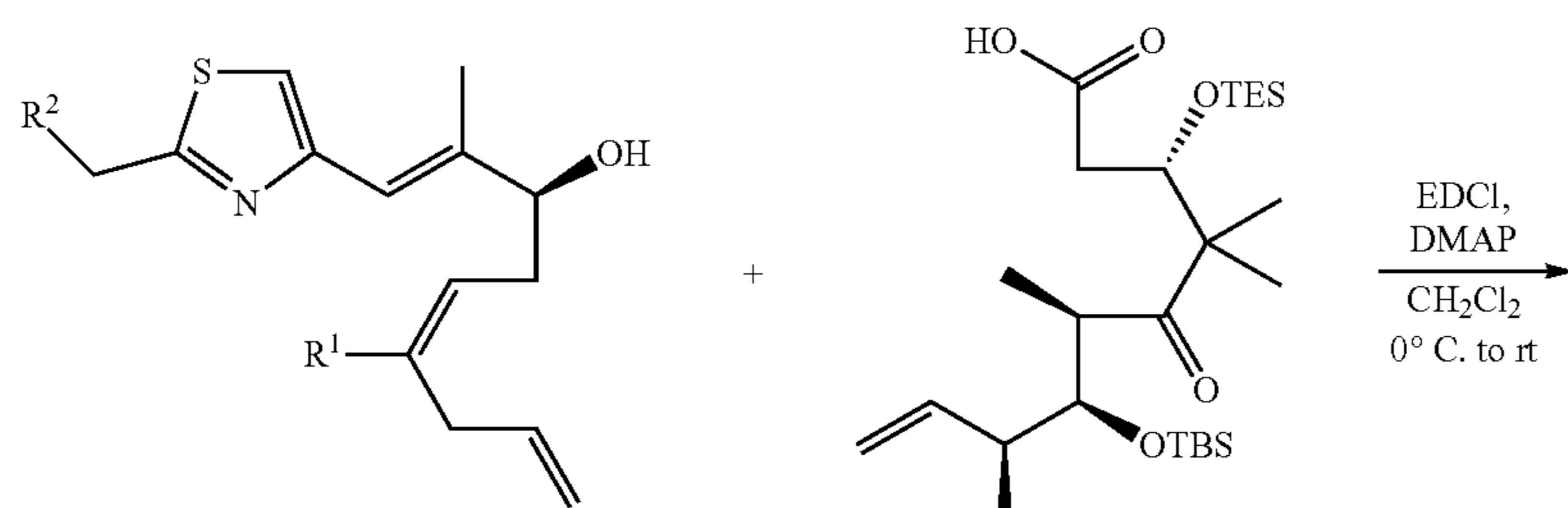
Scheme 7.
