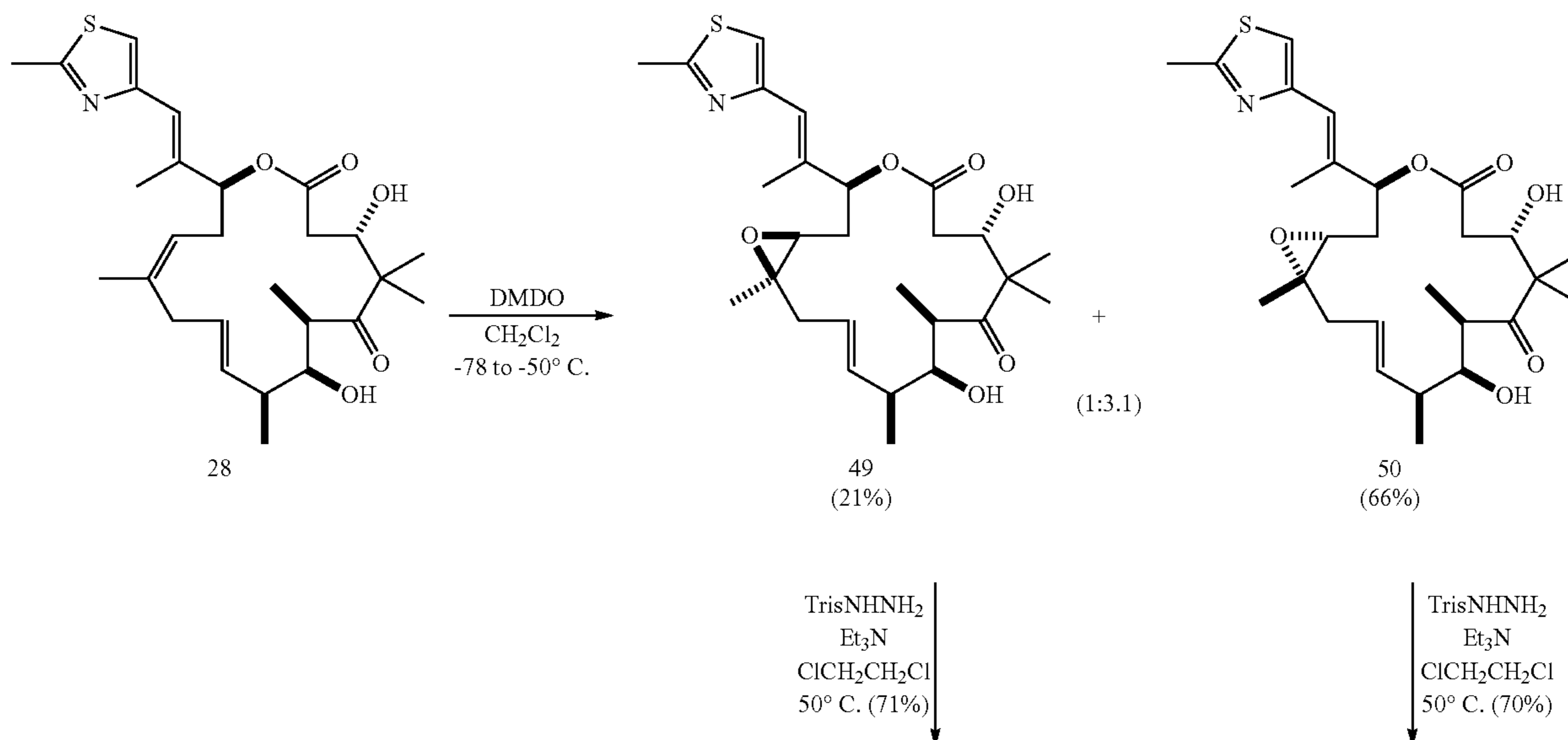
Scheme 9
