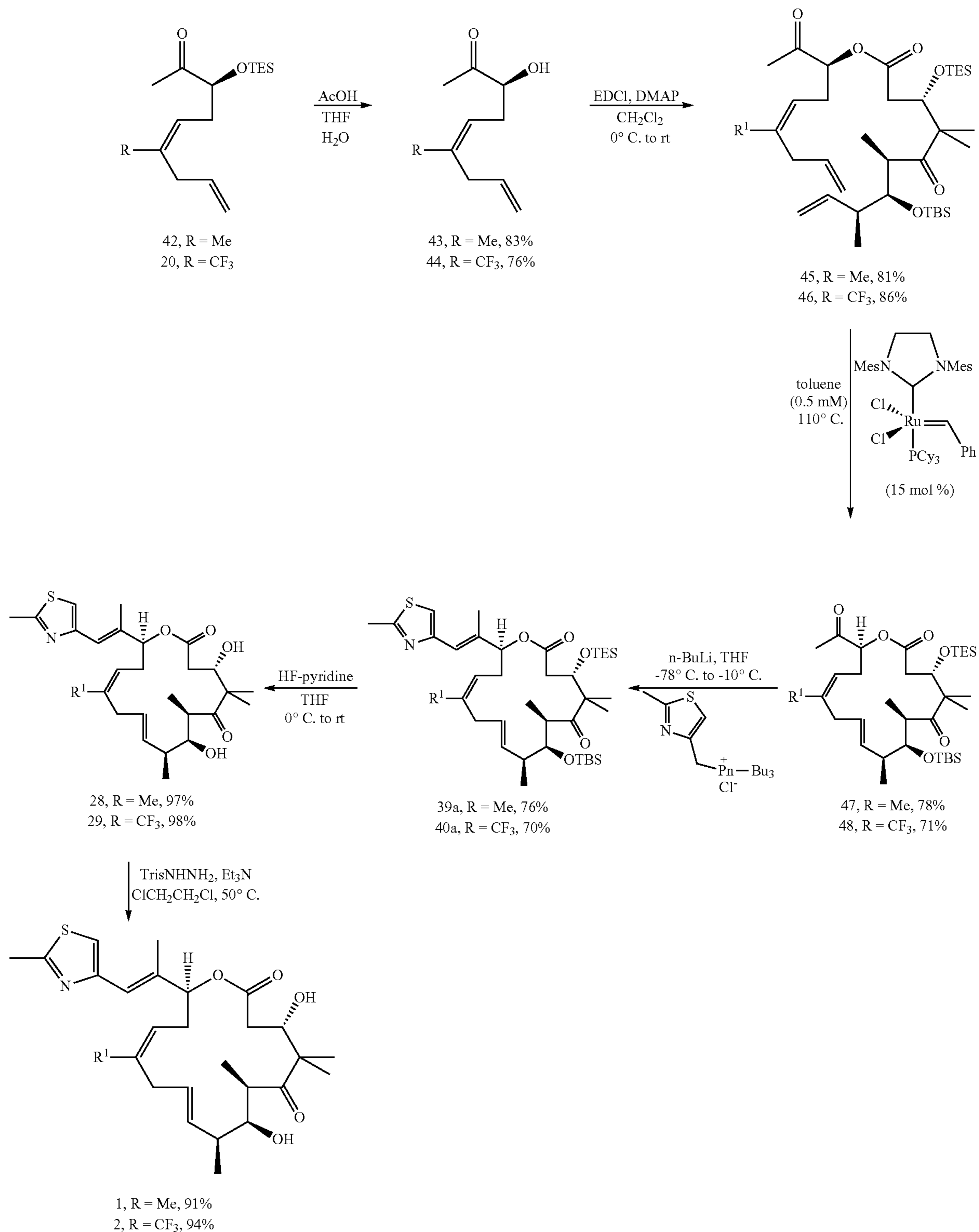
Scheme 8
