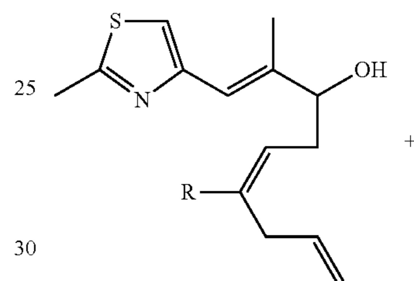
Scheme 5
