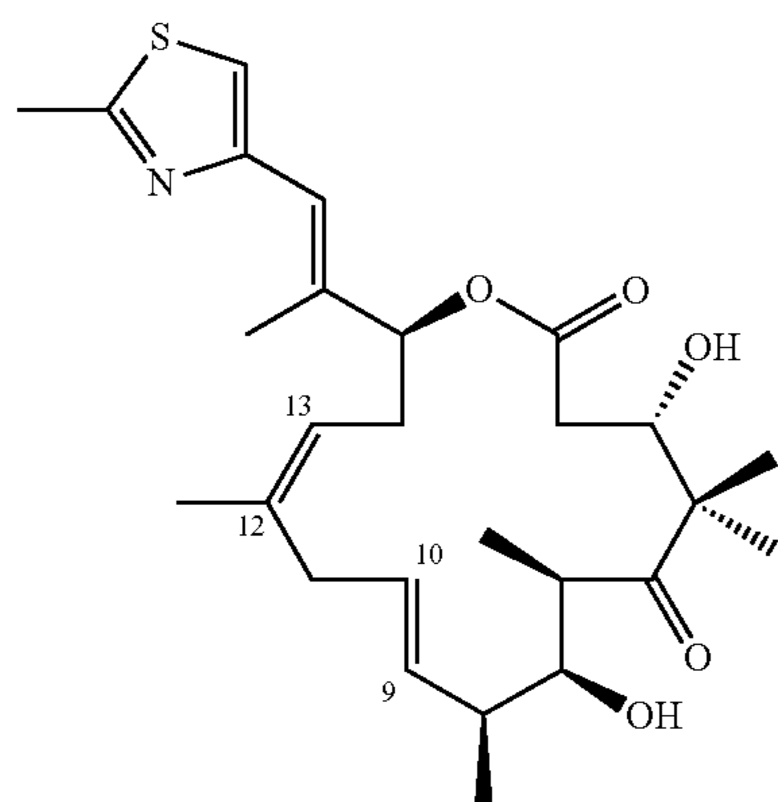
(E)-9,10-dehydro-dEpoB (28)
