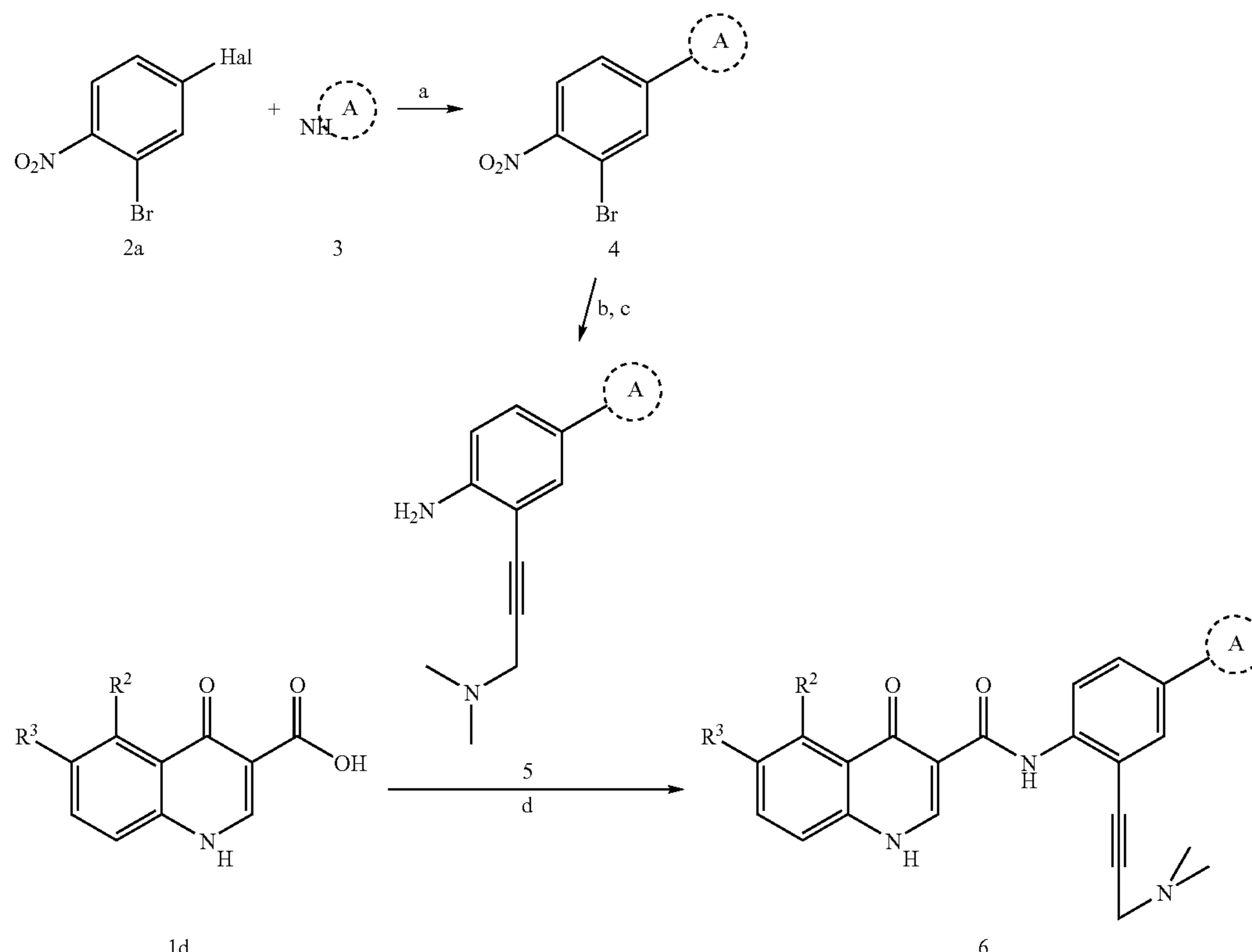
Scheme 2. Preparation of Compounds of Formula (I)
