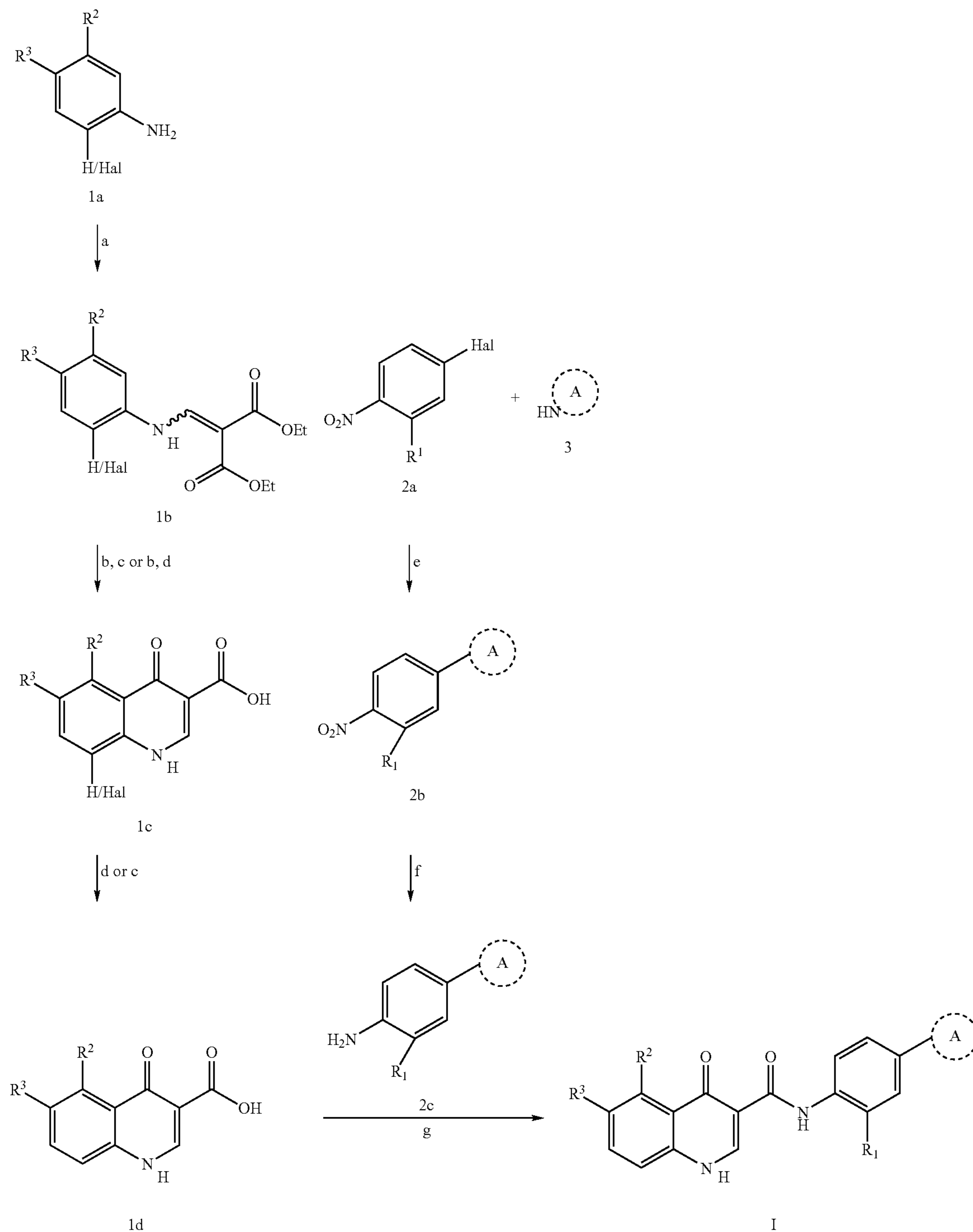
Scheme 1. Preparation of Compounds of Formula (I).
