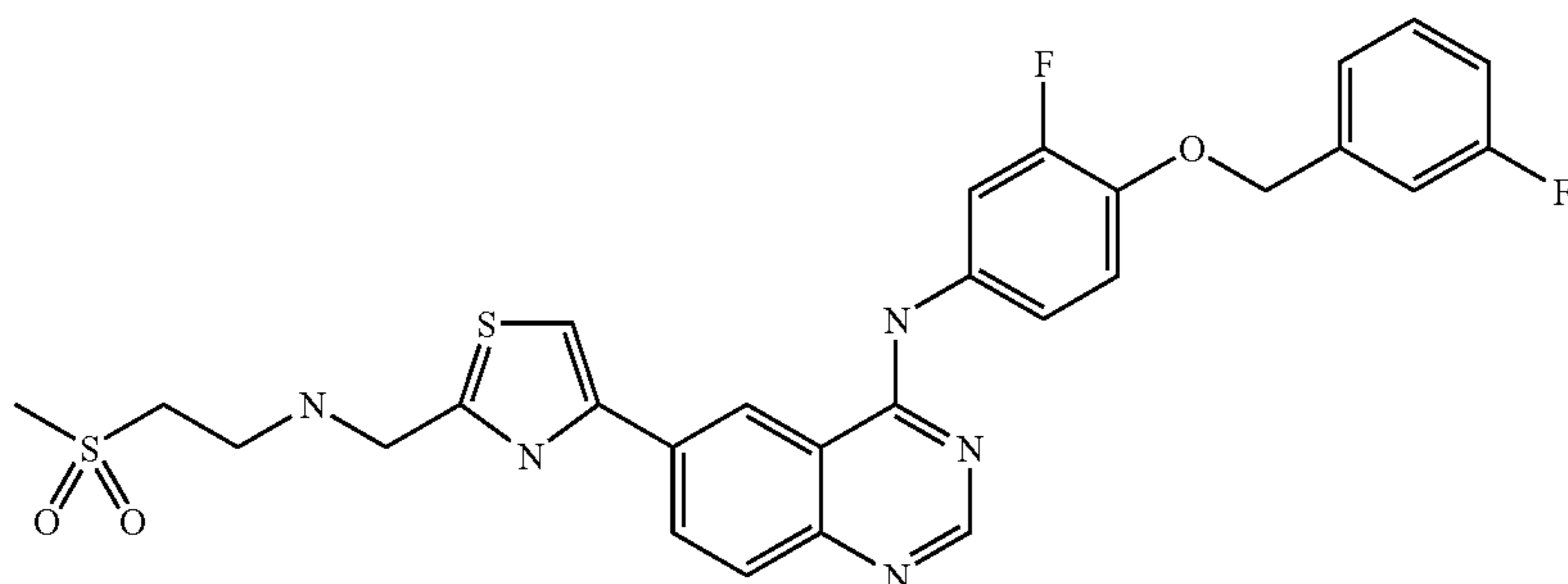
N-{3-fluoro-4-[(3-fluorobenzyl)oxy]phenyl}-6-[2-({2-(methanesulphonyl)ethyl}amino)methyl]-1,3-thiazol-4-yl]-4-quinazolinamine
