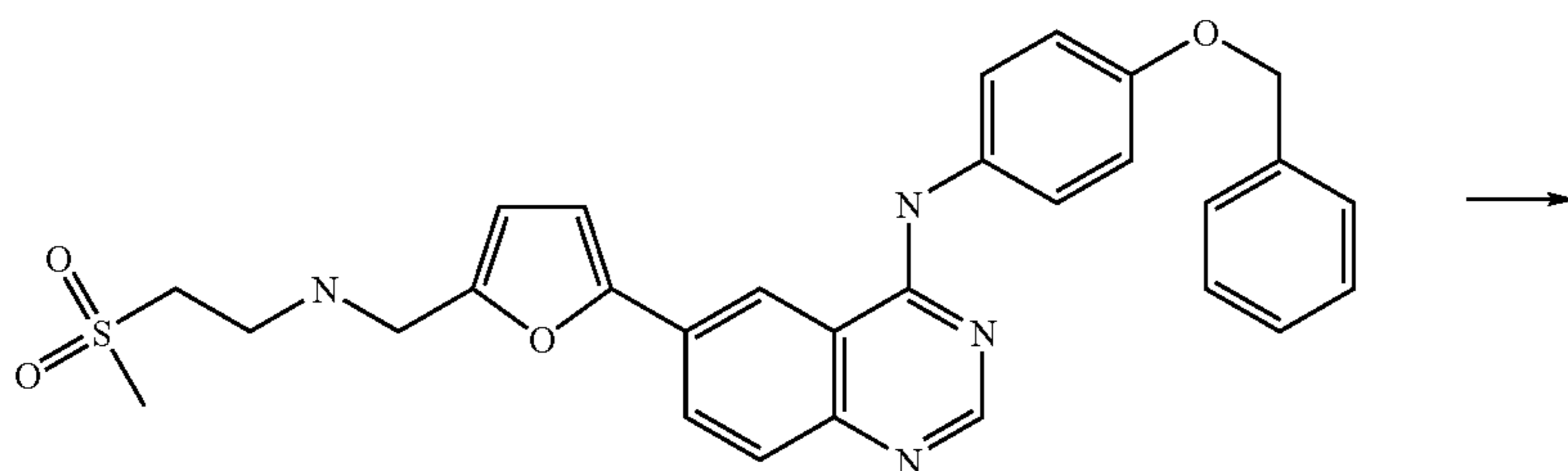
Example 5, m/z 529
