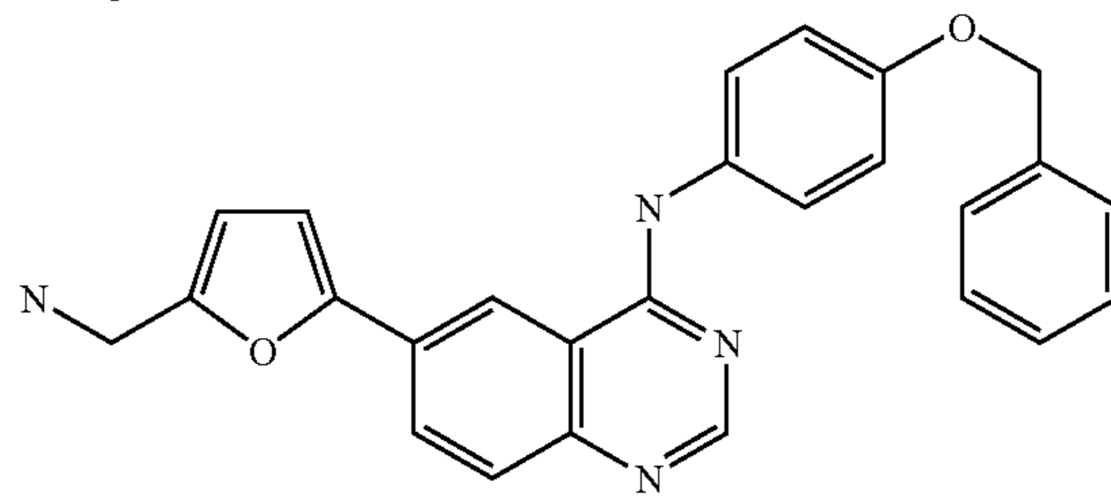
N-dealkylated, m/z 423
