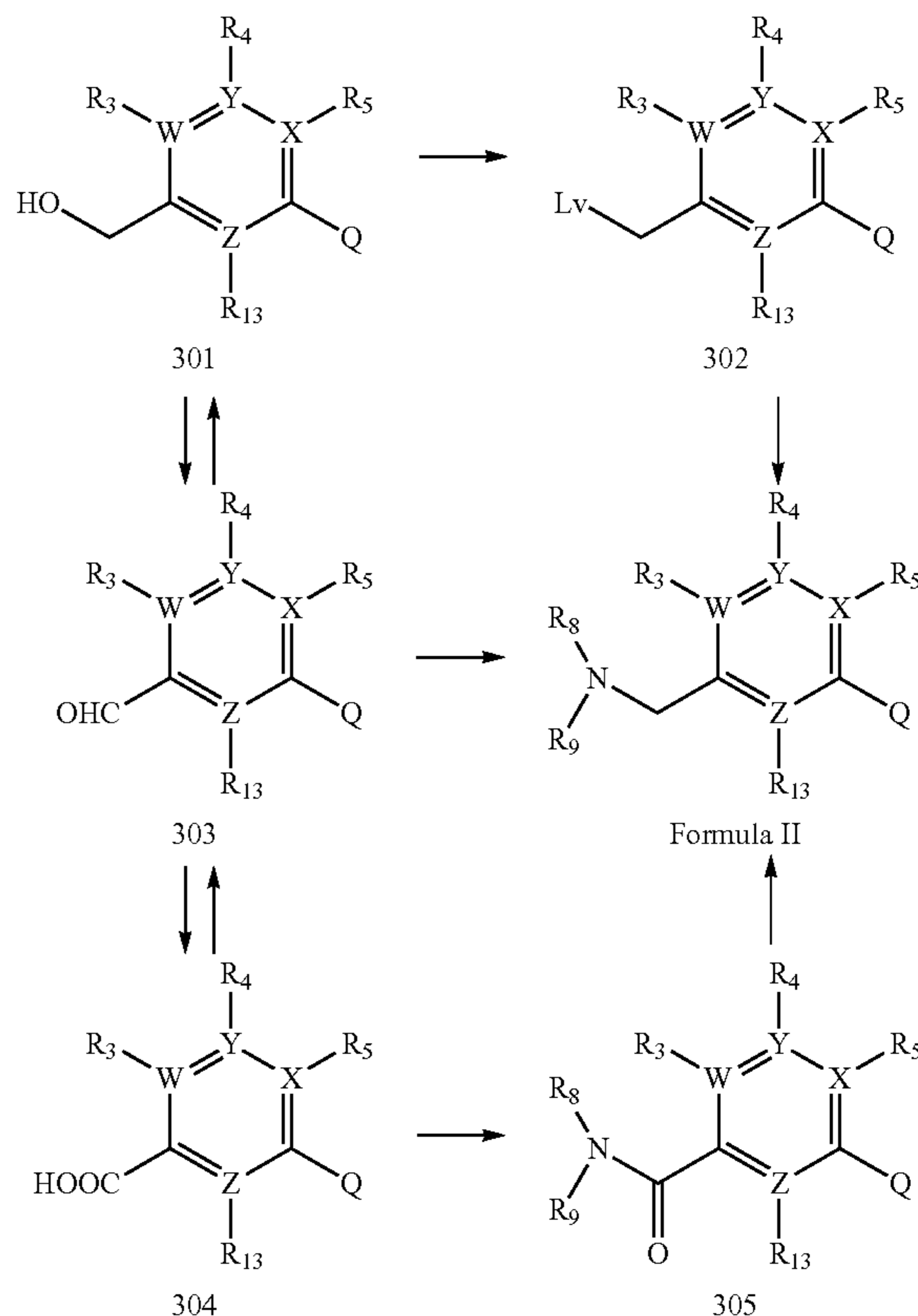
REACTION SCHEME 3
