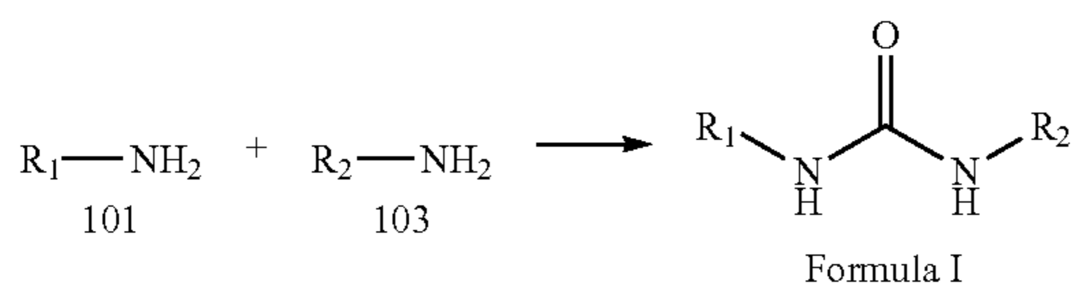
REACTION SCHEME 1
