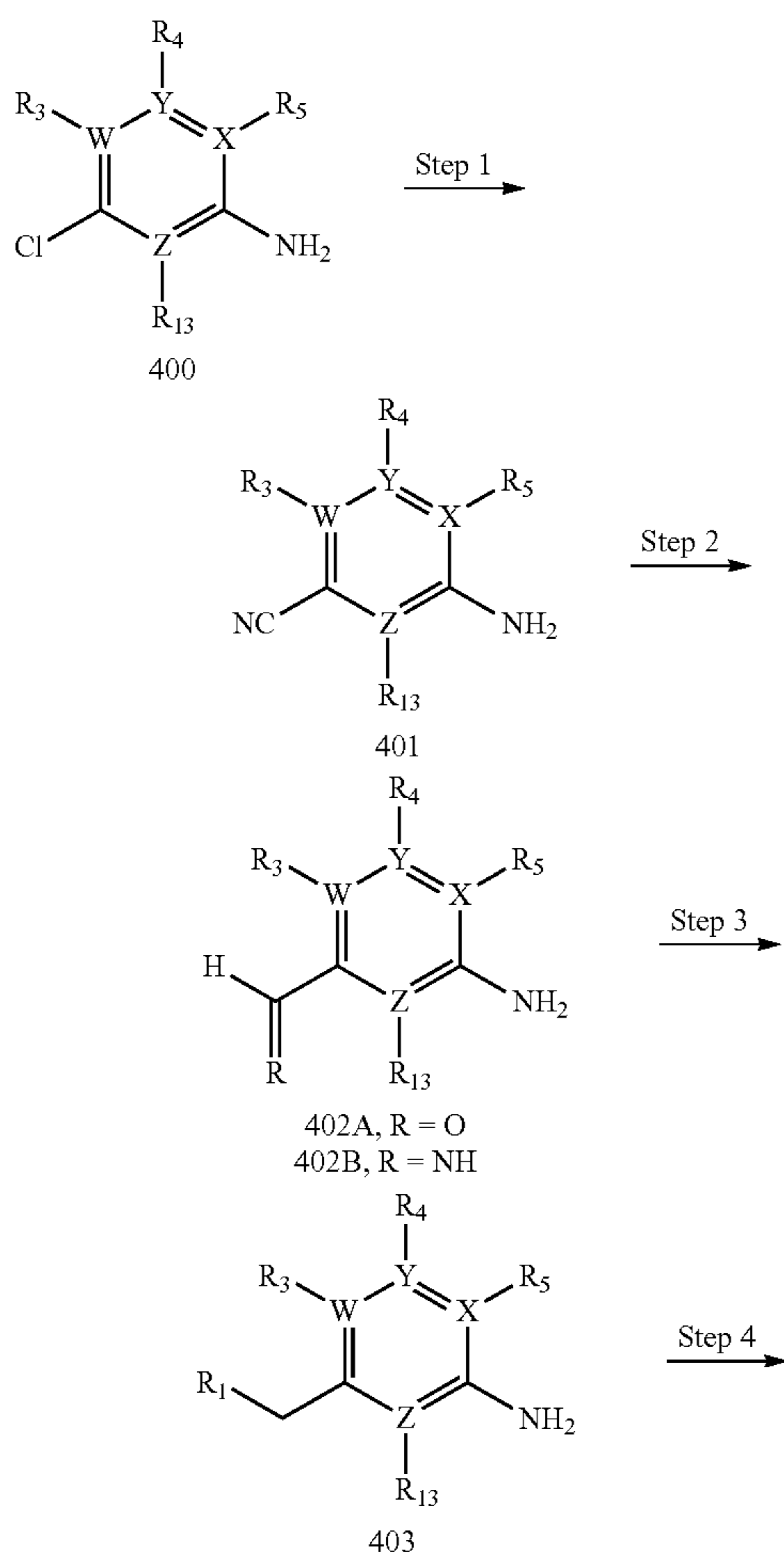
Reaction Scheme 4
