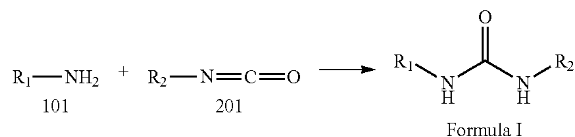
REACTION SCHEME 2
