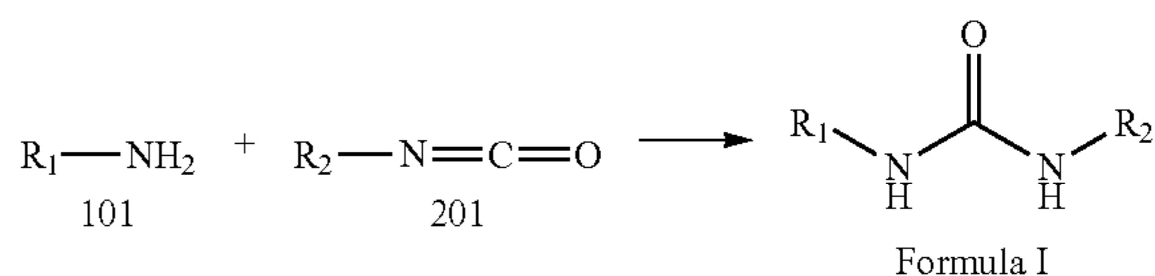
REACTION SCHEME 2
