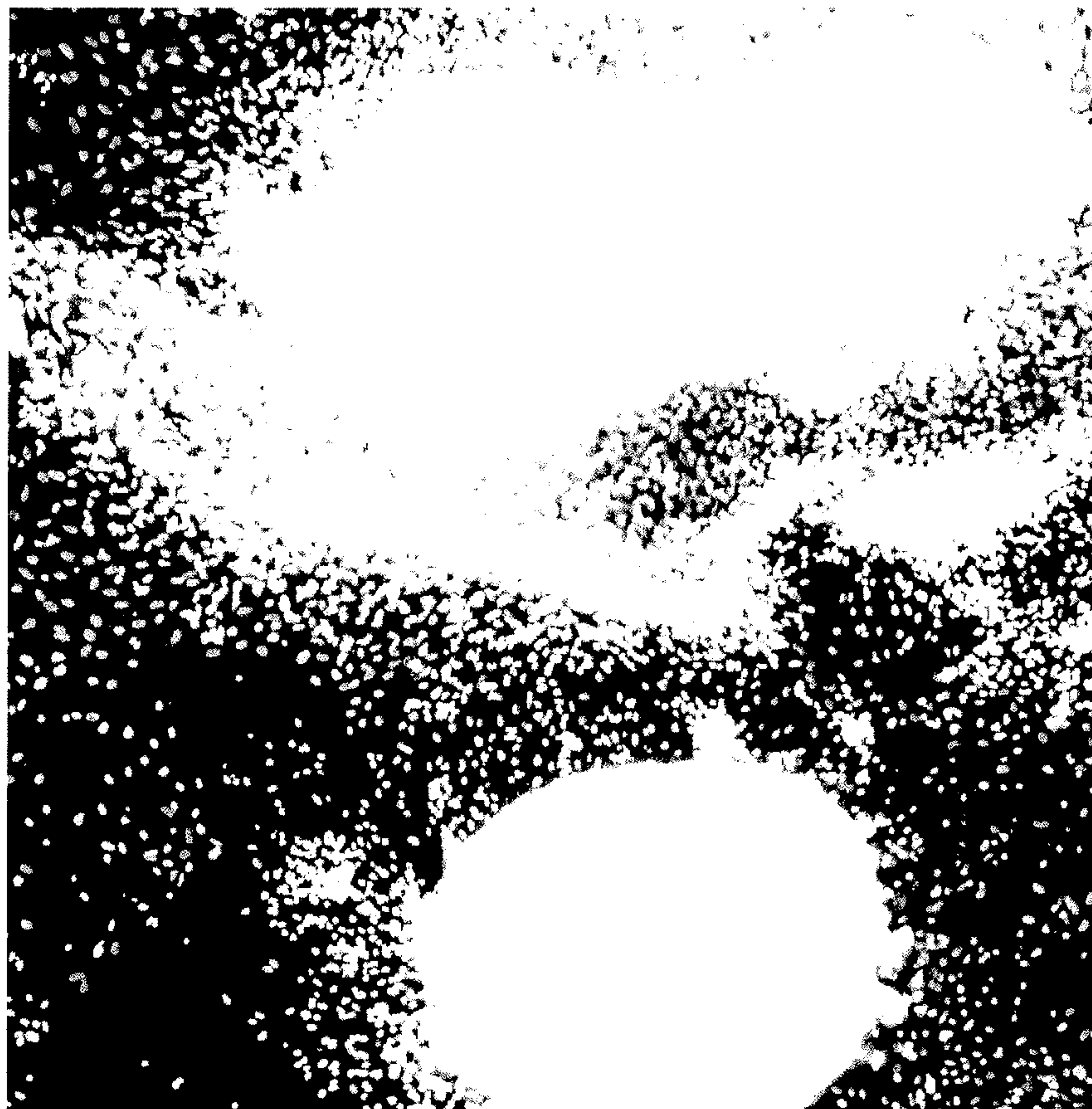
Figure 5A Matrigel
