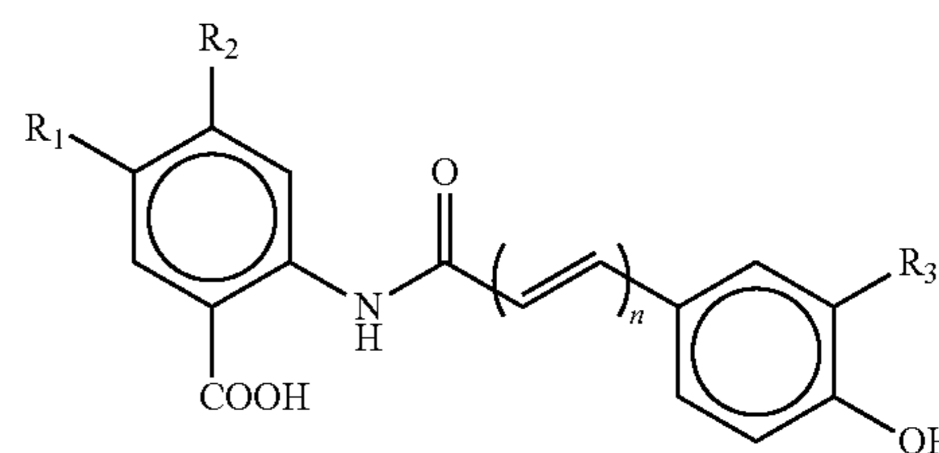
Figure 1. Avenanthramide Nomenclature and Structures
