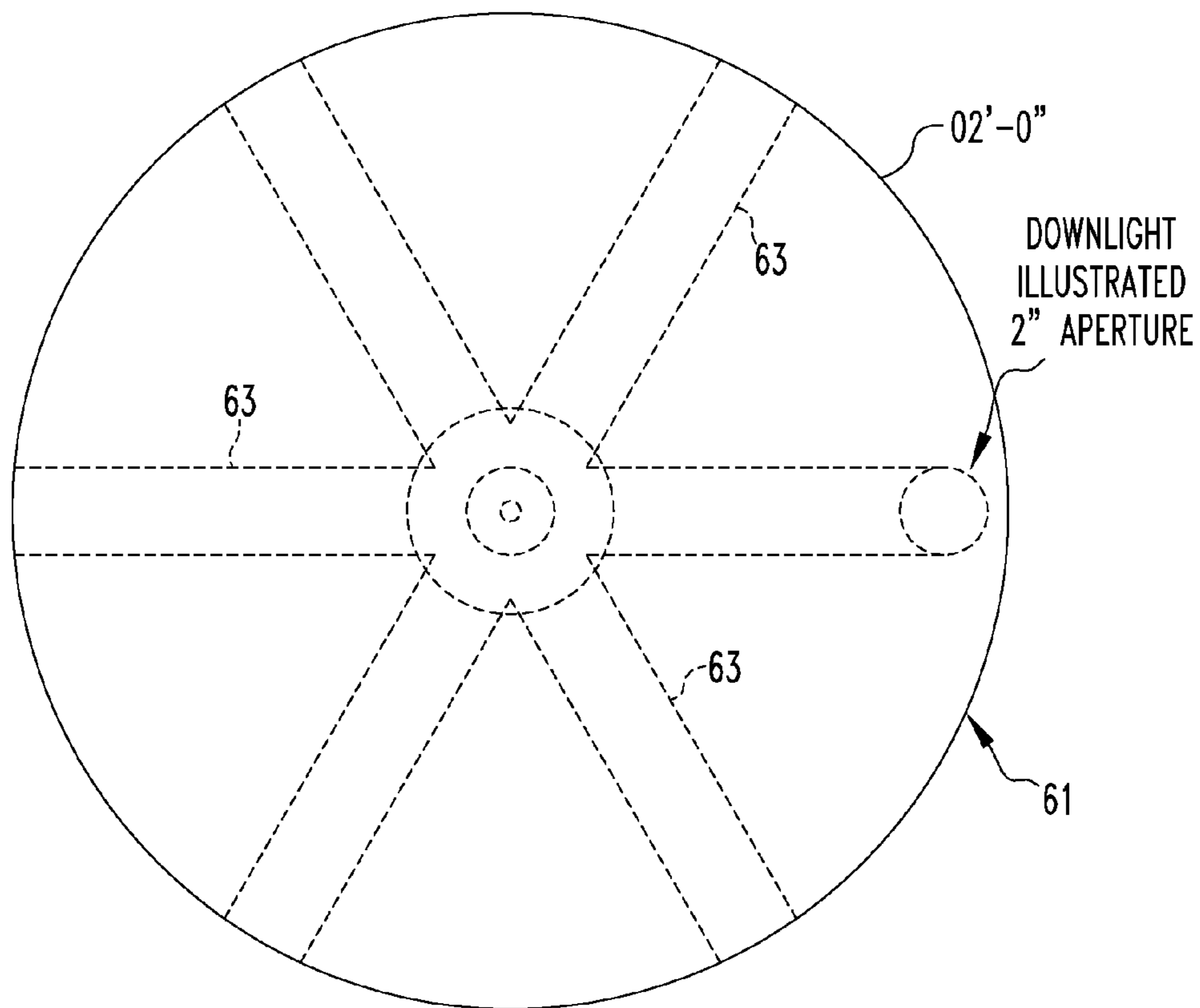
BOTTOM VIEW
