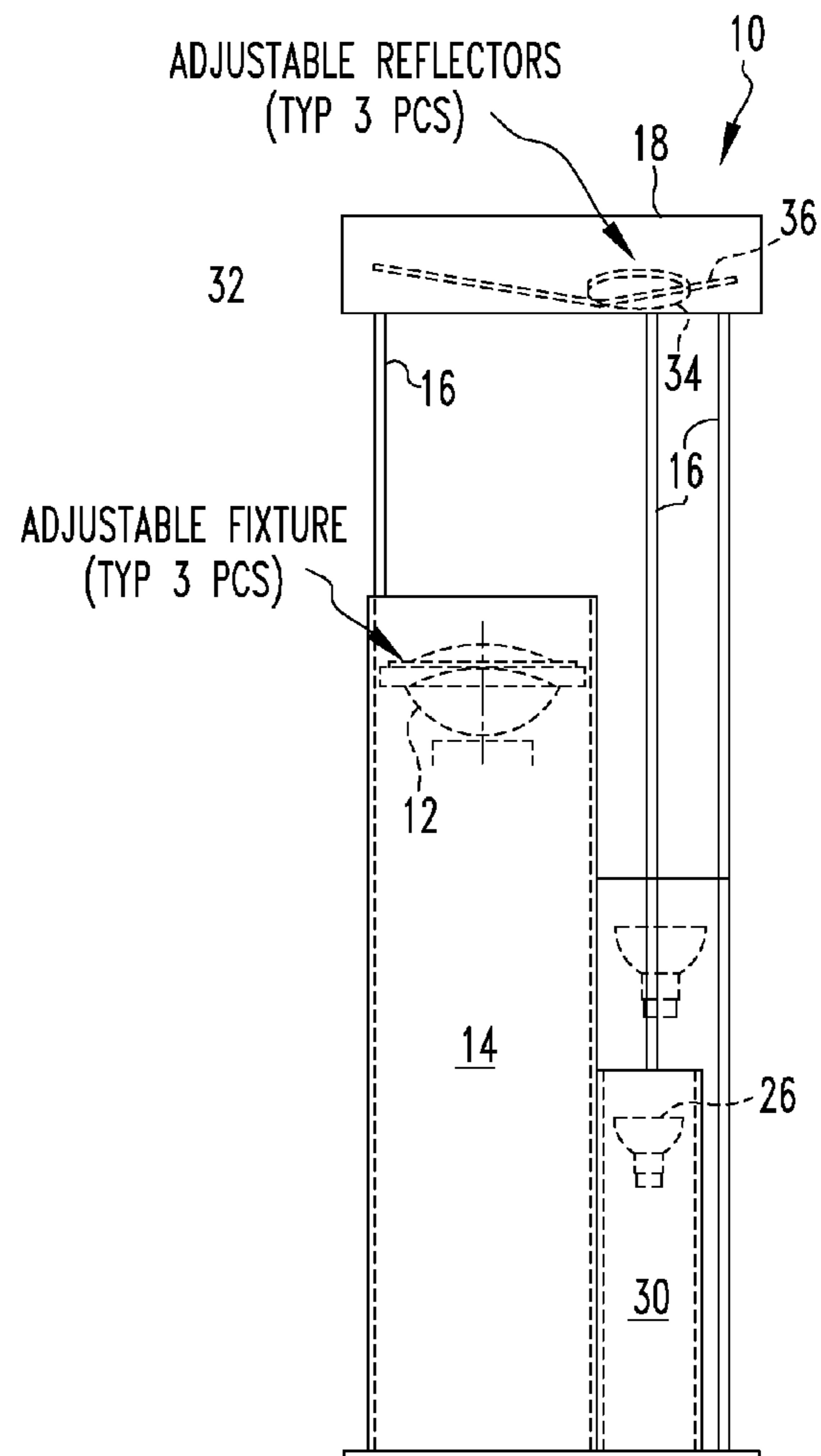
FRONT VIEW FIG. 43
