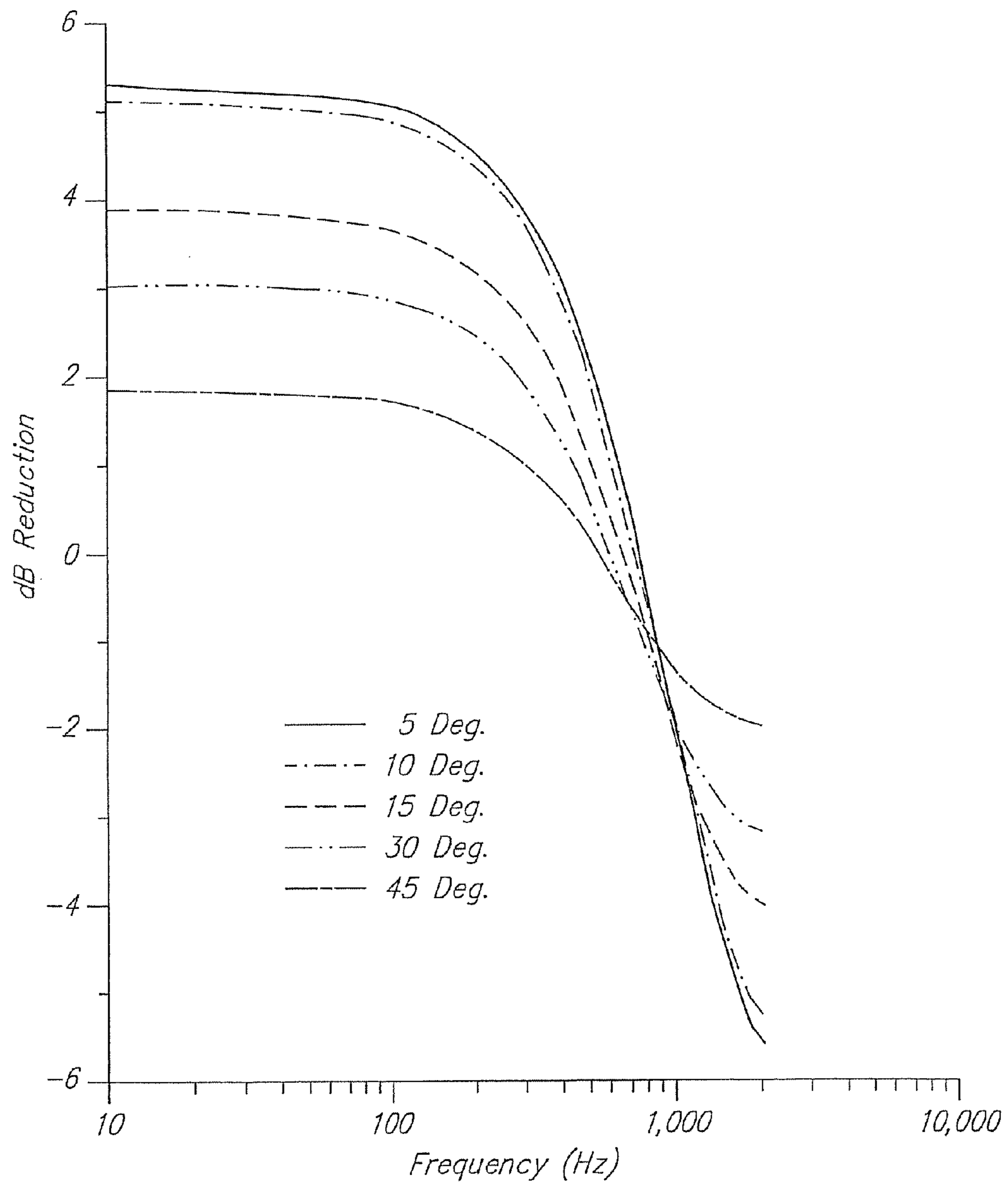
Function Of Flow Angle – Panel Response 32 in. x 12 in. Panel, Mode 1,1 Mach = 0.85, Alt = 35K ft. Distance From Nose = 300 in.
