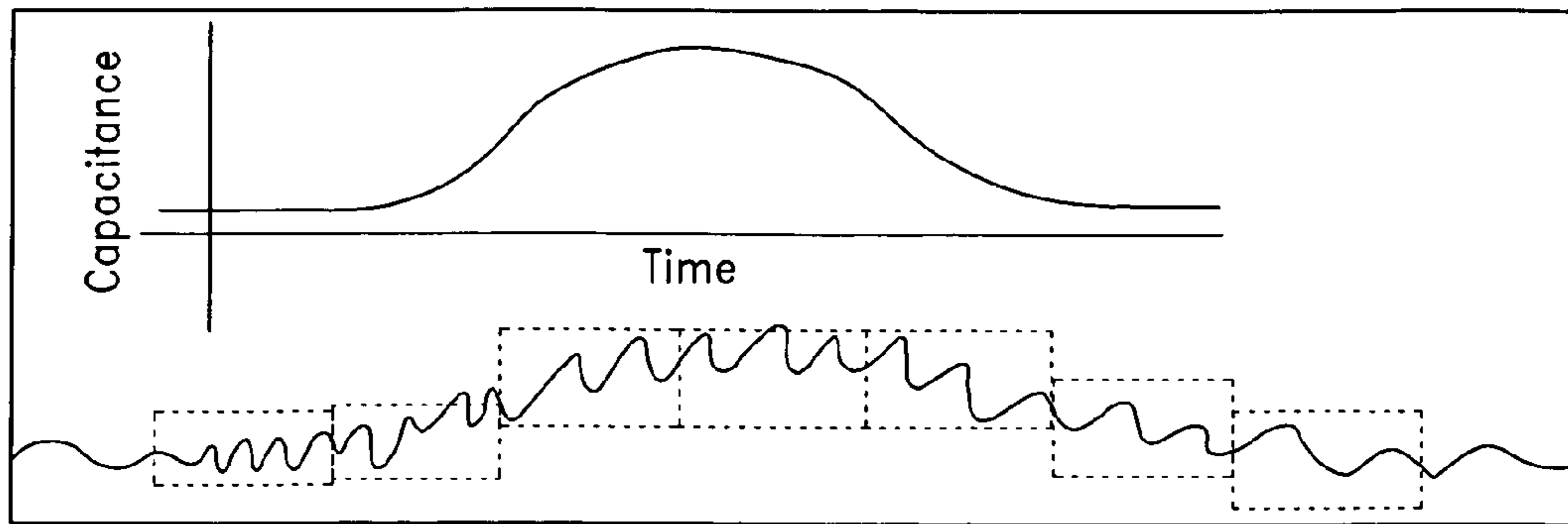
Fig. 11 (Prior Art)
