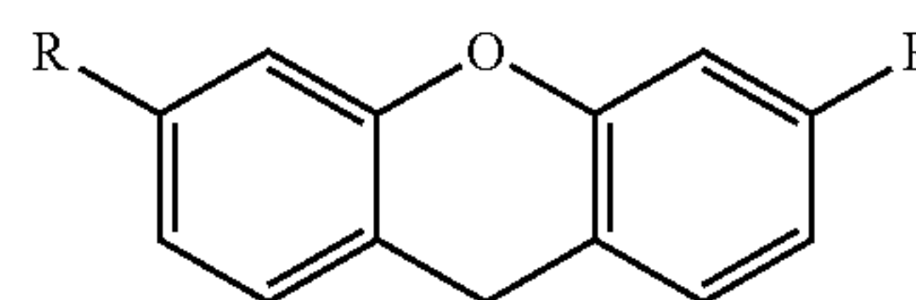
Structure B: Basic Xanthene Structure
