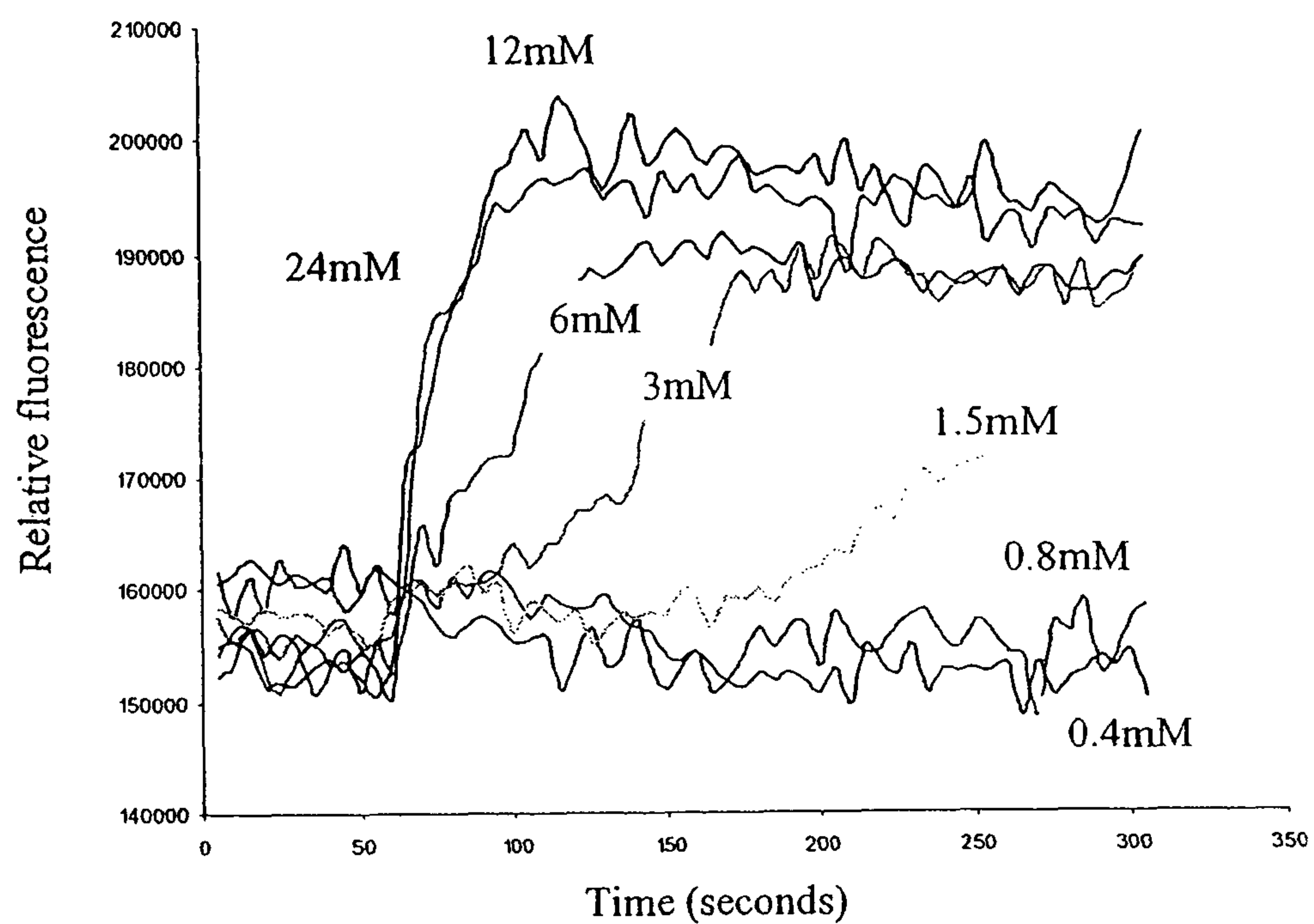
CW Experiments - Fluorescent Response vs Glucose Addition (Concs in mmol) - averaged data
