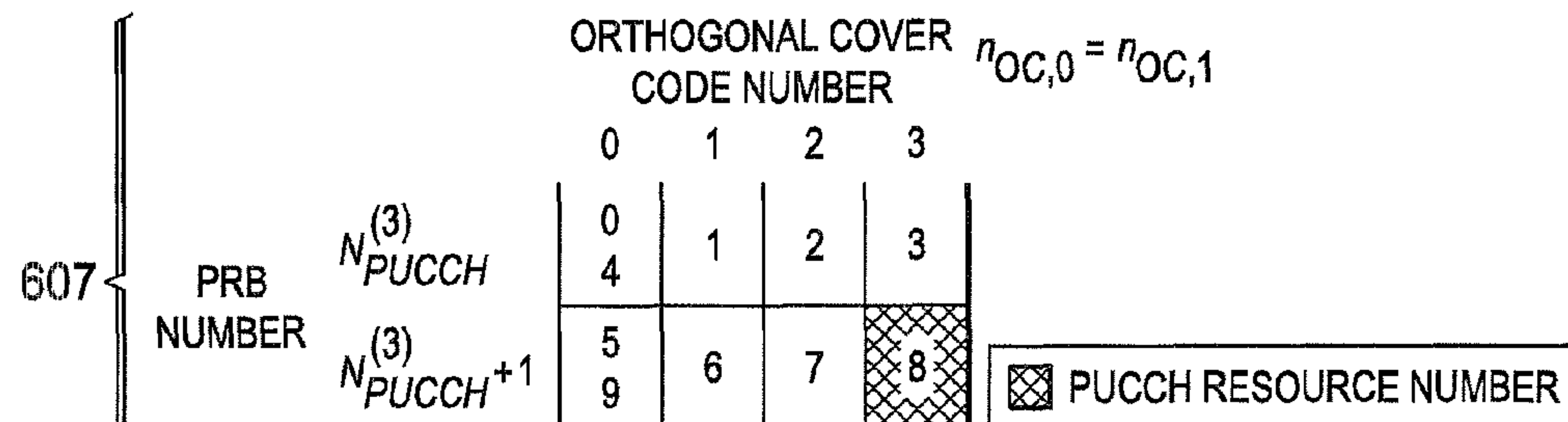
(d) DETERMINATION OF OCC AND PRB NUMBERS OF A (SHORTENED) PUCCH FORMAT X TRANSMITTED IN AN SRS SUBFRAME ACCORDING TO EXAMPLE 3
