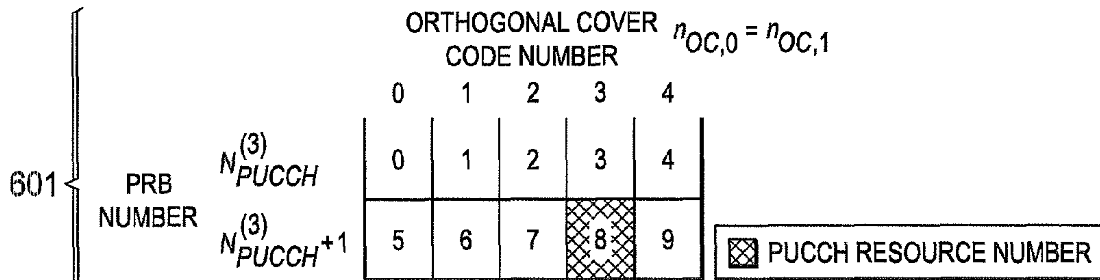
(a) DETERMINATION OF OCC AND PRB NUMBERS OF A PUCCH FORMAT X TRANSMITTED IN A NORMAL SUBFRAME
