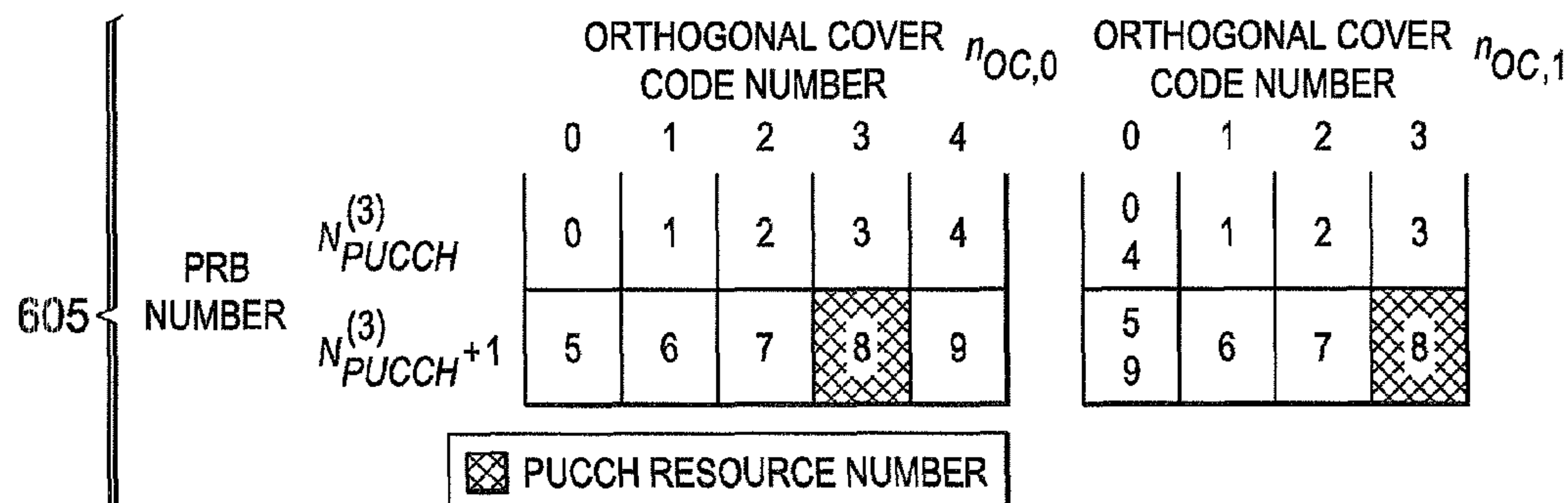
(c) DETERMINATION OF OCC AND PRB NUMBERS OF A (SHORTENED) PUCCH FORMAT X TRANSMITTED IN AN SRS SUBFRAME ACCORDING TO EXAMPLE 2
