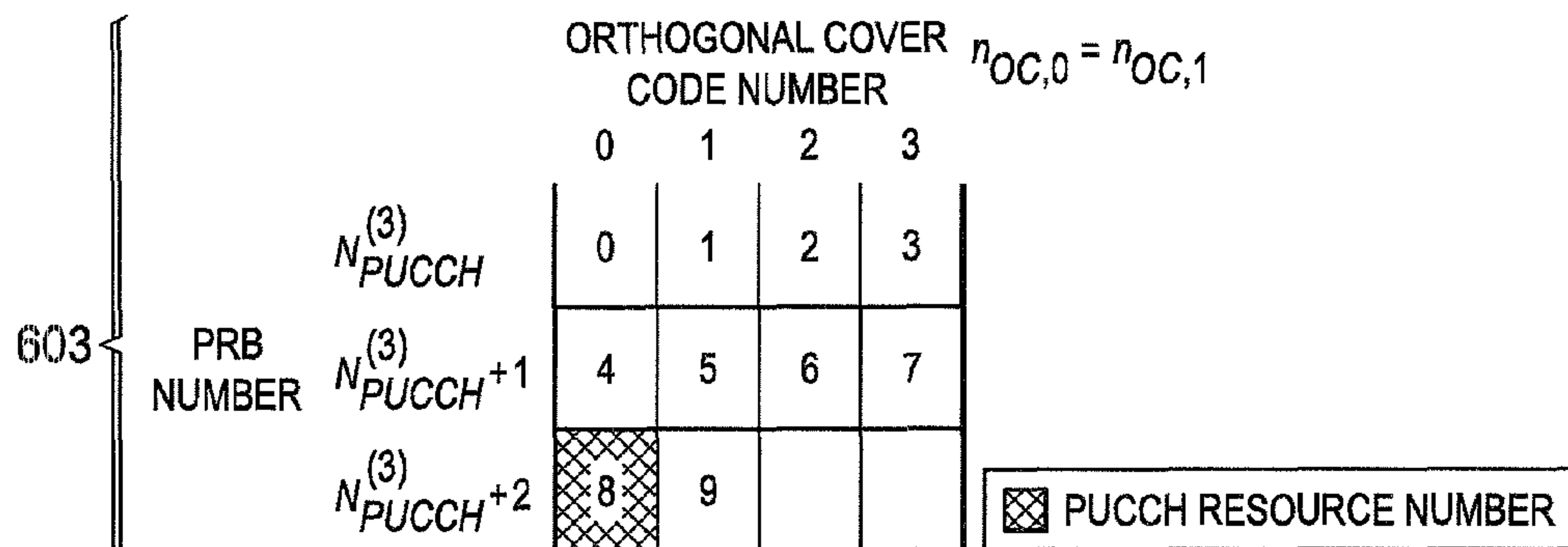
(b) DETERMINATION OF OCC AND PRB NUMBERS OF A (SHORTENED) PUCCH FORMAT X TRANSMITTED IN AN SRS SUBFRAME ACCORDING TO EXAMPLE 1
