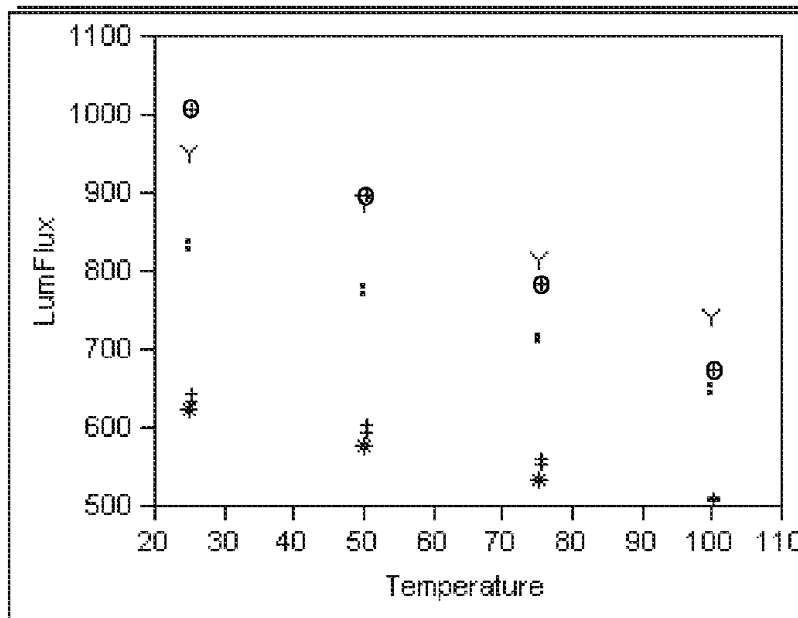
Bivariate Fit of LumFlux By Temperature
