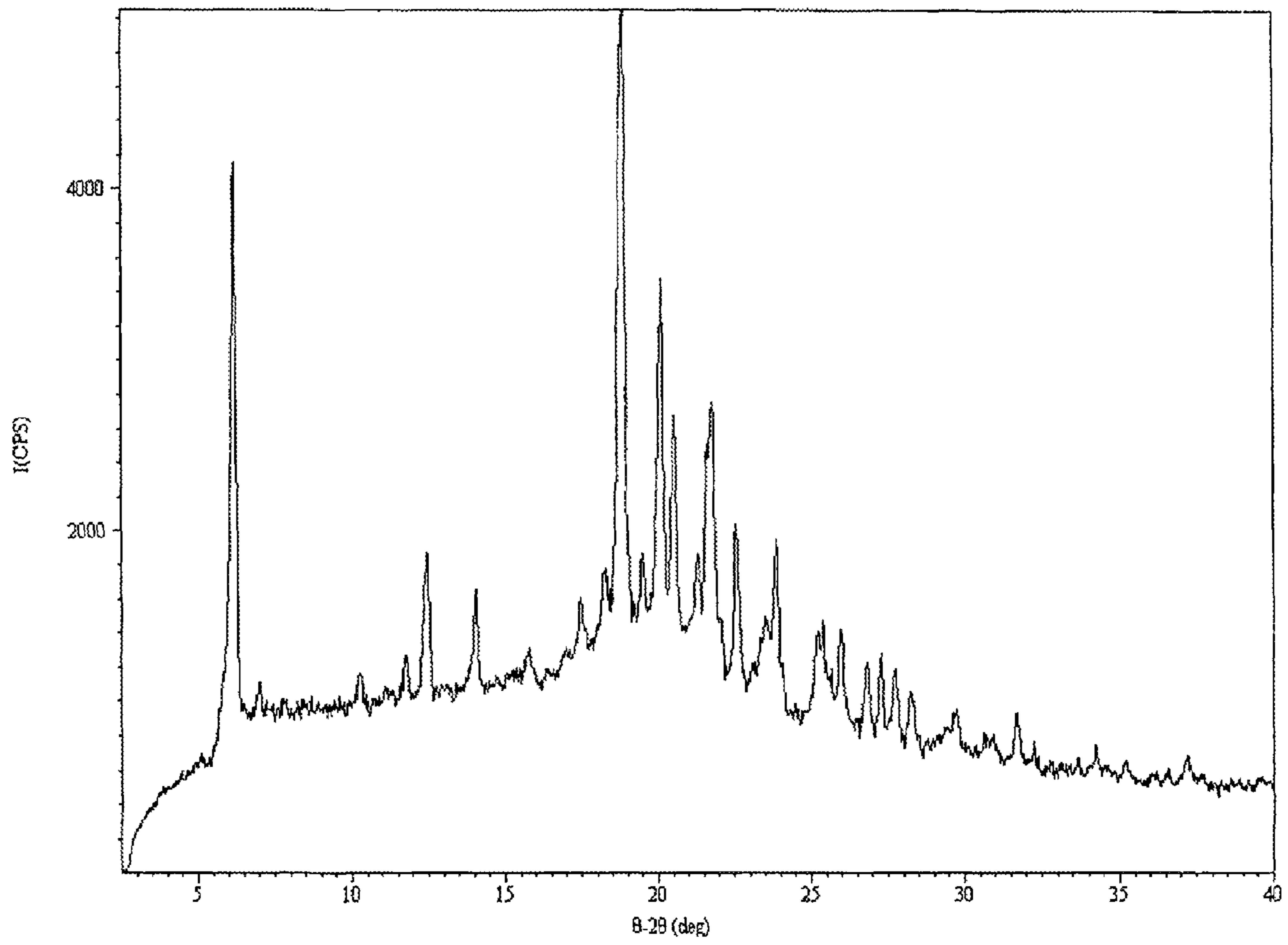
Figure 13 XRPD Pattern of Form B
