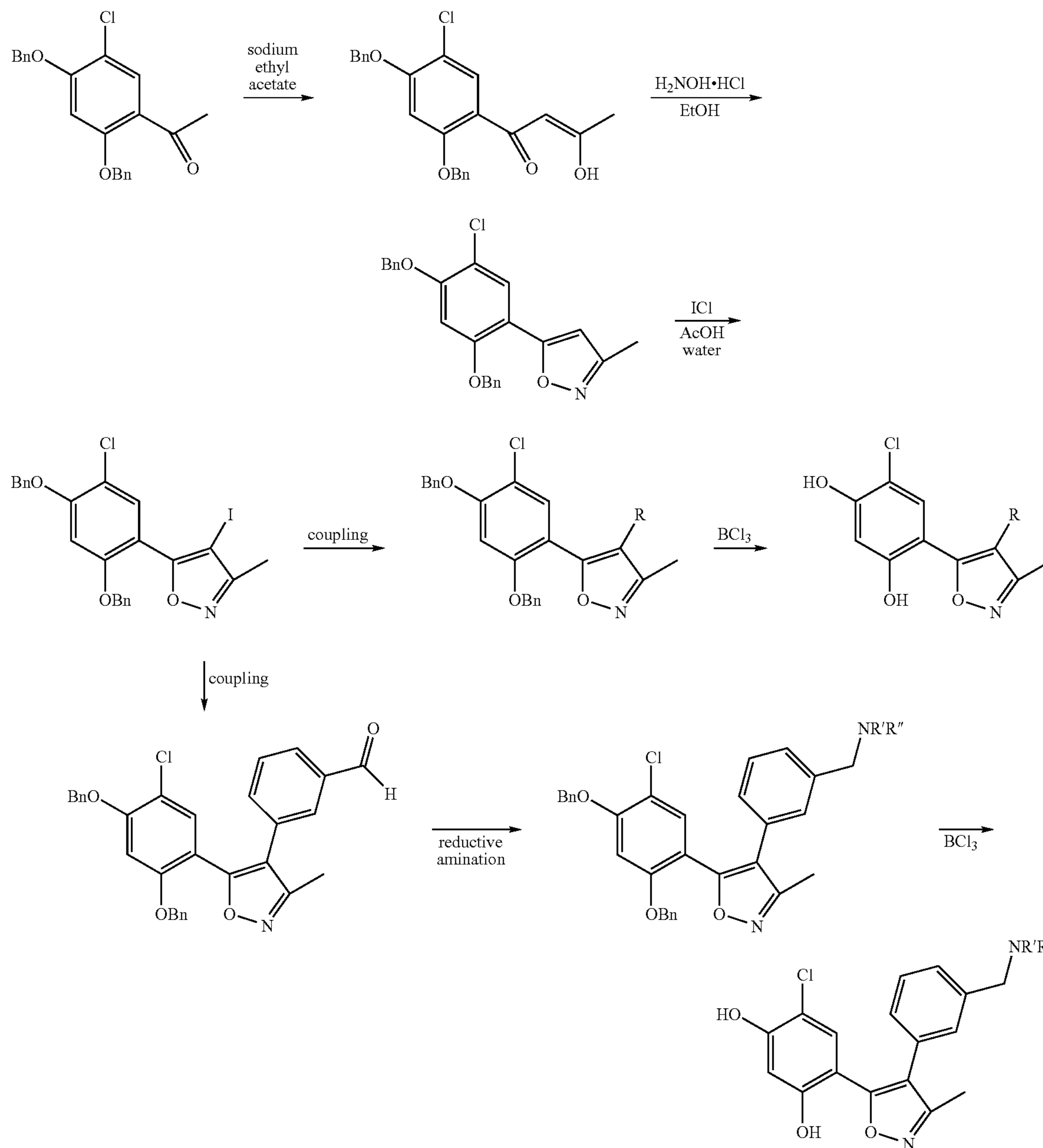
Scheme 7: Preparation of 5-(2,4-bis-benzyloxy-5-chloro-phenyl)-4-iodo-3-methyl-isoxazole intermediate
