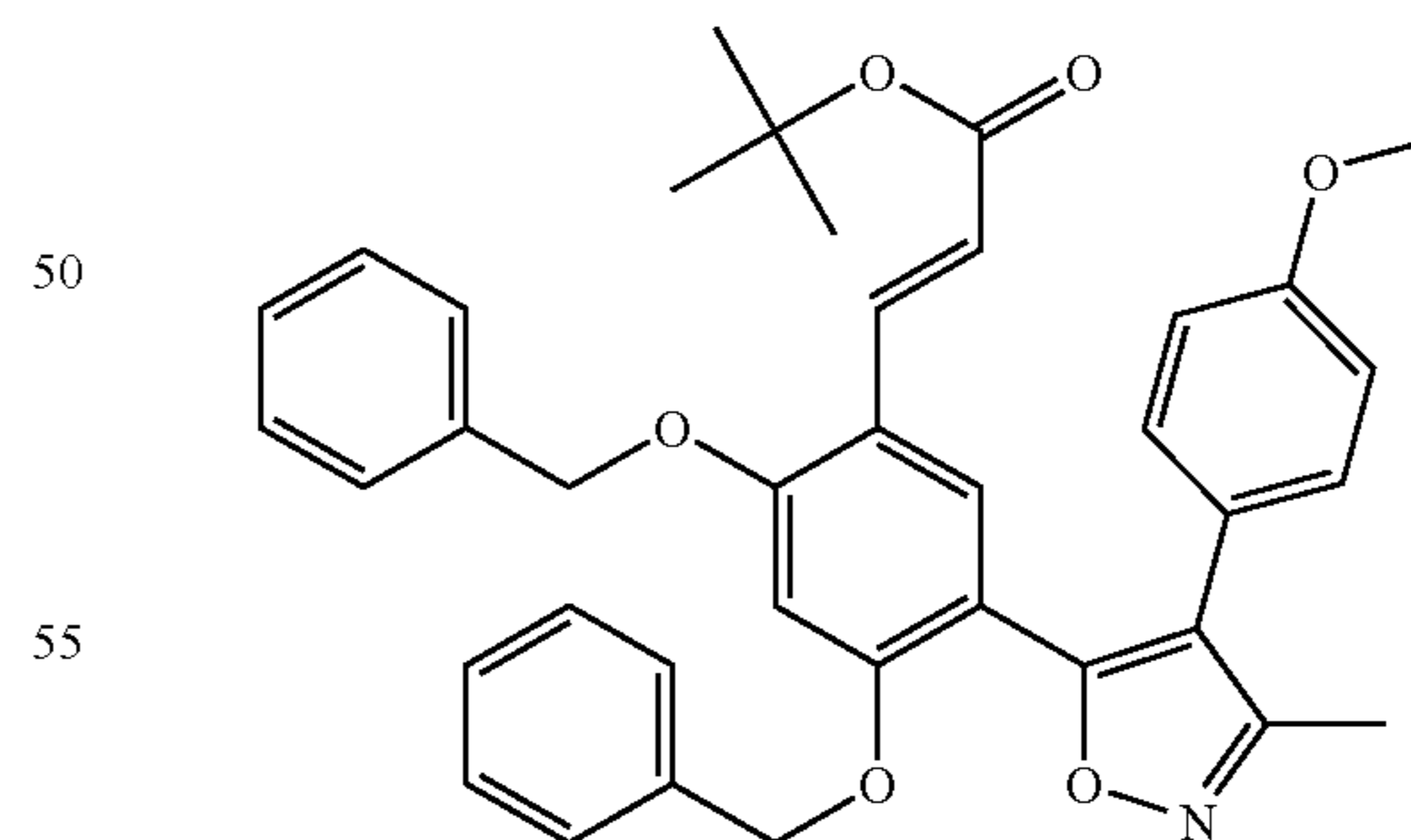
3-{2,4-Dihydroxy-5-[4-(4-methoxy-phenyl)-3-methyl-isoxazol-5-yl]-phenyl}-acrylic acid
