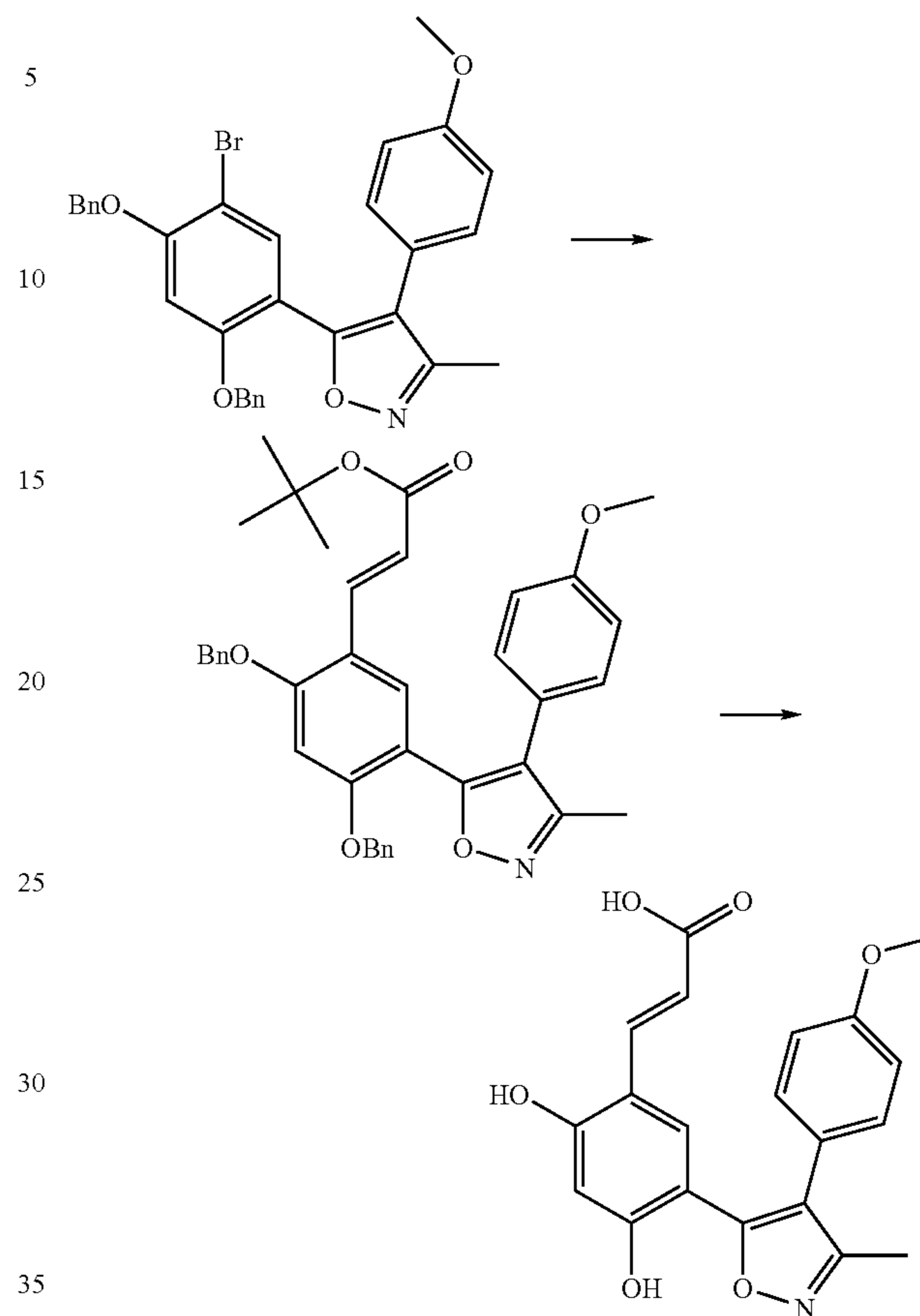
Scheme 5: Heck reaction and boron trichloride deprotection
