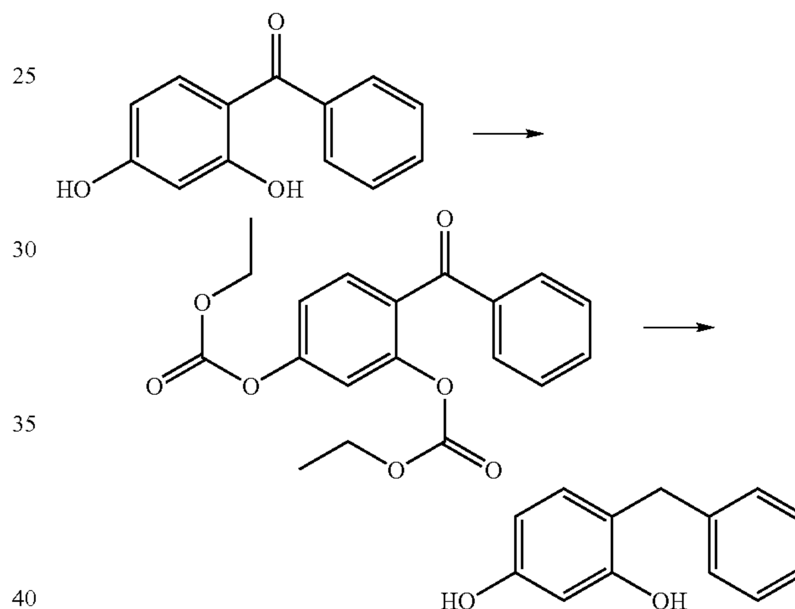
Scheme 4: Synthesis of benzyl resorcinol
