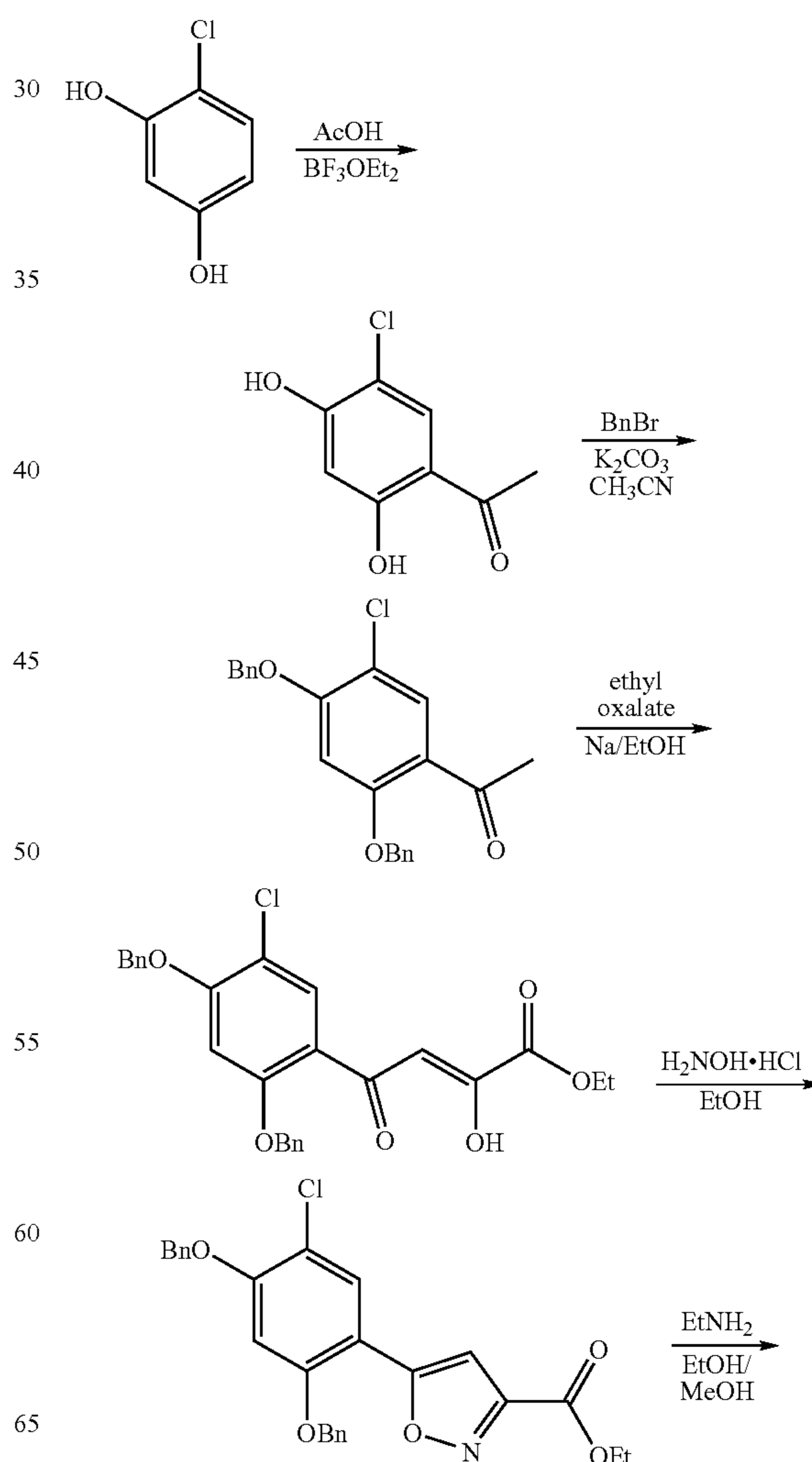
Scheme 6: Synthesis of 5-carboxamido isoxazoles
