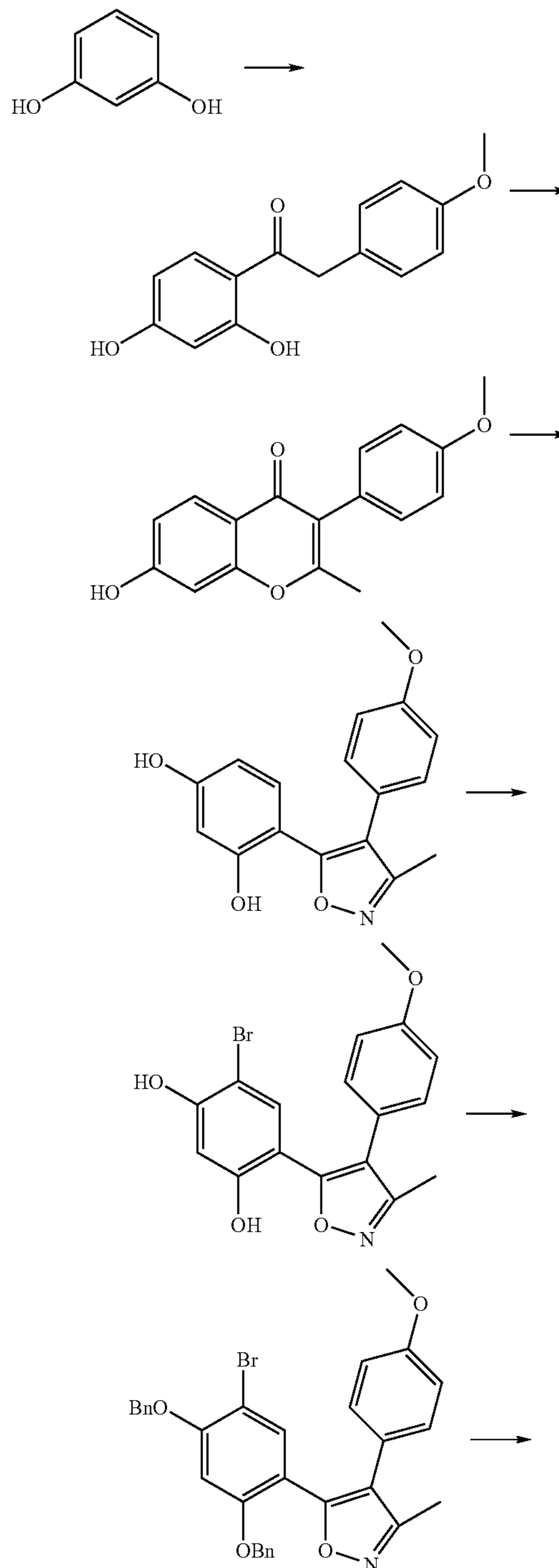
Scheme 1: preparation of bromo intermediate and subsequent arylation
