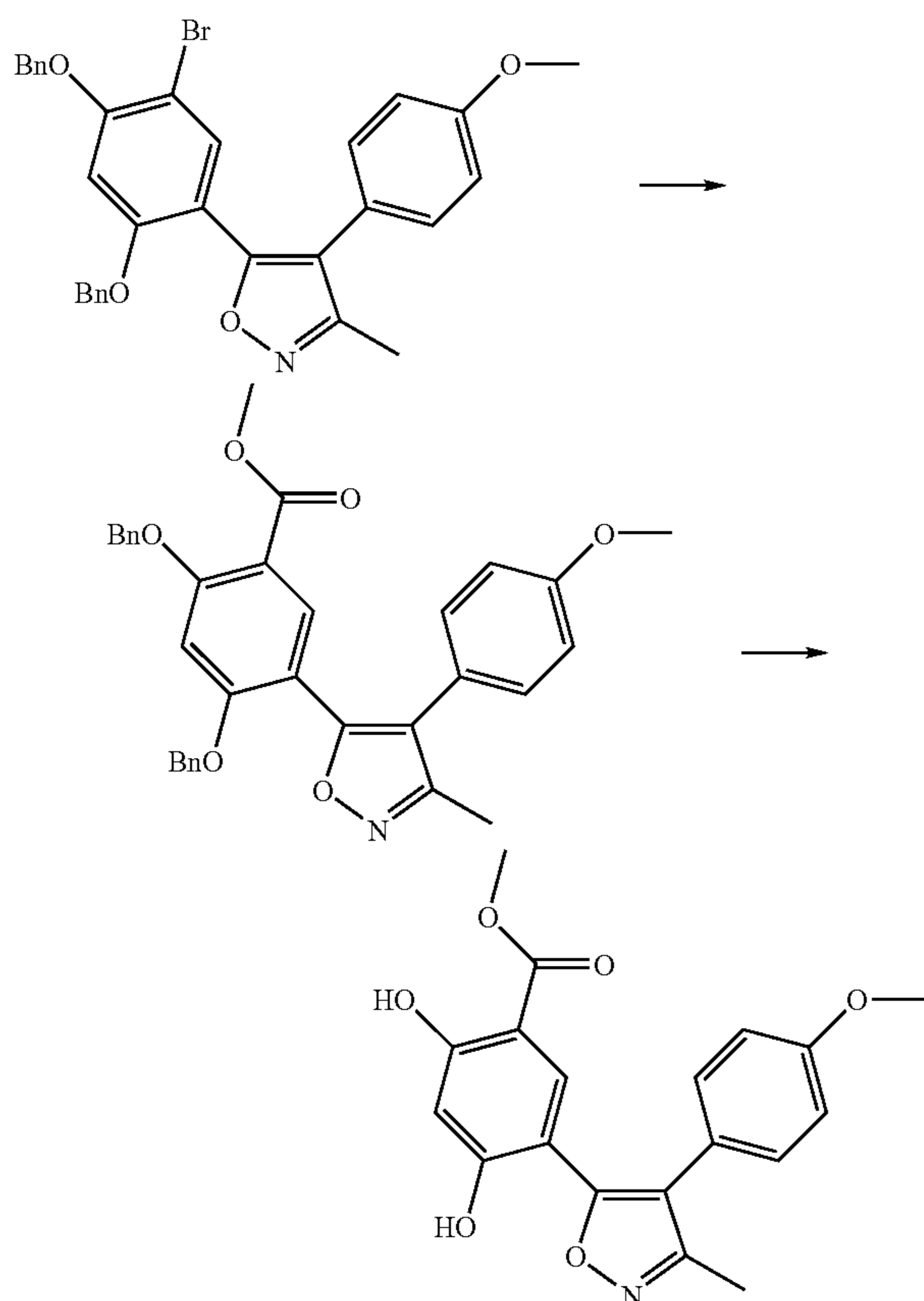
Scheme 3: formation of ester
