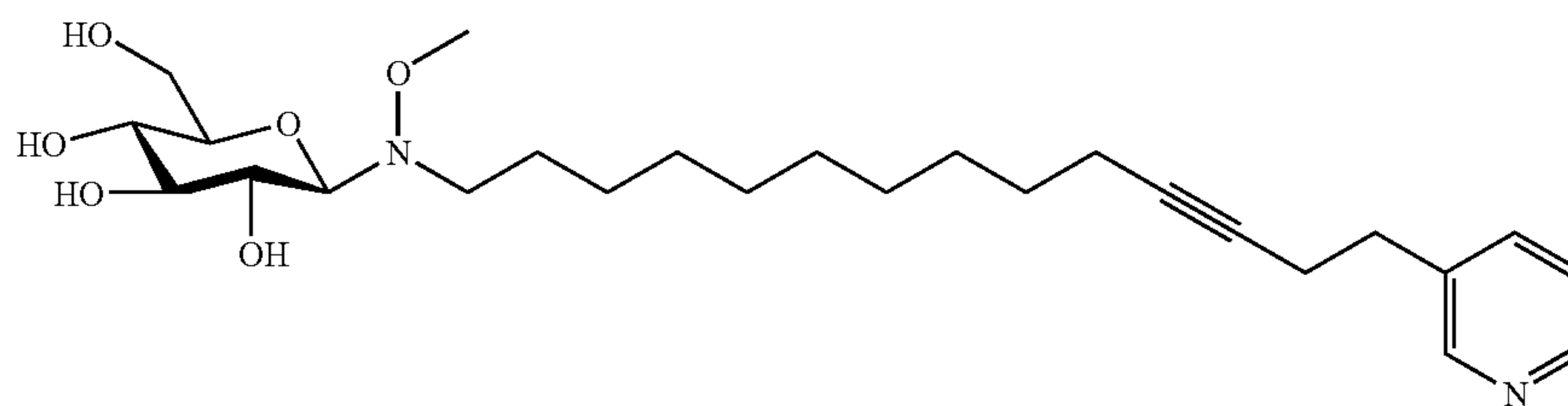
Amphlmedoside C
