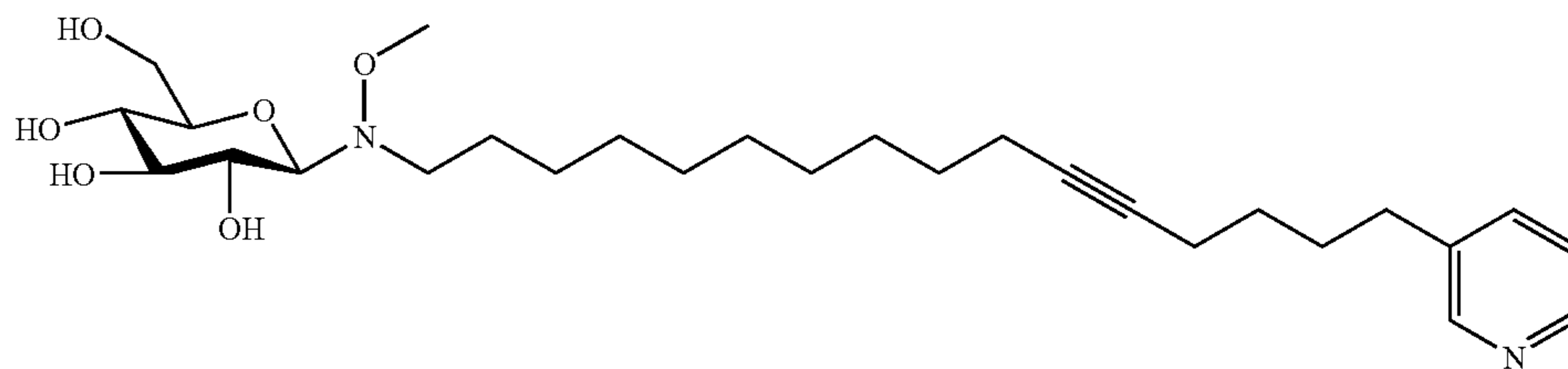
Amphlmedoside A
