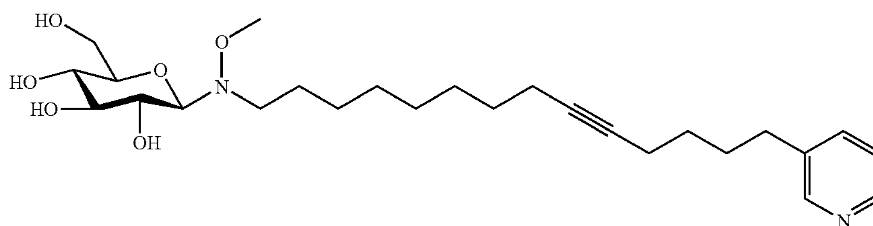
Amphlmedoside B
