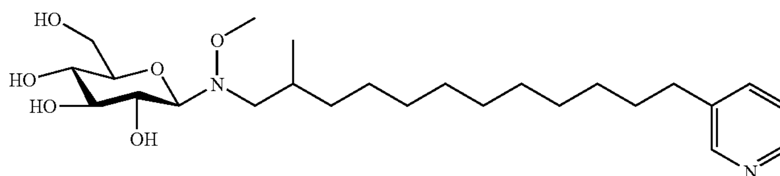
Amphlmedoside D
