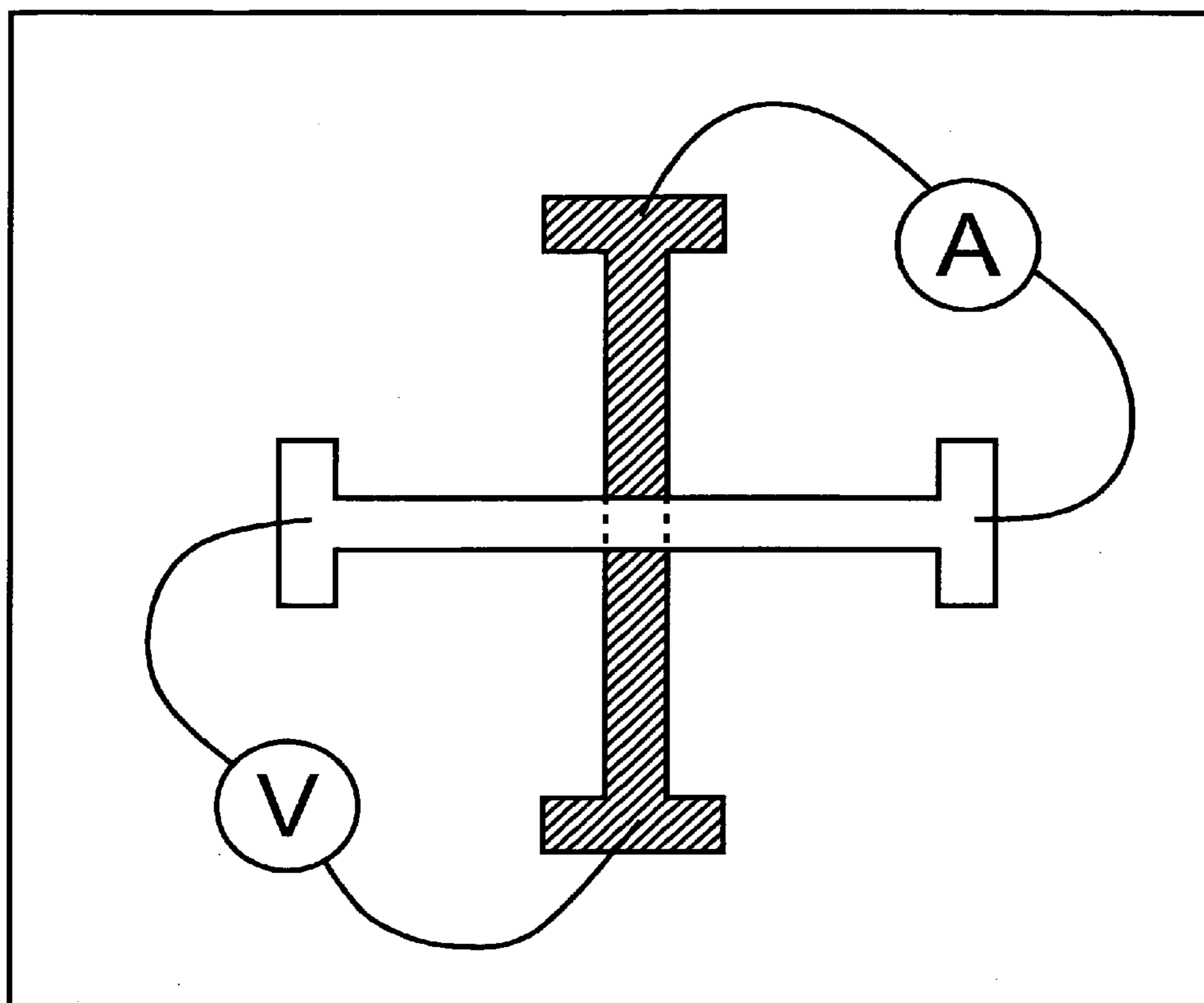
Wiring of a Kelvin pattern
