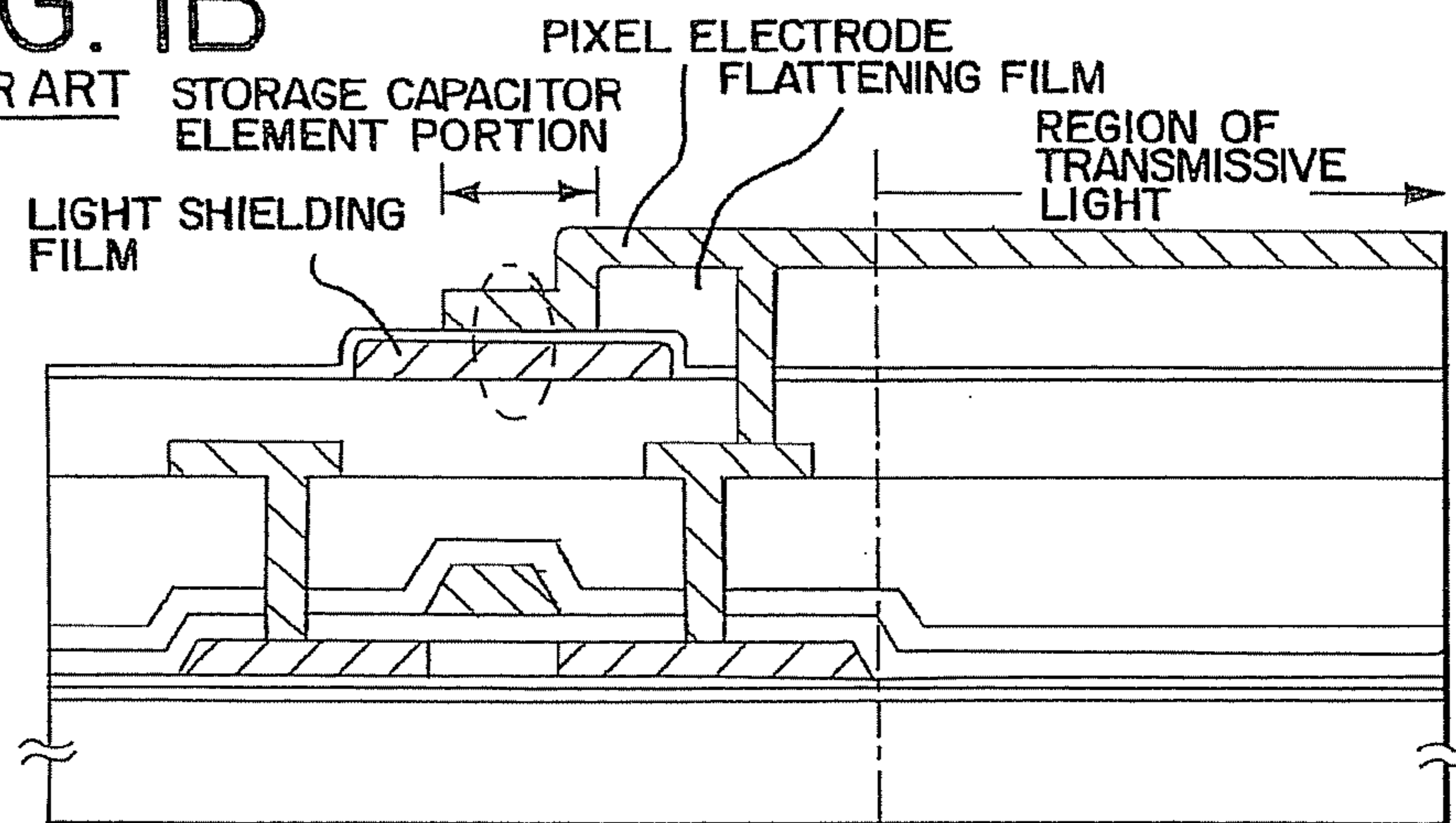
FIG. 1C PRIOR ART
