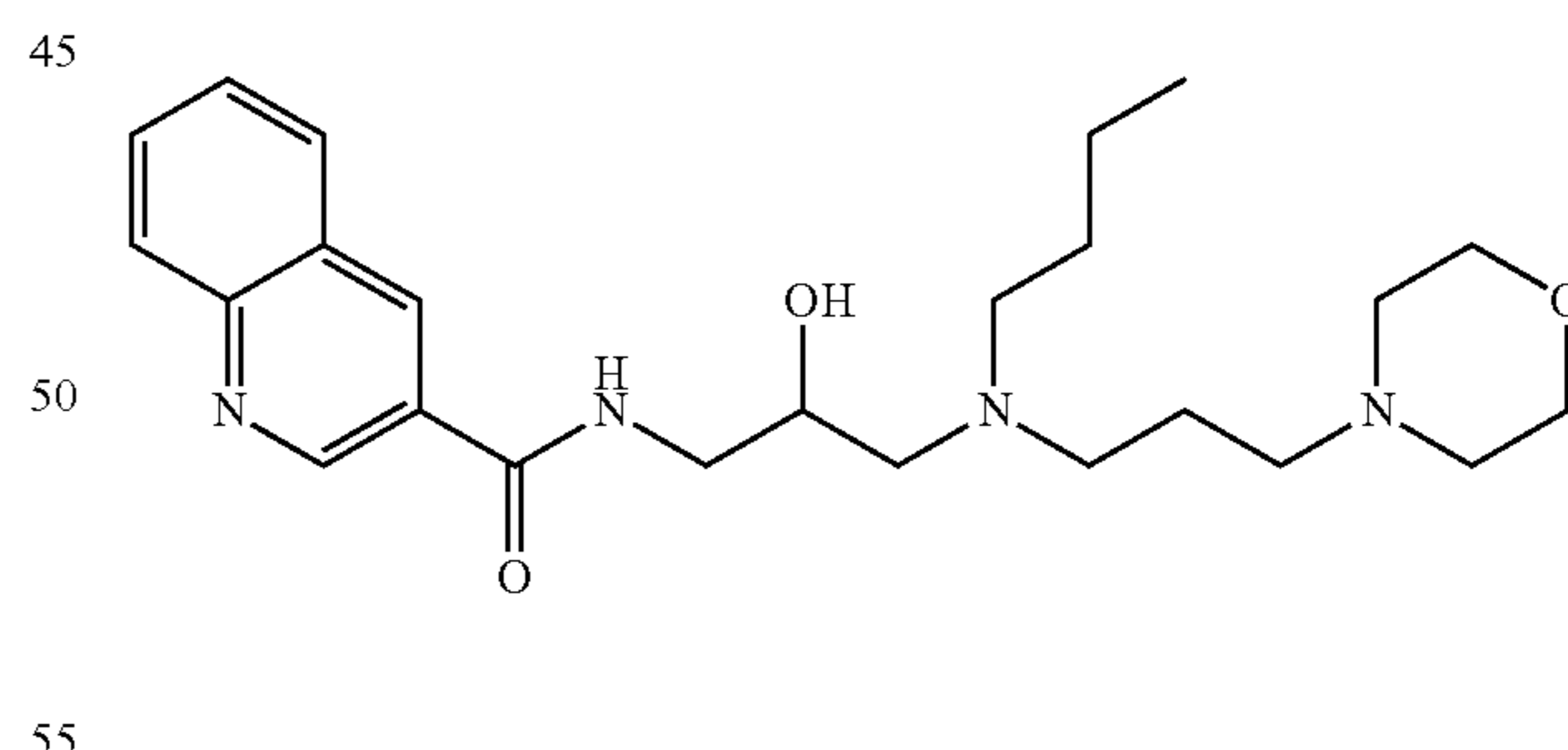
quinoline-3-carboxylic acid{3-[butyl-(3-morpholin-4-yl-propyl)-amino]-2-hydroxy-propyl}amide
