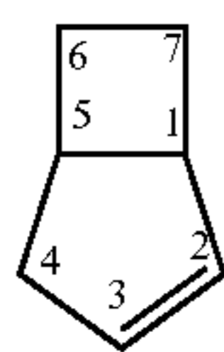
[3.2.0]
