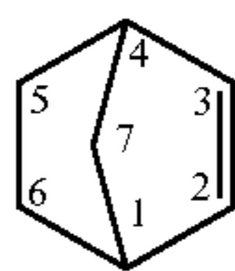
[2.2.1]
