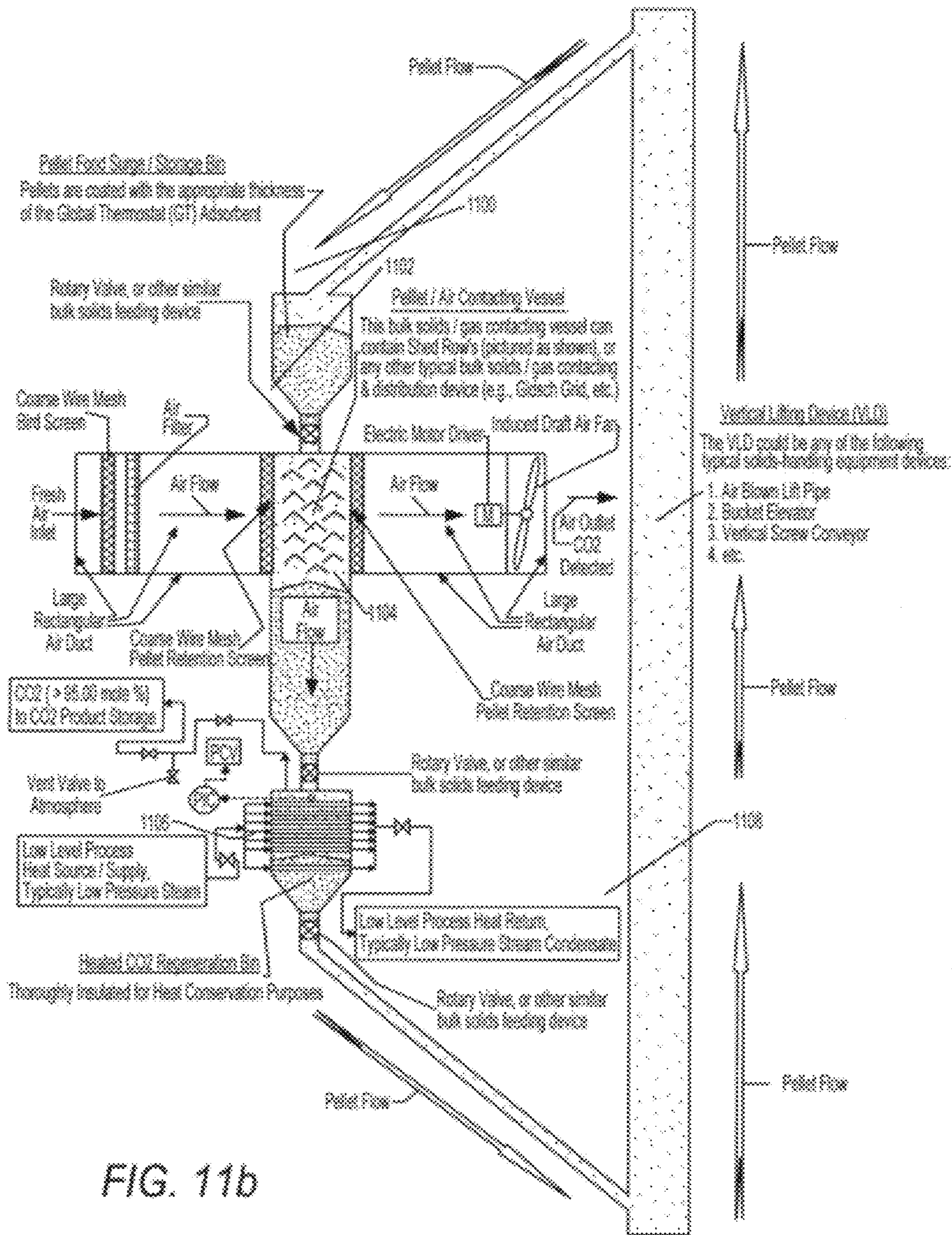
Global Thermostat (GT) Falling Pellet Contact / Cooling Exhaustary / Feed Pass / Overall Contact Drawing DRAWING 8.3 - EP - Falling Pellet Contact / Cooling, with Cross-Current Pellet / Air Flow
