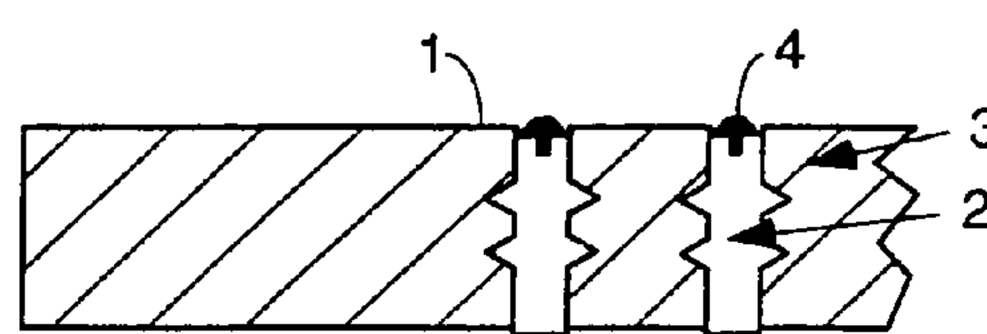
SOLDER BALL MOUNT FIG. 8B
