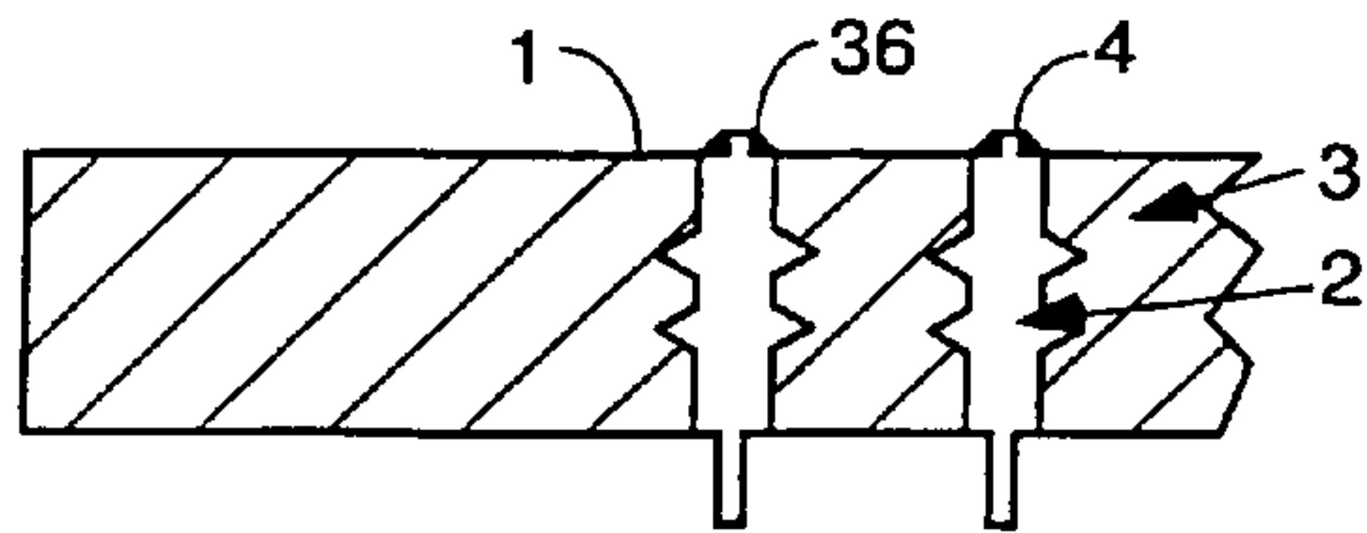
THROUGH HOLE FIG. 5A
