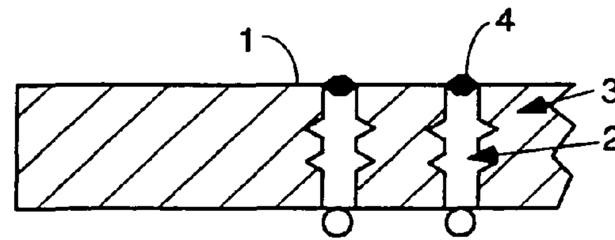
THROUGH HOLE FIG. 11A
