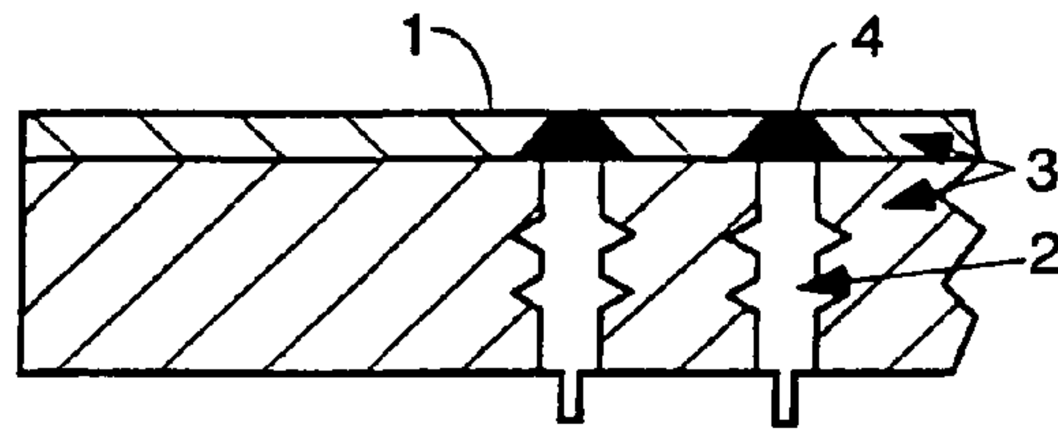
THROUGH HOLE FIG. 10A
