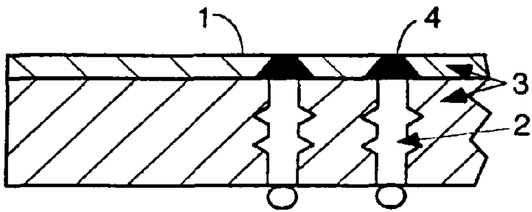
SOLDER BALL MOUNT FIG. 10B
