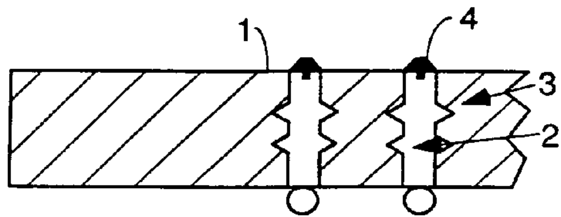
SOLDER BALL MOUNT FIG. 7B
