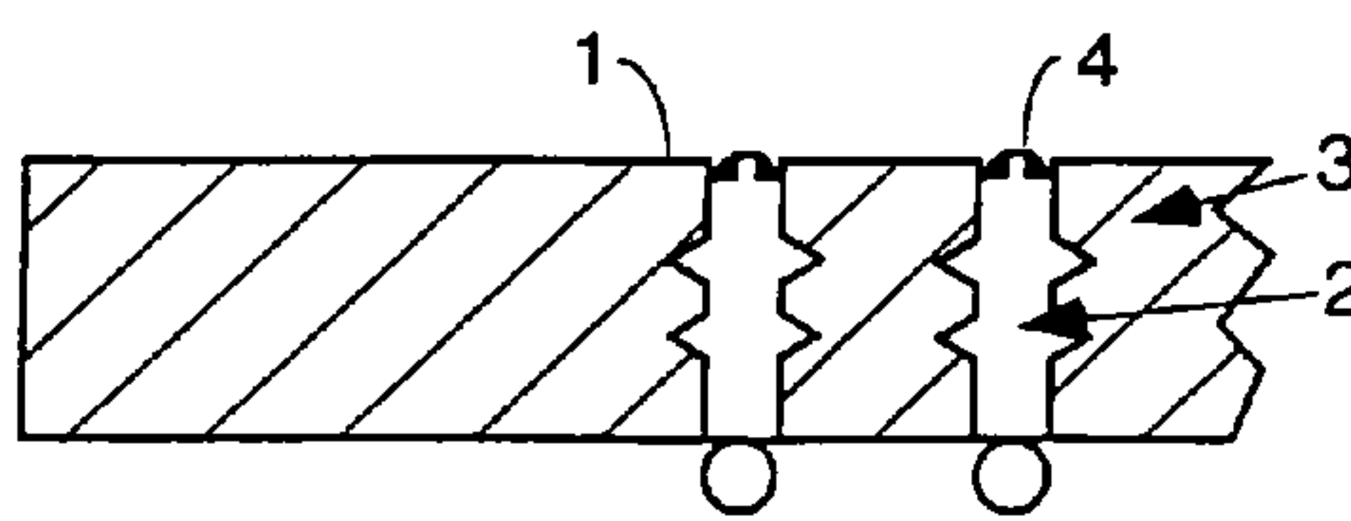
SOLDER BALL MOUNT FIG. 6B
