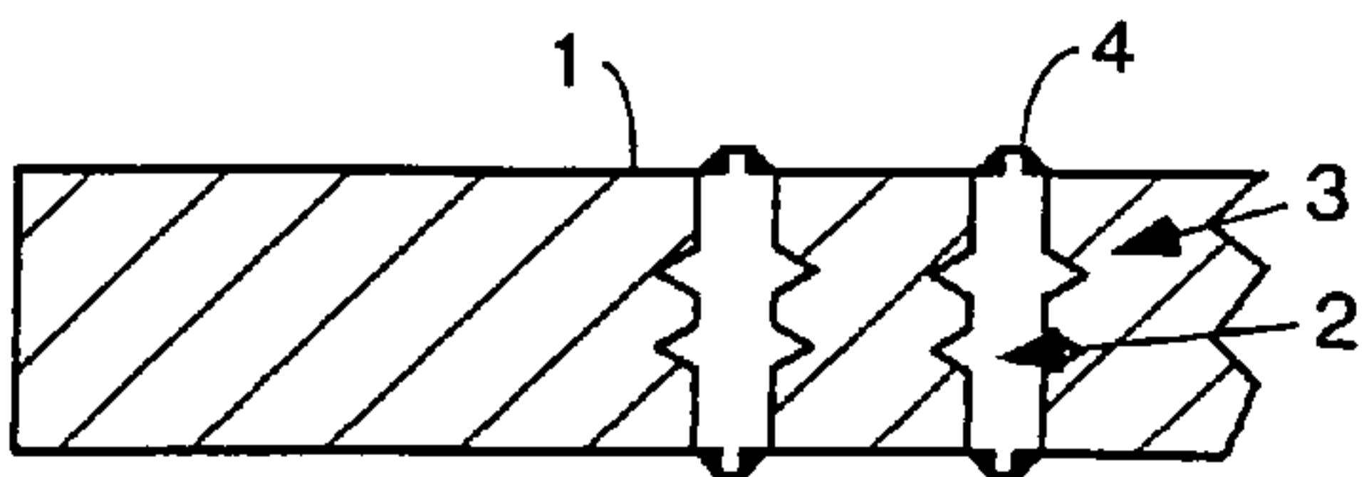
COMPRESSION MOUNT FIG. 5D
