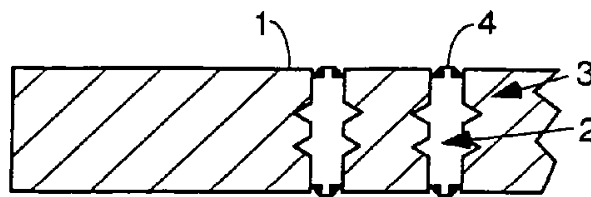
COMPRESSION MOUNT FIG. 6D
