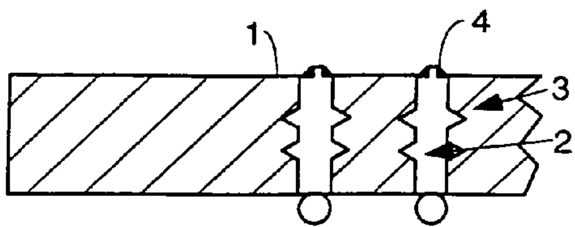
SOLDER BALL MOUNT FIG. 5B
