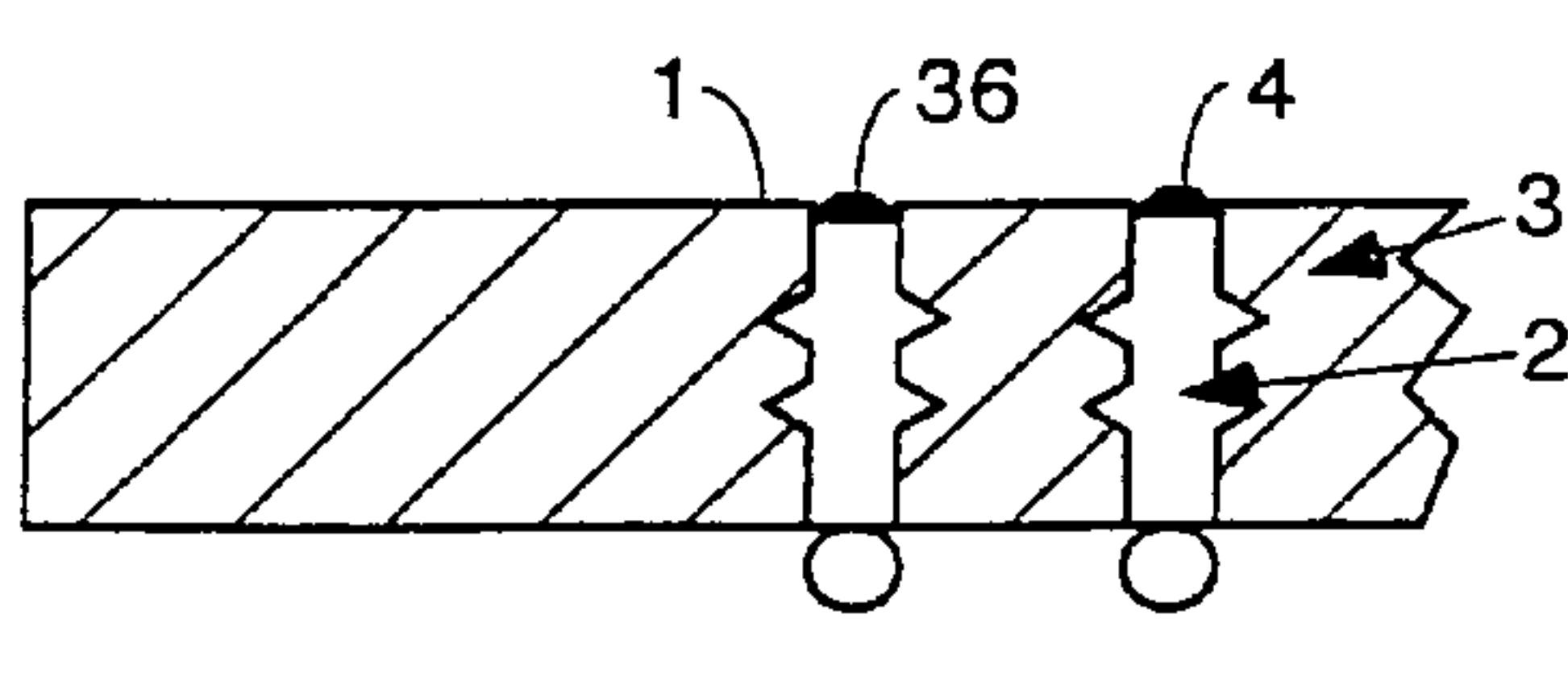
SOLDER BALL MOUNT FIG. 4B
