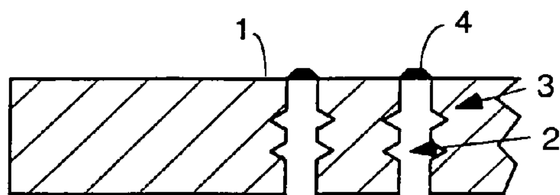
SOLDER BALL MOUNT FIG. 3B
