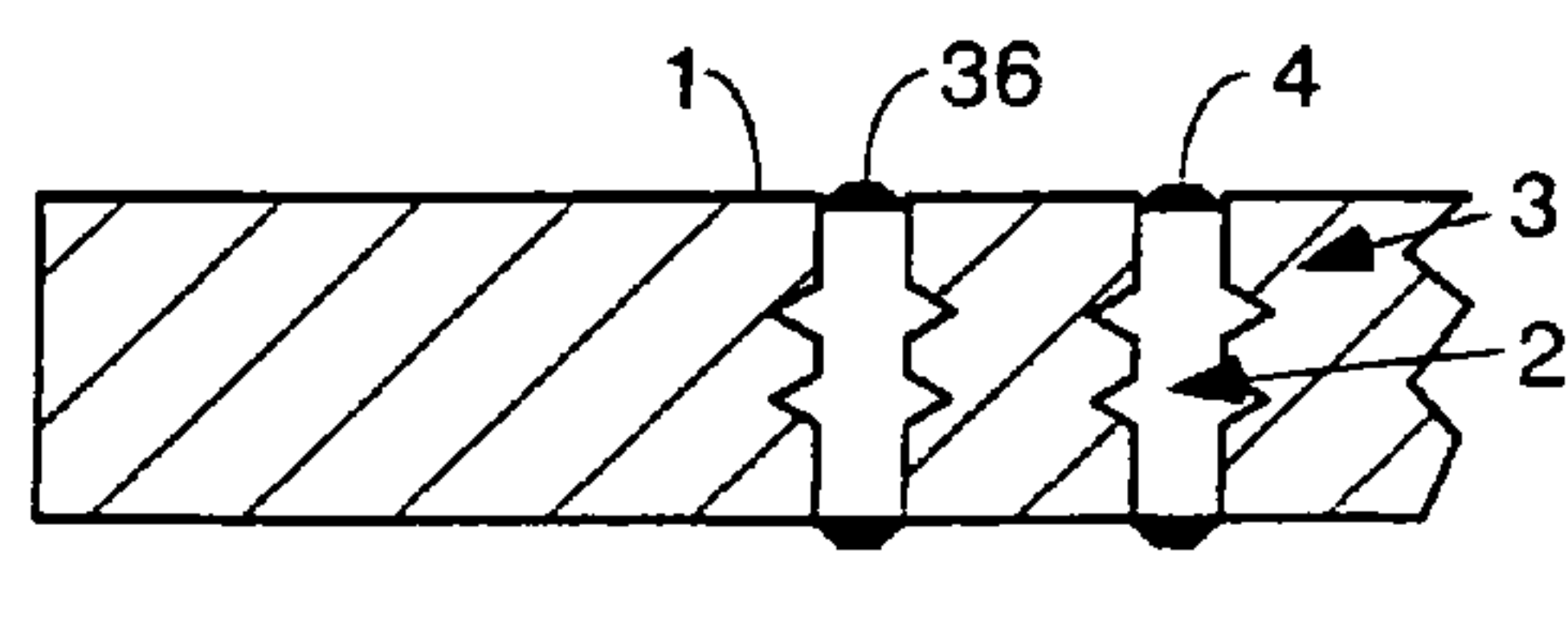
COMPRESSION MOUNT FIG. 4D
