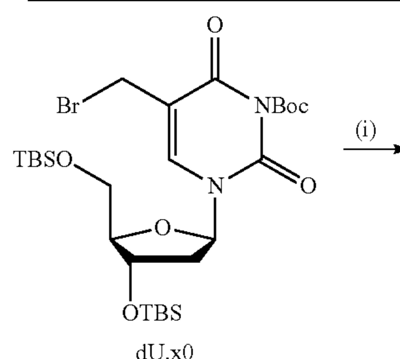
Scheme 17. Synthesis of 6-TAMRA labeled 5-[(R or S)-1-[4-(3-amino-1-propynyl)-2-nitrophenyl]-2,2-dimethyl-propoxy]methyl-2'-deoxycytidine-5'-triphosphate.
