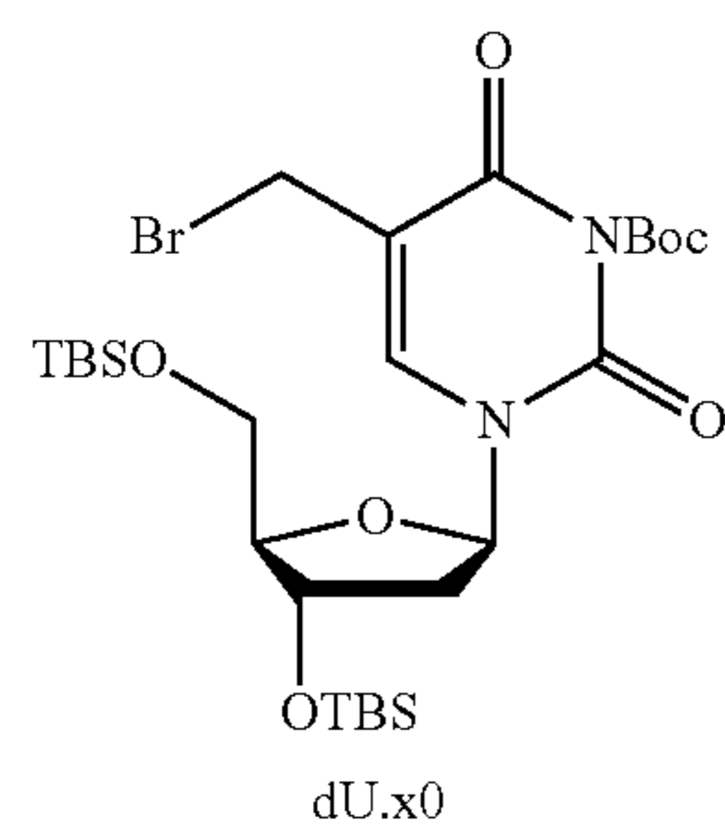
Scheme 11. Synthesis of 5-[(S)-1-(2-nitrophenyl)-2-methyl-propyloxy]methyl-2'-deoxycytidine-5'-triphosphate.
