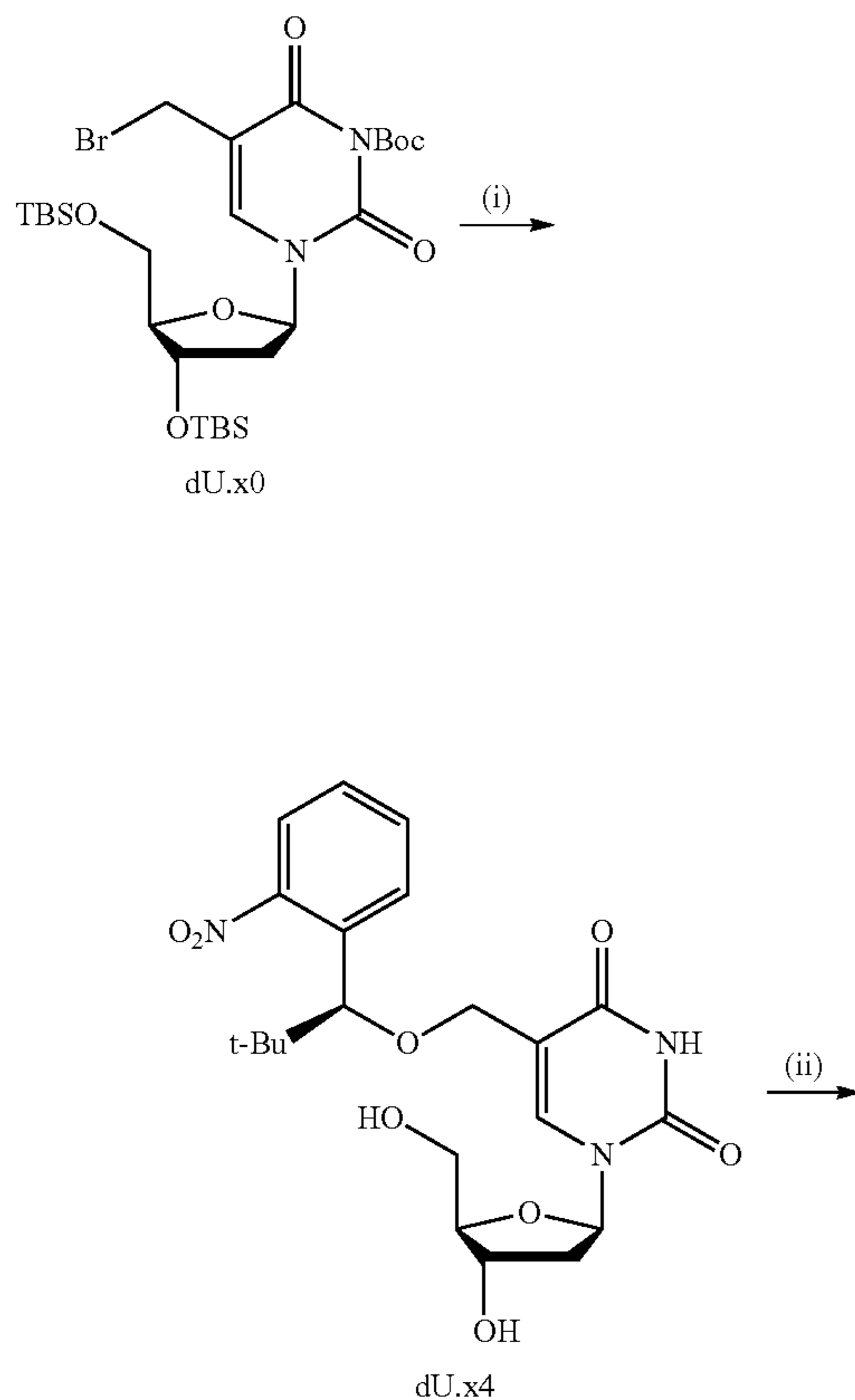
Scheme 12. Synthesis of 5-[(R or S)-1-(2-nitrophenyl)-2,2-dimethyl-1-propyloxy]methyl-2'-deoxyuridine-5'-triphosphate.
