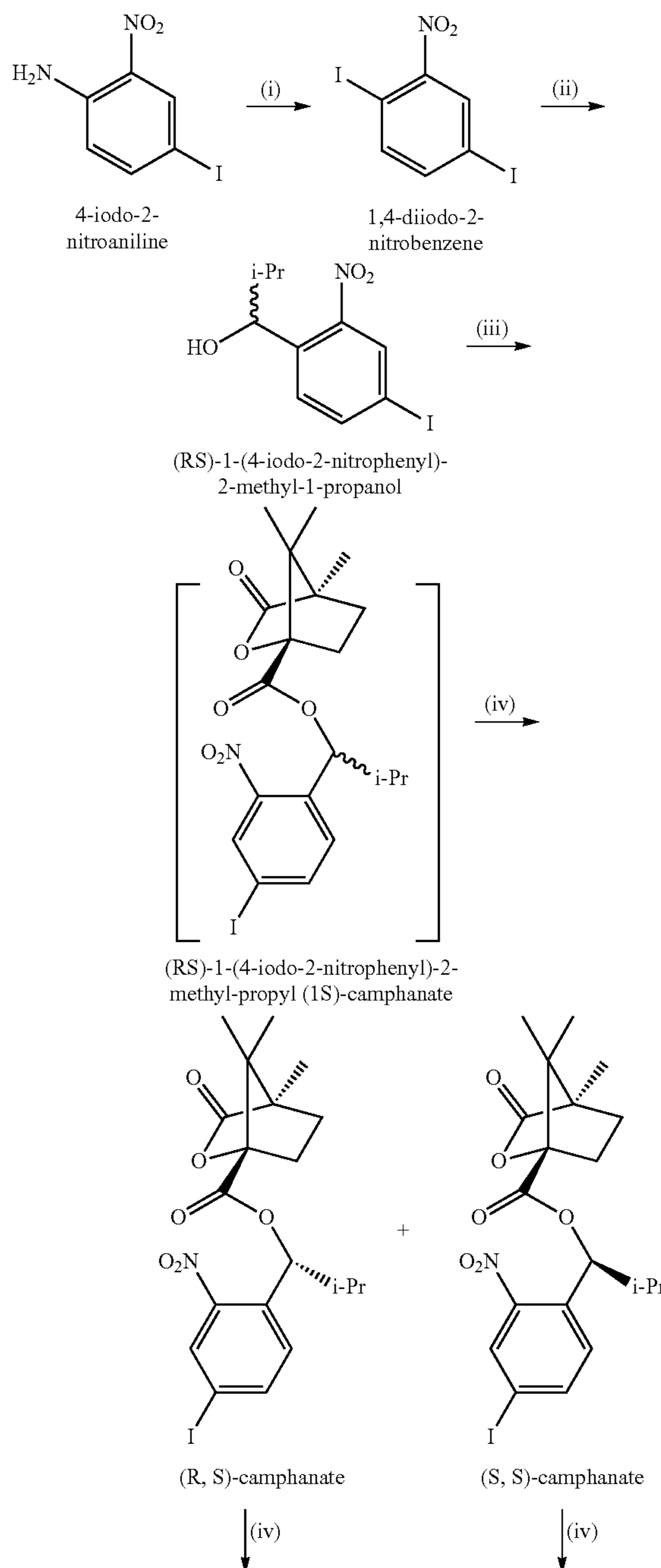
Scheme 4. Synthesis of (RS)-1-(4-Iodo-2-nitrophenyl)-2-methyl-1-propanol, (R)-1-(4-Iodo-2-nitrophenyl)-2-methyl-1-propanol and (S)-1-(4-Iodo-2-nitrophenyl)-2-methyl-1-propanol.
