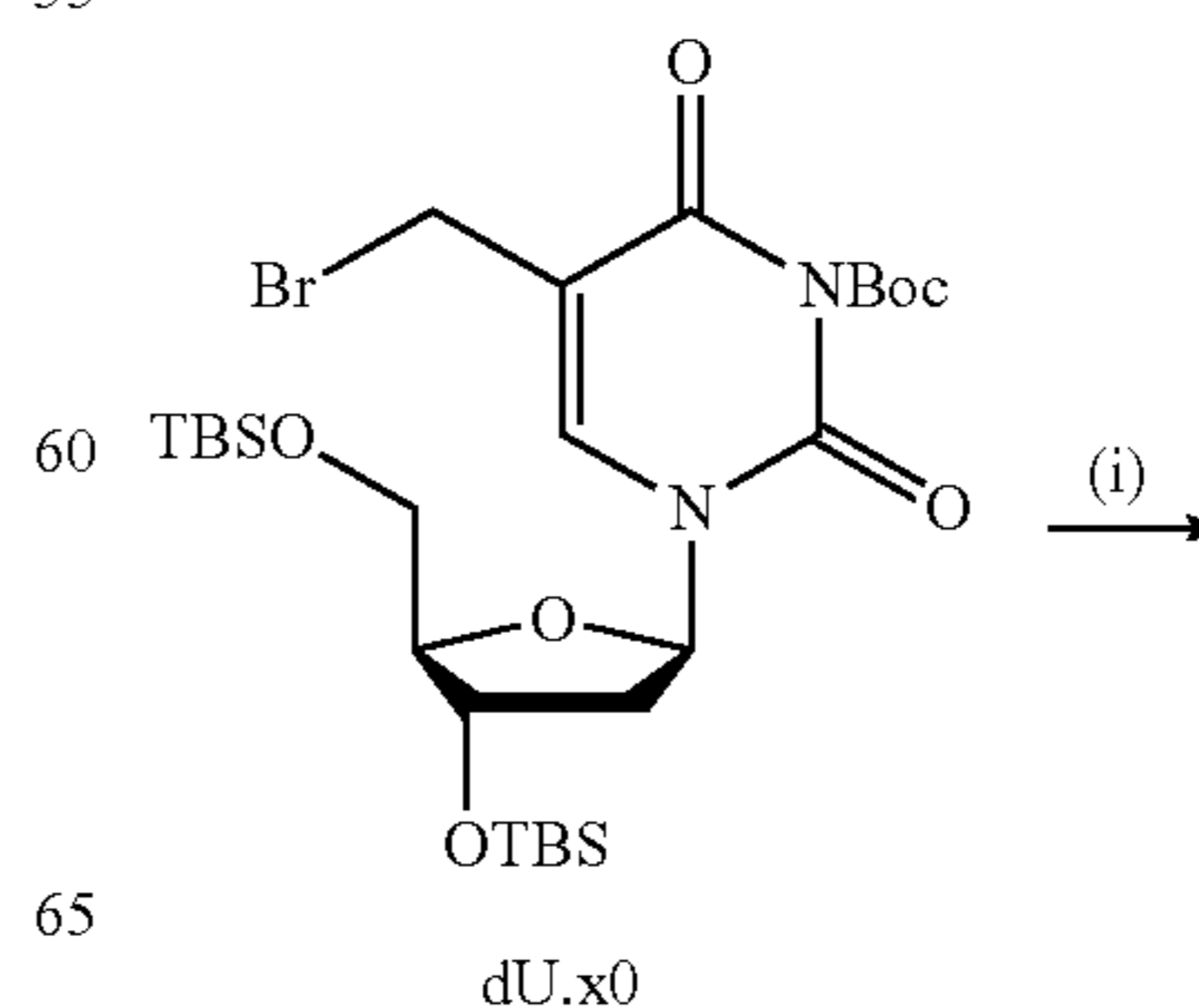
Scheme 31. Synthesis of 5-(1-phenyl-2-methyl-propyloxy)methyl-2'-deoxyuridine-5'-triphosphate.
