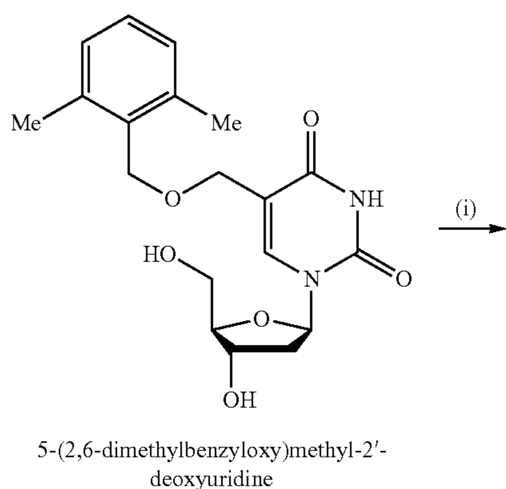
Scheme 41. Chemical cleavage of 5-(2,6-dimethylbenzyloxy)methyl-2'-deoxyuridine
