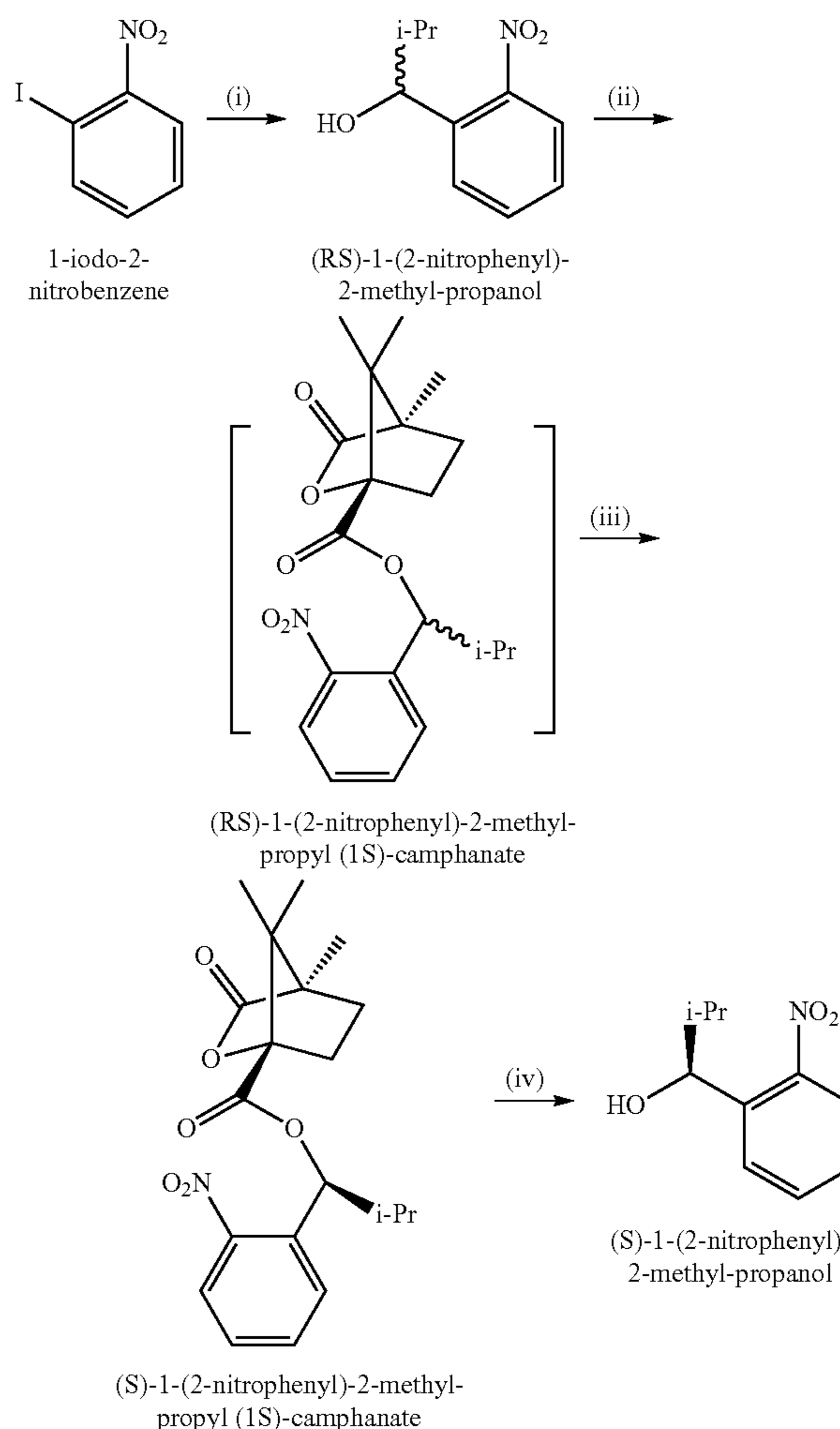
Scheme 3. Synthesis of (RS)-1-(2-nitrophenyl)-2-methyl-1-propanol and (S)-1-(2-nitrophenyl)-2-methyl-1-propanol.
