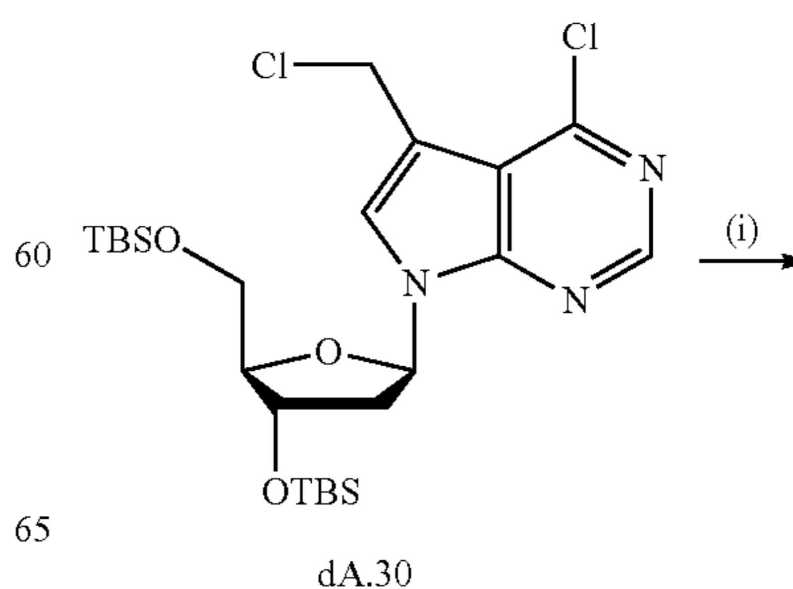
Scheme 26. Synthesis of 6-FAM labeled 7- \{(R)\text{-}1\text{-}[4\text{-}(3\text{-amino-1-propynyl)-2-nitrophenyl]-2-methyl-propyloxy}\} methyl-7-deaza-2'-deoxyadenosine-5'-triphosphate
