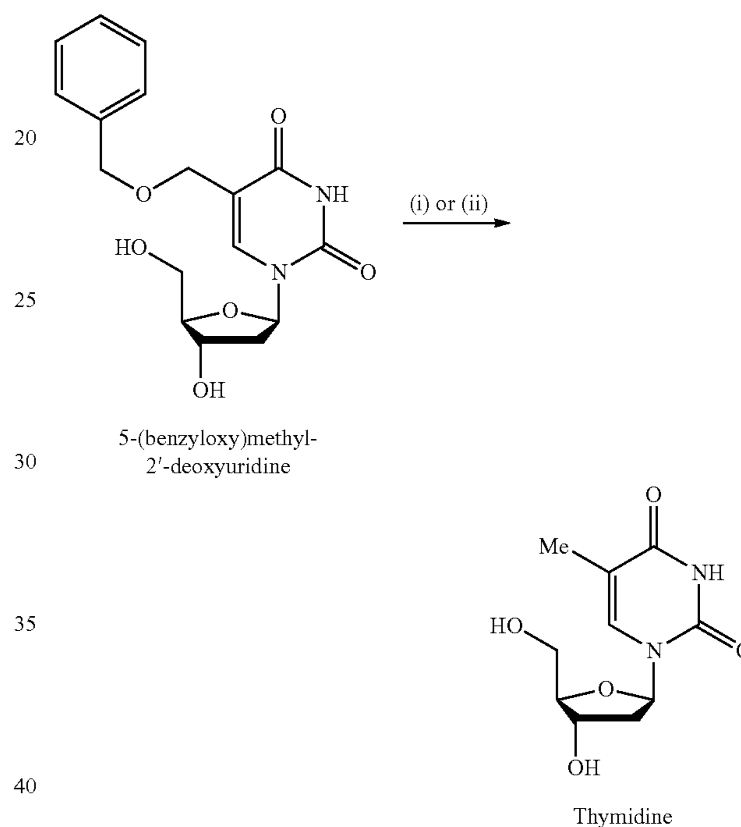
Scheme 38. Chemical cleavage of 5-(benzyloxy)methyl-2'-deoxyuridine.
