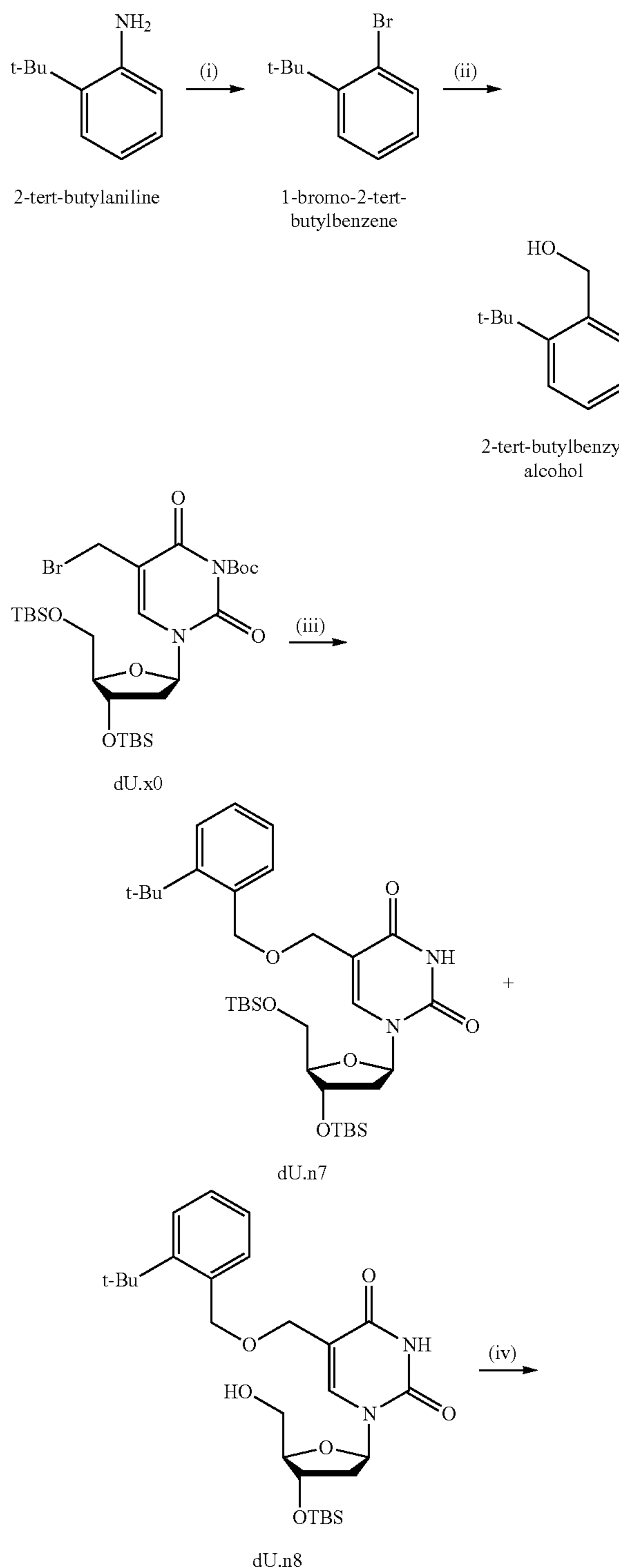
Scheme 34. Synthesis of 5-(2-tert-butylbenzyloxy)methyl-2'-deoxyuridine-5'-triphosphate.
