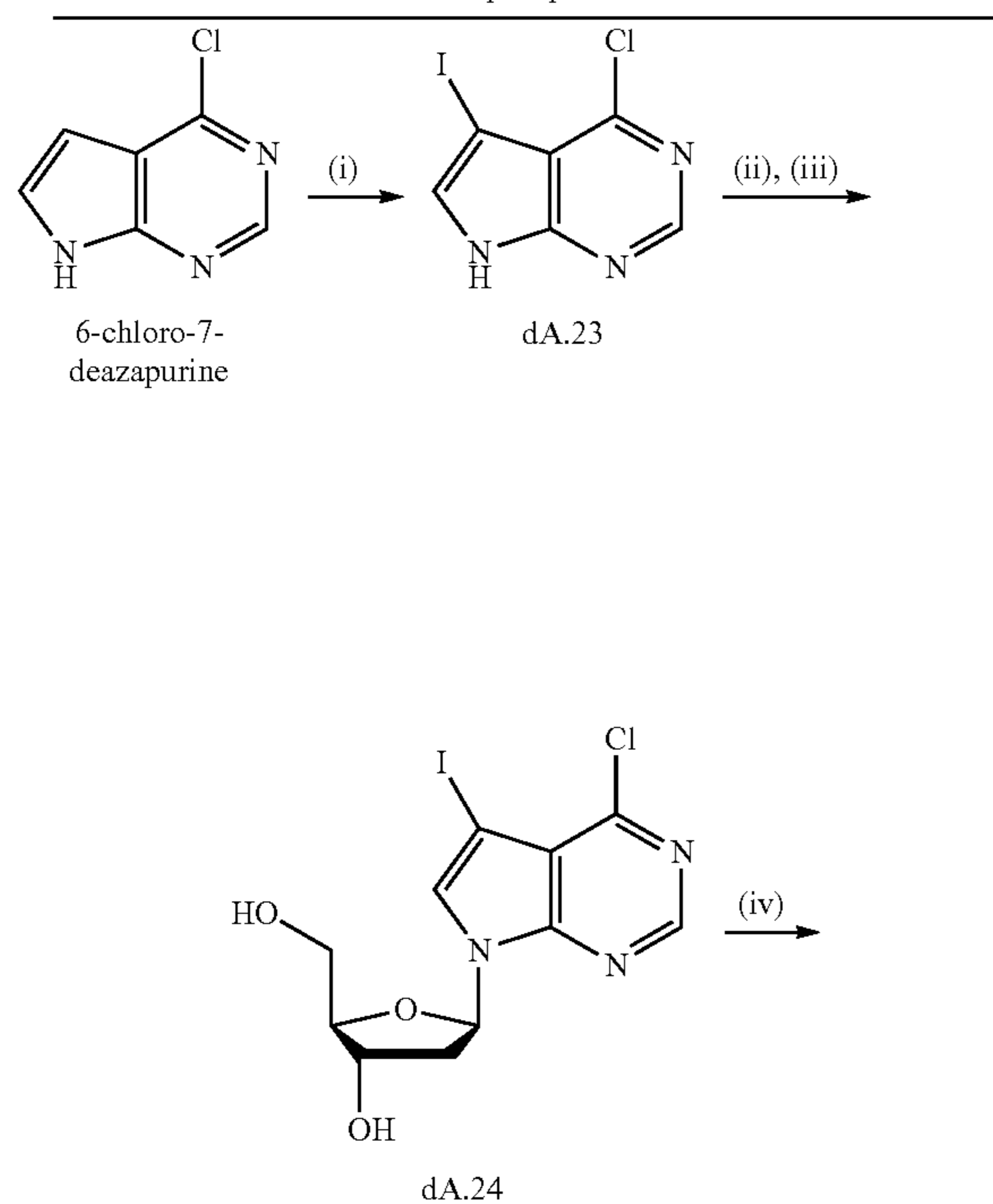
Scheme 24. Synthesis of 7-(2-nitrobenzyloxy)methyl-7-deaza-2'-deoxyadenosine-5'-triphosphate.
