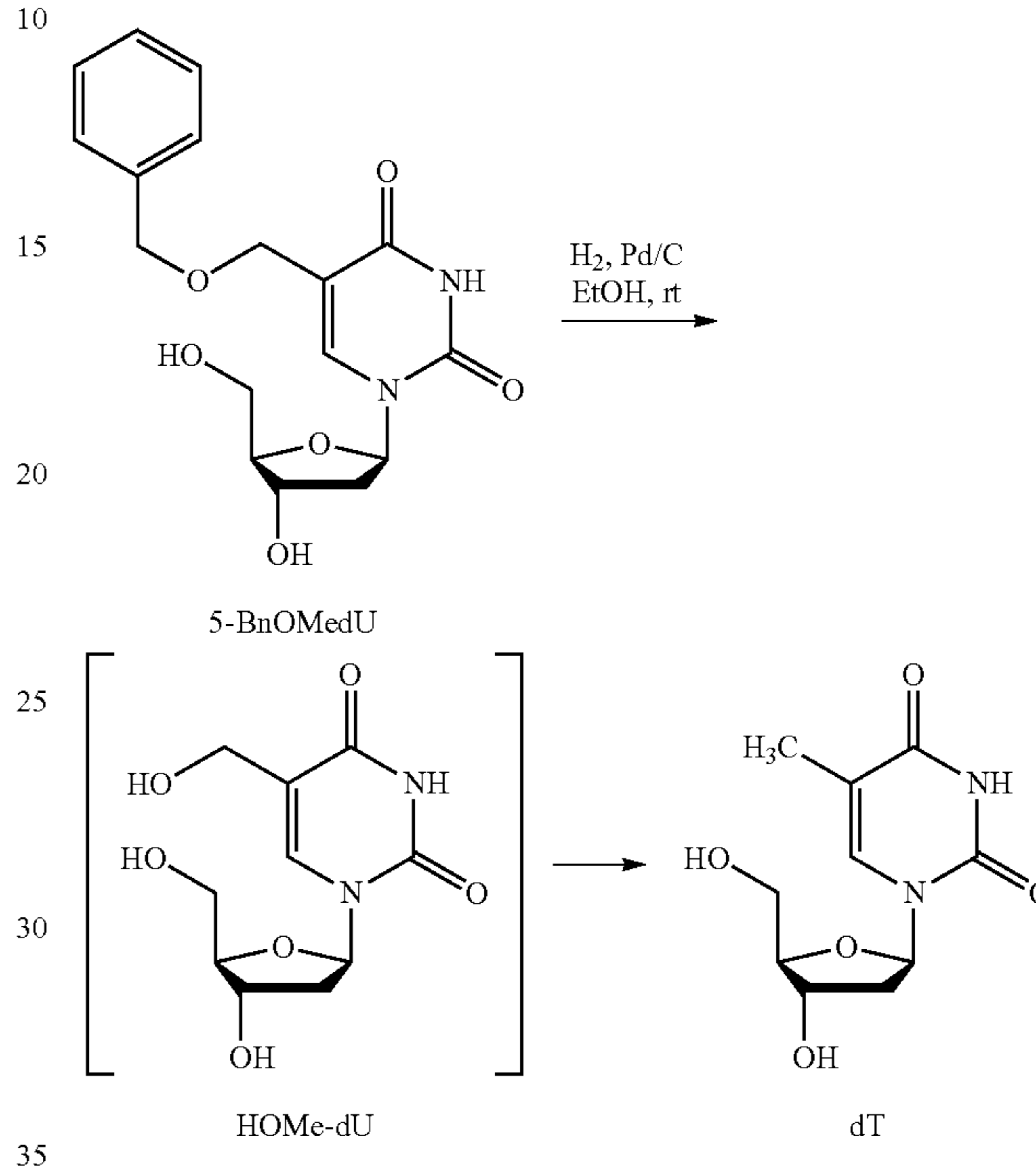
Scheme 42. Catalytic hydrogenolysis of 5-benzyloxymethyl-2'-deoxyuridine
