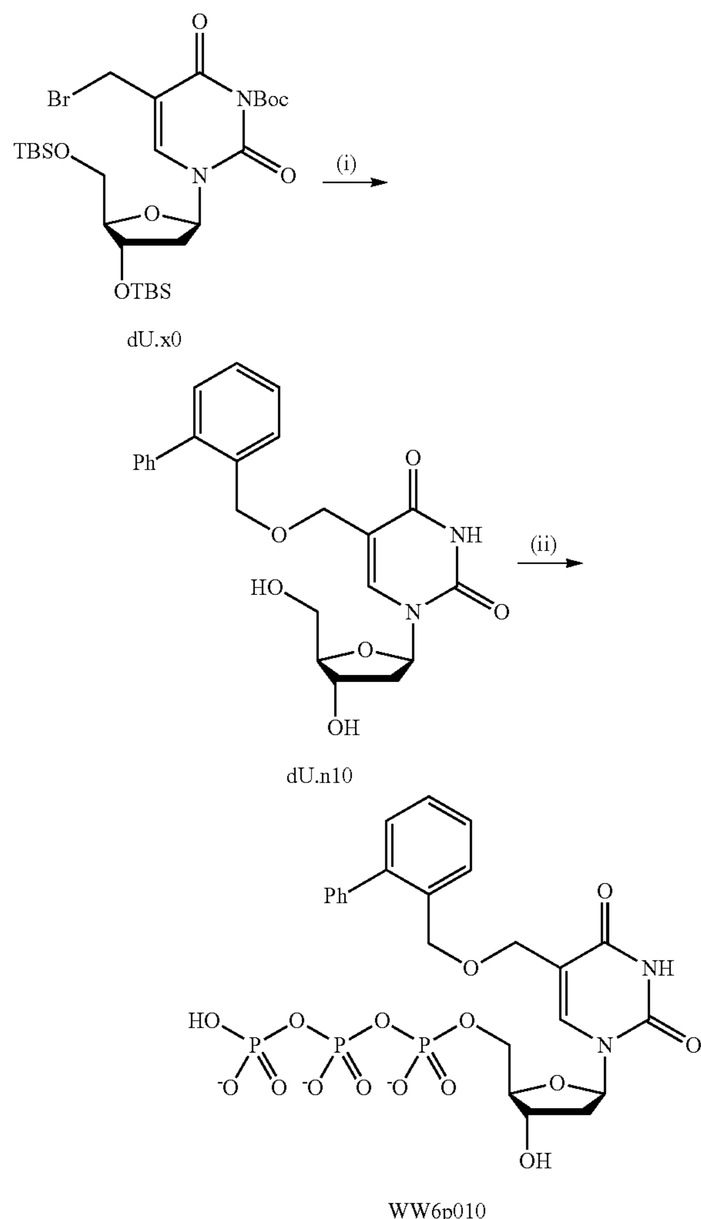
Scheme 35. Synthesis of 5-(2-phenylbenzyloxy)methyl-2'-deoxyuridine-5'-triphosphate
