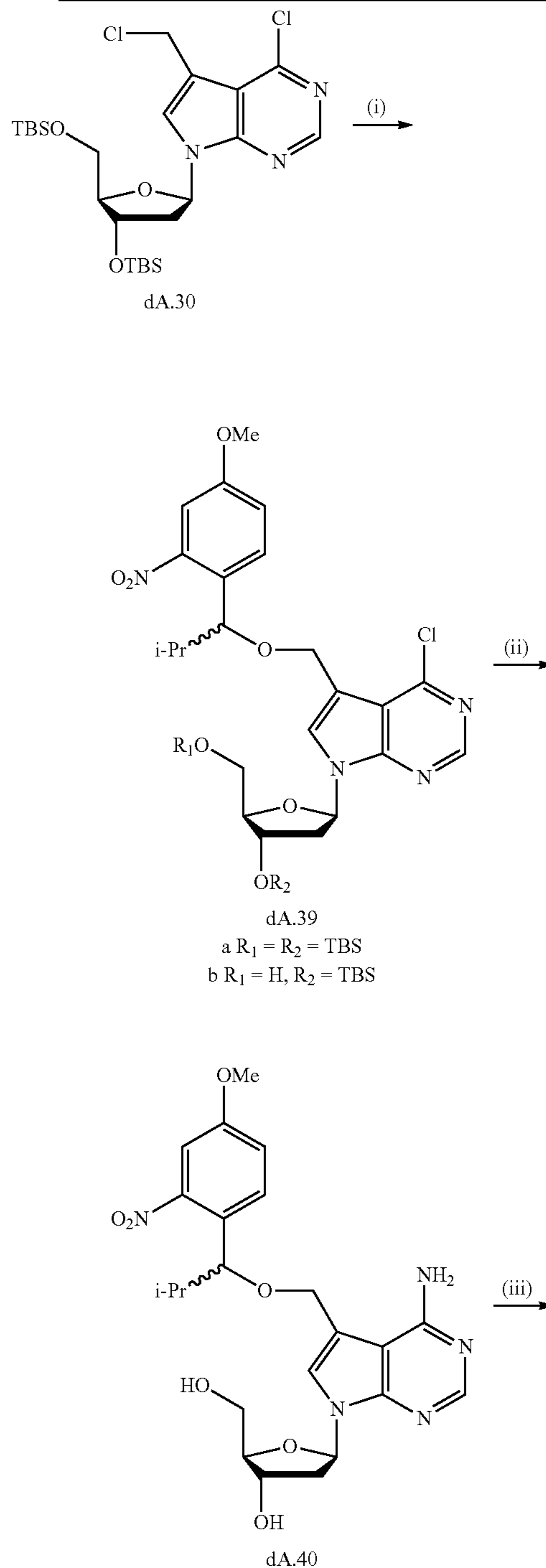
Scheme 29. Synthesis of 7-[1-(4-methoxy-2-nitrophenyl)-2-methyl-propyloxy]methyl-7-deaza-2'-deoxyadenosine-5'-triphosphate.
