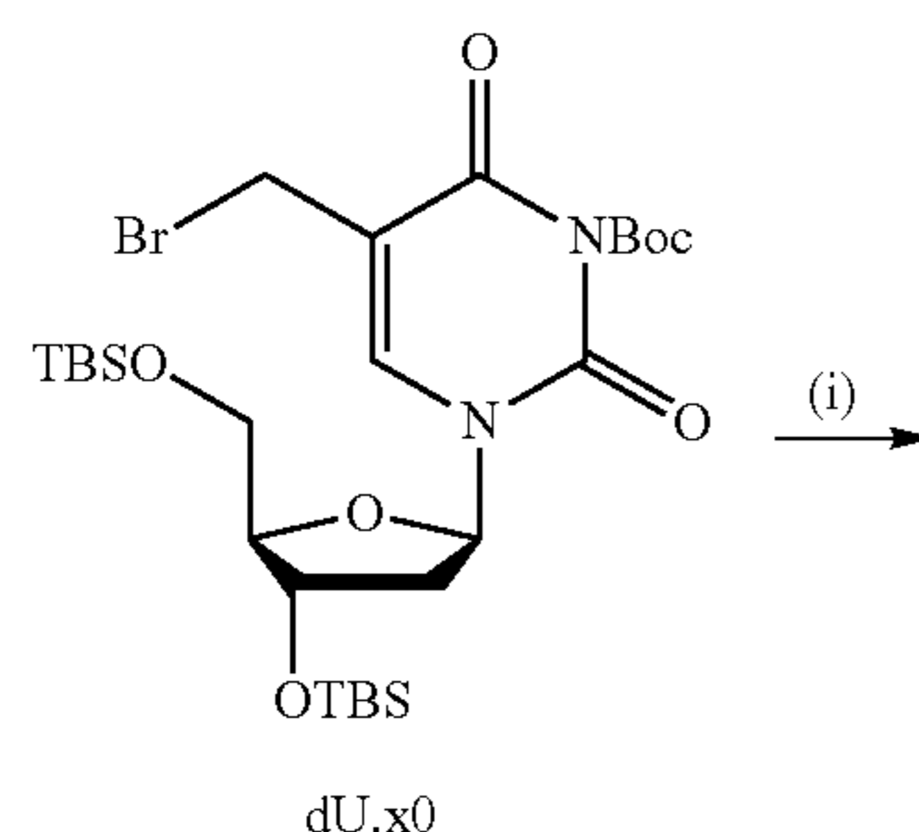
Scheme 37. Synthesis of 5-(3-phenyl-2-propenyloxy)methyl-2'-deoxyuridine-5'-triphosphate.
