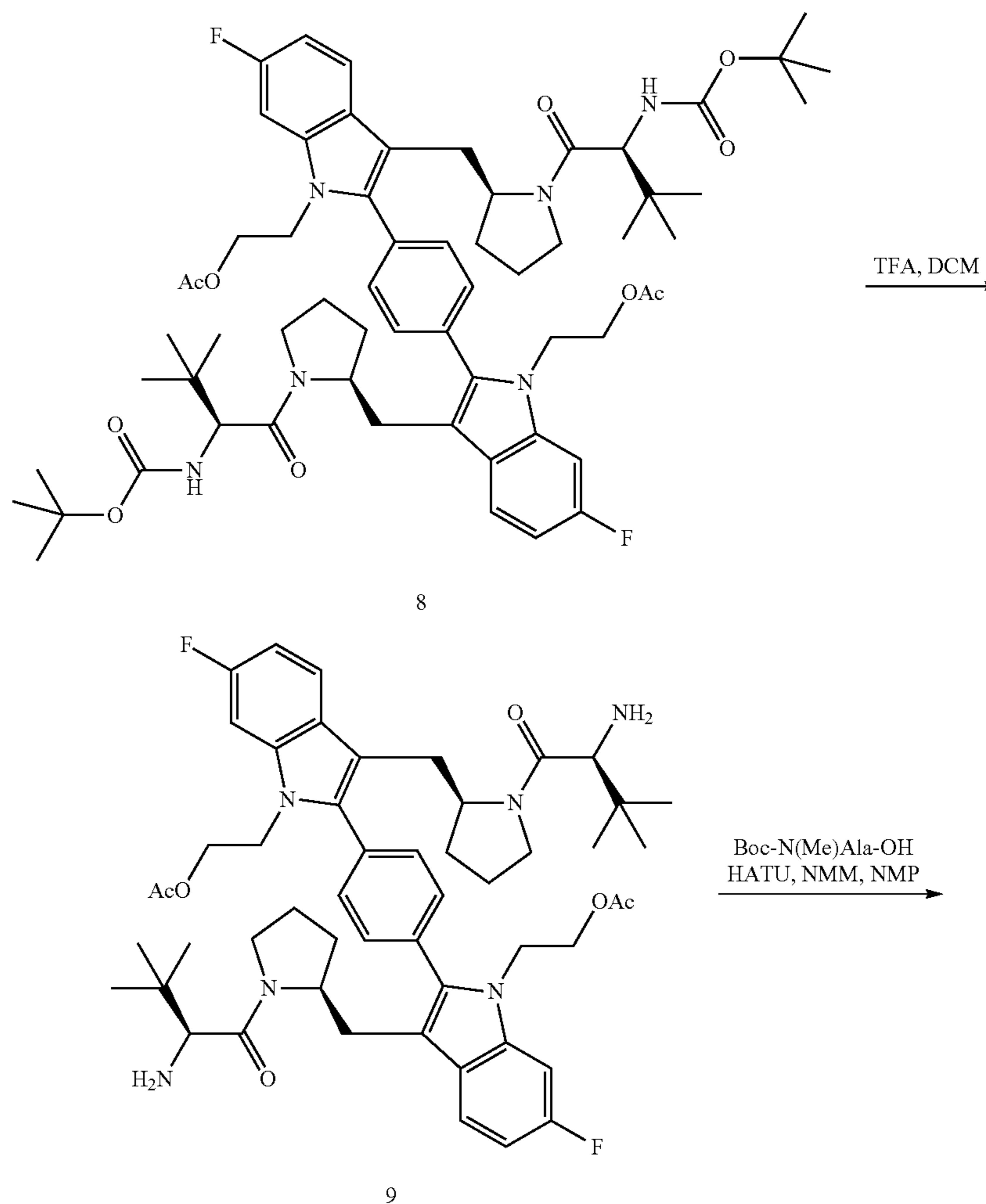
Scheme IV
