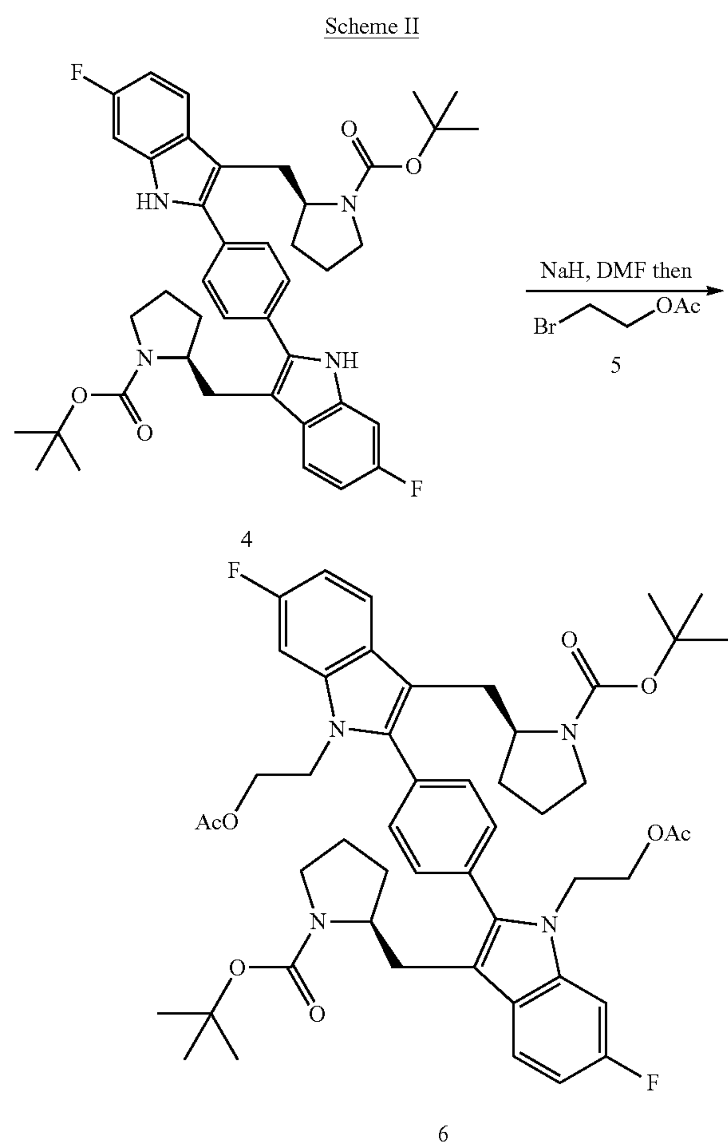
1,4-Bis-{2-[1-(2-Acetoxy-ethyl)-6-fluoro-1H-indol-3-ylmethyl]-pyrrolidine-1-carboxylic acid tert-butyl ester}benzene (6)
