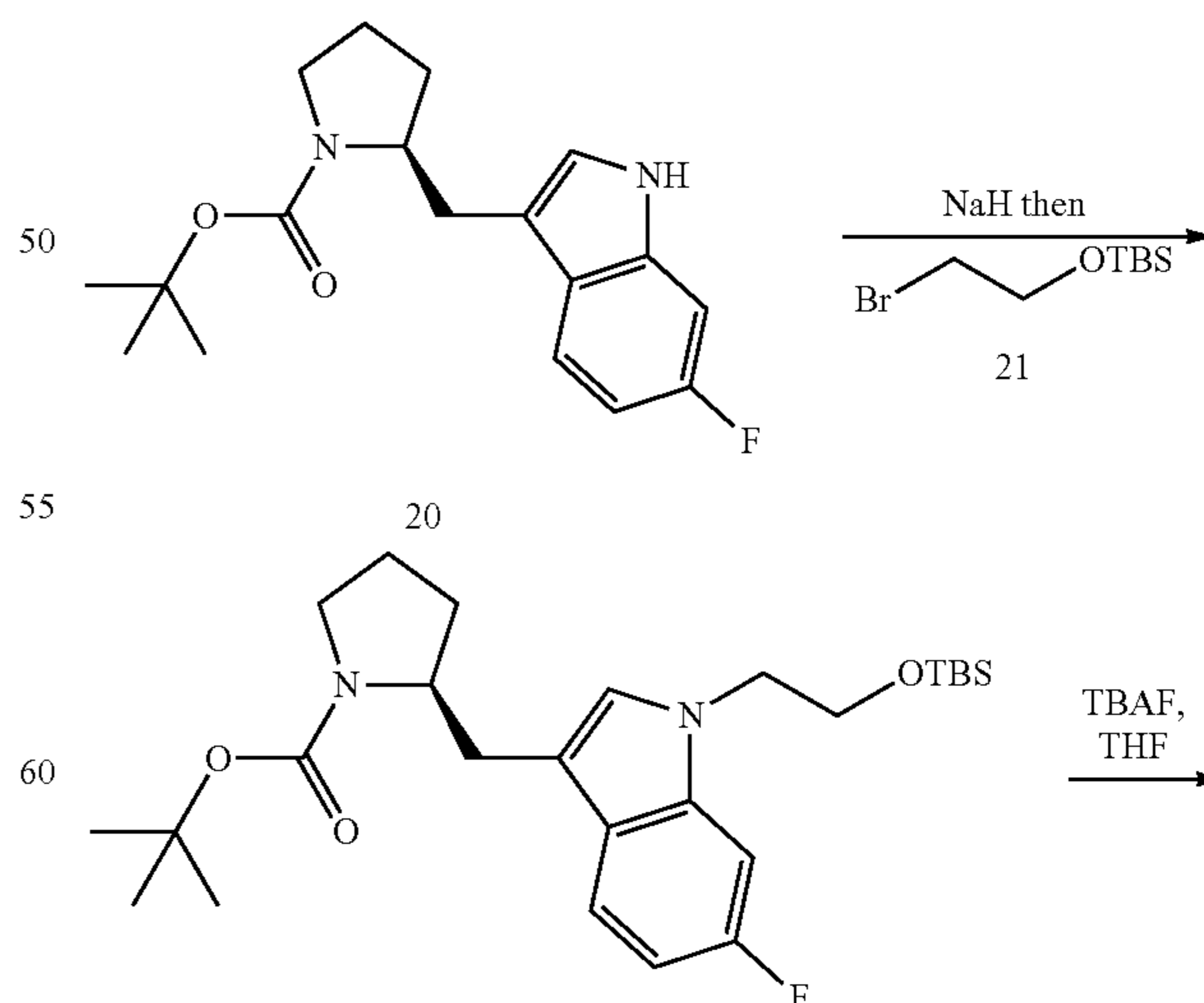
Scheme VIII
