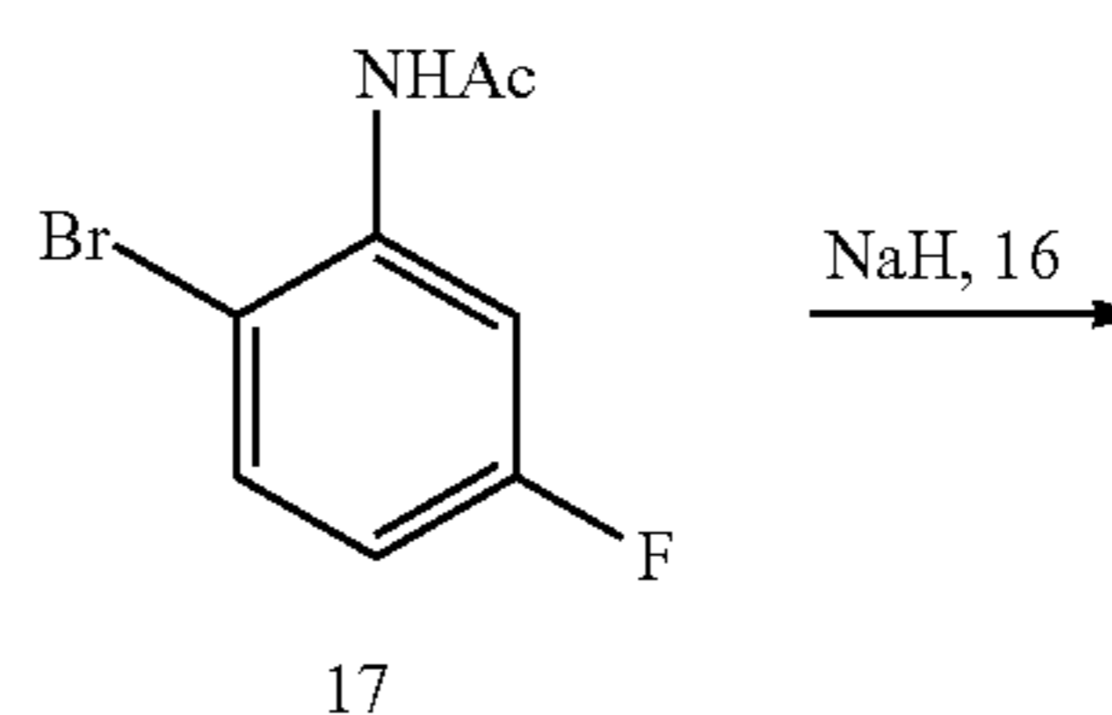
Scheme VII
