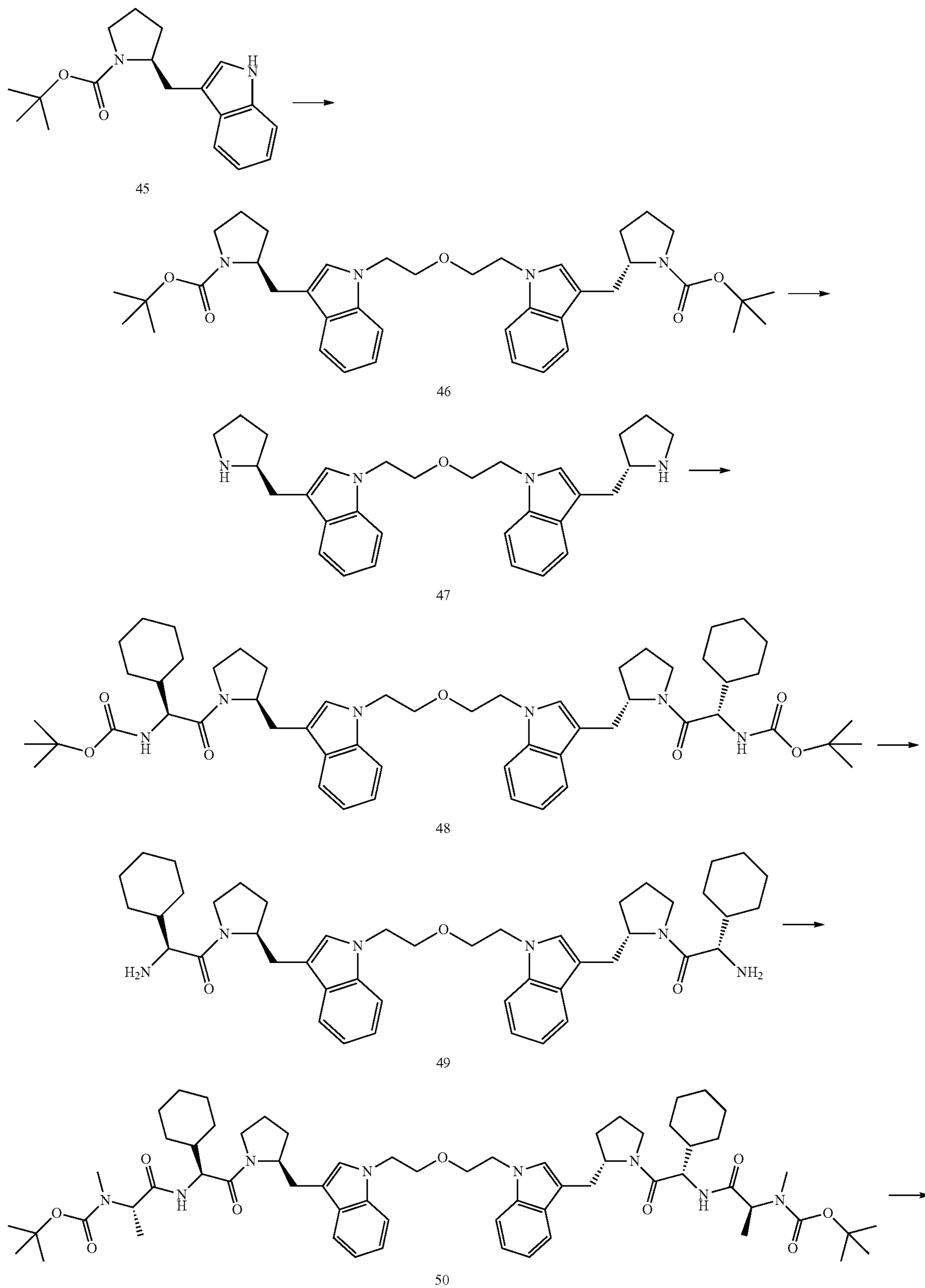
Scheme XXI
