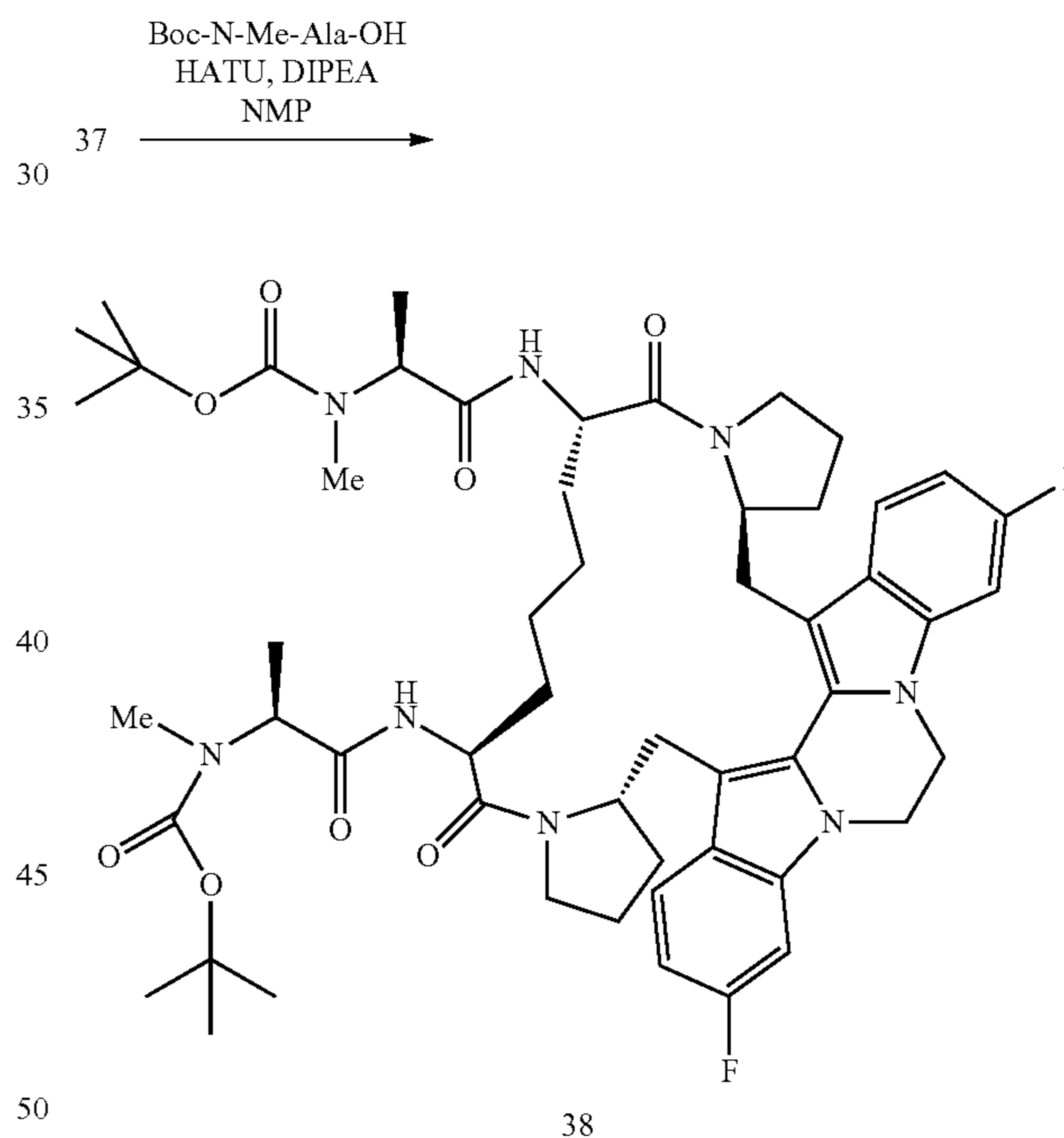
Scheme XVIII
