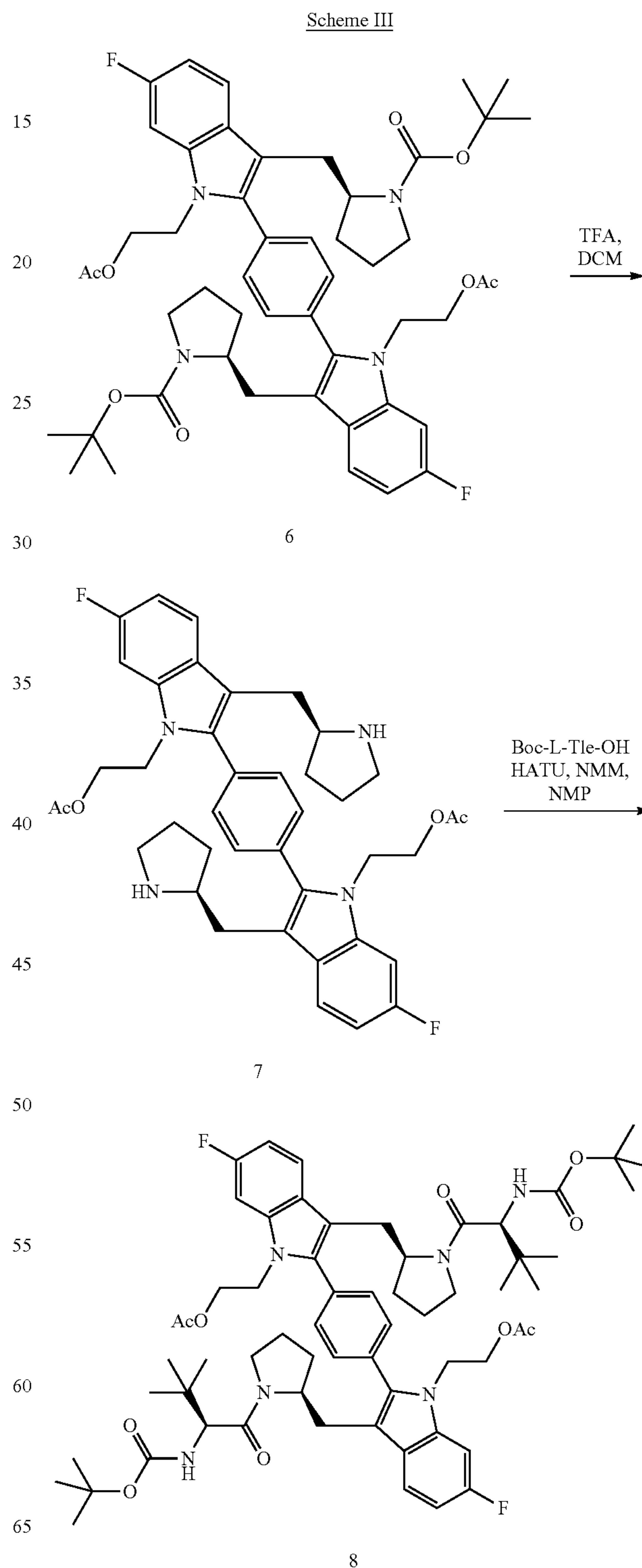
1,4-Bis-{2-[1-(2-Acetoxy-ethyl)-6-fluoro-1H-indol-3-ylmethyl]-pyrrolidine-1-carboxylic acid tert-butyl ester}benzene (6)
