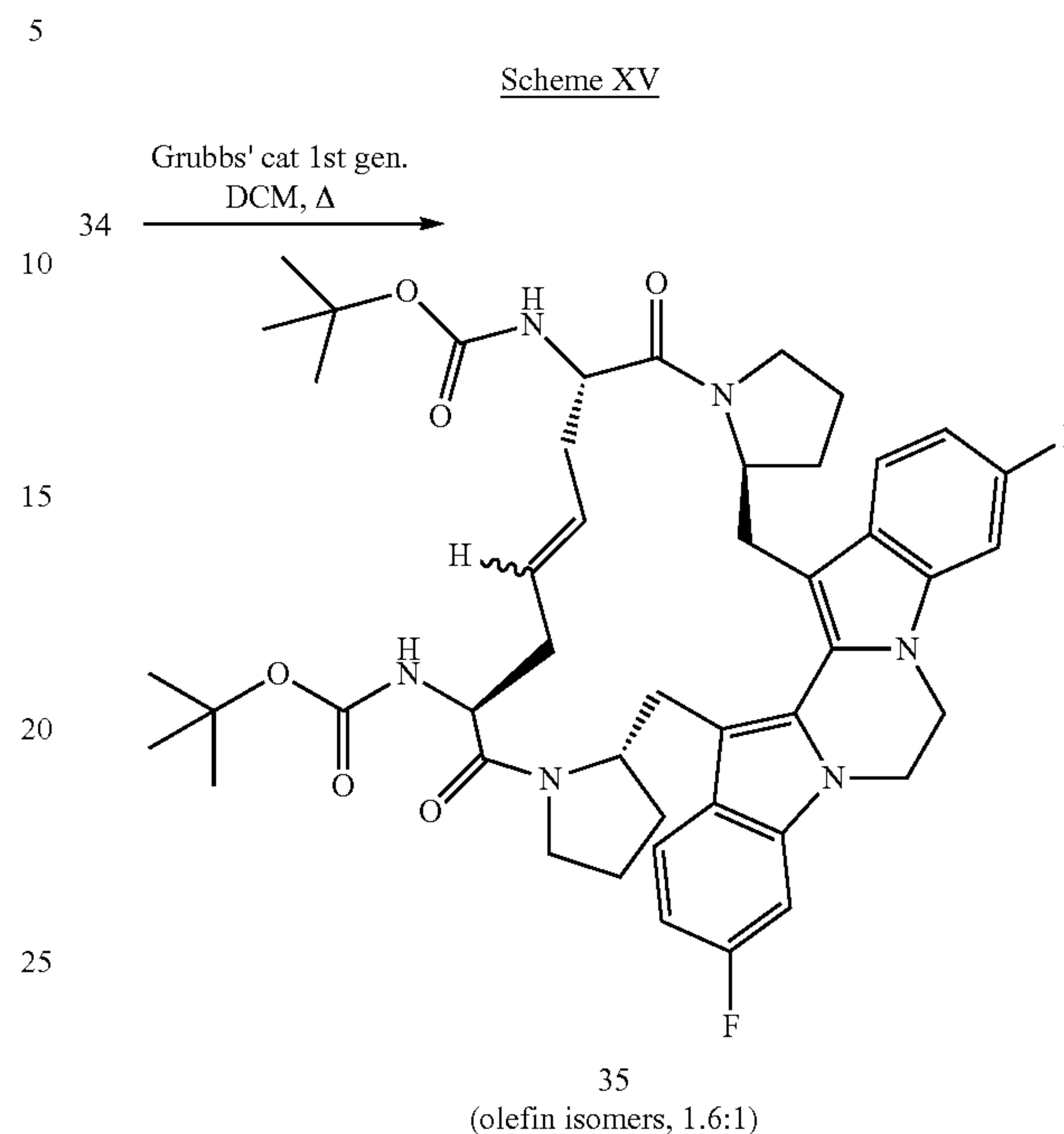
Ring Closing Metathesis (RCM) Product (35):
