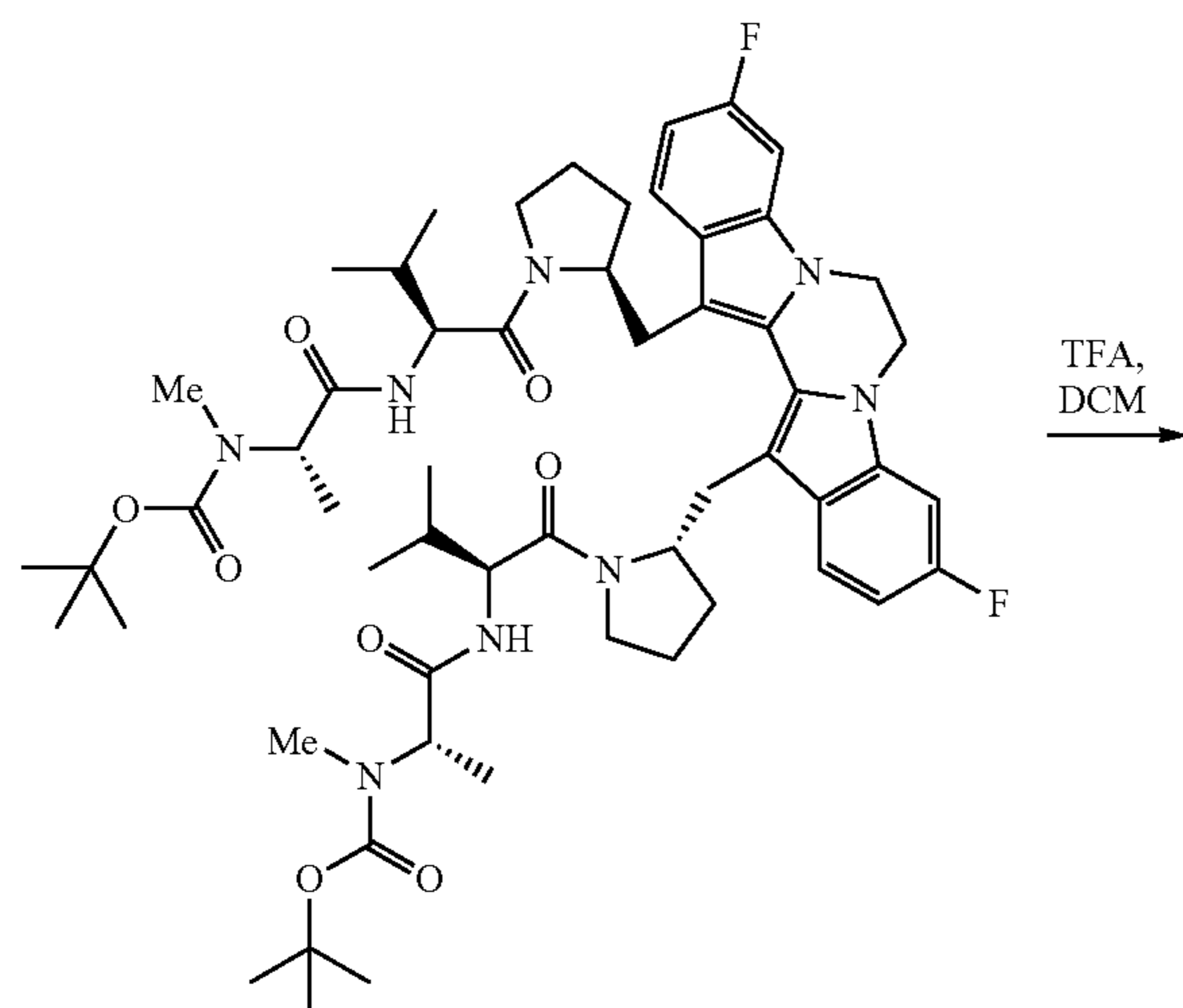
Scheme XIII
