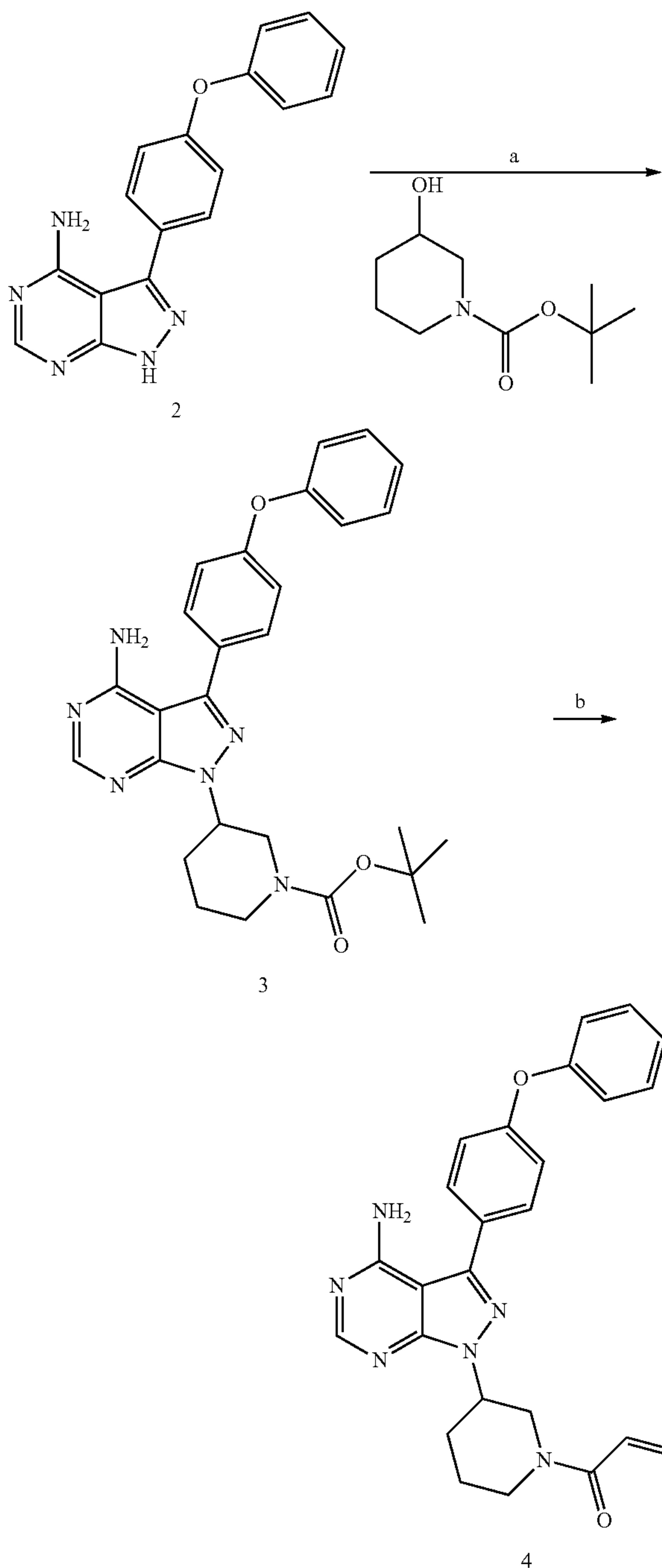
Scheme 1
