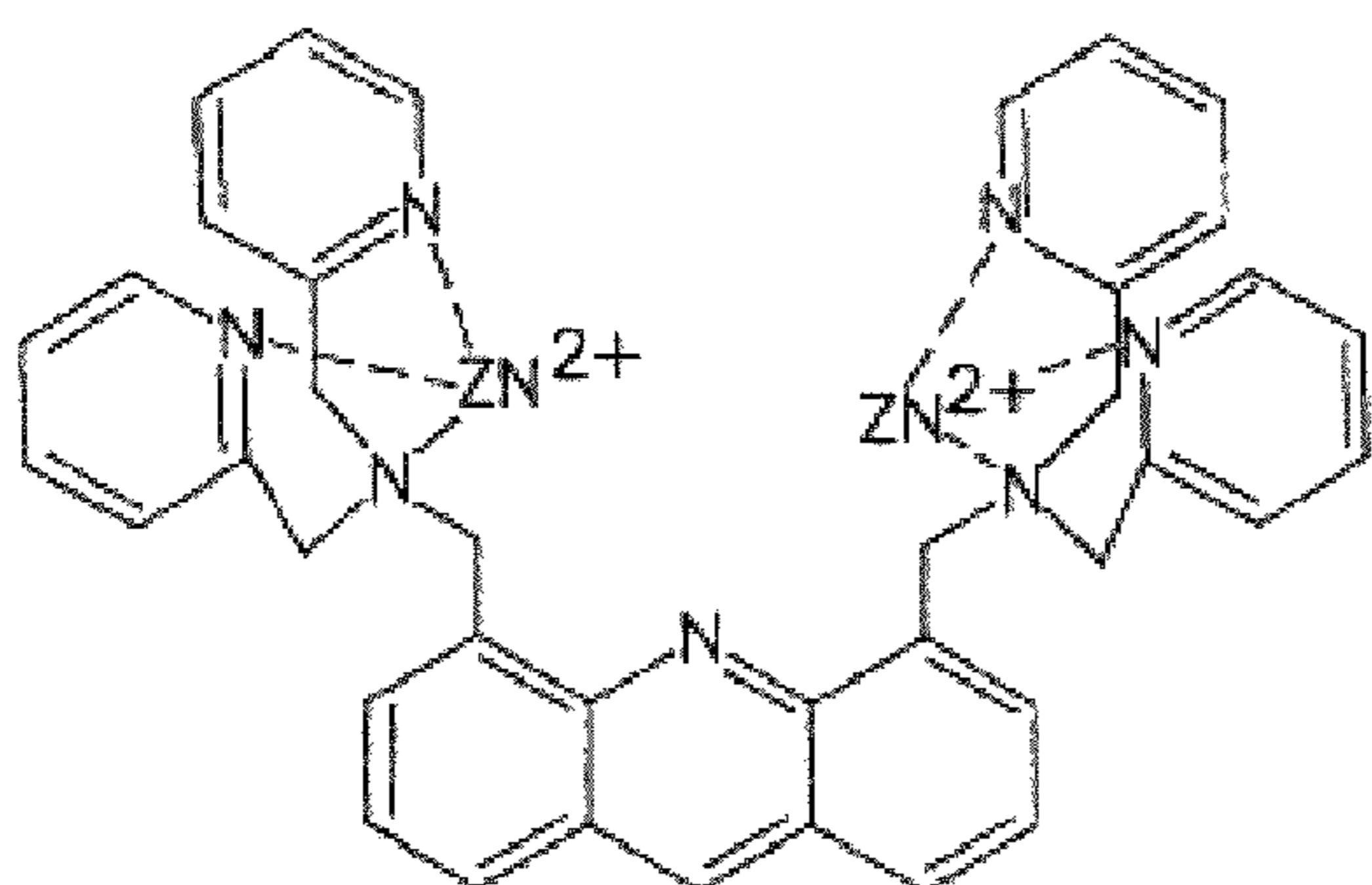
Compound 3
