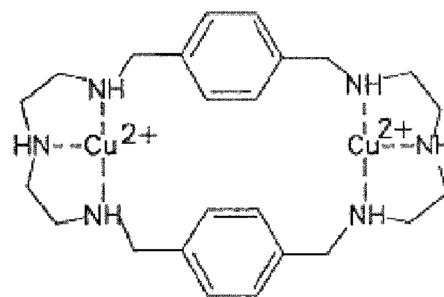
Compound 4
