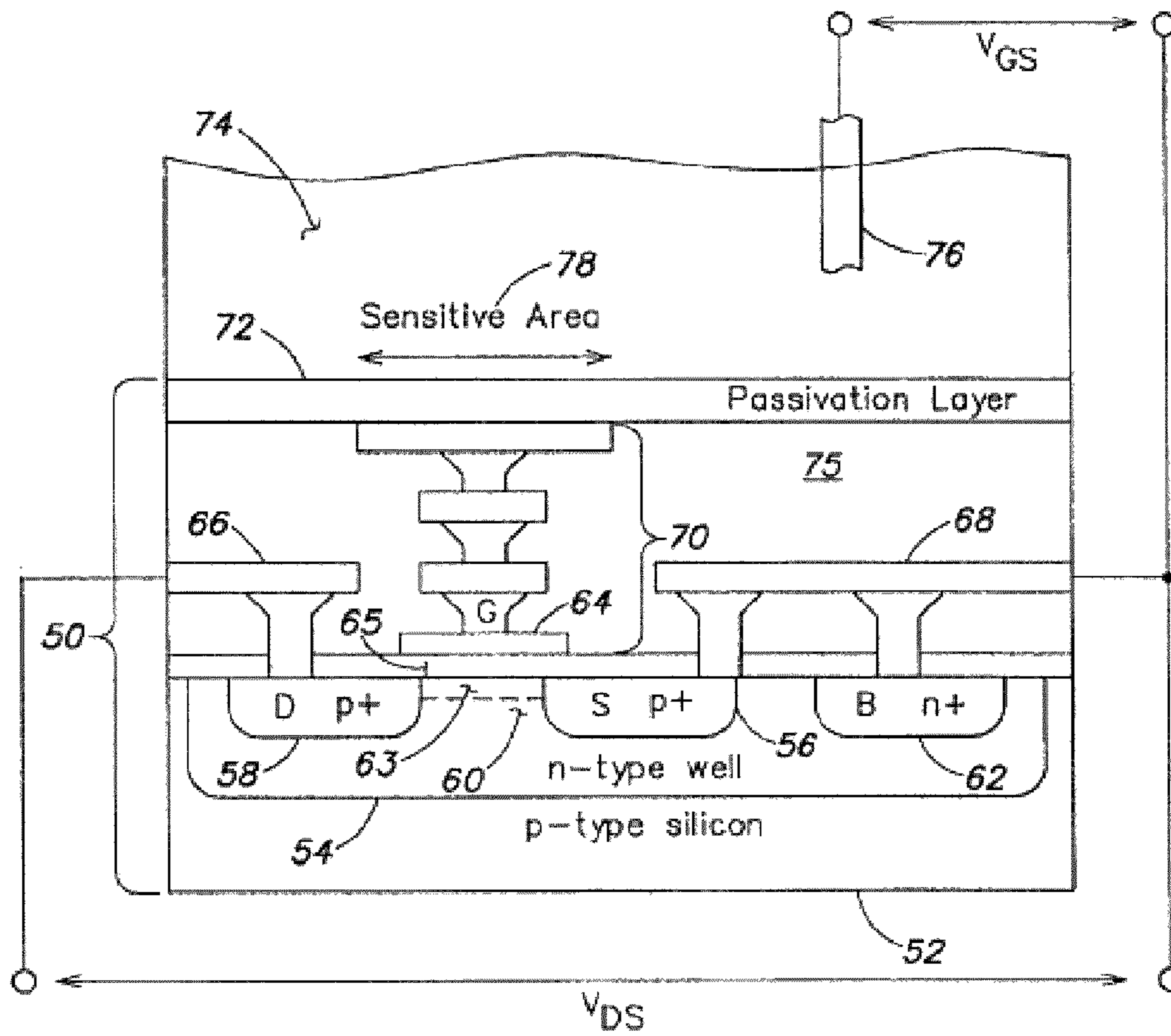
FIG. 1 (Prior Art)
