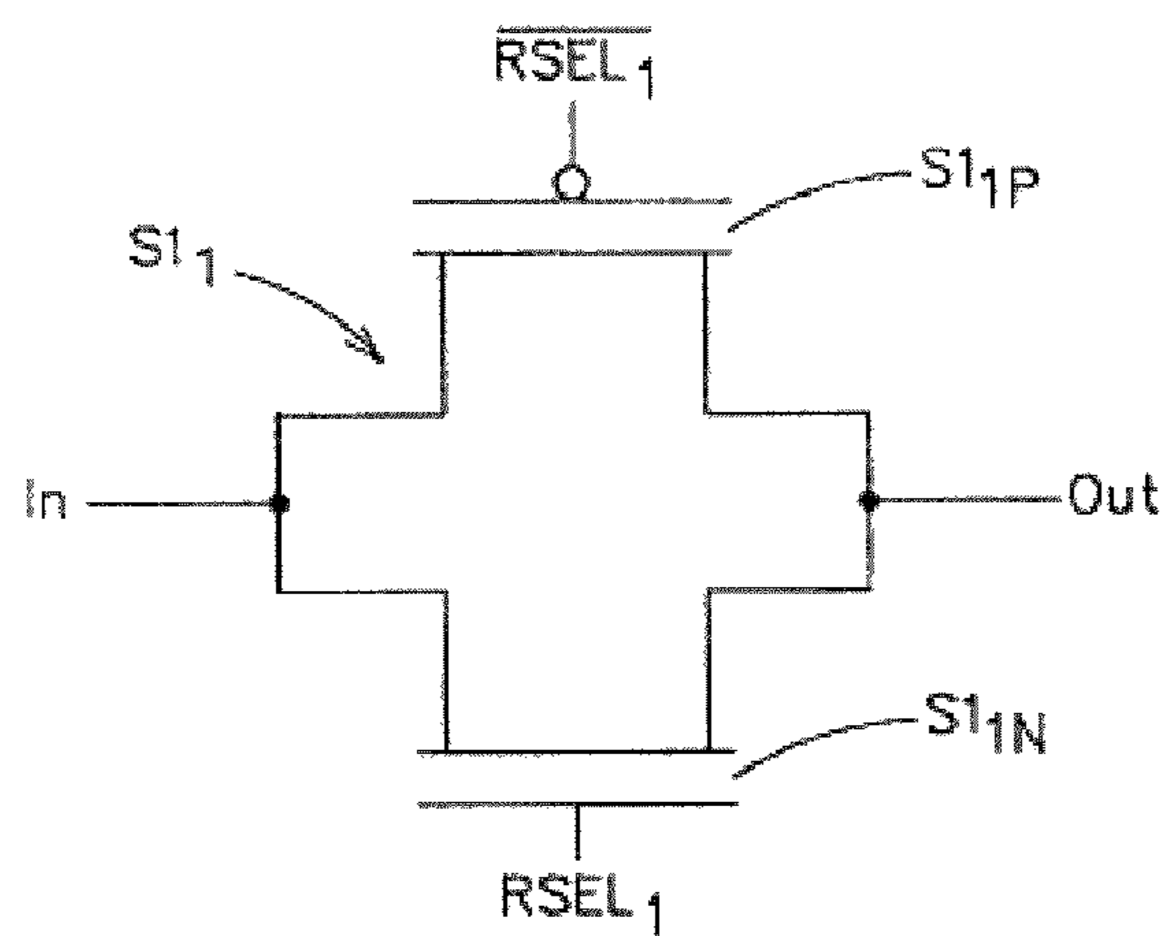
FIG. 4 (Prior Art)
