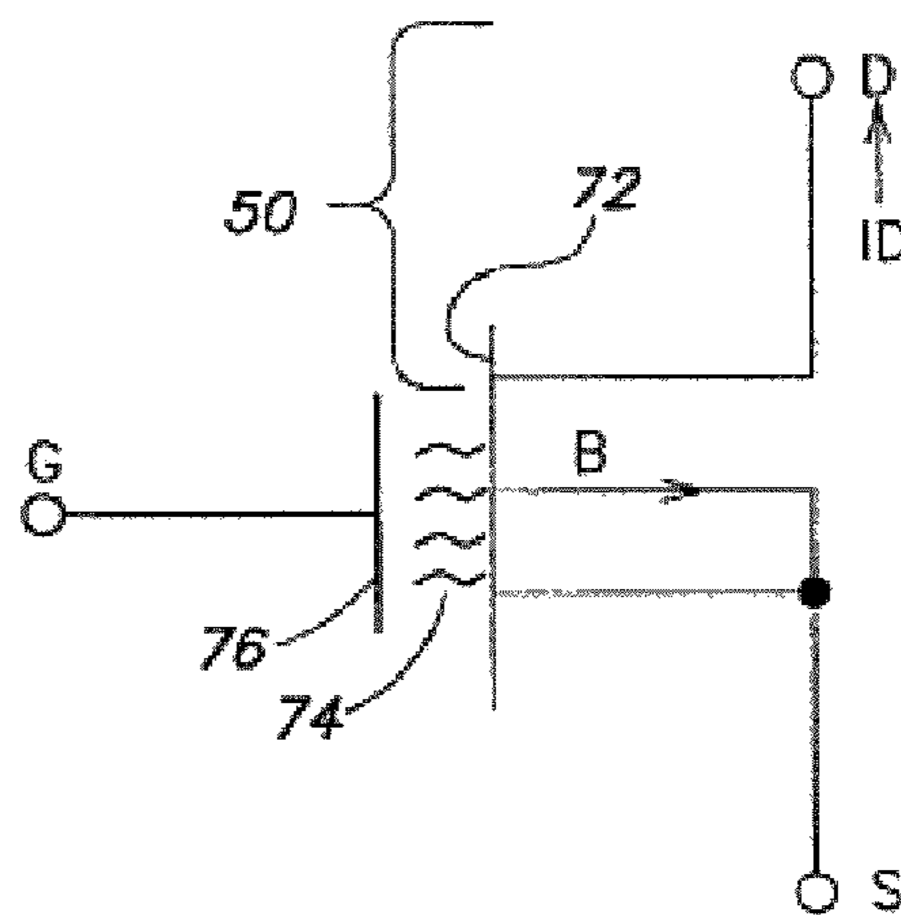
FIG. 2 (Prior Art)
