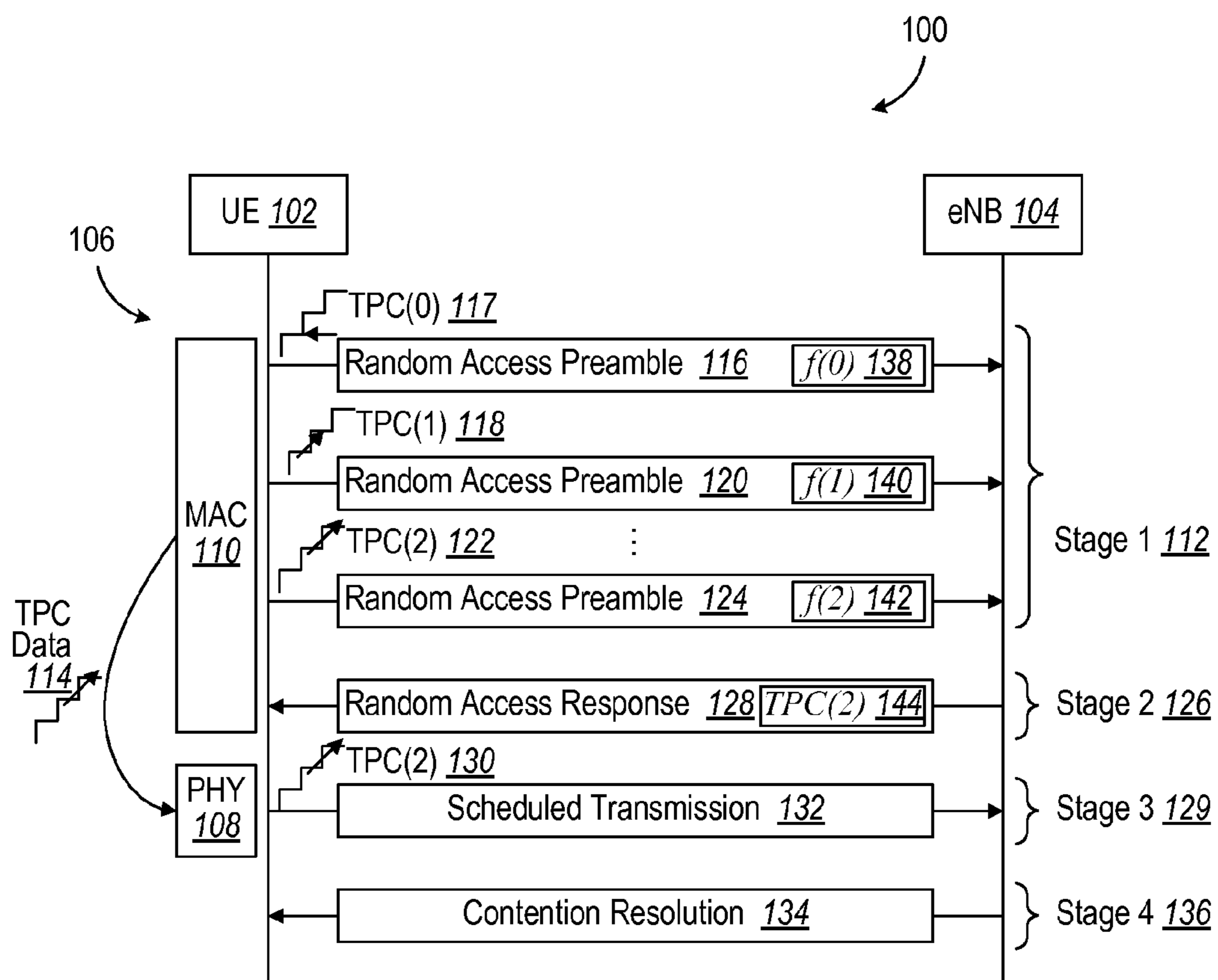
Contention-Based Random Access (RACH) Procedure
