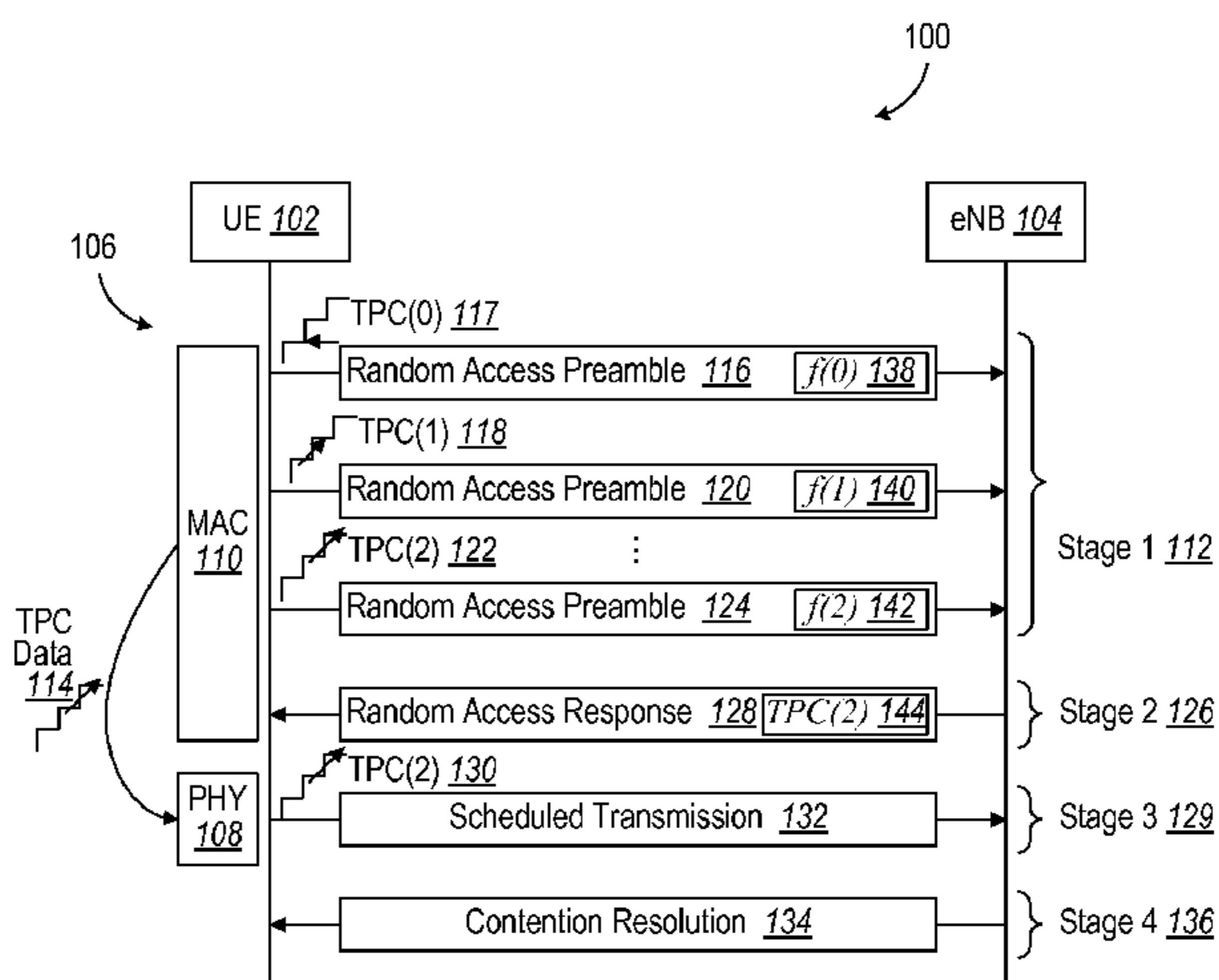
Contention-Based Random Access (RACH) Procedure
