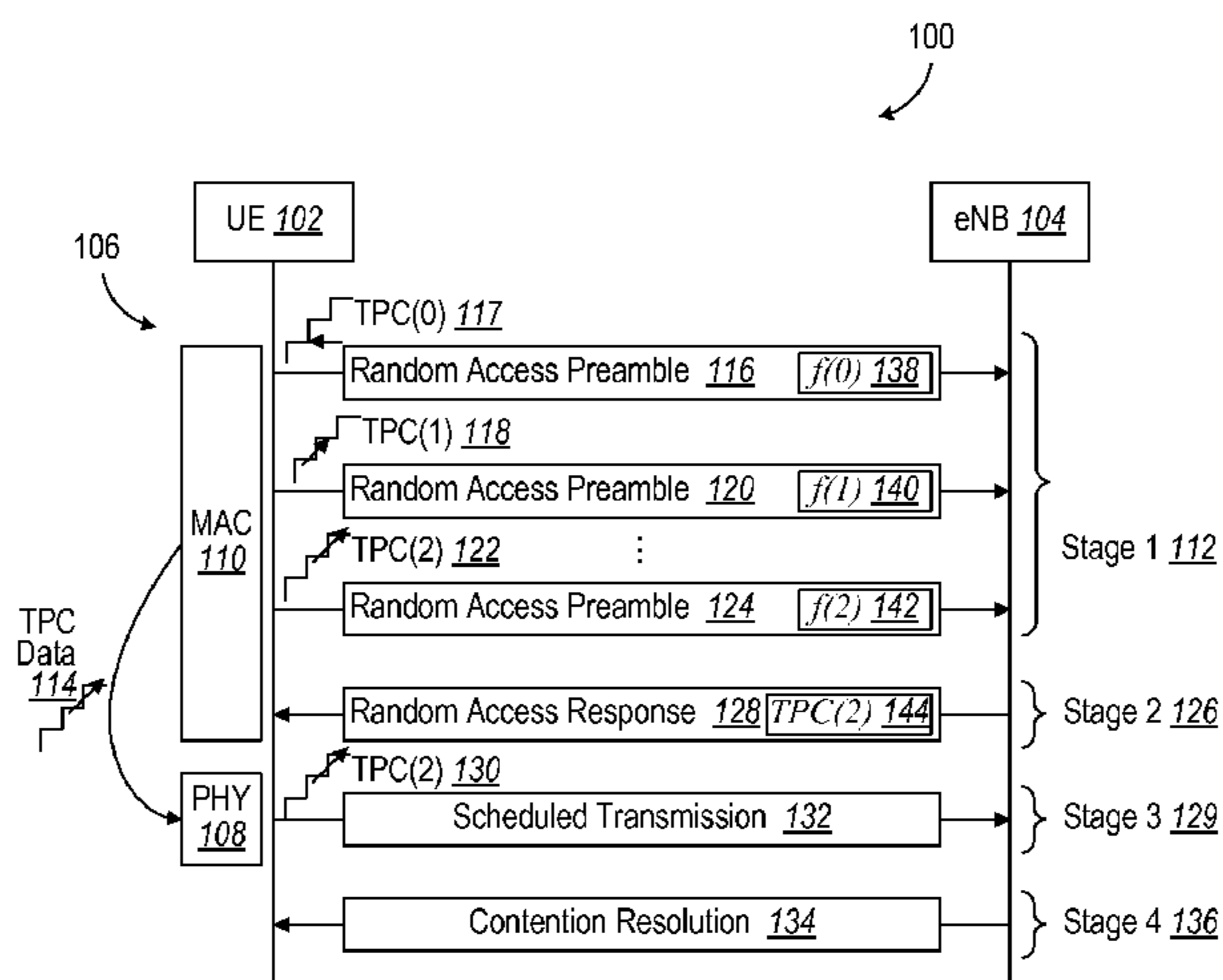
Contention-Based Random Access (RACH) Procedure
