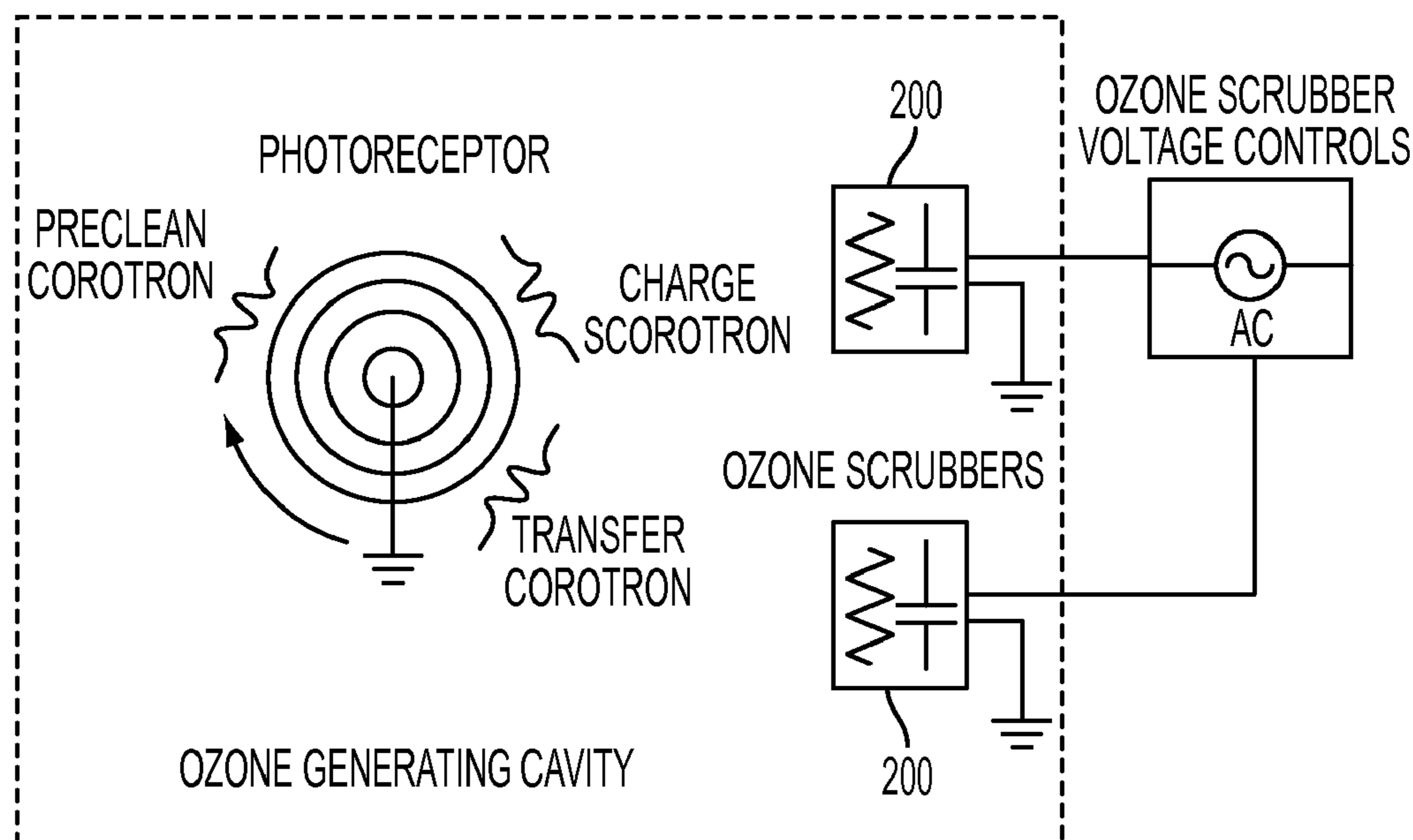
ACTIVE OZONE SCRUBBER OPERATIONAL LAYOUT
