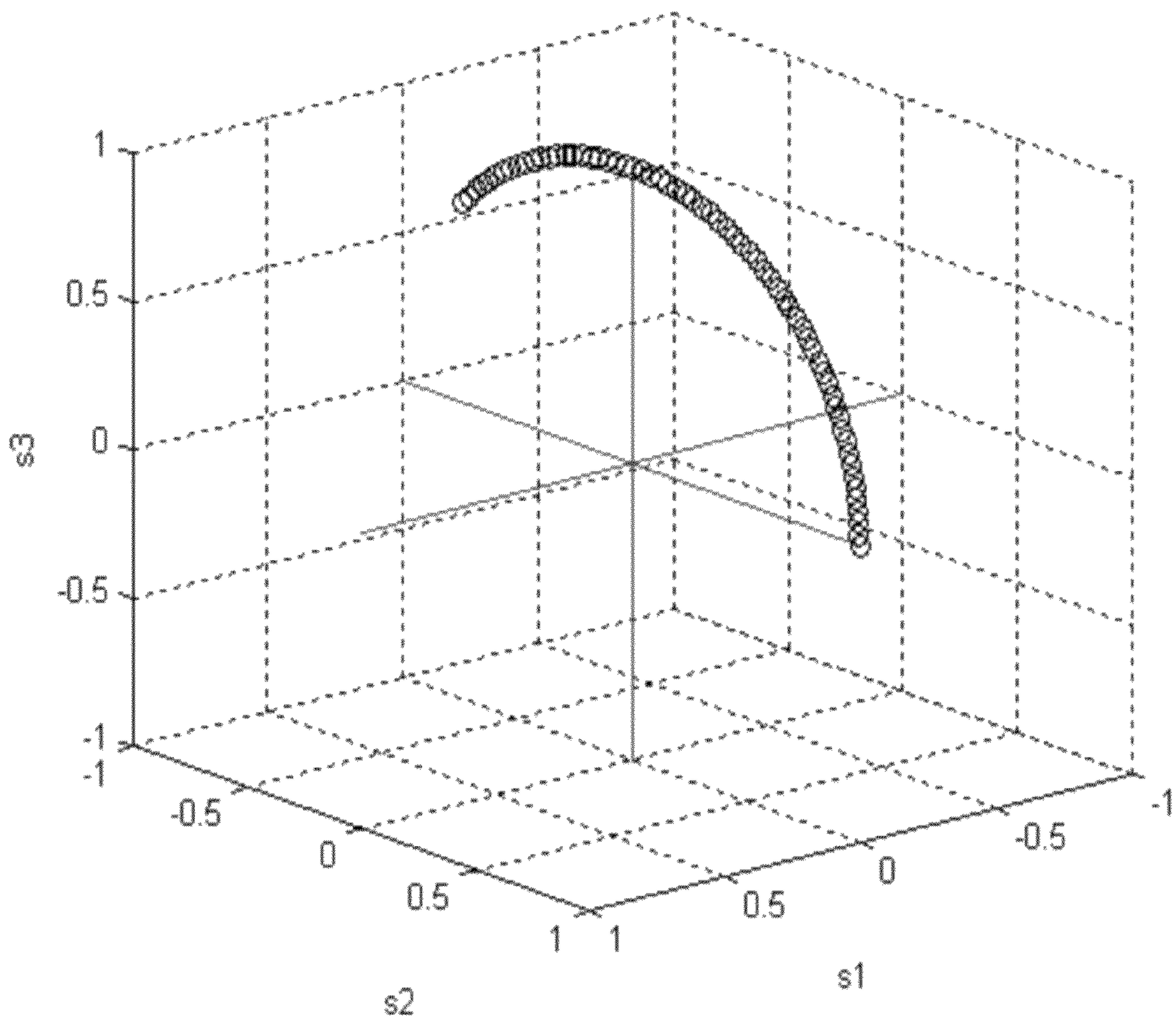
Poincare Sphere - Rotations caused by Bend Method Fiber Tap - 2.4 radians, > 90degrees
