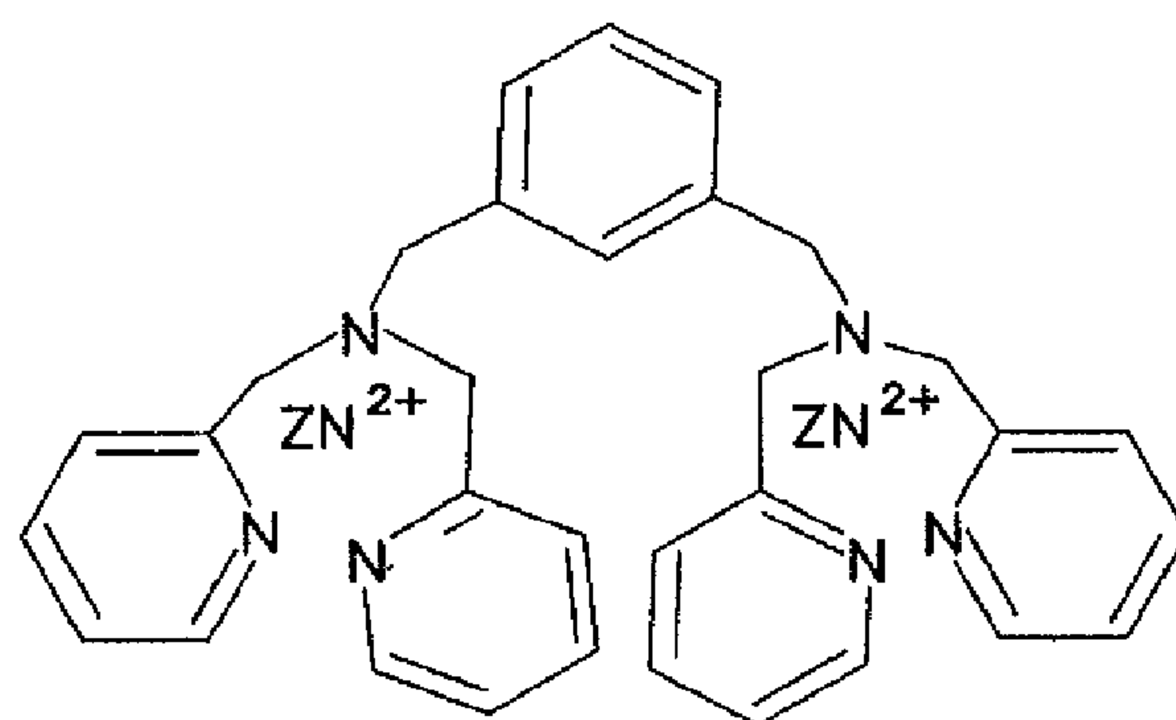
\text{Zn}^{2+} -dipicolylamine Compound 5
