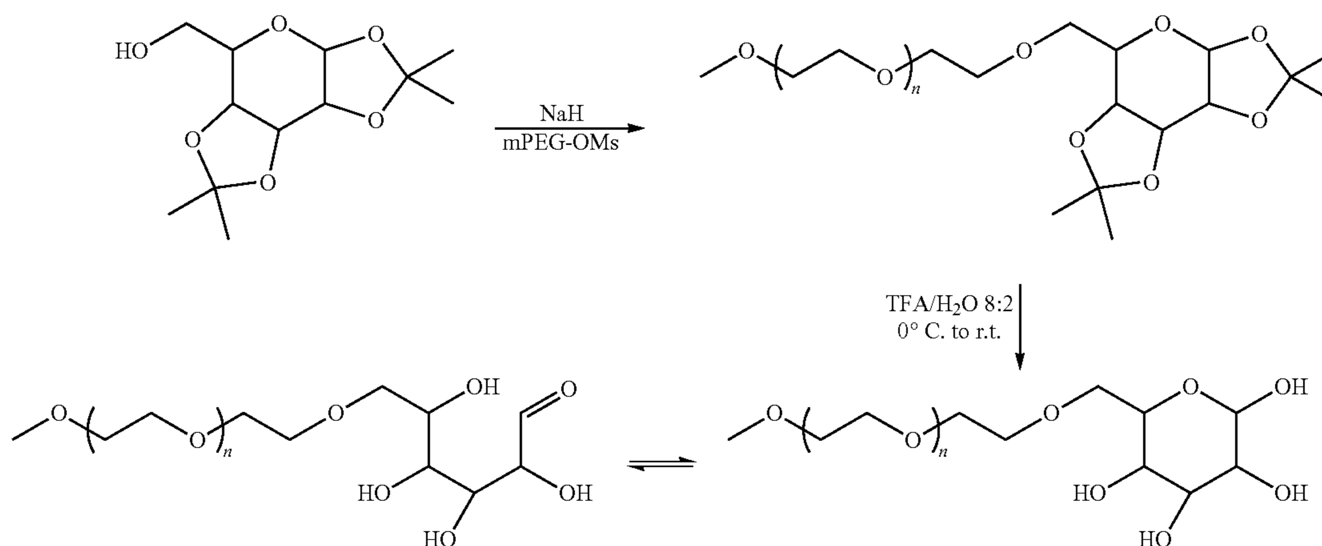
Hemiacetal form of an alpha-hydroxyaldehyde
