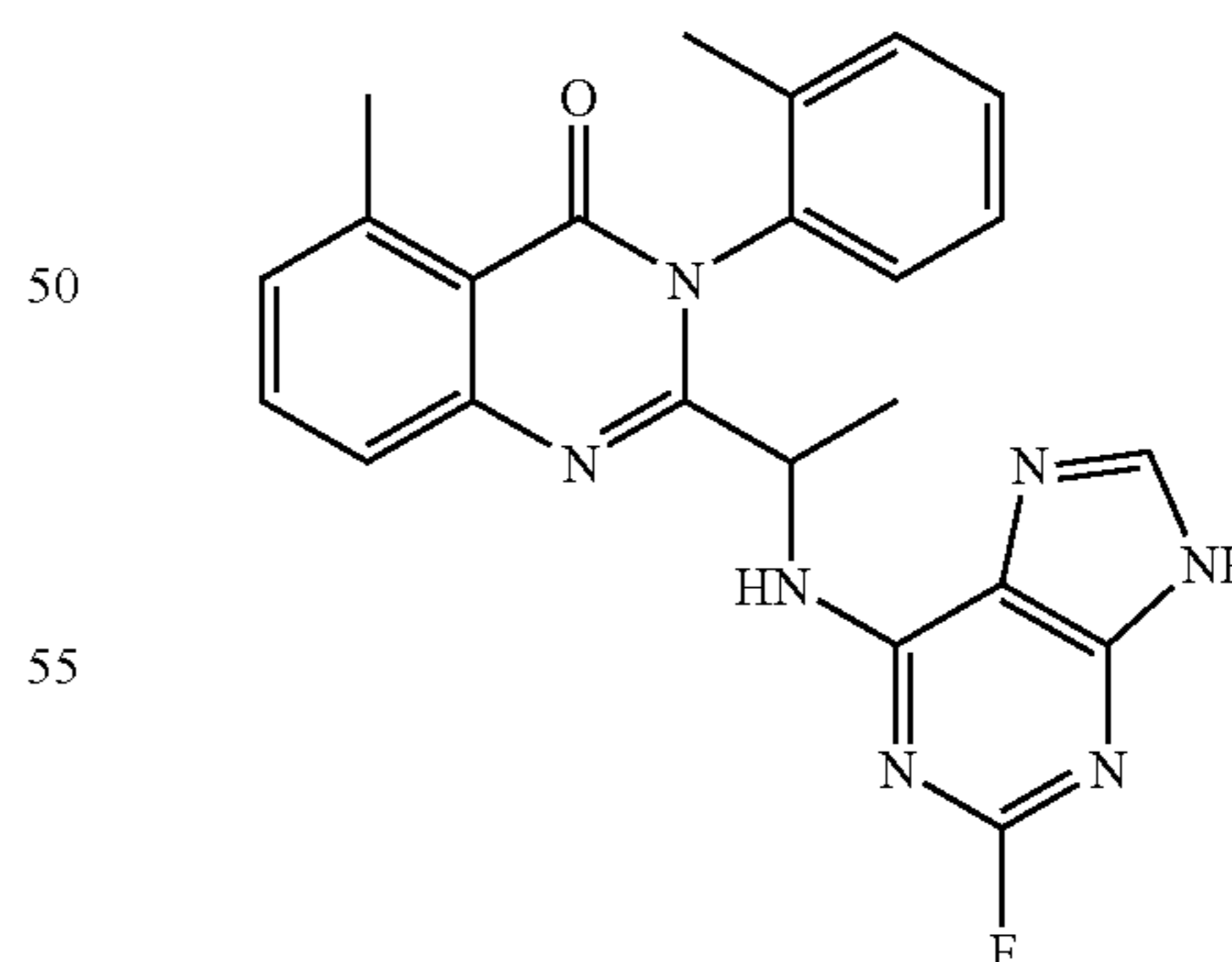
2-[1-(2-Fluoro-9H-purin-6-ylamino)ethyl]-5-methyl-3-o-tolyl-3H-quinazolin-4-one (D-080)
