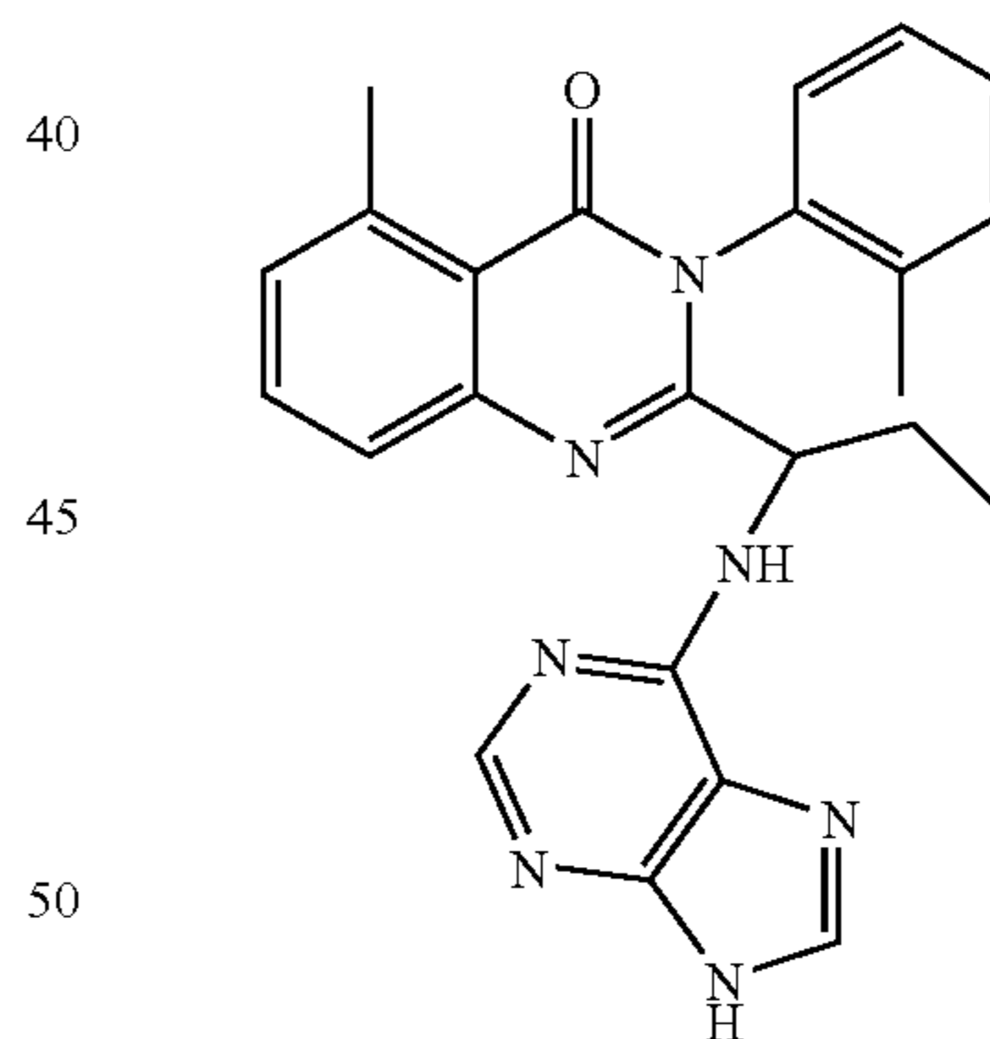
5-Methyl-2-(1-(9H-purin-6-ylamino)propyl)-3-o-tolyl-3H-quinazolin-4-one (D-081b)
