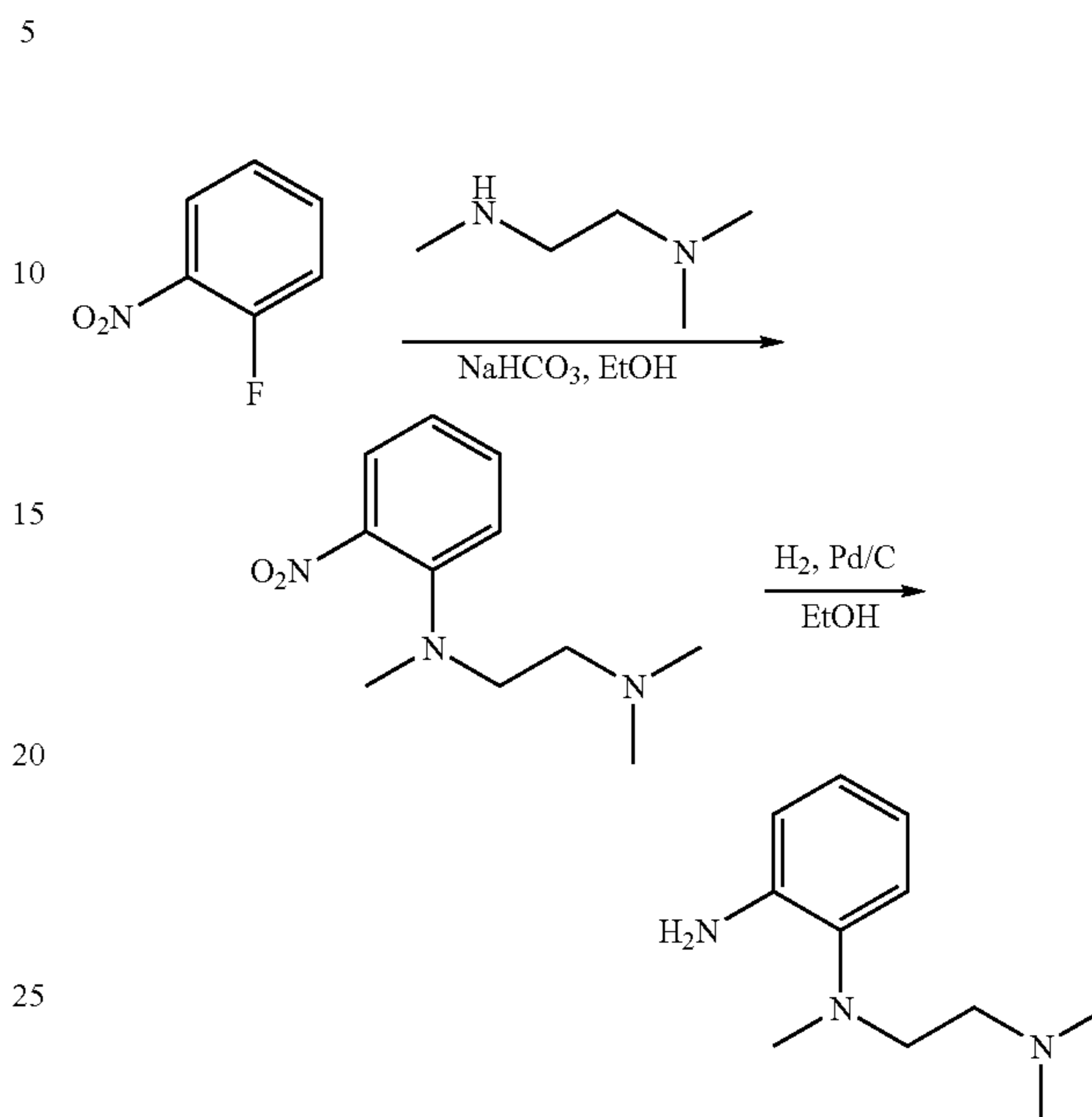
Intermediate E-3
