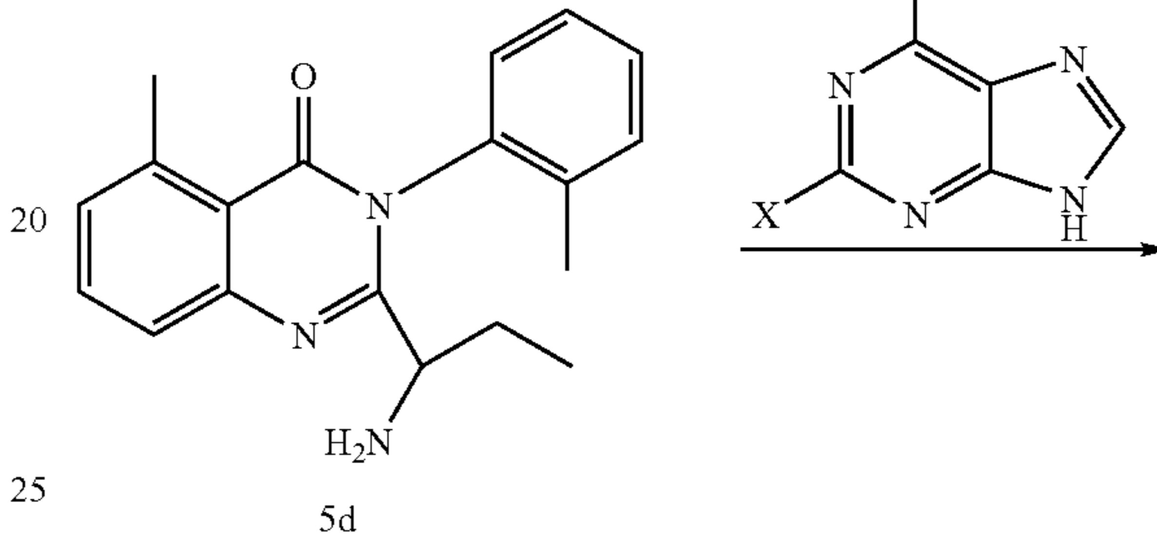
5d
