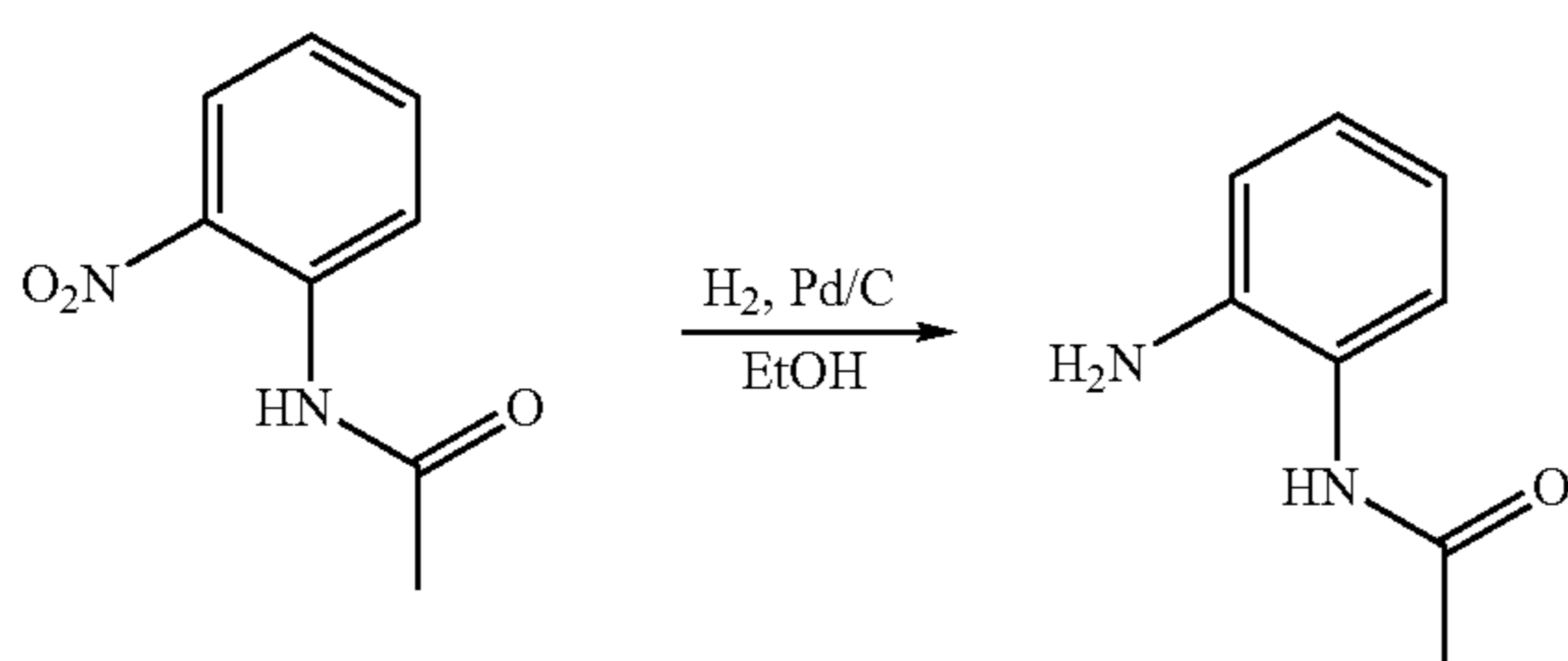
Intermediate E-2
