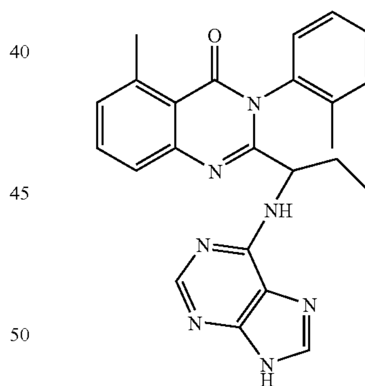
5-Methyl-2-(1-(9H-purin-6-ylamino)propyl)-3-o-tolyl-3H-quinazolin-4-one (D-081b)
