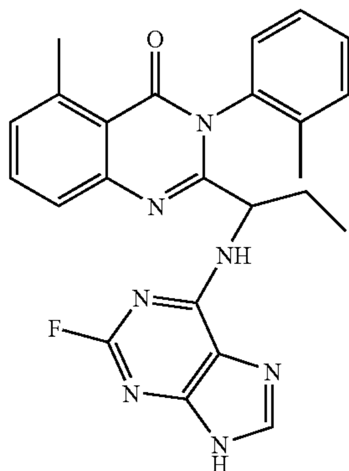
2-(1-(2-Fluoro-9H-purin-6-ylamino)propyl)-5-methyl-3-o-tolyl-3H-quinazolin-4-one (D-081c)
