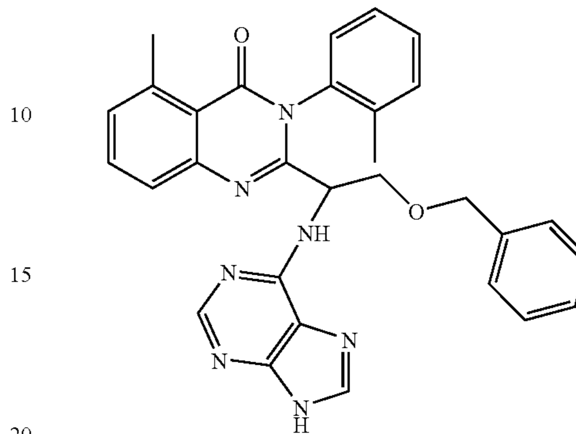
2-[2-Benzyloxy-1-(9H-purin-6-ylamino)ethyl]-5-methyl-3-o-tolyl-3H-quinazolin-4-one (D-081e)
