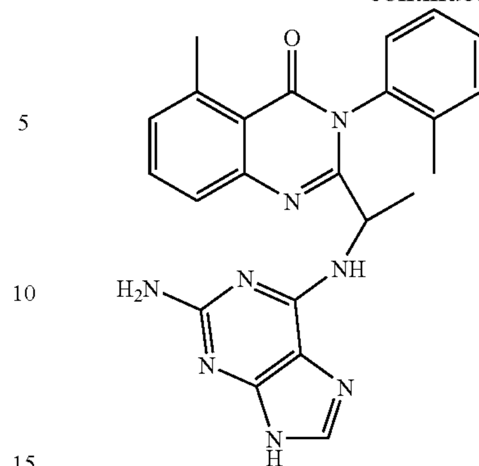
2-(1-(2-Amino-9H-purin-6-ylamino)ethyl)-5-methyl-3-o-tolyl-3H-quinazolin-4-one (D-081a)
