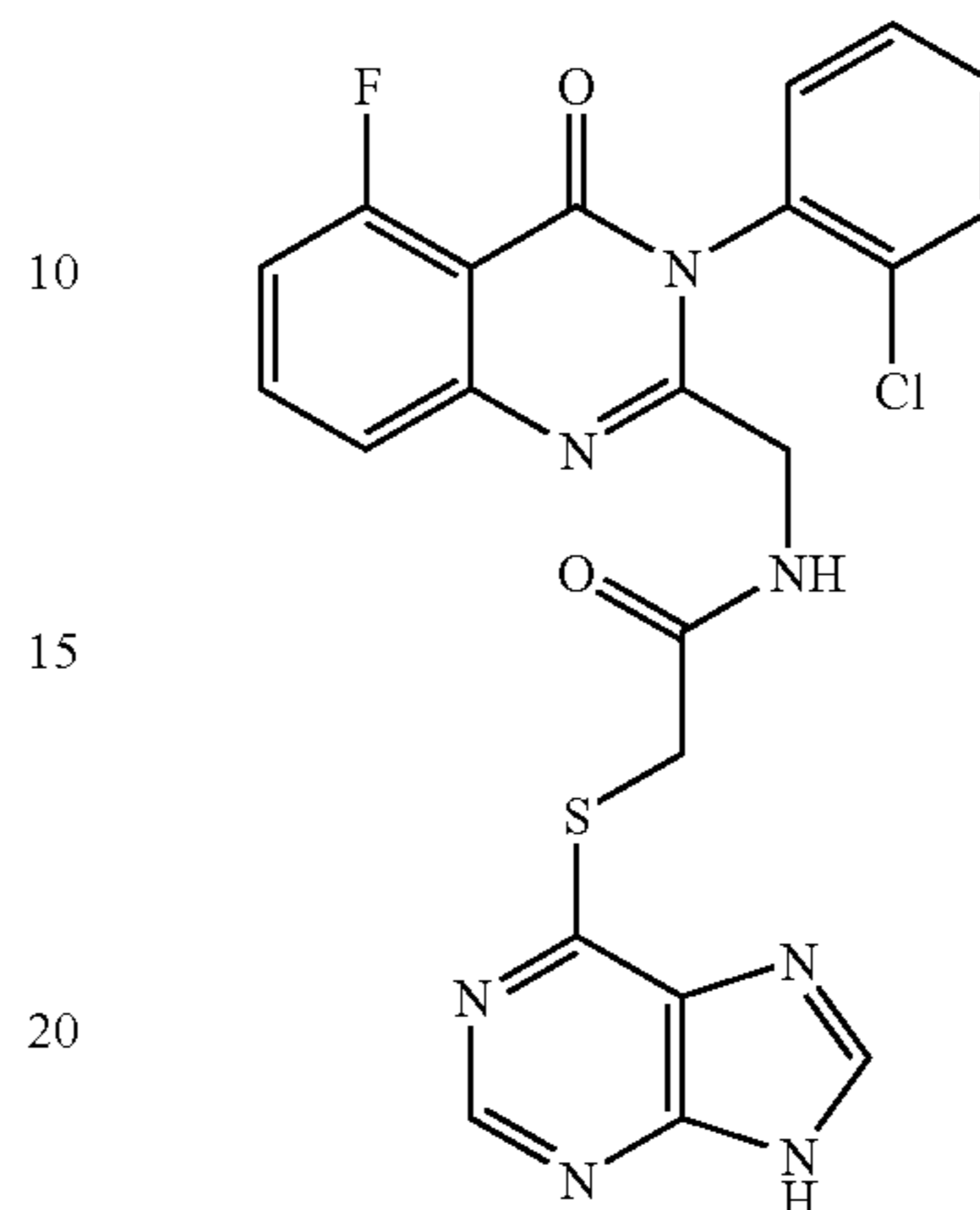
N-[3-(2-Chlorophenyl)-5-fluoro-4-oxo-3,4-dihydro-quinazolin-2-ylmethyl]-2-(9H-purin-6-ylsulfanyl)-acetamide (D-077)
