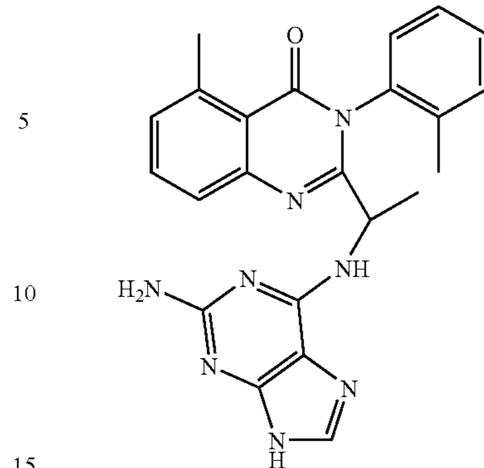
2-(1-(2-Amino-9H-purin-6-ylamino)ethyl)-5-methyl-3-o-tolyl-3H-quinazolin-4-one (D-081a)
