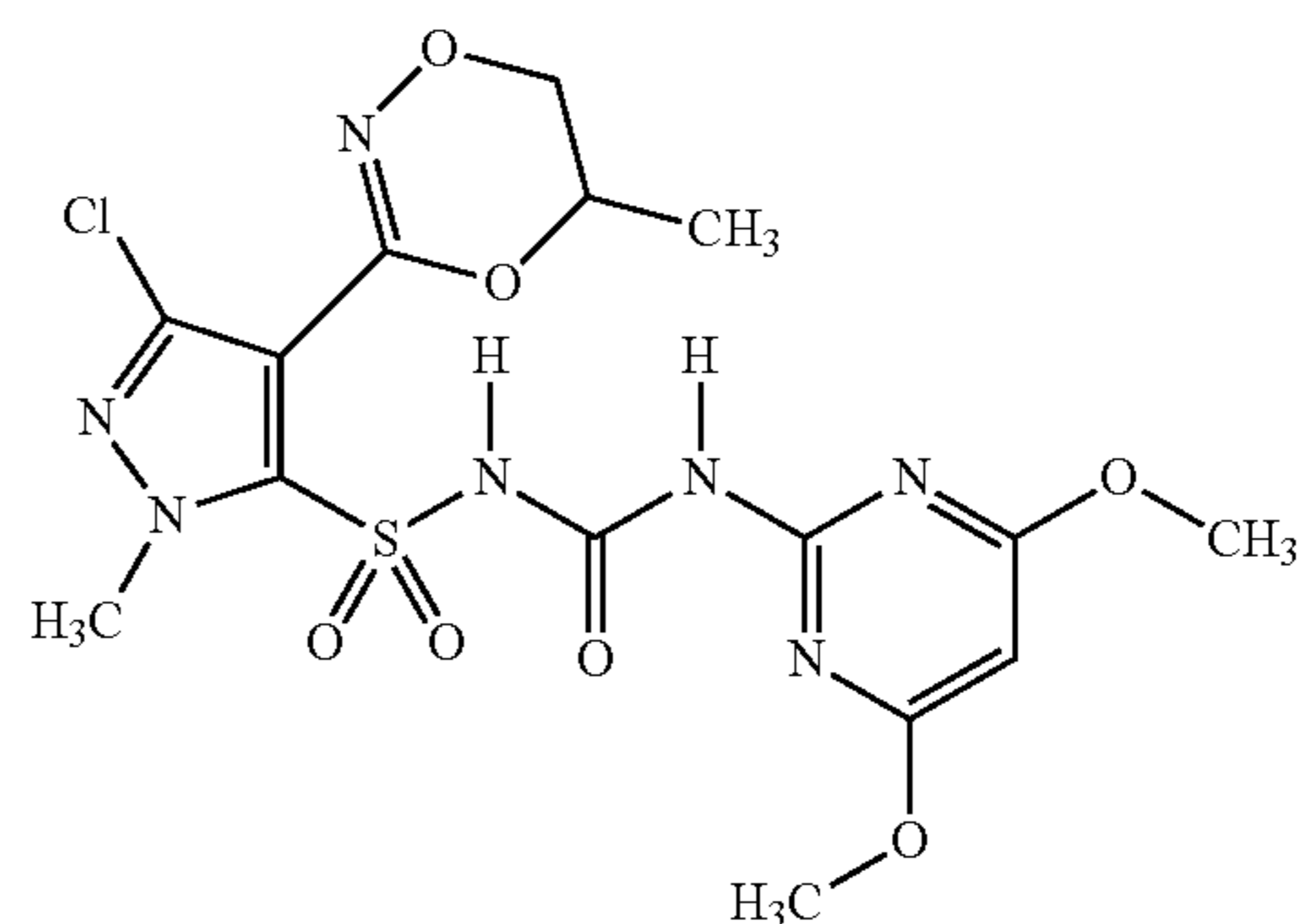
3-chloro-N-[(4,6-dimethoxypyrimidin-2-yl)carbamoyl]-1-methyl-4-(5-methyl-5,6-dihydro-1,4,2-dioxazin-3-yl)-1H-pyrazole-5-sulfonamide
