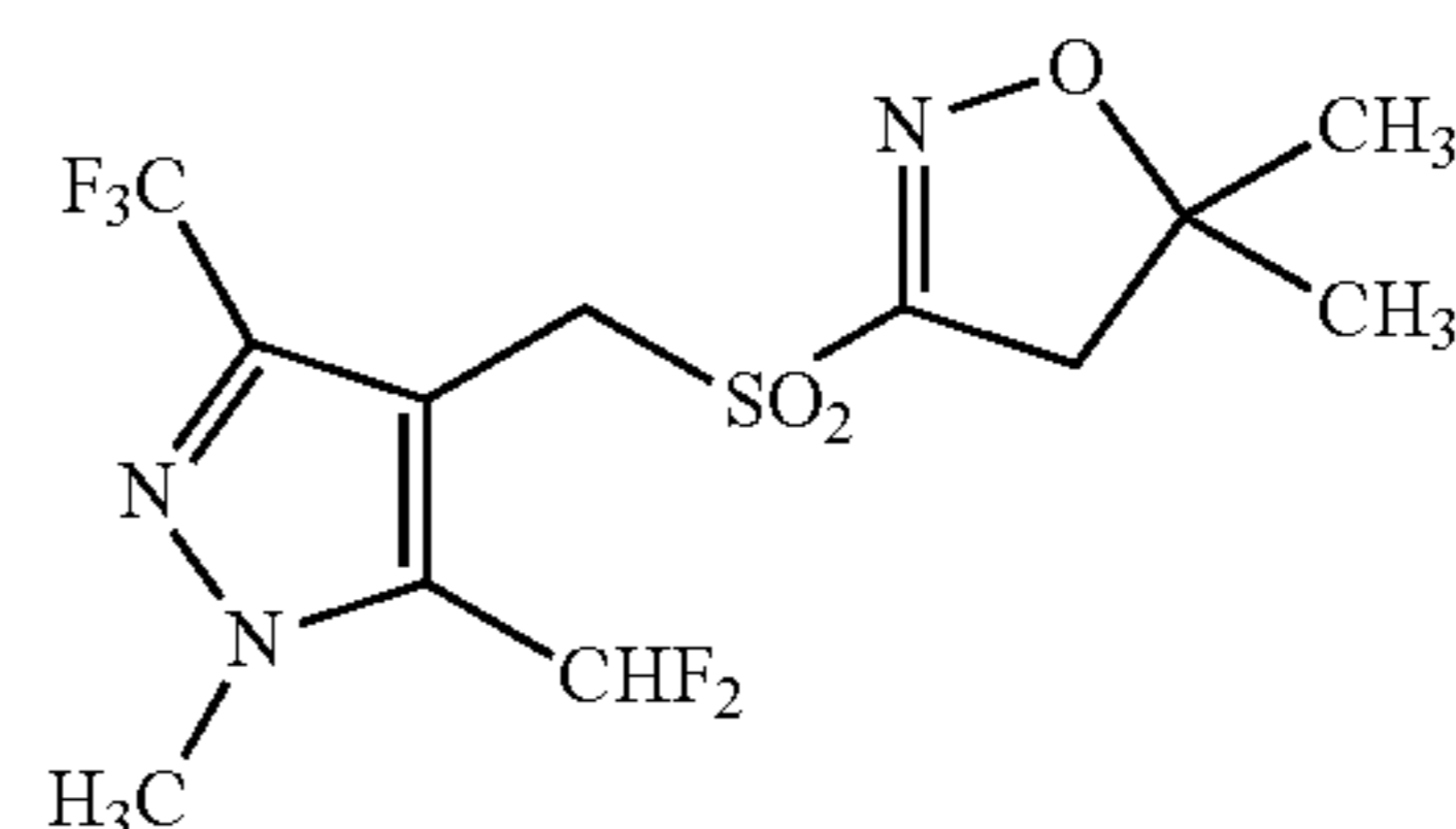
3-({[5-(difluoromethyl)-1-methyl-3-(trifluoromethyl)-1H-pyrazol-4-yl]methyl}sulfonyl)-5,5-dimethyl-4,5-dihydro-1,2-oxazole
