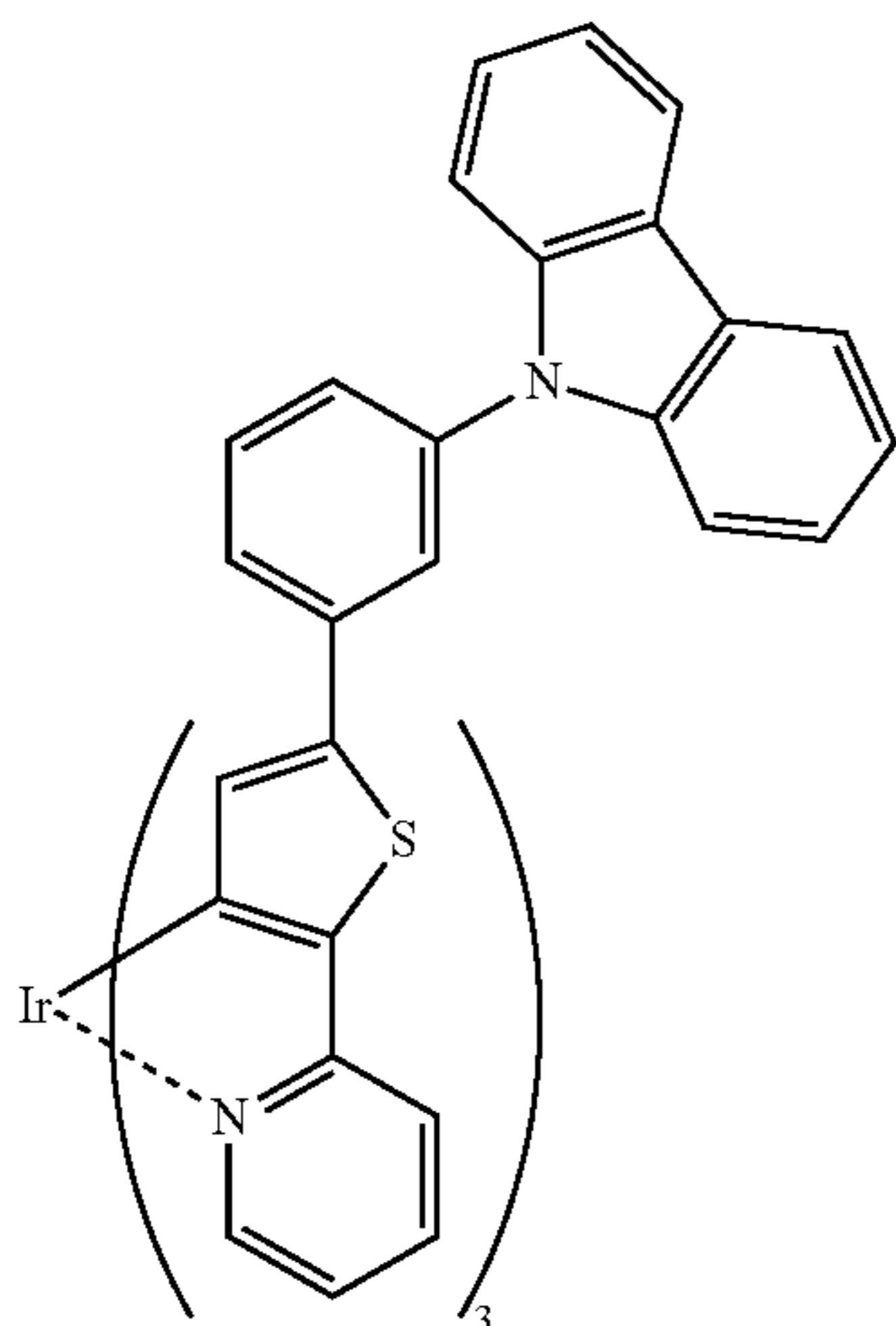
Complex B
