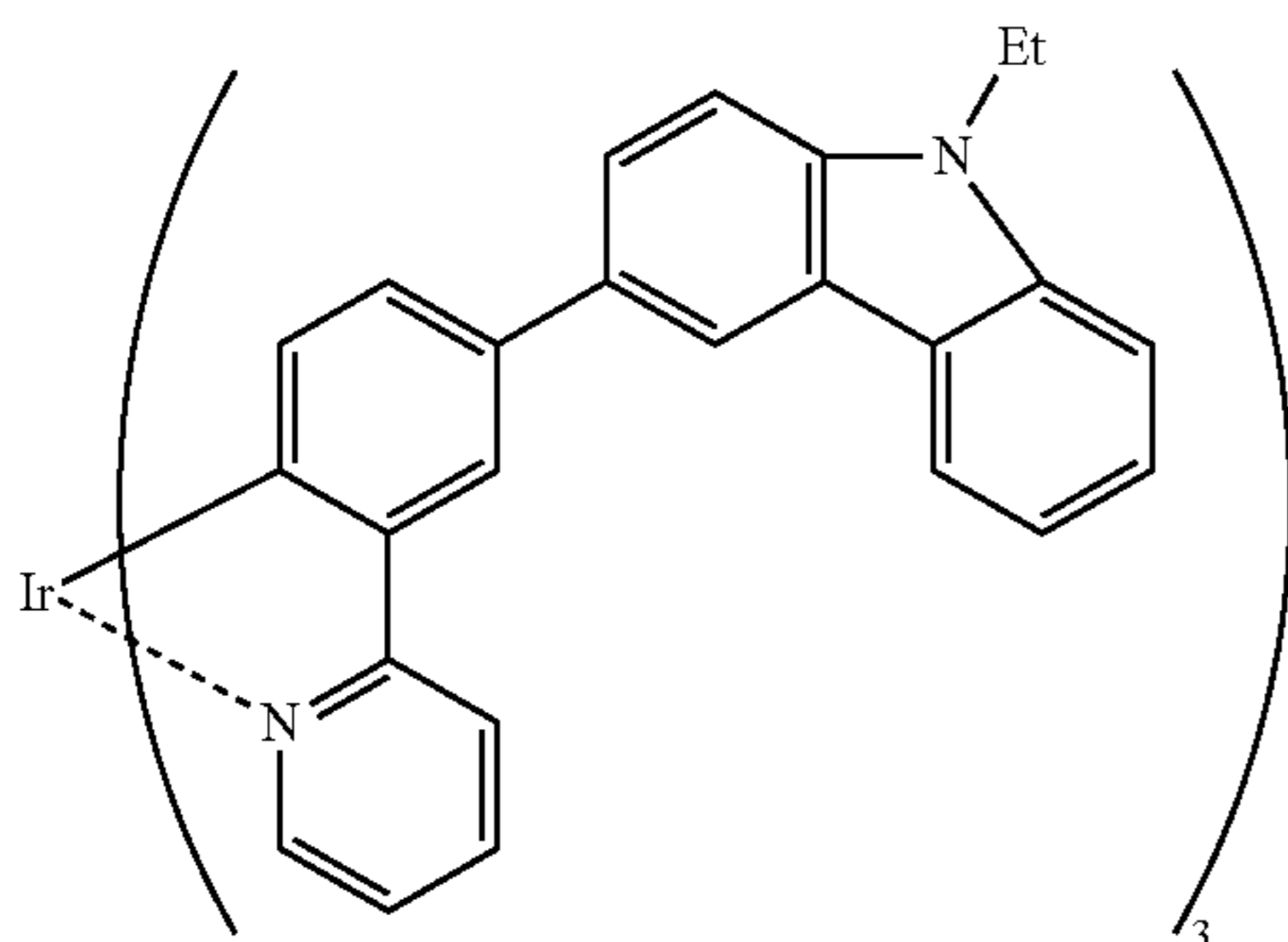
Complex C
