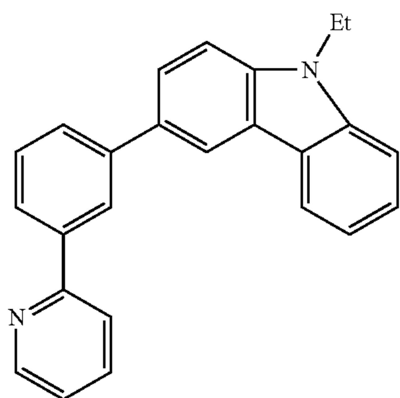
Ligand C
