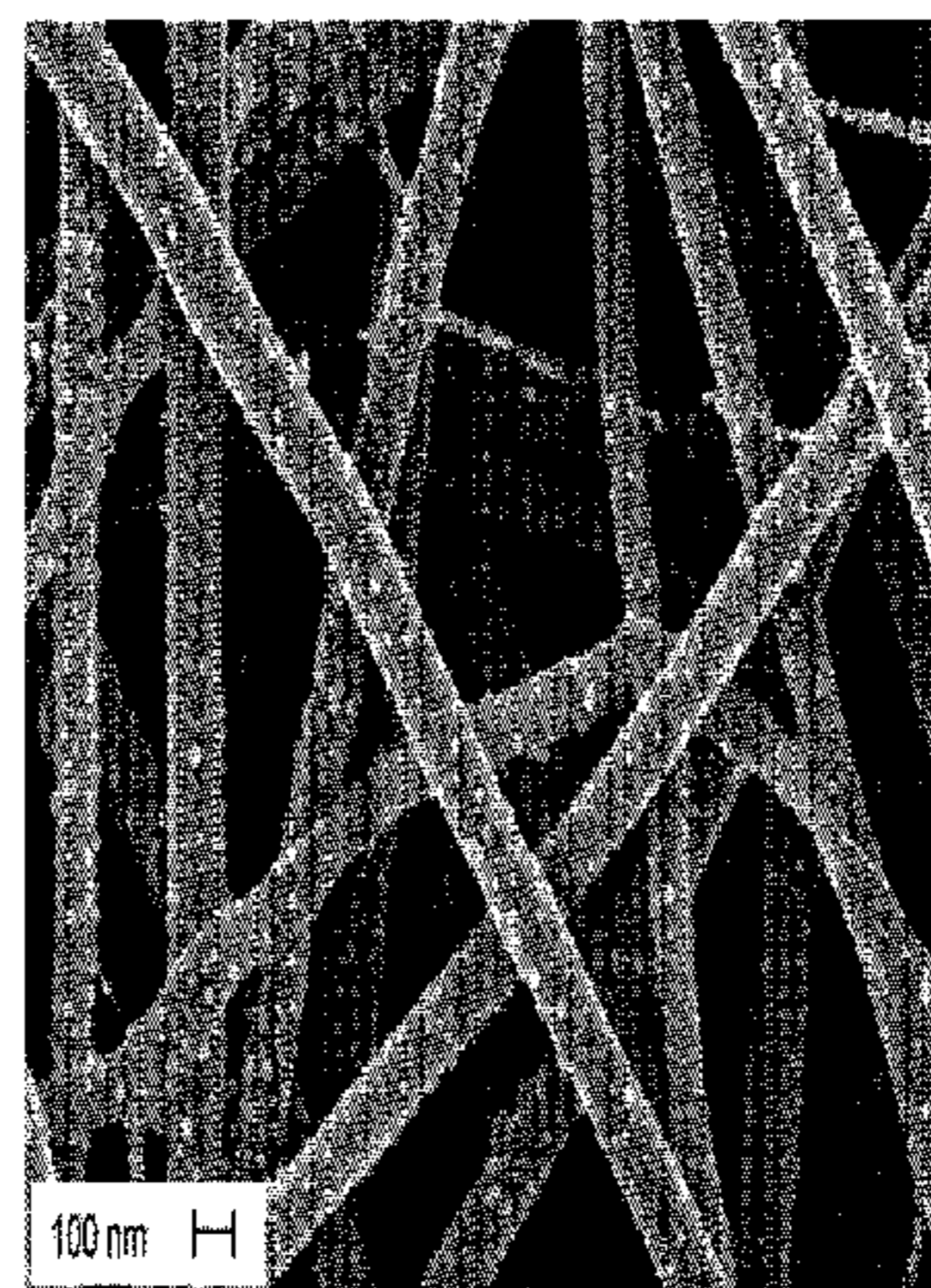
Keek SEM WD = 3 mm EHT = 2.00KV Aperture Size = 20.00µm Date: 2 Feb 2007 Mag = 60.00 KX File Name = Ag-Hylon6-pH4-02.tif Signal A = InLens Time: 11:37:47
