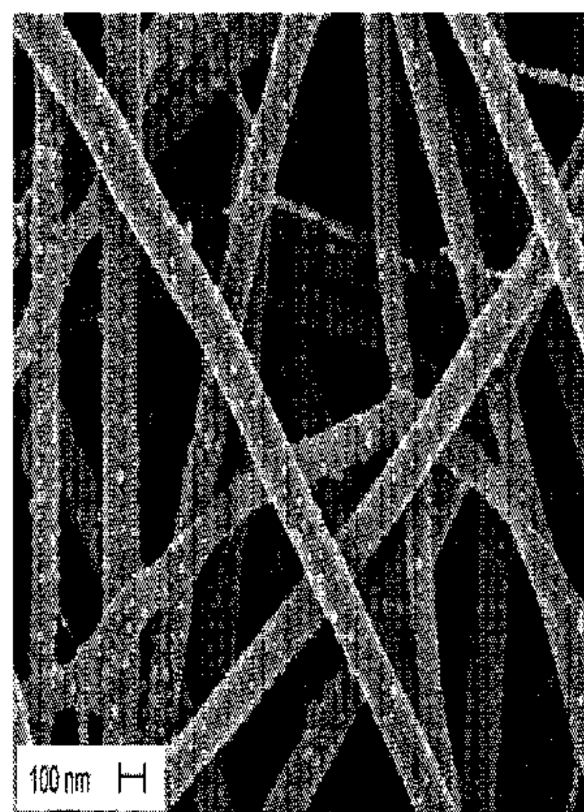
Keek SEM WD = 3 mm EHT = 2.00KV Aperture Size = 20.00µm Date: 2 Feb 2007 Mag = 60.00 KX File Name = Ag-Hylon6-pH4-02.tif Signal A = InLens Time: 11:37:47
