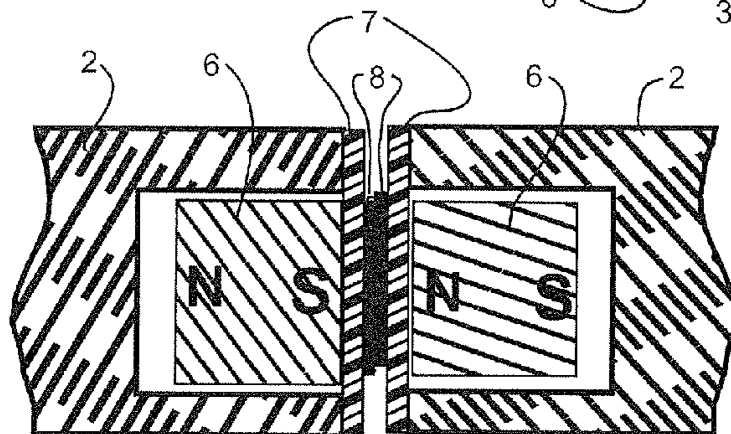
FIG. 10 SECTION B-B
