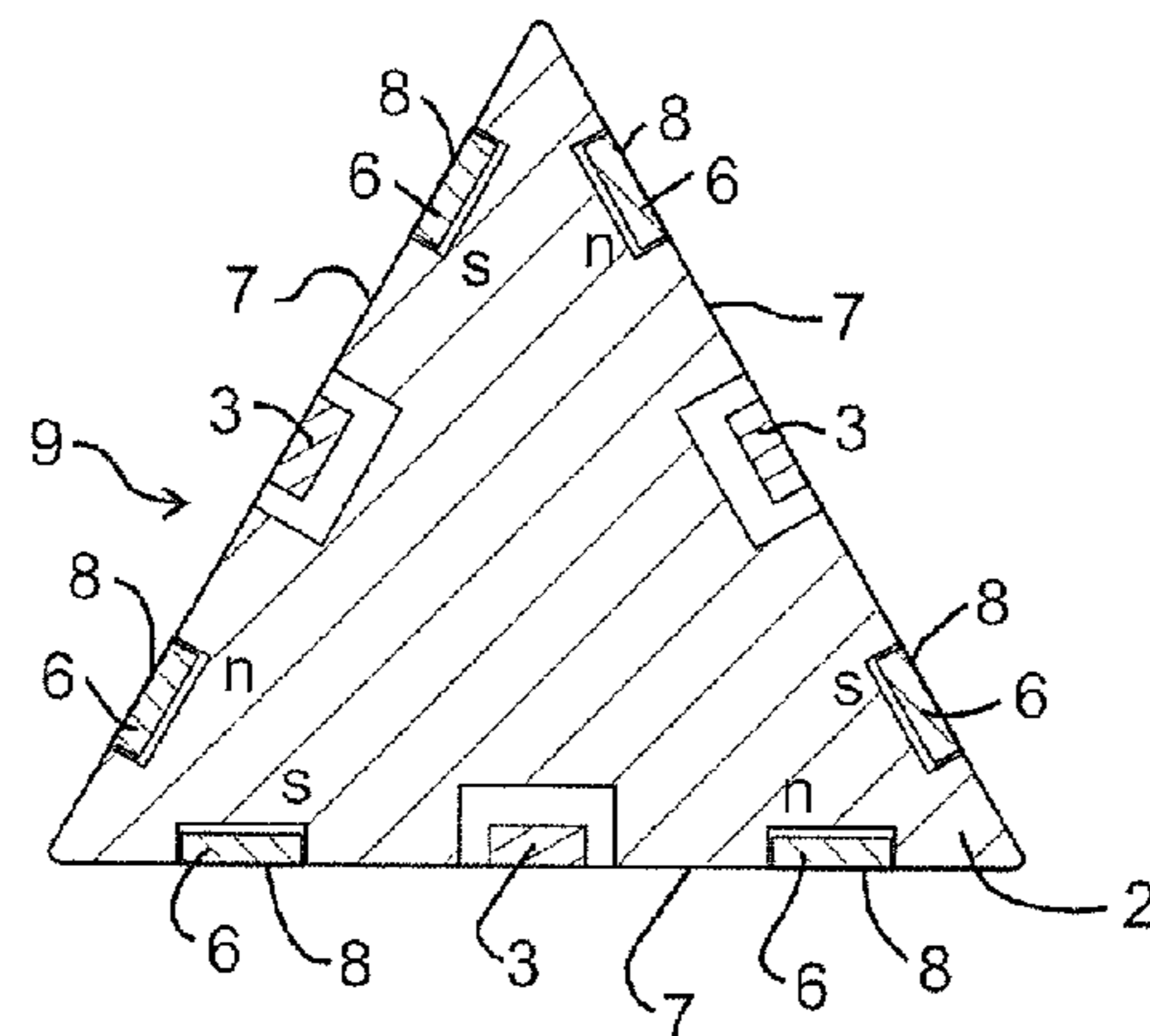
FIG. 5 SECTION C-C
