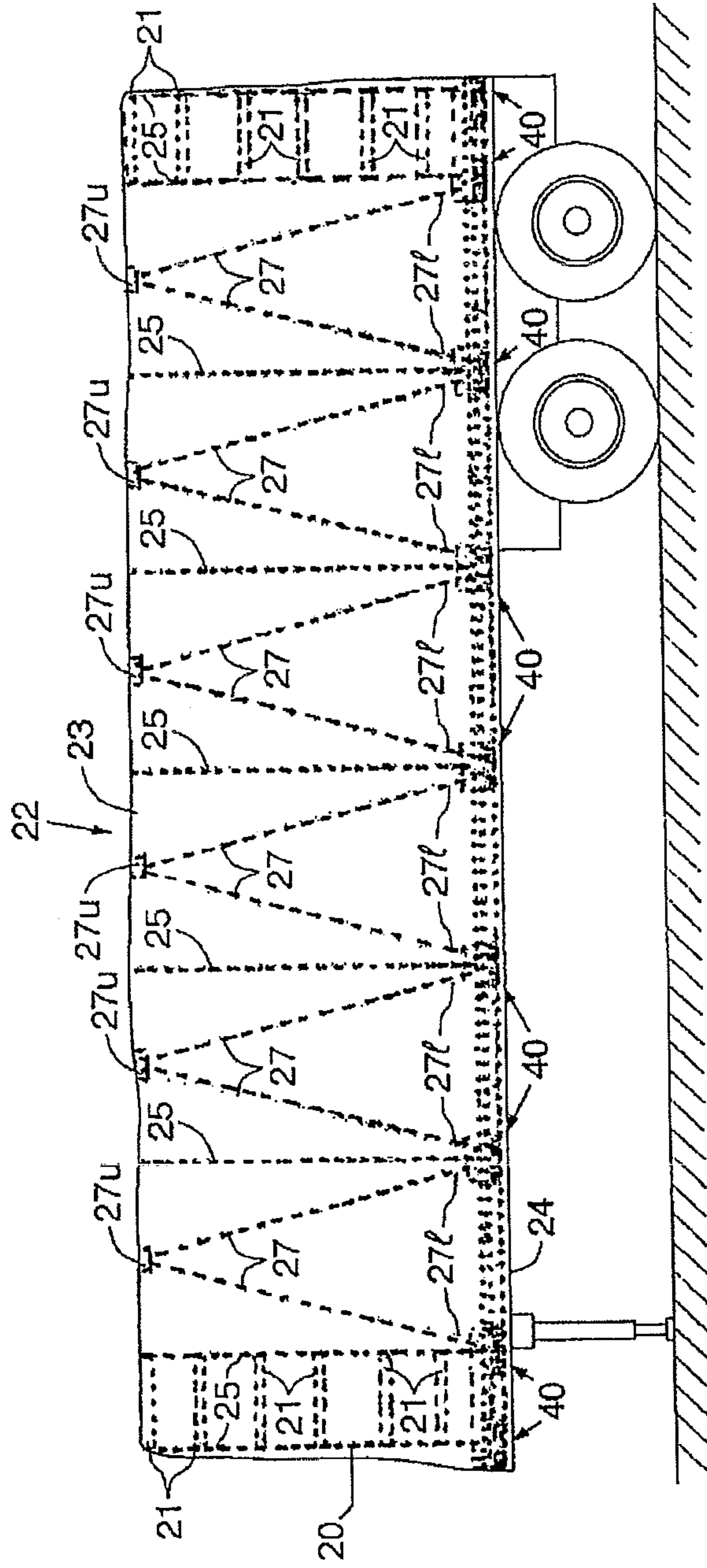
Fig. 2 PRIOR ART
