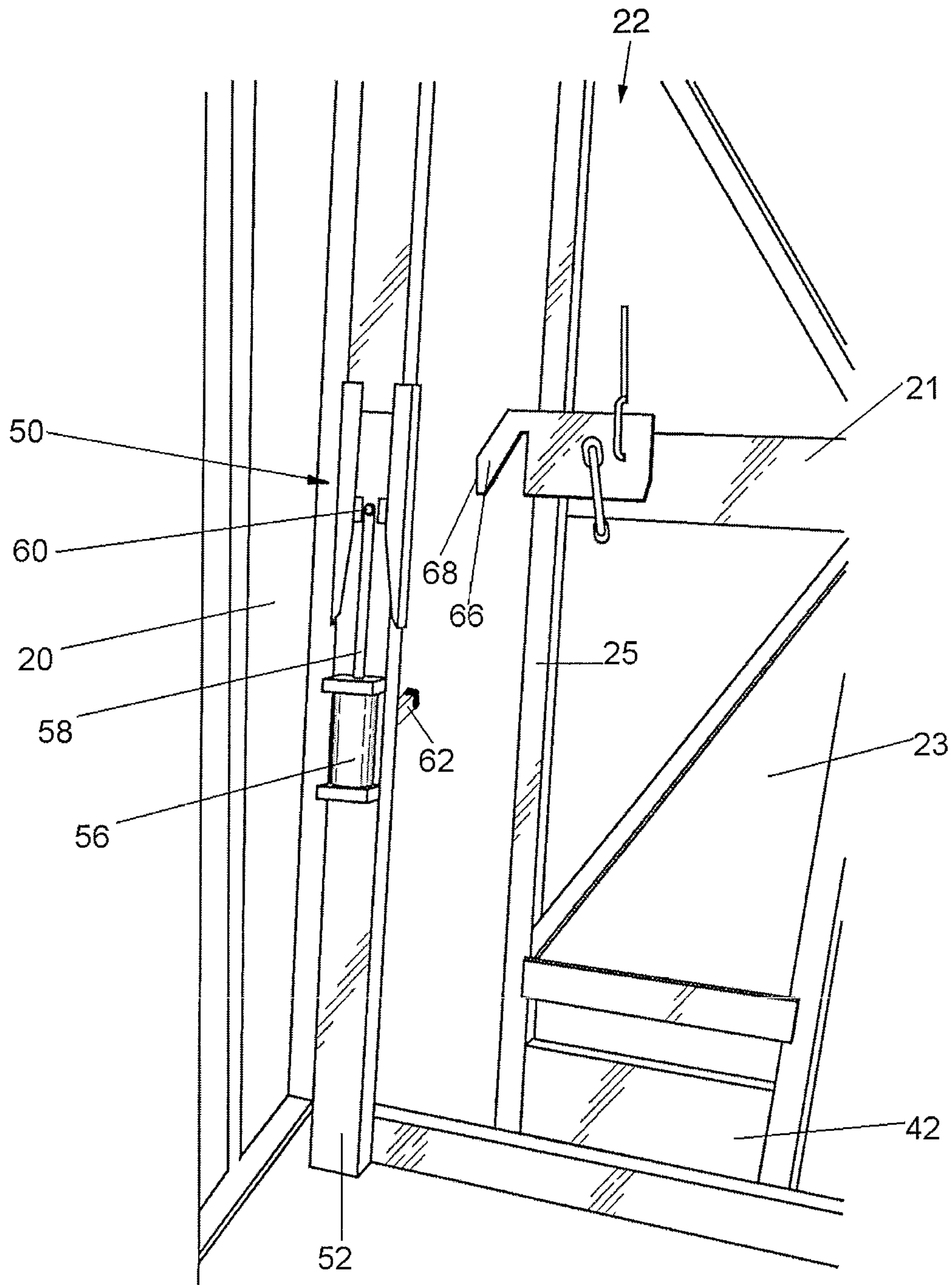
Fig. 3 PRIOR ART
