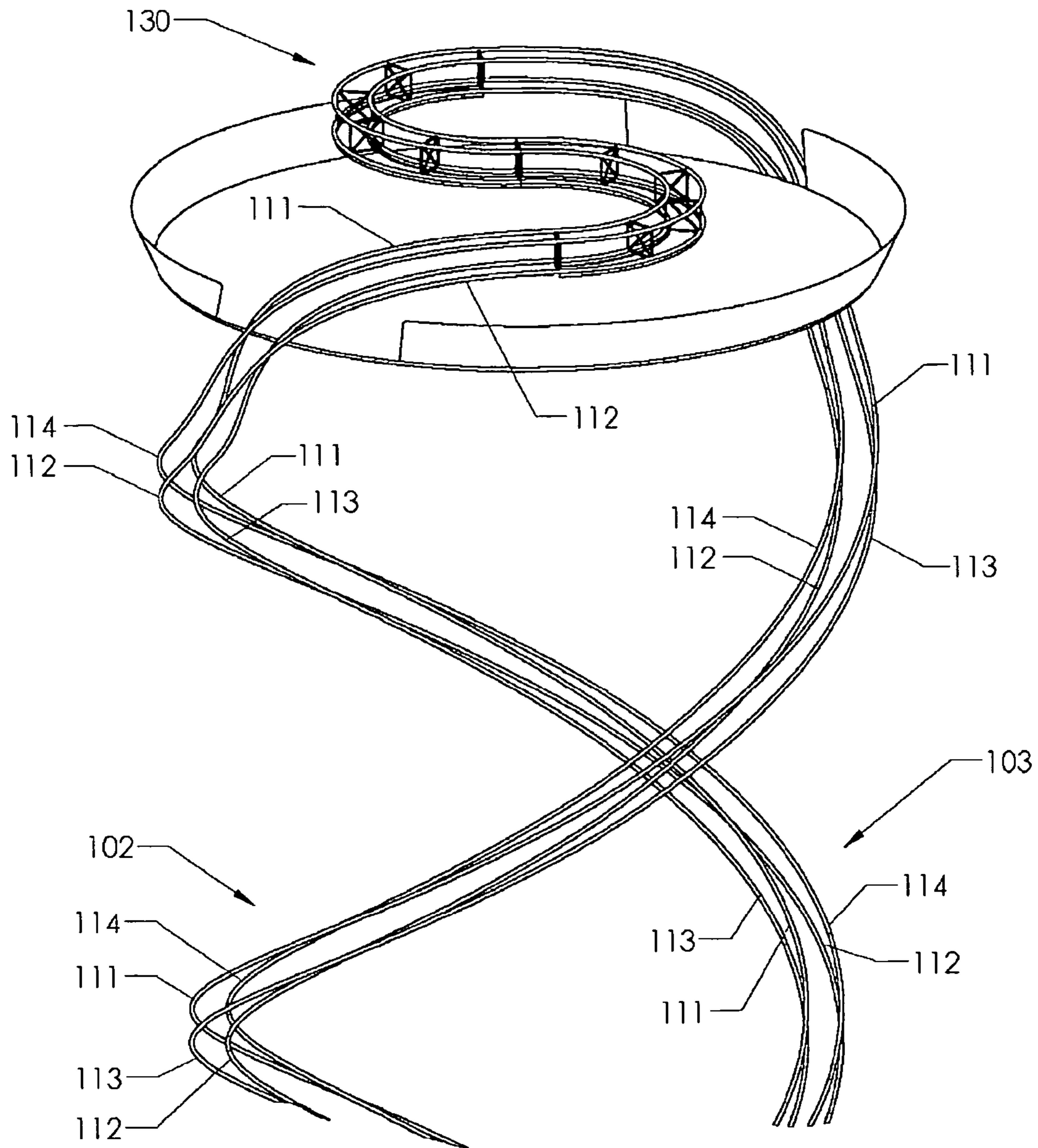
FIGURE 5
