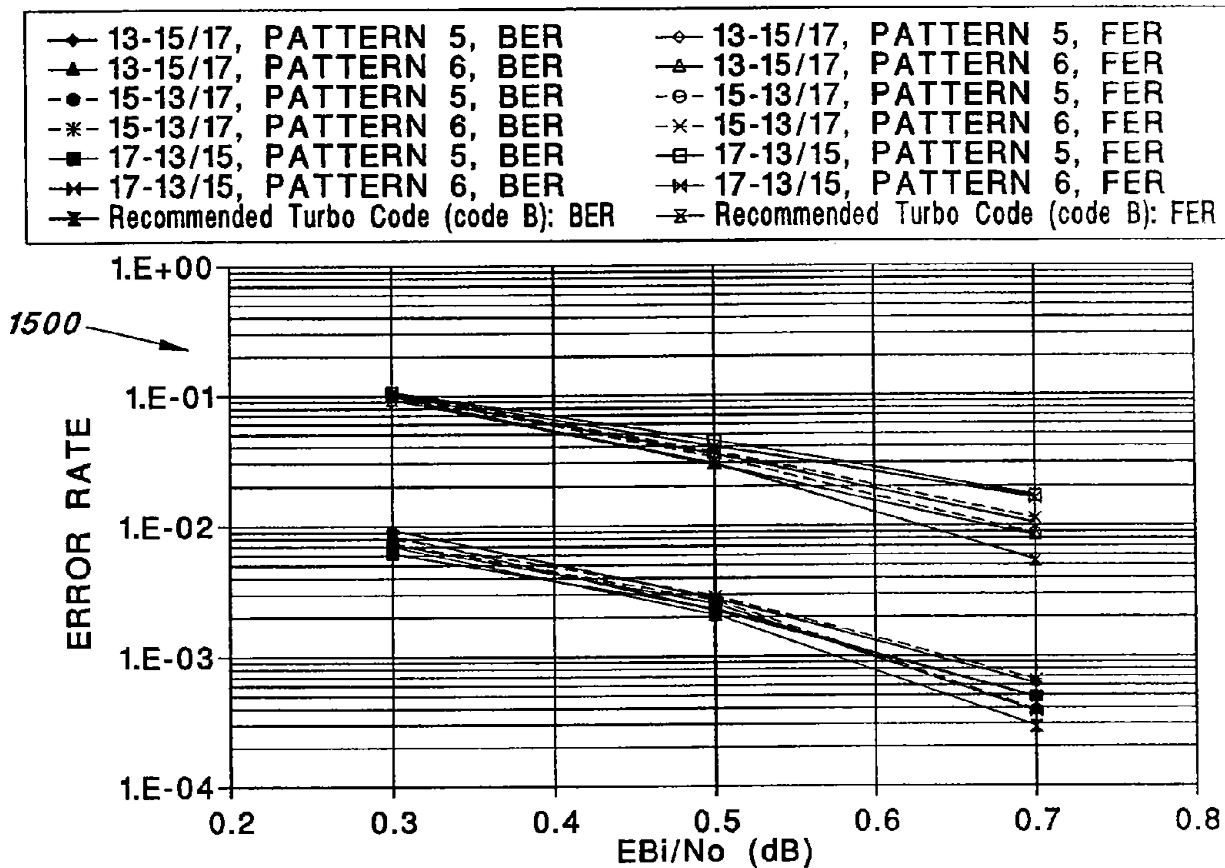
FIG. 15 COMPARISON AGAINST OTHER PUNCTURING SCHEMES, FRAME=512
