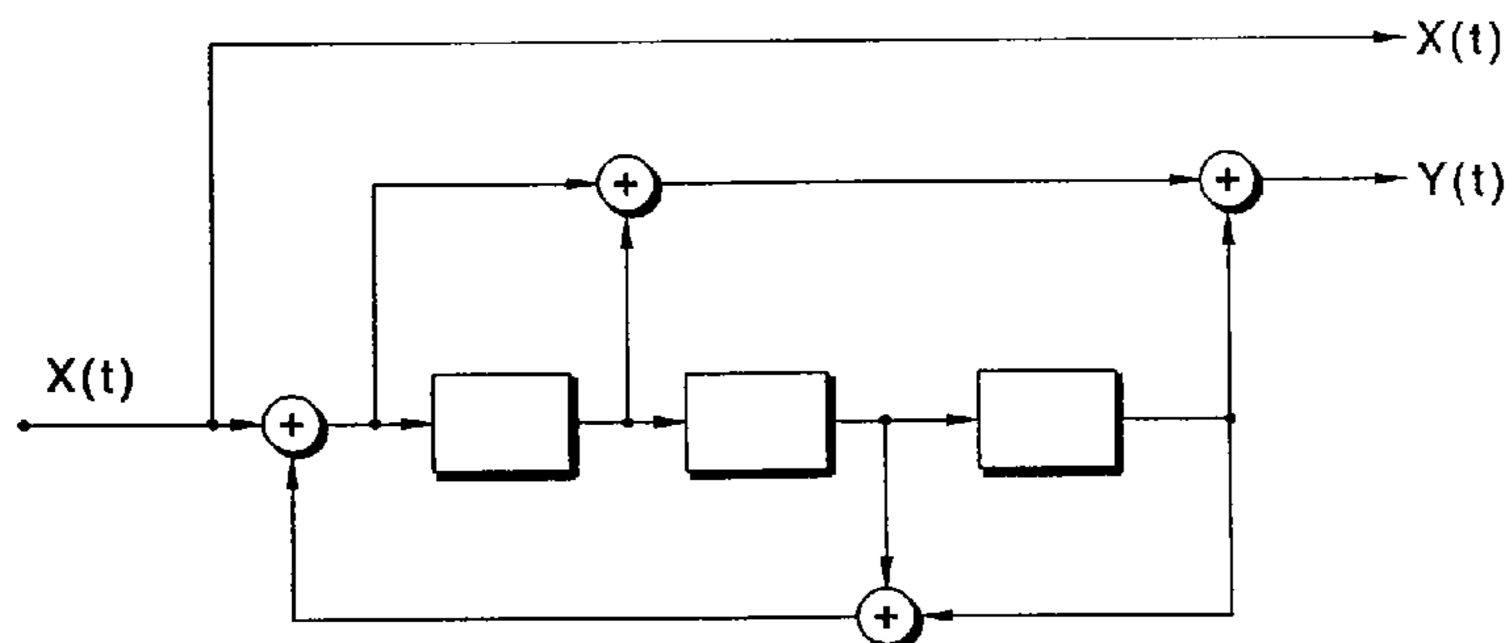
UNIVERSAL CONSTITUENT ENCODER RECOMMENDED FOR R=1/2 AND R=1/3 TURBO CODES OF VARYING INTERLEAVER DEPTH
